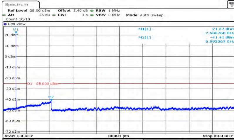
Band38-20MHz-16QAM-38000-1RB#0-Range2:1000~30000MHz
