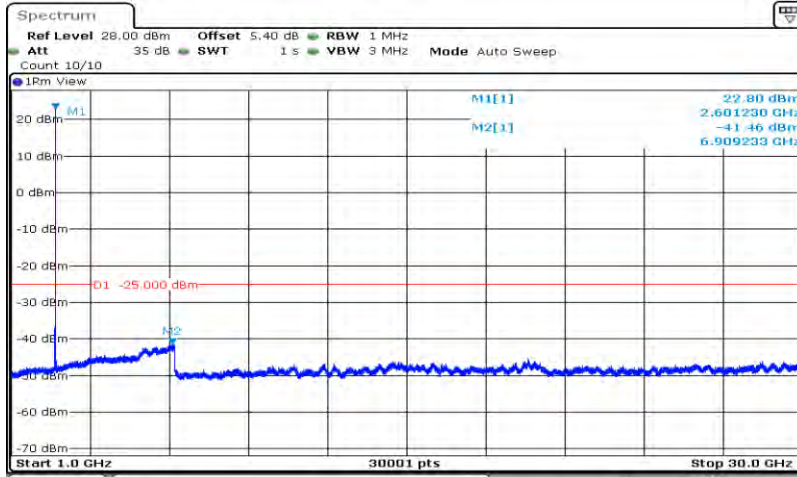
Band38-20MHz-64QAM-38150-1RB#0-Range2:1000~30000MHz
