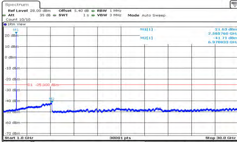
Band38-20MHz-64QAM-38000-1RB#0-Range2:1000~30000MHz
