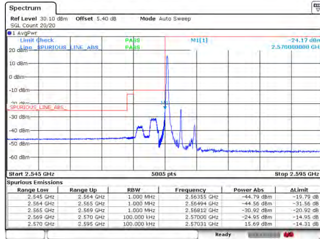
Band38_5MHz_QPSK_37775_1RB#0
