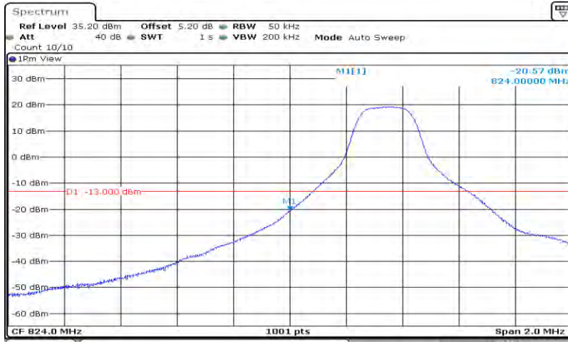
Band 26_5MHz_16QAM_26815_25RB#0
