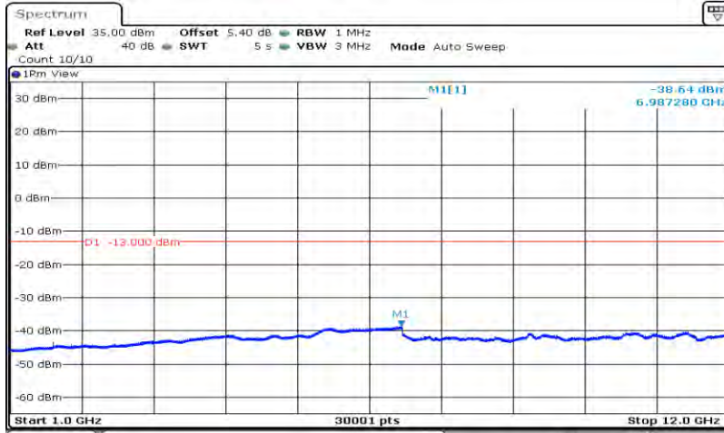
Band26-15MHz-16QAM-26865-1RB#0-Range2:1000~12000MHz
