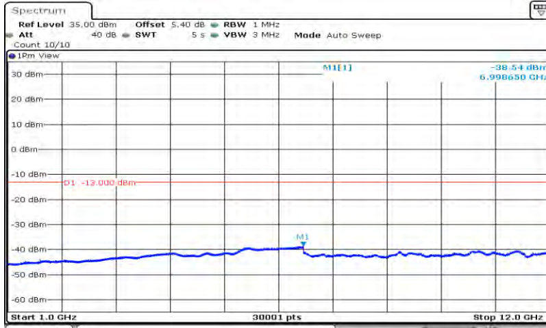
Band26-15MHz-64QAM-26865-1RB#0-Range2:1000~12000MHz
