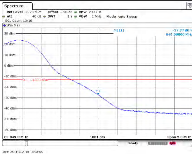
Band 26_15MHz_QPSK_26965_75RB#0
