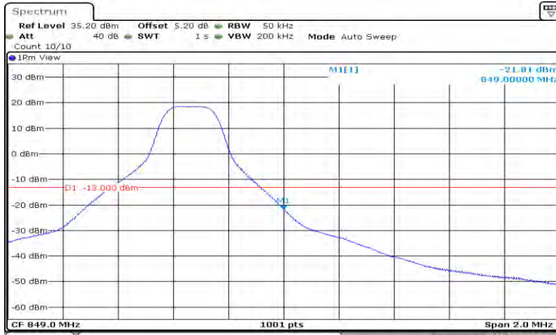
Band 26_5MHz_16QAM_27015_25RB#0
