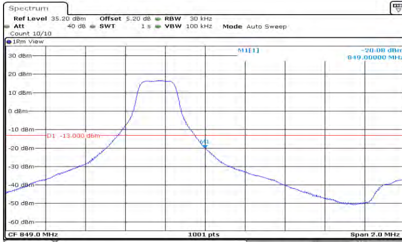
Band 26_3MHz_16QAM_27025_15RB#0
