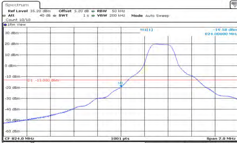
Band 26_5MHz_QPSK_26815_25RB#0
