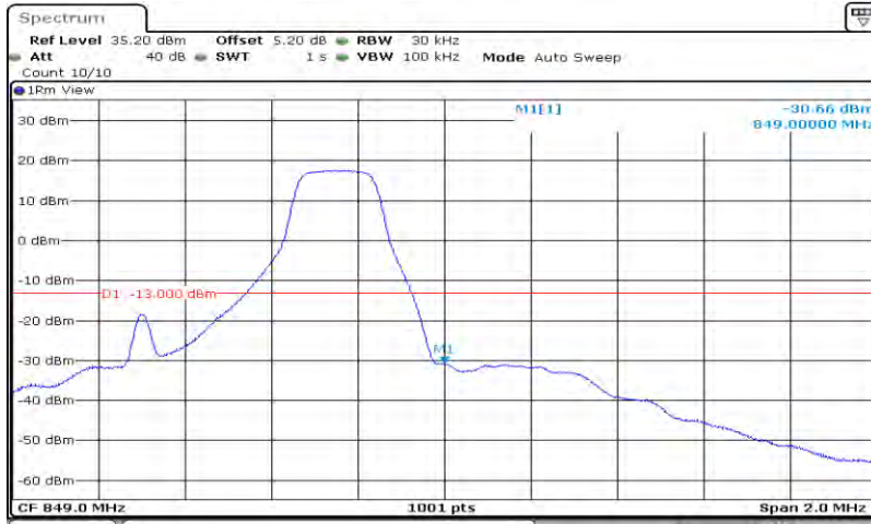
Band 26_1.4MHz_QPSK_27033_6RB#0
