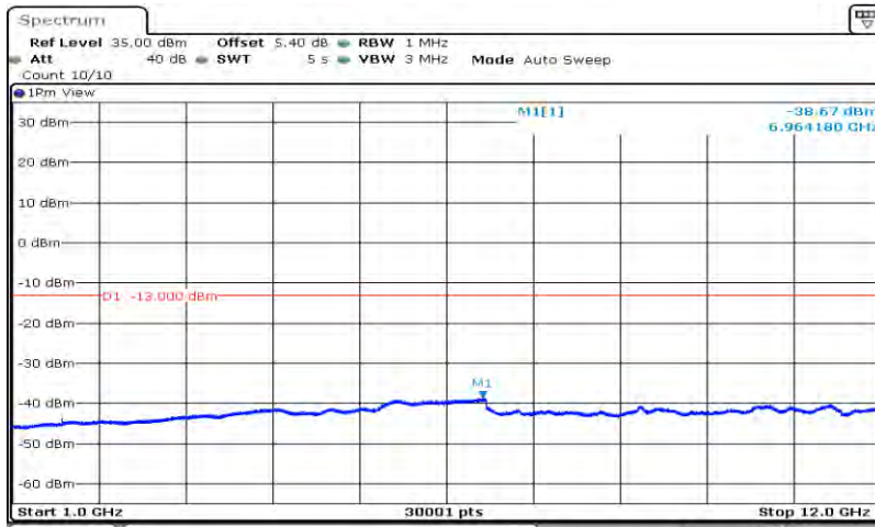
Band26-10MHz-64QAM-26740-1RB#0-Range2:1000~12000MHz
