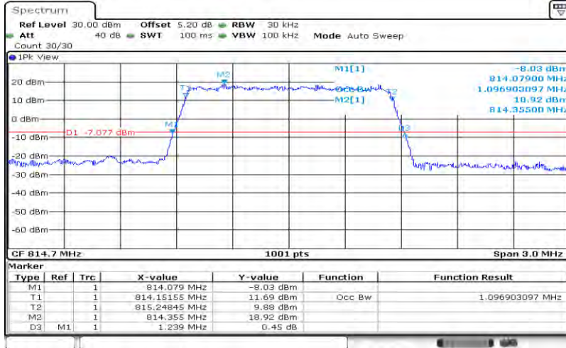
Band26-1.4MHz-QPSK-26697-6RB#0-1.097
