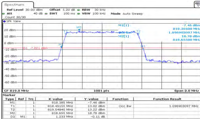
Band26-1.4MHz-QPSK-26740-6RB#0-1.097
