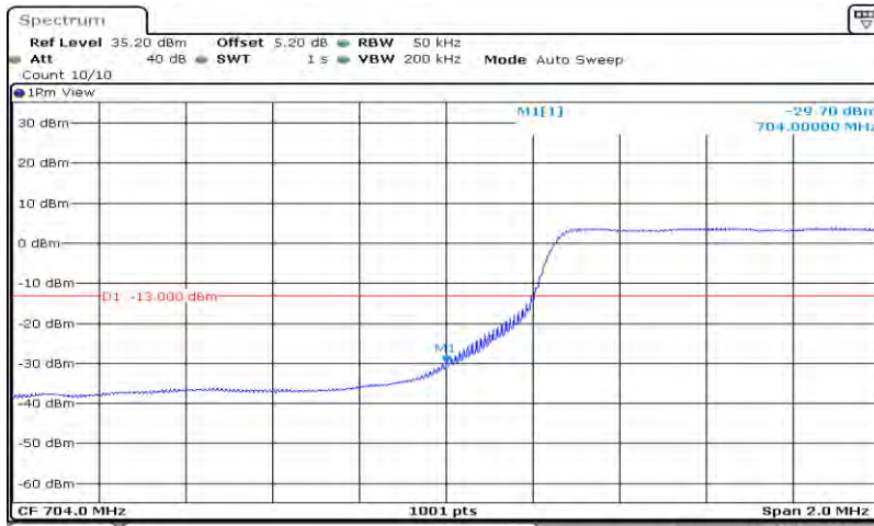
Band17-5MHz-64QAM-23755-25RB#0
