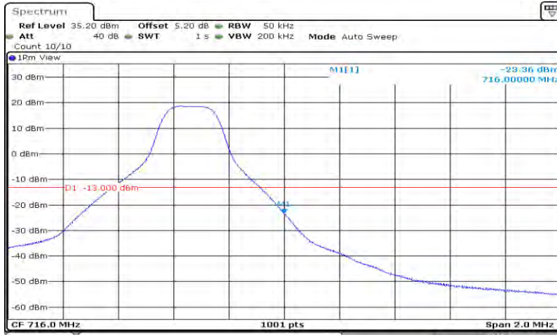
Band17-5MHz-16QAM-23825-25RB#0
