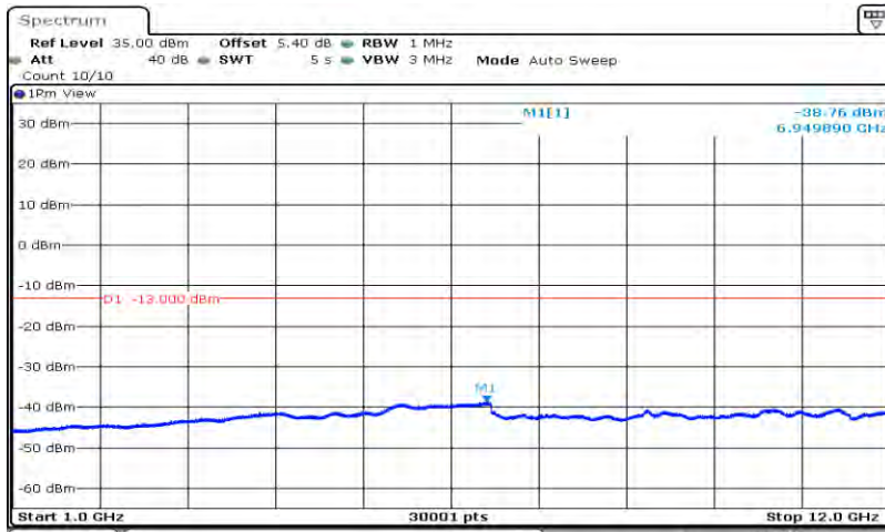
Band17-10MHz-64QAM-23780-1RB#0-Range2:1000~12000MHz
