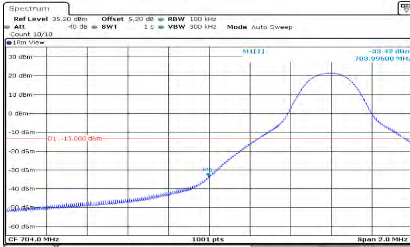
Band17-10MHz-64QAM-23780-50RB#0
