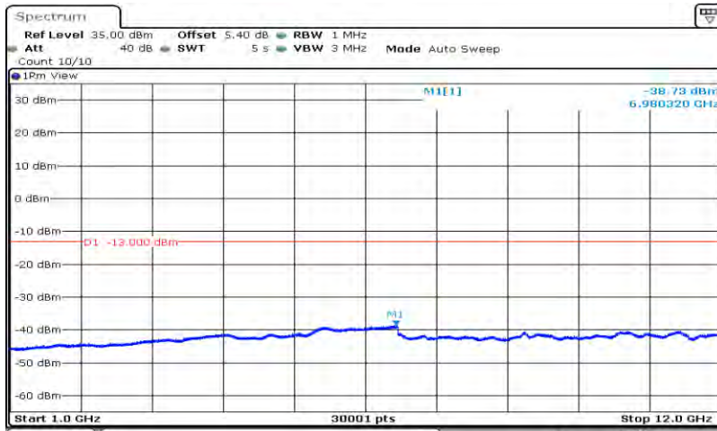
Band17-10MHz-16QAM-23780-1RB#0-Range2:1000~12000MHz
