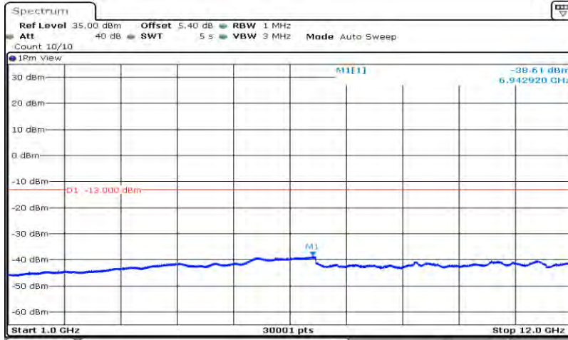
Band17-10MHz-16QAM-23790-1RB#0-Range2:1000~12000MHz
