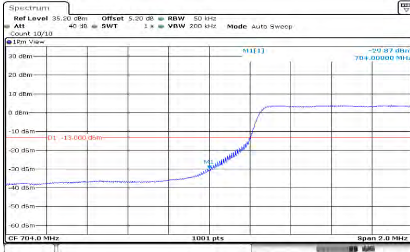
Band17-5MHz-16QAM-23755-25RB#0
