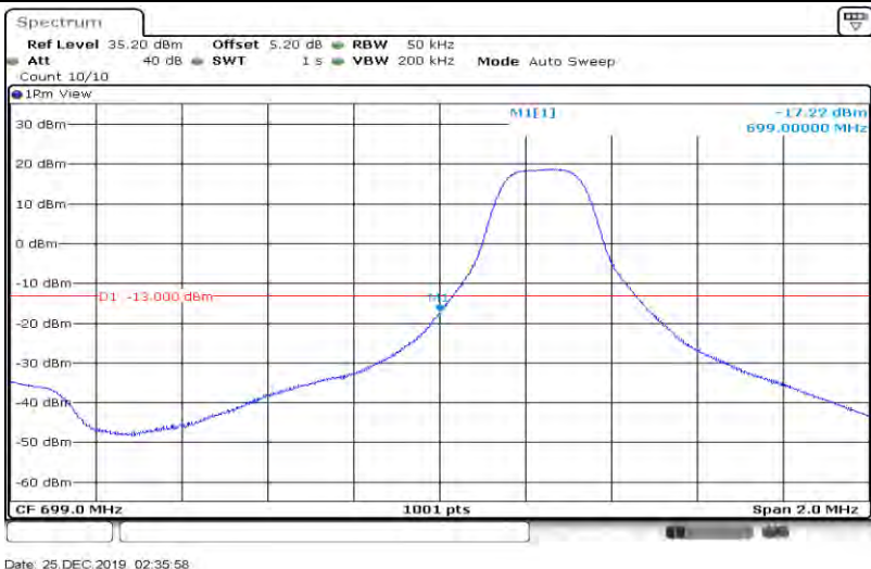
Band12-3MHz-16QAM-23025-15RB#0
