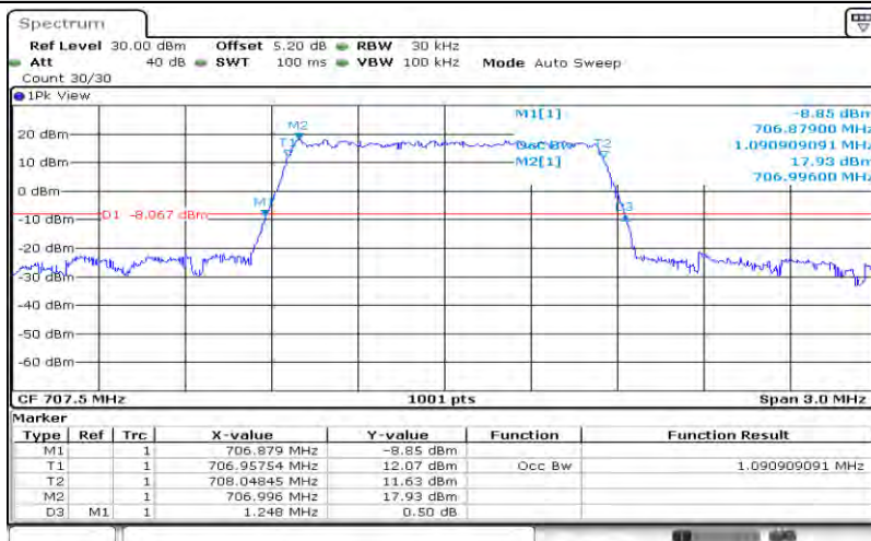
Band12-1.4MHz-QPSK-23095-6RB#0-1.091
