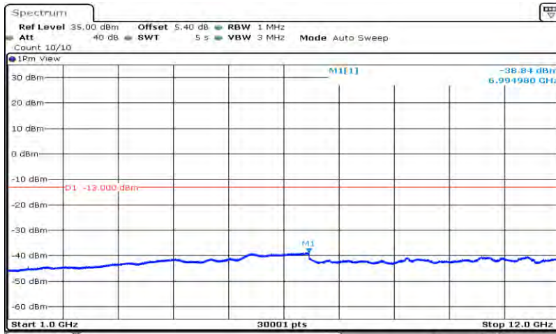
Band12-10MHz-64QAM-23095-1RB#0-Range2:1000~12000MHz
