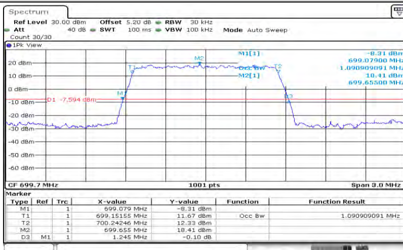
Band12-1.4MHz-QPSK-23017-6RB#0-1.091
