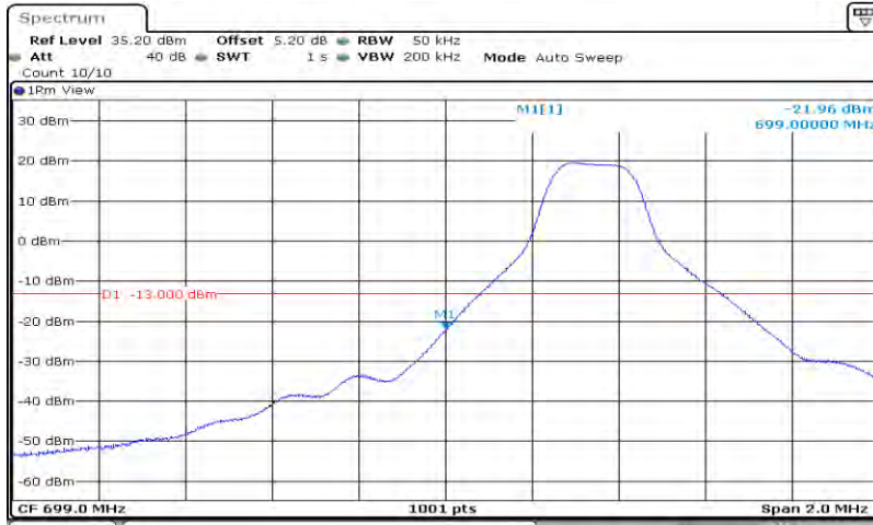
Band12-5MHz-QPSK-23035-25RB#0
