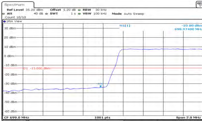
Band12-1.4MHz-16QAM-23017-6RB#0
