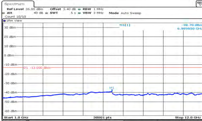
Band12-10MHz-64QAM-23130-1RB#0-Range2:1000~12000MHz
