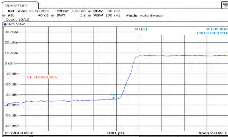
Band12-1.4MHz-64QAM-23017-6RB#0
