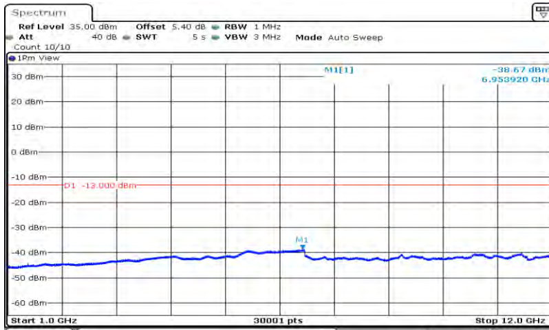
Band12-10MHz-16QAM-23095-1RB#0-Range2:1000~12000MHz
