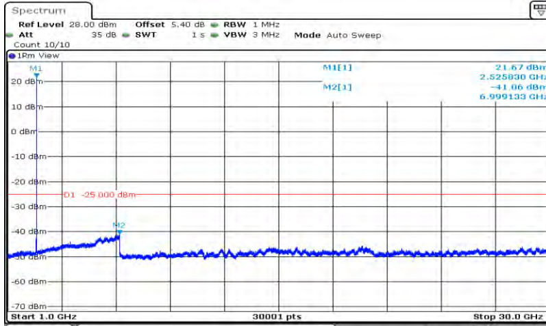
Band7-20MHz-16QAM-21100-1RB#0-Range2:1000~30000MHz
