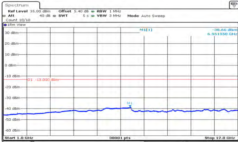
Band5-10MHz-16QAM-20450-1RB#0-Range2:1000~12000MHz
