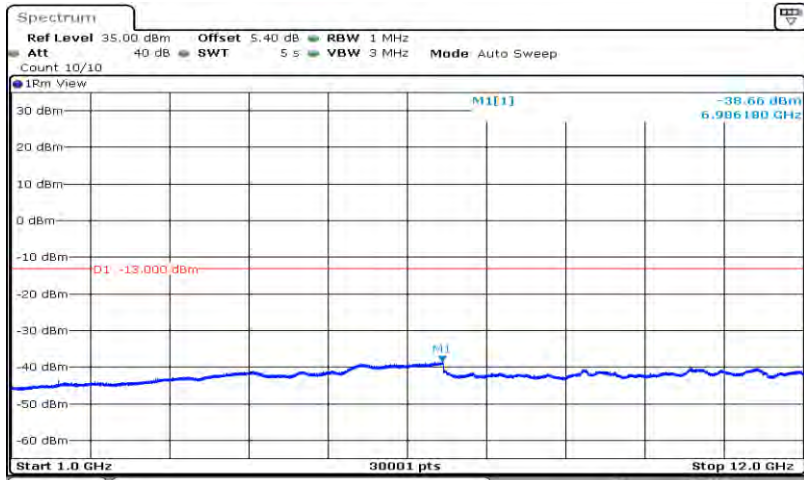
Band5-10MHz-64QAM-20450-1RB#0-Range2:1000~12000MHz
