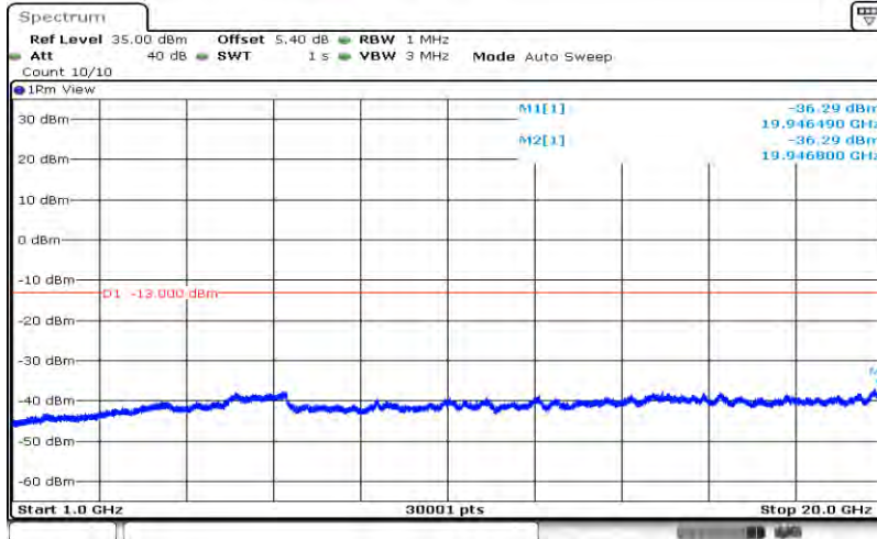
Band4-20MHz-64QAM-20050-1RB#0-Range2:1000~20000MHz
