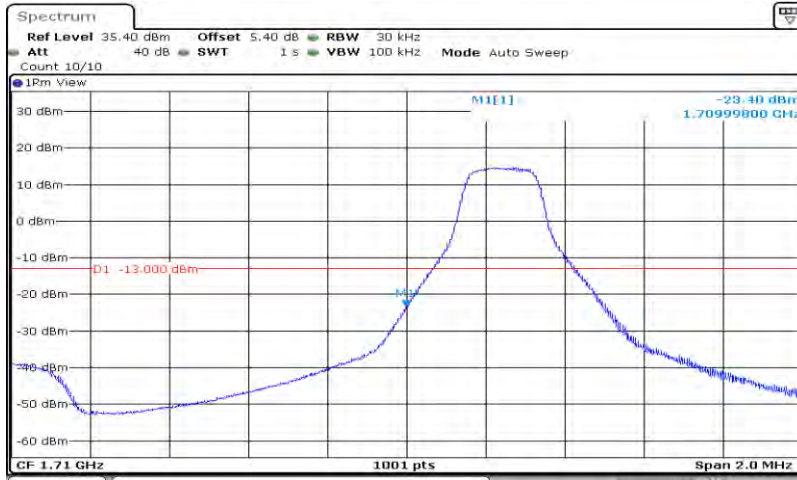
Band4-3MHz-64QAM-19965-15RB#0
