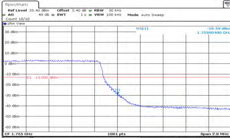
Band4-3MHz-QPSK-20385-15RB#0
