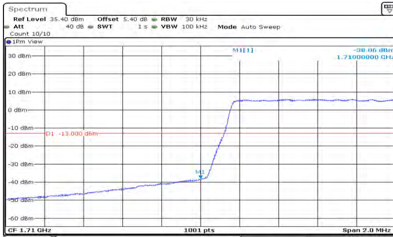
Band4-1.4MHz-16QAM-19957-6RB#0
