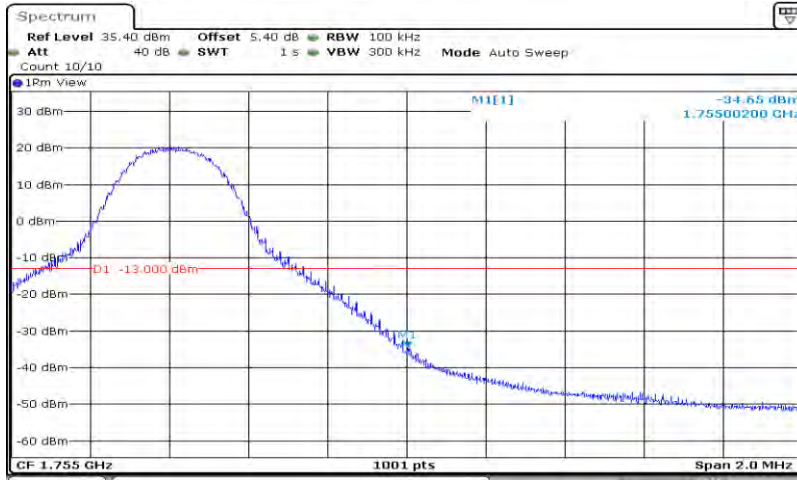
Band4-10MHz-16QAM-20350-50RB#0
