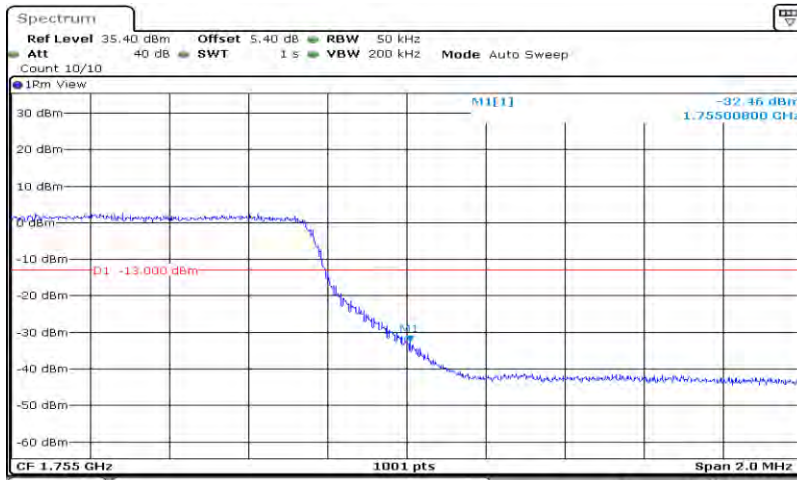
Band4-5MHz-16QAM-20375-25RB#0
