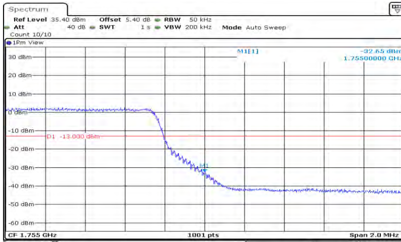
Band4-5MHz-64QAM-20375-25RB#0
