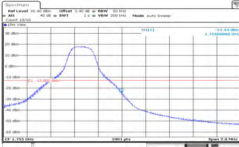
Band4-5MHz-QPSK-20375-25RB#0
