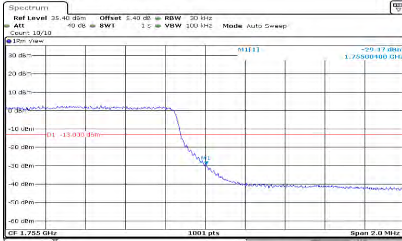
Band4-3MHz-16QAM-20385-15RB#0
