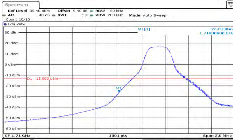
Band4-5MHz-64QAM-19975-25RB#0
