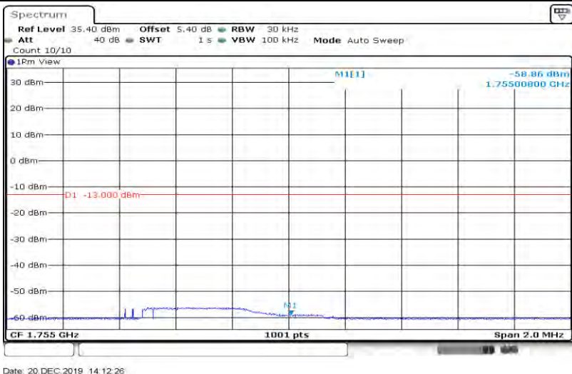
Band4-1.4MHz-64QAM-20393-6RB#0
