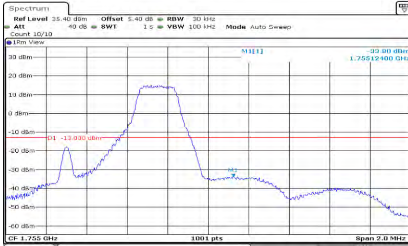
Band4-1.4MHz-16QAM-20393-6RB#0
