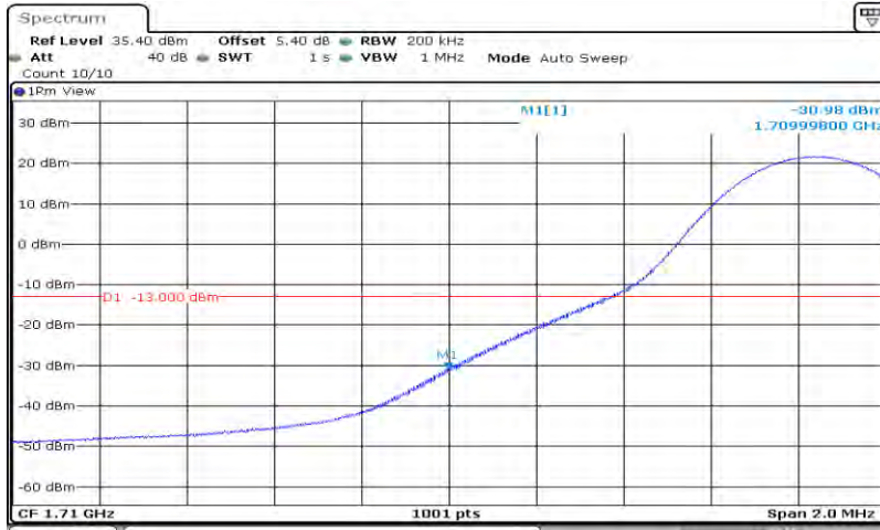
Band4-15MHz-16QAM-20025-75RB#0
