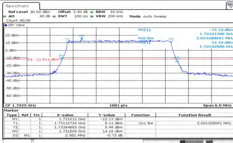
Band4-3MHz-64QAM-20175-15RB#0-2.691
