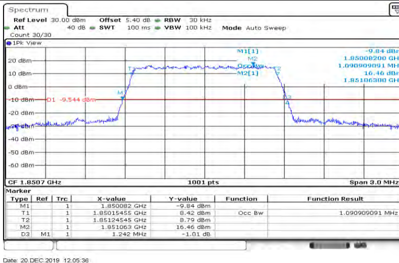
Band2-1.4MHz-QPSK-18900-6RB#0-1.094
