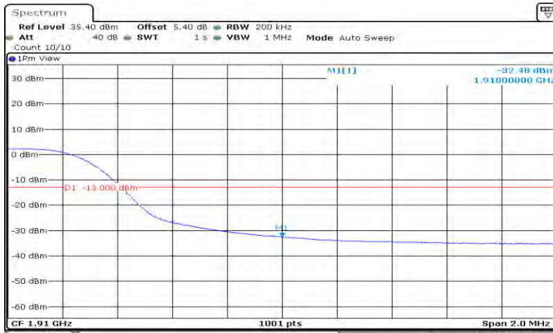
Band2-15MHz-64QAM-19125-75RB#0
