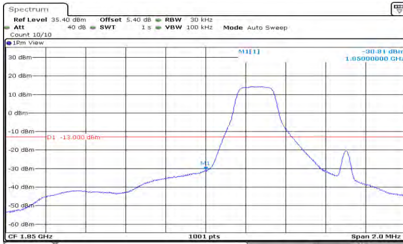
Band2-1.4MHz-64QAM-18607-6RB#0
