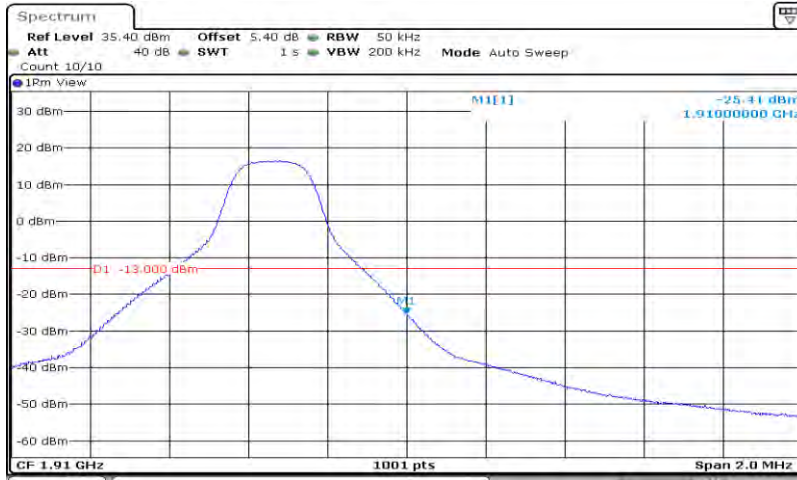
Band2-5MHz-64QAM-19175-25RB#0
