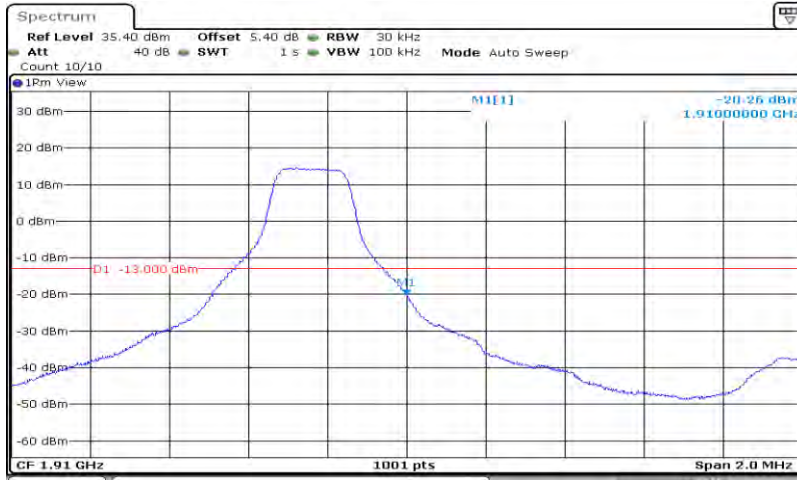
Band2-3MHz-16QAM-19185-15RB#0
