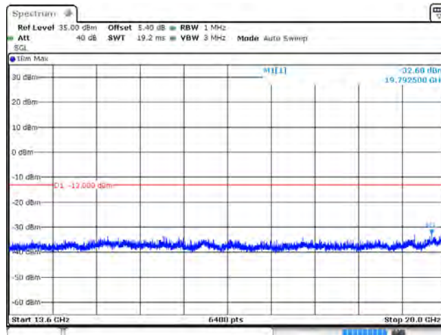
EGPRS1900_512
