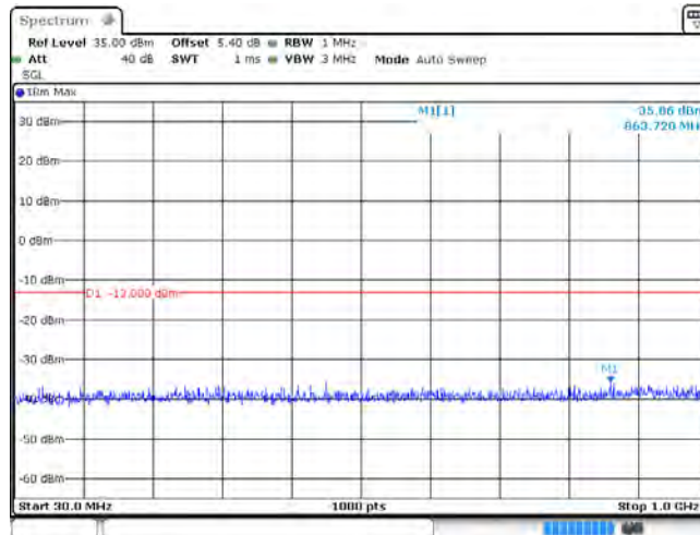
GSM1900_512
