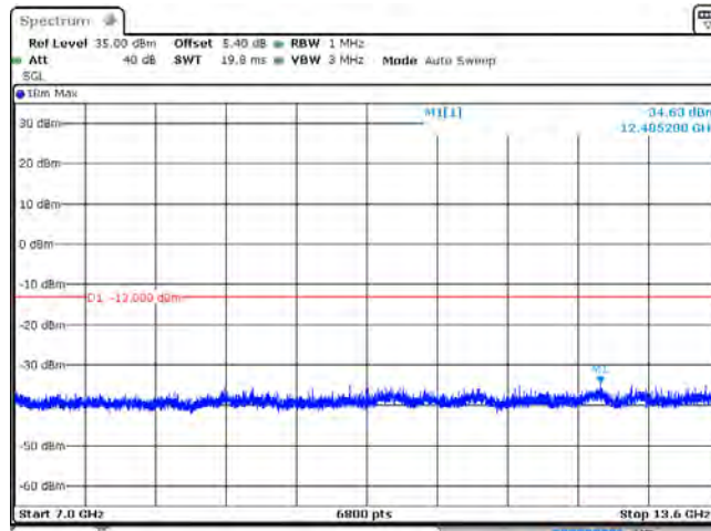
EGPRS1900_512
