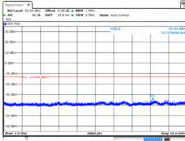
GSM1900_512
