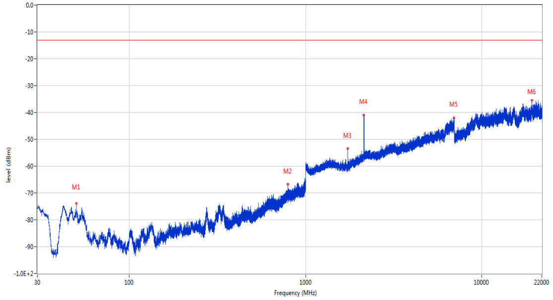
OPPO 特殊要求_RSE Test case_FCC PART22&24&27_FCC PART 27_1700_WCDMA B4&LTE B4
