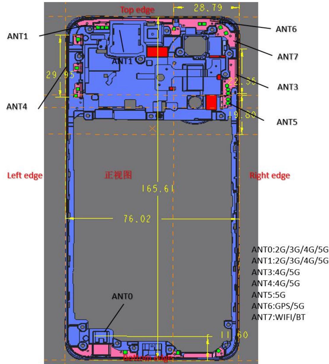
Fig 1 Antenna location&dimension
