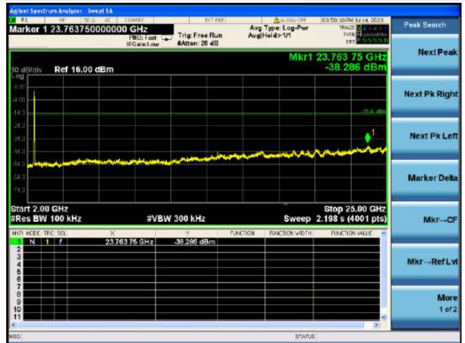
802.11n-20 MHz CHANNEL 10, SPURIOUS 2 GHz ~ 25 GHz
