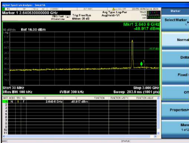
802.11n-20 MHz CHANNEL 11, SPURIOUS 30 MHz ~ 3 GHz
