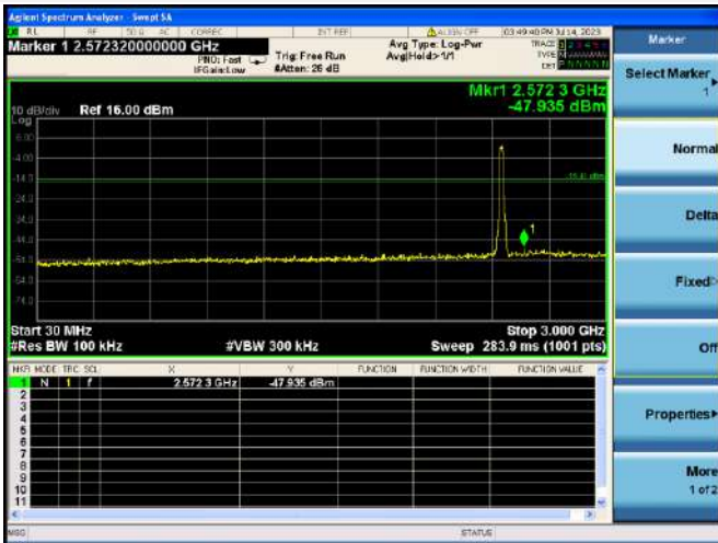
802.11n-20 MHz CHANNEL 10, SPURIOUS 30 MHz ~ 3 GHz
