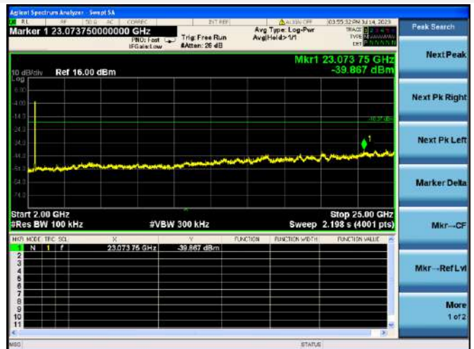
802.11n-20 MHz CHANNEL 11, SPURIOUS 2 GHz ~ 25 GHz
