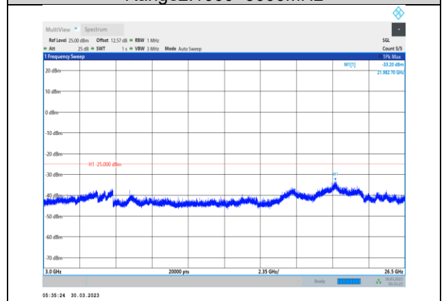
Band38-5MHz-QPSK-38000-1RB#0- Range3:3000~26500MHz
