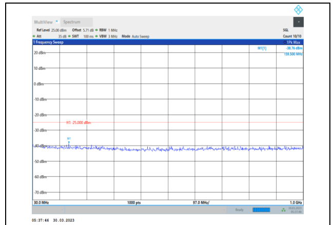
Band38-5MHz-16QAM-38225-1RB#0- Range1:30~1000MHz
