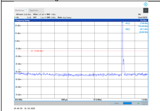
Band26-10MHz-16QAM-26740-1RB#0- Range1:30~1000MHz
