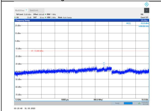
Band26-3MHz-16QAM-26705-1RB#0- Range2:1000~10000MHz
