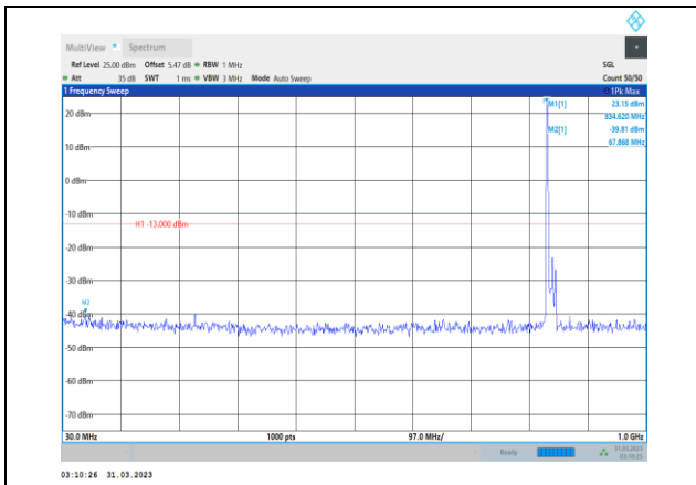
Band26-15MHz-QPSK-26965-1RB#0- Range1:30~1000MHz
