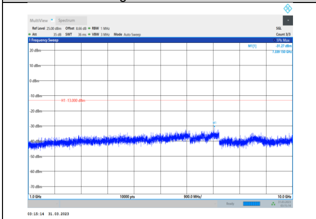
Band26-3MHz-QPSK-26705-1RB#0- Range2:1000~10000MHz
