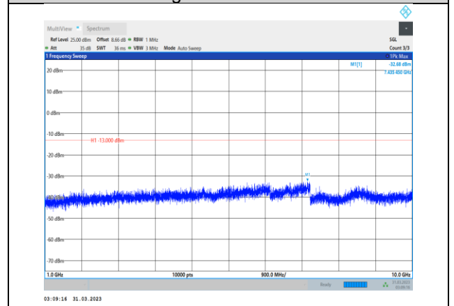
Band26-15MHz-QPSK-26915-1RB#0- Range2:1000~10000MHz
