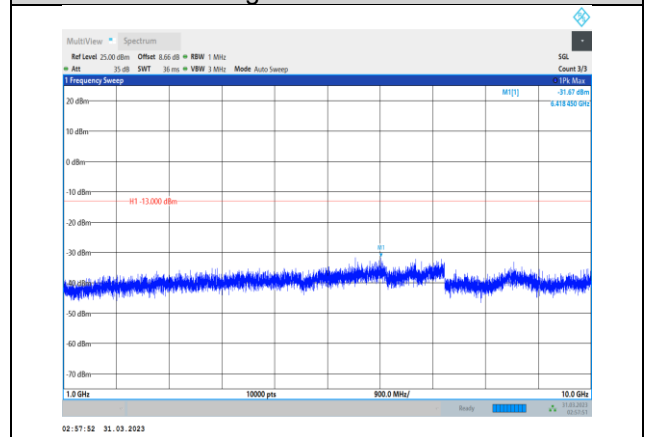
Band26-5MHz-64QAM-26765-1RB#0- Range2:1000~10000MHz
