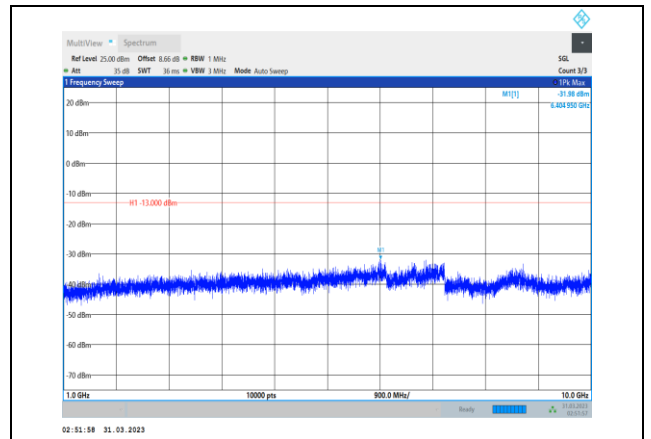
Band26-1.4MHz-64QAM-26740-1RB#0- Range2:1000~10000MHz
