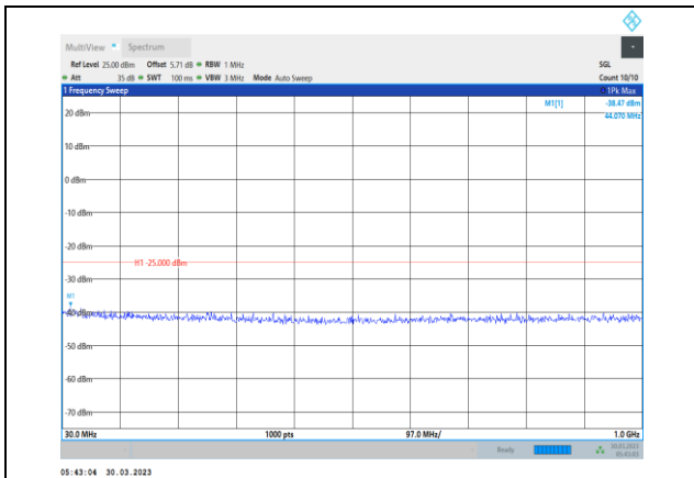
Band38-10MHz-64QAM-38000-1RB#0-Range1:30~1000MHz
