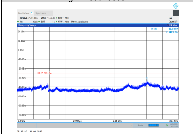
Band38-5MHz-QPSK-37775-1RB#0- Range3:3000~26500MHz
