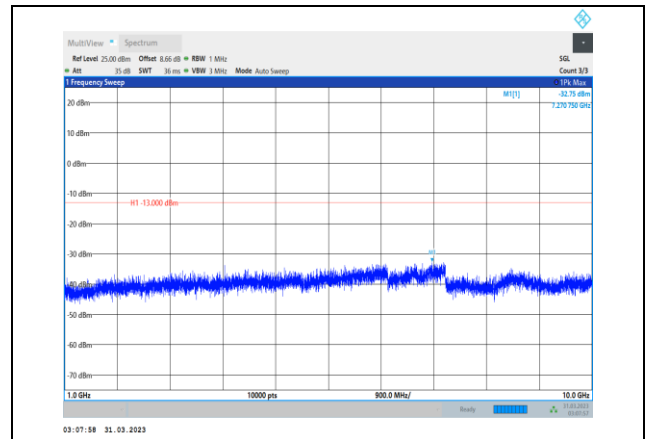
Band26-15MHz-QPSK-26865-1RB#0- Range2:1000~10000MHz
