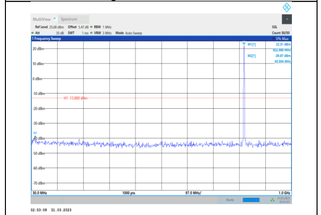
Band26-1.4MHz-64QAM-26783-1RB#0- Range1:30~1000MHz
