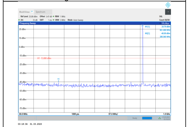
Band26-3MHz-64QAM-26775-1RB#0- Range1:30~1000MHz
