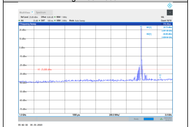
Band38-10MHz-16QAM-38000-1RB#0-Range2:1000~3000MHz
