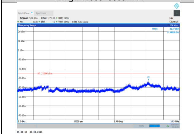
Band38-5MHz-64QAM-38225-1RB#0- Range3:3000~26500MHz
