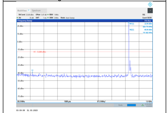
Band26-15MHz-QPSK-26915-1RB#0- Range1:30~1000MHz
