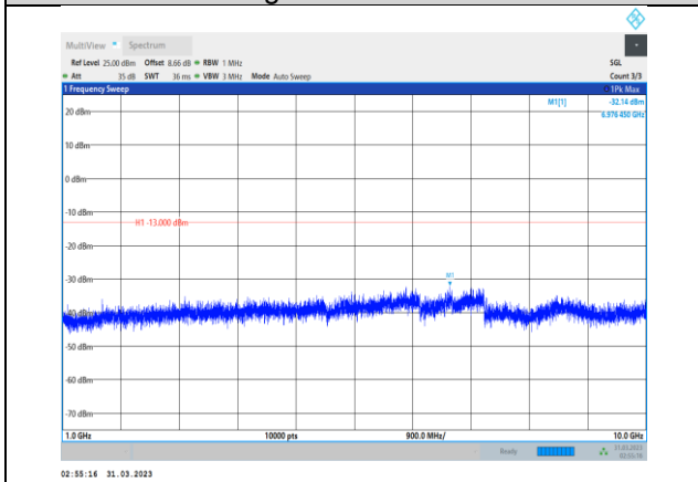
Band26-5MHz-64QAM-26715-1RB#0- Range2:1000~10000MHz
