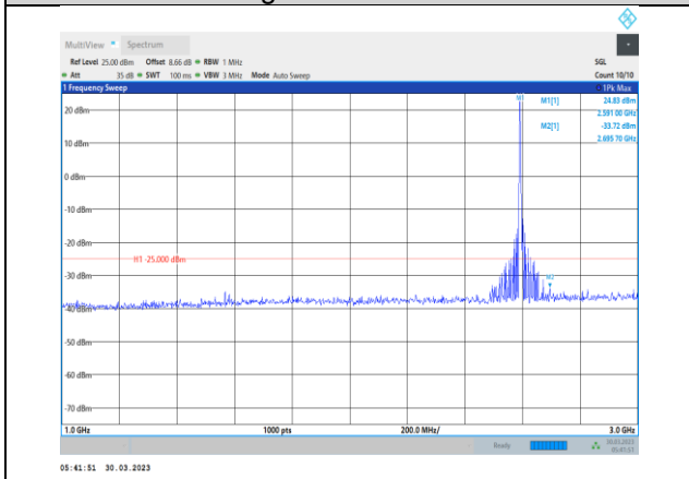
Band38-10MHz-QPSK-38000-1RB#0- Range2:1000~3000MHz
