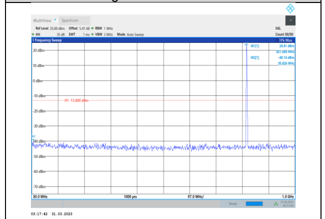
Band26-3MHz-QPSK-26775-1RB#0- Range1:30~1000MHz
