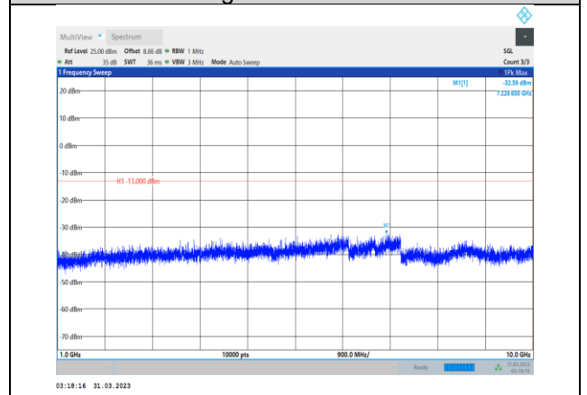
Band26-3MHz-16QAM-26775-1RB#0- Range2:1000~10000MHz
