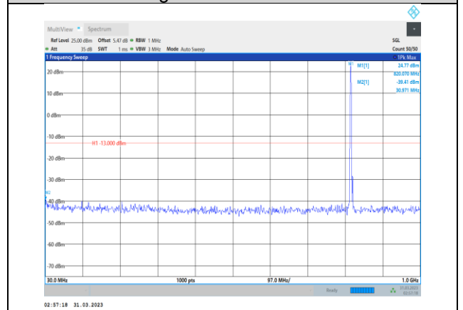
Band26-5MHz-16QAM-26765-1RB#0- Range1:30~1000MHz
