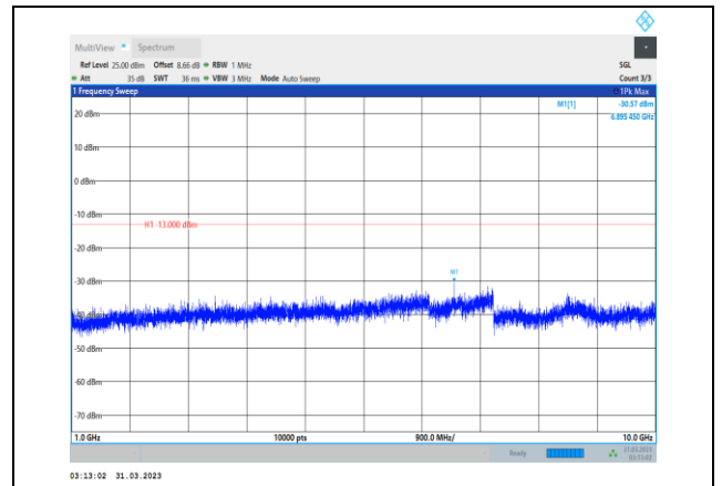
Band26-15MHz-16QAM-26765-1RB#0- Range2:1000~10000MHz
