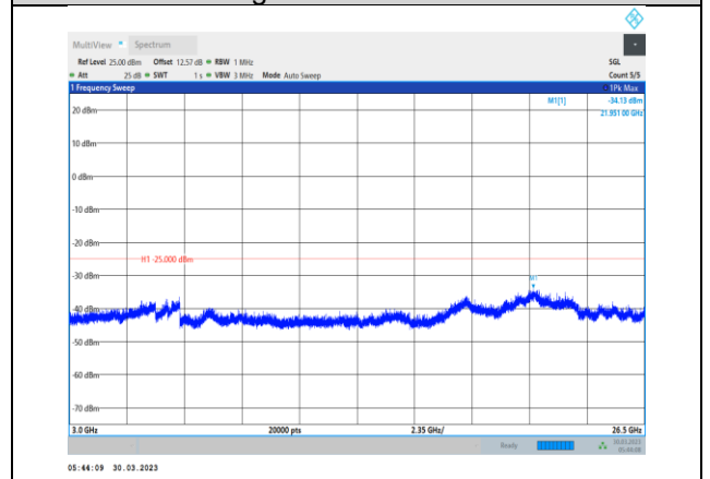
Band38-10MHz-QPSK-38200-1RB#0- Range3:3000~26500MHz
