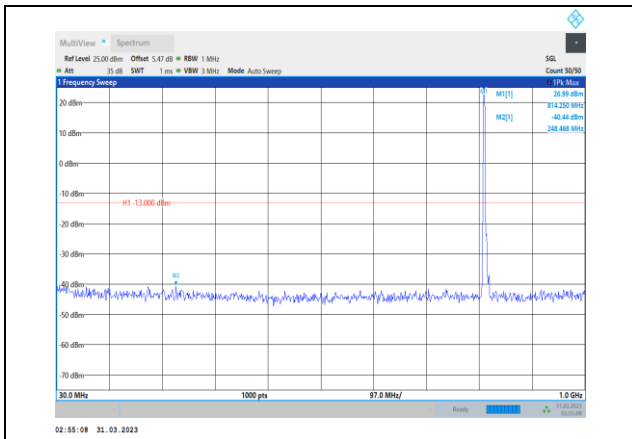
Band26-5MHz-64QAM-26715-1RB#0- Range1:30~1000MHz
