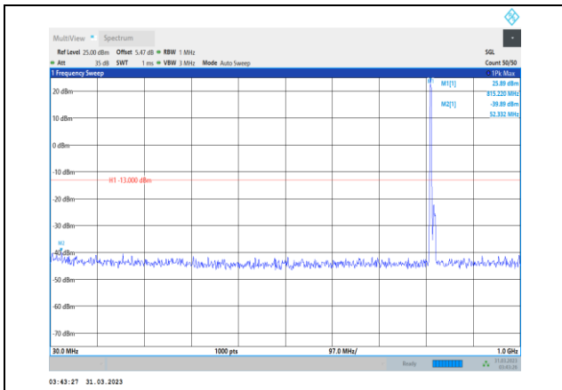
Band26-10MHz-QPSK-26740-1RB#0- Range1:30~1000MHz
