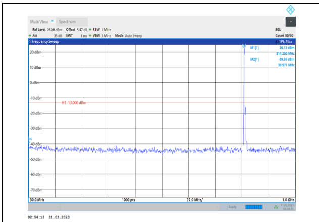
Band26-5MHz-QPSK-26715-1RB#0-Range1:30~1000MHz
