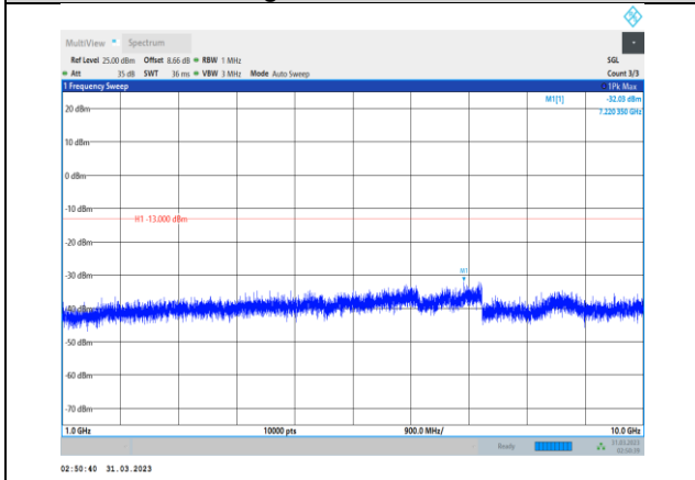
Band26-1.4MHz-64QAM-26697-1RB#0- Range2:1000~10000MHz
