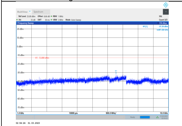
Band26-5MHz-QPSK-26715-1RB#0-Range2:1000~10000MHz
