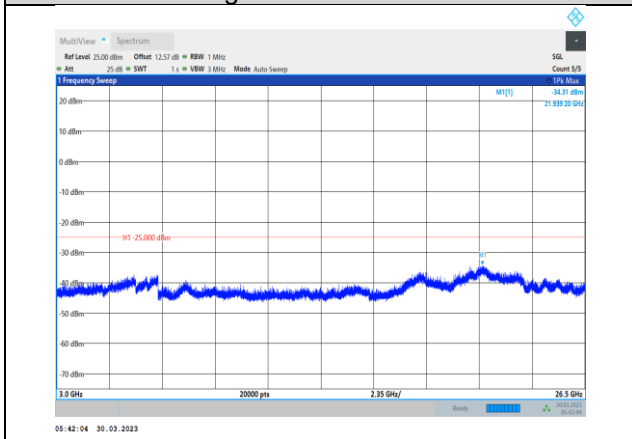
Band38-10MHz-QPSK-38000-1RB#0- Range3:3000~26500MHz
