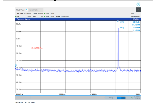
Band26-15MHz-16QAM-26865-1RB#0- Range1:30~1000MHz
