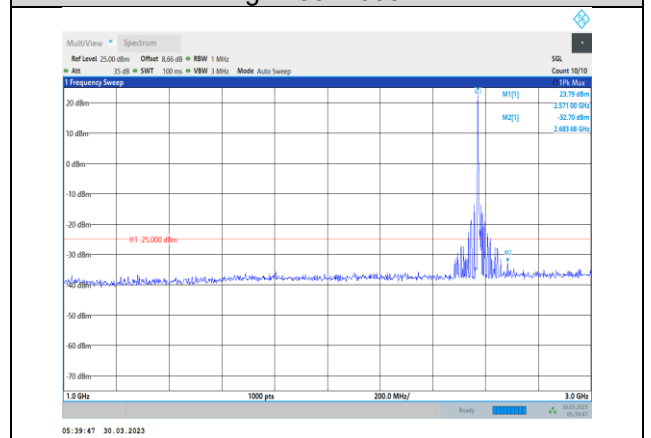
Band38-10MHz-QPSK-37800-1RB#0- Range2:1000~3000MHz
