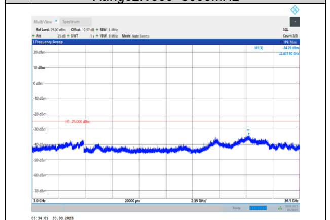
Band38-5MHz-16QAM-37775-1RB#0-Range3:3000~26500MHz
