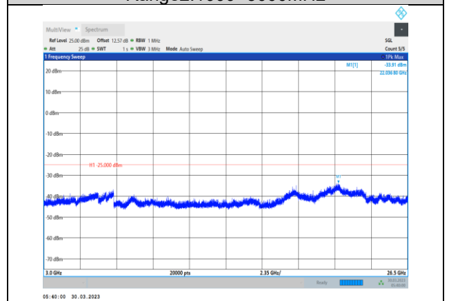
Band38-10MHz-QPSK-37800-1RB#0- Range3:3000~26500MHz
