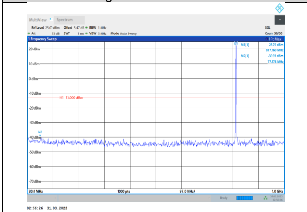
Band26-5MHz-64QAM-26740-1RB#0- Range1:30~1000MHz
