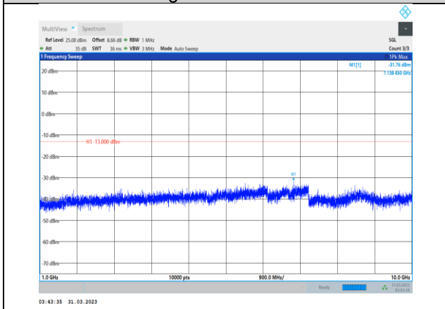
Band26-10MHz-QPSK-26740-1RB#0- Range2:1000~10000MHz
