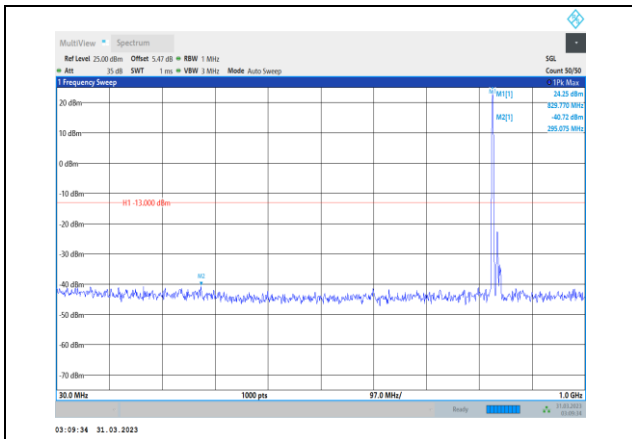
Band26-15MHz-16QAM-26915-1RB#0- Range1:30~1000MHz
