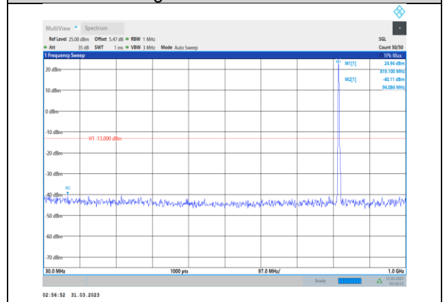
Band26-5MHz-QPSK-26765-1RB#0-Range1:30~1000MHz
