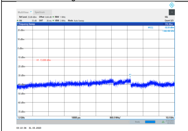
Band26-15MHz-QPSK-26965-1RB#0- Range2:1000~10000MHz
