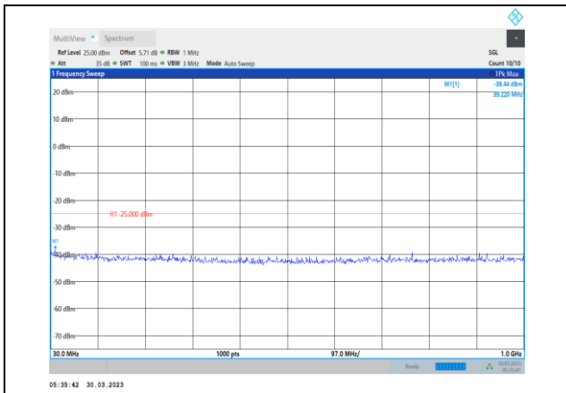
Band38-5MHz-16QAM-38000-1RB#0- Range1:30~1000MHz
