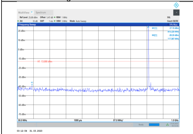
Band26-15MHz-16QAM-26765-1RB#0- Range1:30~1000MHz
