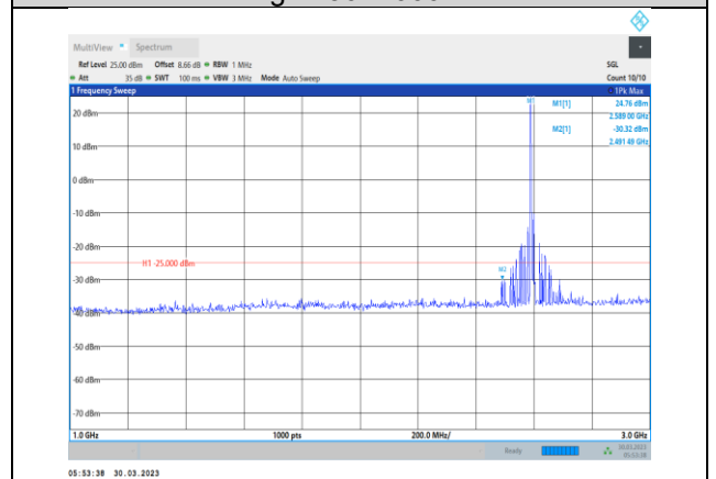
Band38-15MHz-QPSK-38000-1RB#0- Range2:1000~3000MHz
