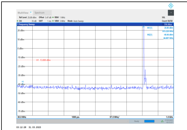
Band26-15MHz-QPSK-26765-1RB#0- Range1:30~1000MHz
