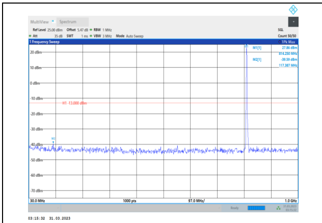
Band26-3MHz-16QAM-26705-1RB#0- Range1:30~1000MHz
