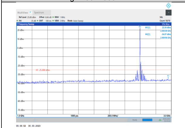
Band38-5MHz-16QAM-38000-1RB#0- Range2:1000~3000MHz
