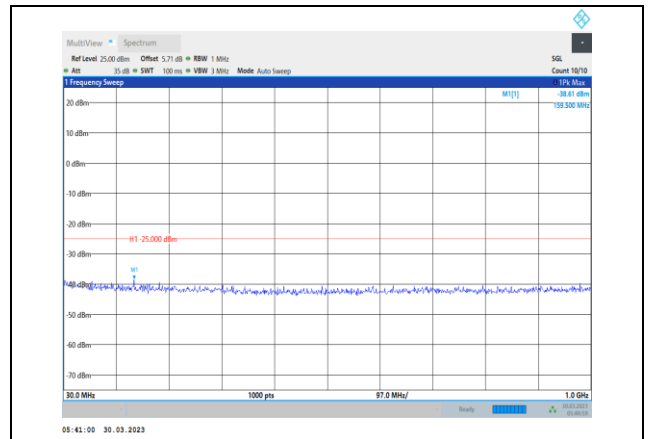
Band38-10MHz-64QAM-37800-1RB#0- Range1:30~1000MHz
