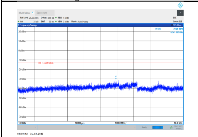
Band26-15MHz-16QAM-26915-1RB#0- Range2:1000~10000MHz
