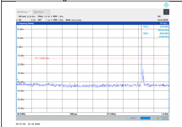
Band26-15MHz-QPSK-26865-1RB#0- Range1:30~1000MHz
