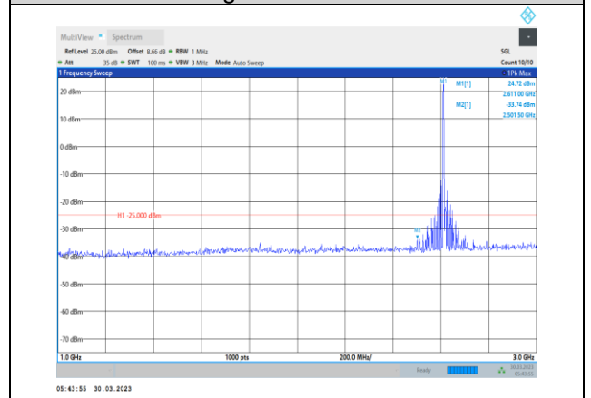
Band38-10MHz-QPSK-38200-1RB#0- Range2:1000~3000MHz
