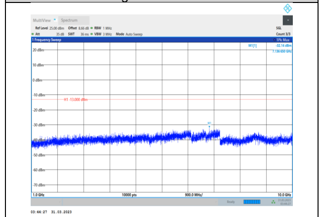
Band26-10MHz-64QAM-26740-1RB#0- Range2:1000~10000MHz
