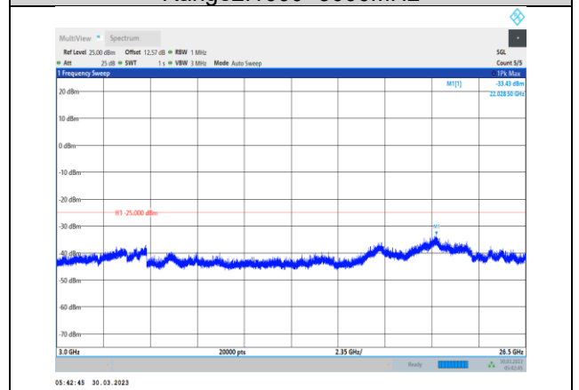
Band38-10MHz-16QAM-38000-1RB#0-Range3:3000~26500MHz
