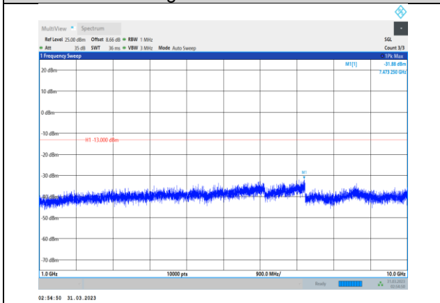
Band26-5MHz-16QAM-26715-1RB#0- Range2:1000~10000MHz
