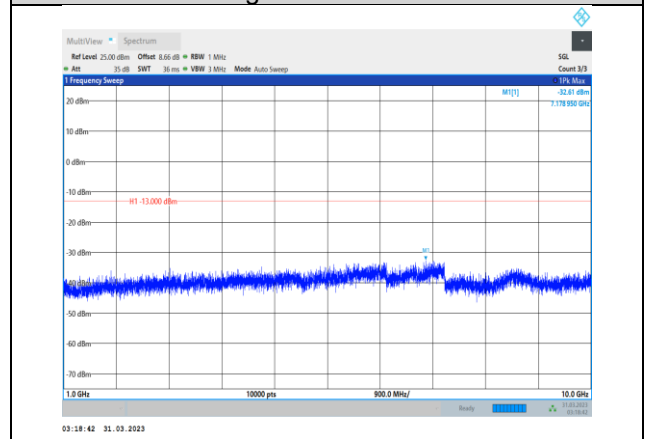
Band26-3MHz-64QAM-26775-1RB#0- Range2:1000~10000MHz
