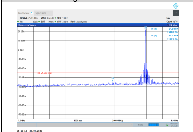
Band38-10MHz-64QAM-38000-1RB#0-Range2:1000~3000MHz
