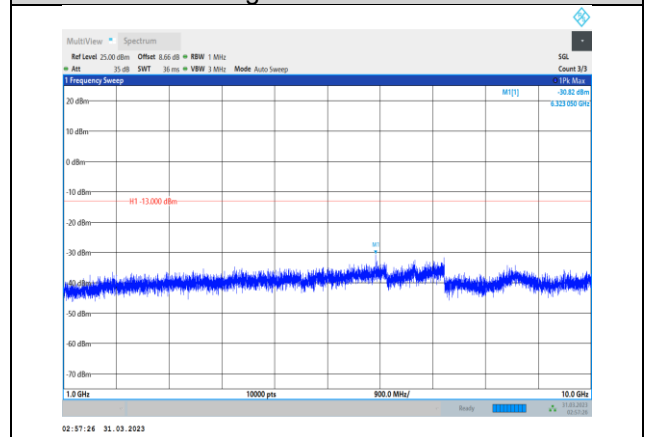
Band26-5MHz-16QAM-26765-1RB#0- Range2:1000~10000MHz
