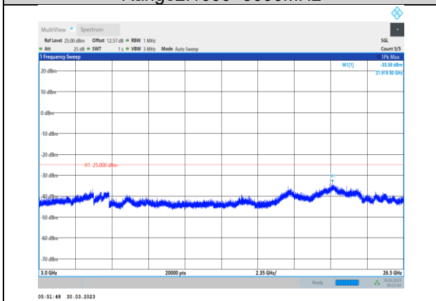
Band38-15MHz-QPSK-37825-1RB#0- Range3:3000~26500MHz
