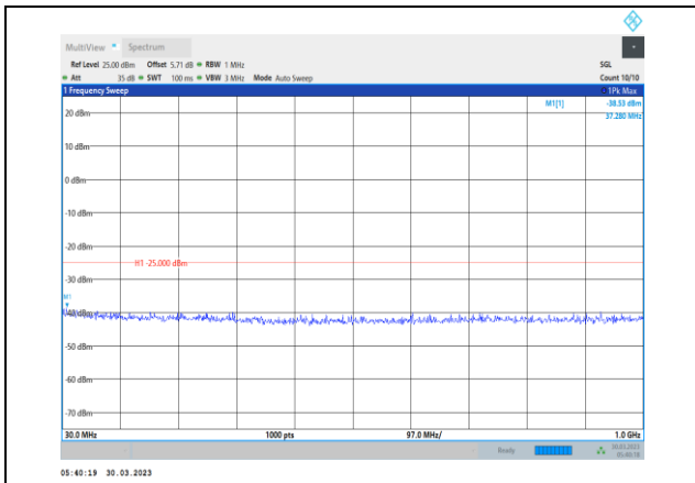
Band38-10MHz-16QAM-37800-1RB#0-Range1:30~1000MHz
