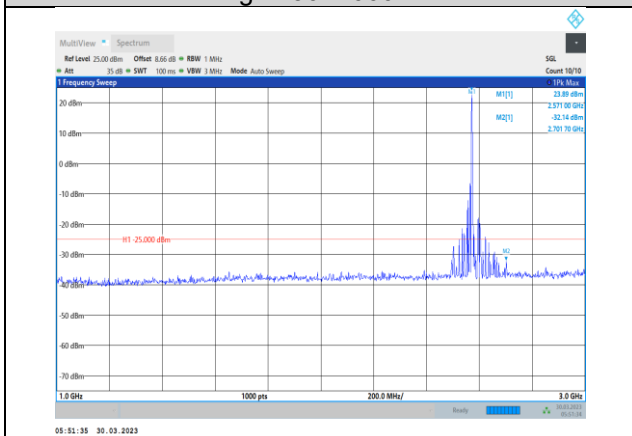
Band38-15MHz-QPSK-37825-1RB#0- Range2:1000~3000MHz
