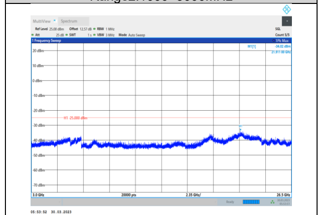
Band38-15MHz-QPSK-38000-1RB#0- Range3:3000~26500MHz
