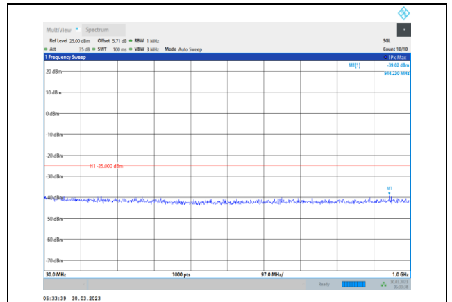
Band38-5MHz-16QAM-37775-1RB#0-Range1:30~1000MHz
