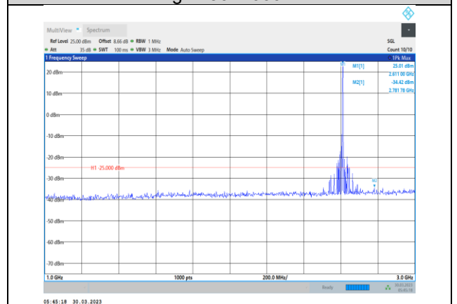
Band38-10MHz-64QAM-38200-1RB#0-Range2:1000~3000MHz
