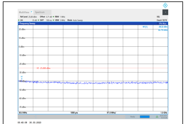
Band38-10MHz-64QAM-38200-1RB#0-Range1:30~1000MHz
