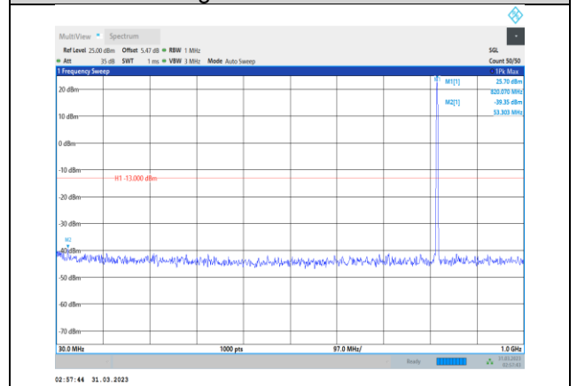
Band26-5MHz-64QAM-26765-1RB#0- Range1:30~1000MHz
