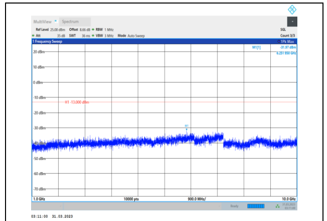
Band26-15MHz-16QAM-26965-1RB#0- Range2:1000~10000MHz
