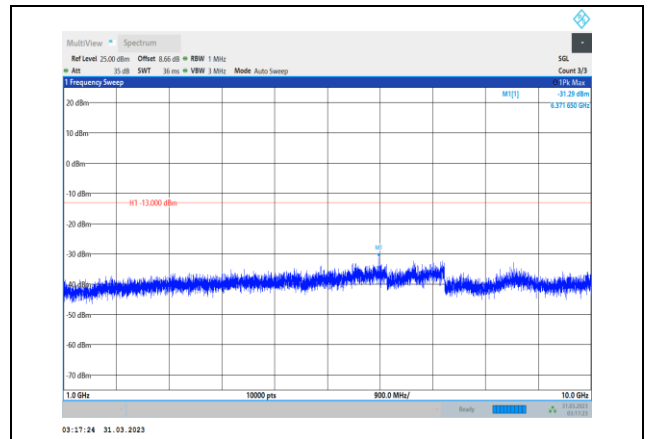
Band26-3MHz-64QAM-26740-1RB#0- Range2:1000~10000MHz
