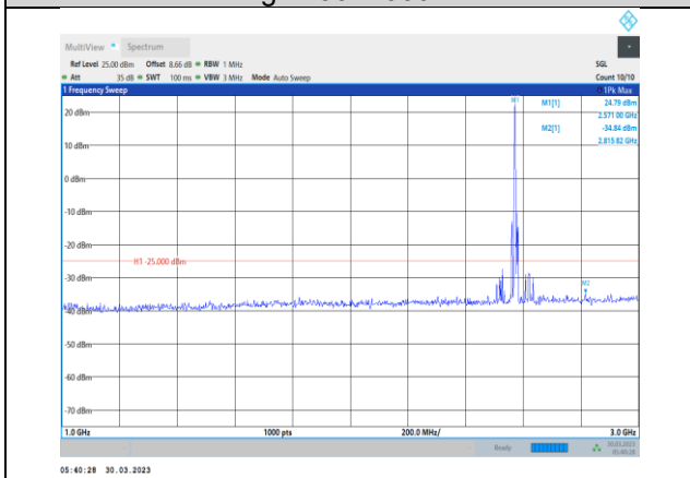
Band38-10MHz-16QAM-37800-1RB#0-Range2:1000~3000MHz
