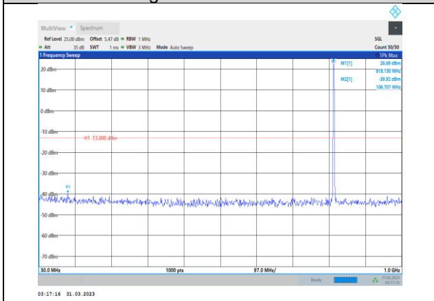
Band26-3MHz-64QAM-26740-1RB#0- Range1:30~1000MHz
