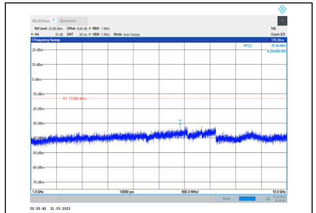
Band26-5MHz-QPSK-26740-1RB#0-Range2:1000~10000MHz
