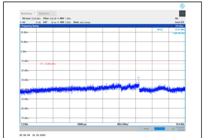
Band26-5MHz-64QAM-26740-1RB#0- Range2:1000~10000MHz
