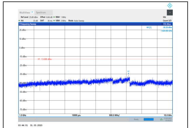
Band26-10MHz-16QAM-26740-1RB#0- Range2:1000~10000MHz
