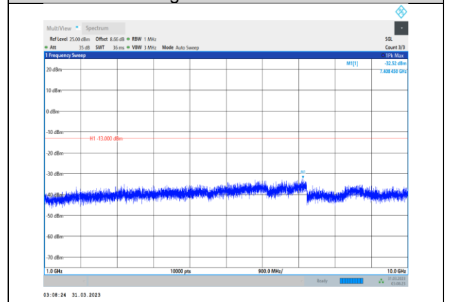
Band26-15MHz-16QAM-26865-1RB#0- Range2:1000~10000MHz
