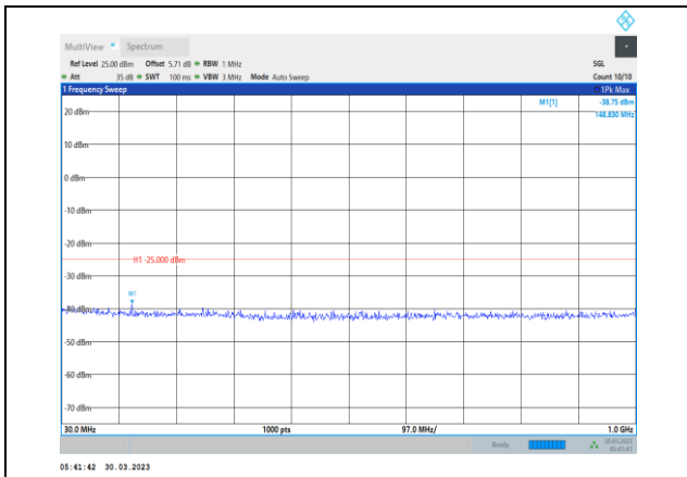
Band38-10MHz-QPSK-38000-1RB#0- Range1:30~1000MHz
