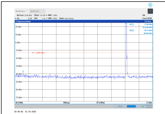
Band26-5MHz-16QAM-26715-1RB#0- Range1:30~1000MHz
