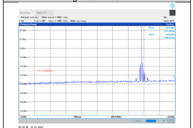
Band38-5MHz-16QAM-37775-1RB#0-Range2:1000~3000MHz
