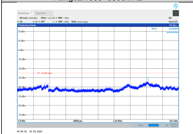
Band38-10MHz-16QAM-37800-1RB#0-Range3:3000~26500MHz
