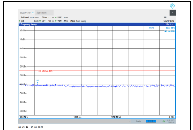
Band38-10MHz-QPSK-38200-1RB#0- Range1:30~1000MHz
