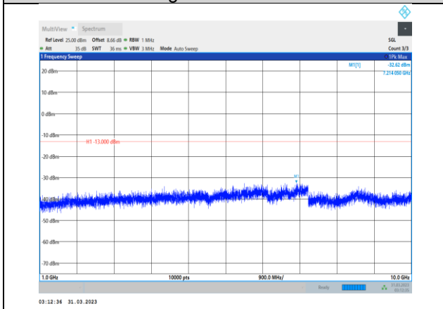
Band26-15MHz-QPSK-26765-1RB#0- Range2:1000~10000MHz
