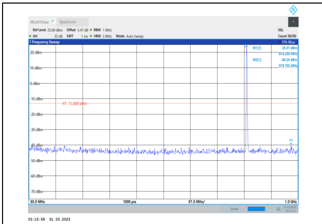
Band26-3MHz-64QAM-26705-1RB#0- Range1:30~1000MHz
