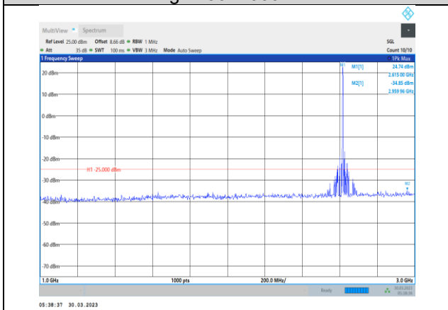
Band38-5MHz-64QAM-38225-1RB#0- Range2:1000~3000MHz
