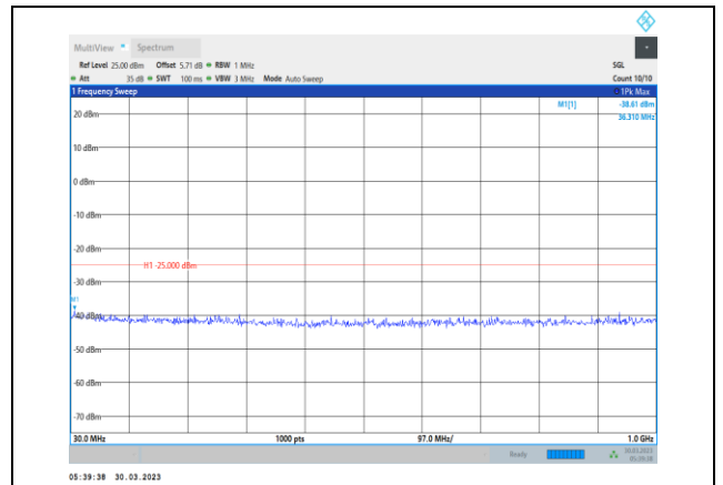
Band38-10MHz-QPSK-37800-1RB#0- Range1:30~1000MHz
