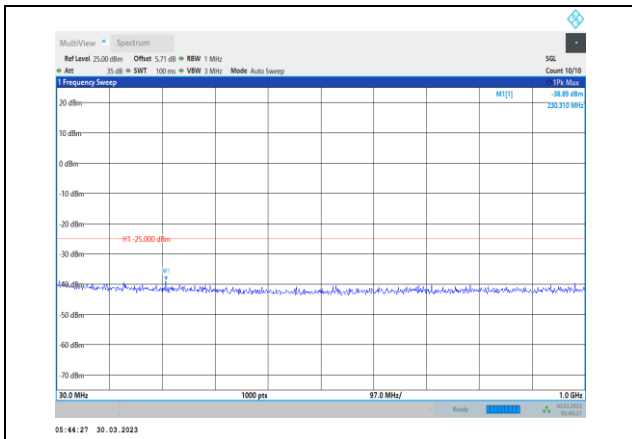
Band38-10MHz-16QAM-38200-1RB#0- Range1:30~1000MHz
