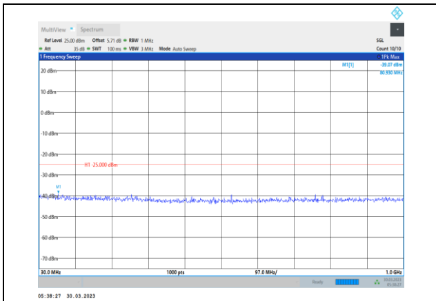
Band38-5MHz-64QAM-38225-1RB#0- Range1:30~1000MHz
