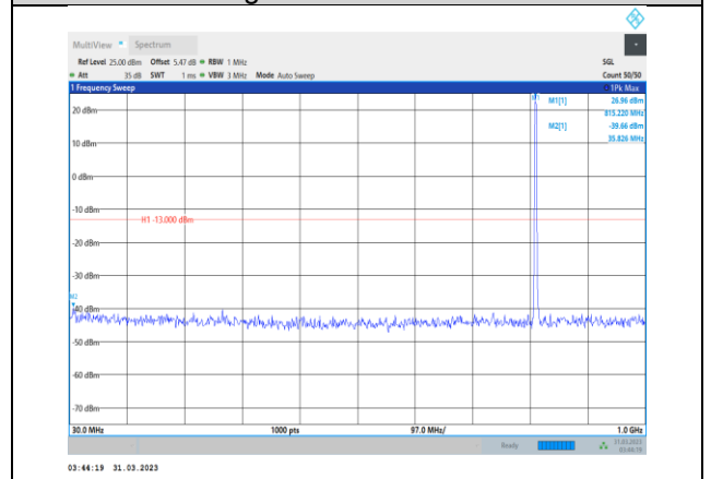
Band26-10MHz-64QAM-26740-1RB#0- Range1:30~1000MHz
