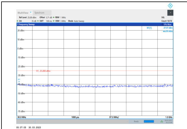
Band38-5MHz-QPSK-38225-1RB#0-Range1:30~1000MHz
