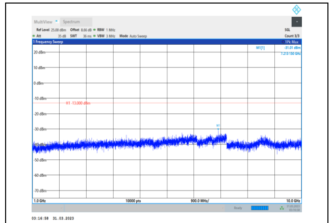
Band26-3MHz-16QAM-26740-1RB#0- Range2:1000~10000MHz
