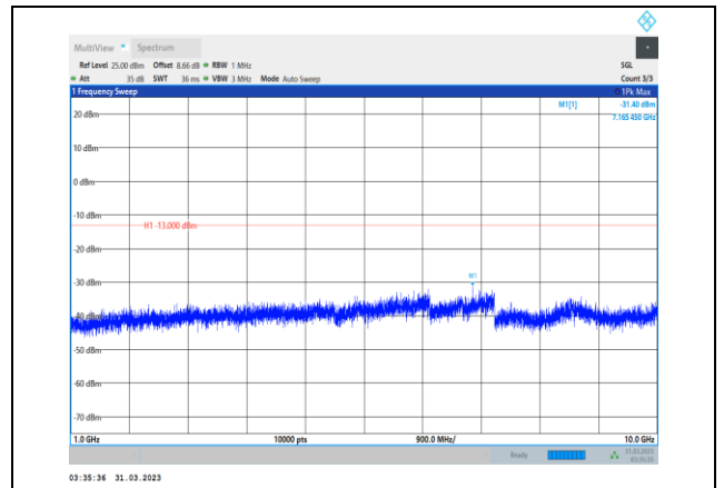
Band12-1.4MHz-QPSK-23095-1RB#0- Range2:1000~10000MHz
