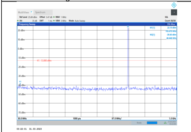
Band12-10MHz-64QAM-23095-1RB#0- Range1:30~1000MHz
