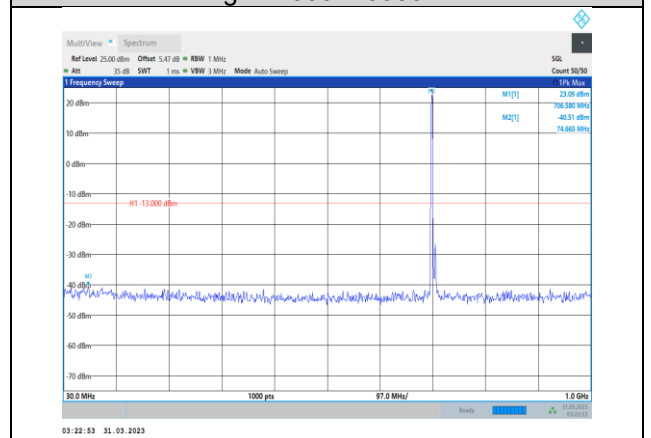
Band12-10MHz-16QAM-23130-1RB#0- Range1:30~1000MHz
