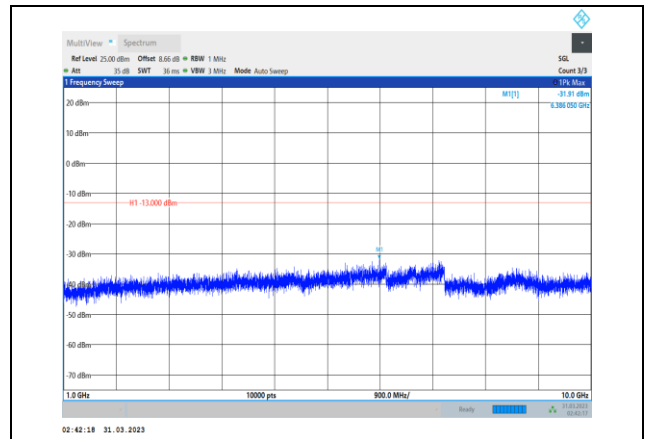
Band12-5MHz-16QAM-23095-1RB#0- Range2:1000~10000MHz
