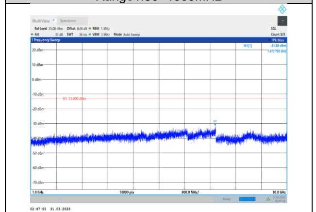
Band17-10MHz-QPSK-23800-1RB#0- Range2:1000~10000MHz
