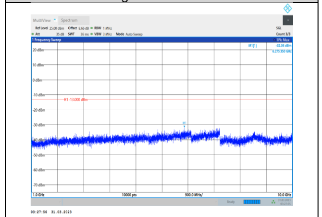
Band12-3MHz-64QAM-23165-1RB#0- Range2:1000~10000MHz
