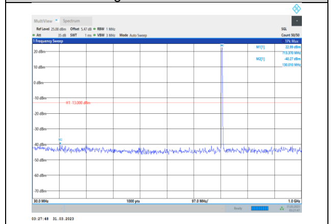
Band12-3MHz-64QAM-23165-1RB#0- Range1:30~1000MHz
