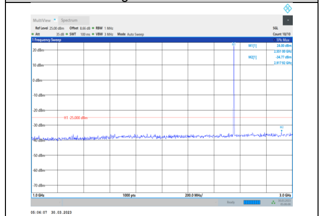
Band7-20MHz-64QAM-21350-1RB#0- Range2:1000~3000MHz
