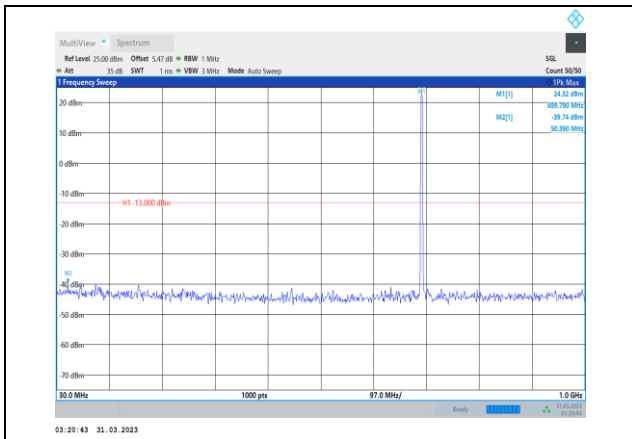
Band12-10MHz-64QAM-23060-1RB#0- Range1:30~1000MHz
