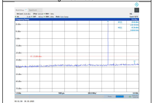
Band7-20MHz-64QAM-20850-1RB#0- Range2:1000~3000MHz
