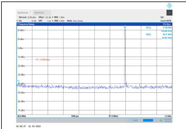
Band17-10MHz-16QAM-23780-1RB#0- Range1:30~1000MHz
