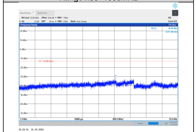
Band12-10MHz-16QAM-23130-1RB#0- Range2:1000~10000MHz
