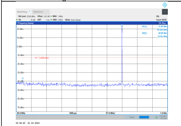
Band12-1.4MHz-64QAM-23095-1RB#0- Range1:30~1000MHz
