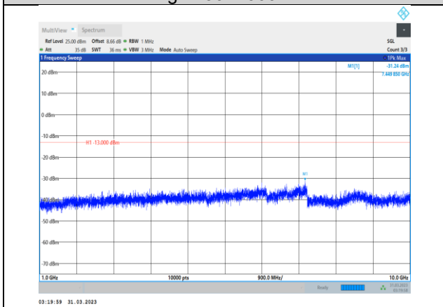
Band12-10MHz-QPSK-23060-1RB#0- Range2:1000~10000MHz
