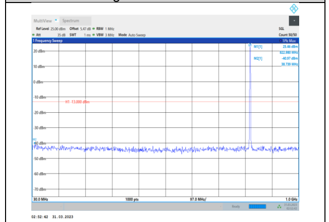
Band26-1.4MHz-16QAM-26783-1RB#0-Range1:30~1000MHz
