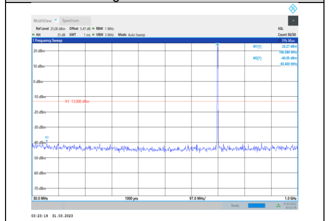
Band12-10MHz-64QAM-23130-1RB#0- Range1:30~1000MHz
