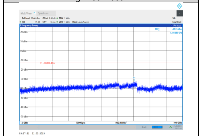
Band12-3MHz-16QAM-23165-1RB#0- Range2:1000~10000MHz
