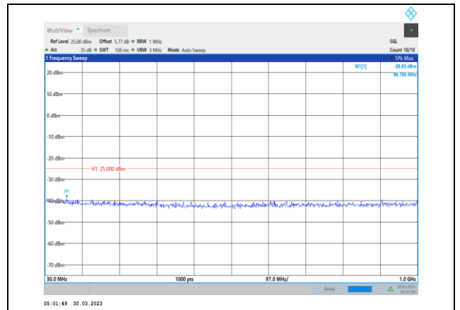
Band7-20MHz-64QAM-20850-1RB#0- Range1:30~1000MHz
