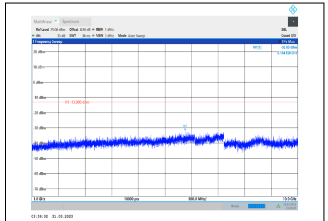
Band12-1.4MHz-16QAM-23095-1RB#0- Range2:1000~10000MHz
