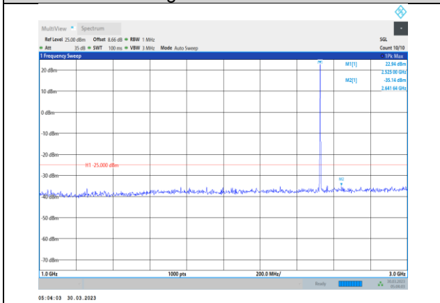
Band7-20MHz-64QAM-21100-1RB#0- Range2:1000~3000MHz
