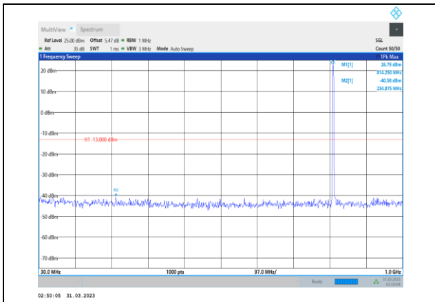
Band26-1.4MHz-16QAM-26697-1RB#0-Range1:30~1000MHz
