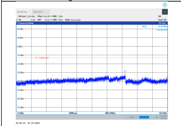
Band26-1.4MHz-16QAM-26697-1RB#0-Range2:1000~10000MHz
