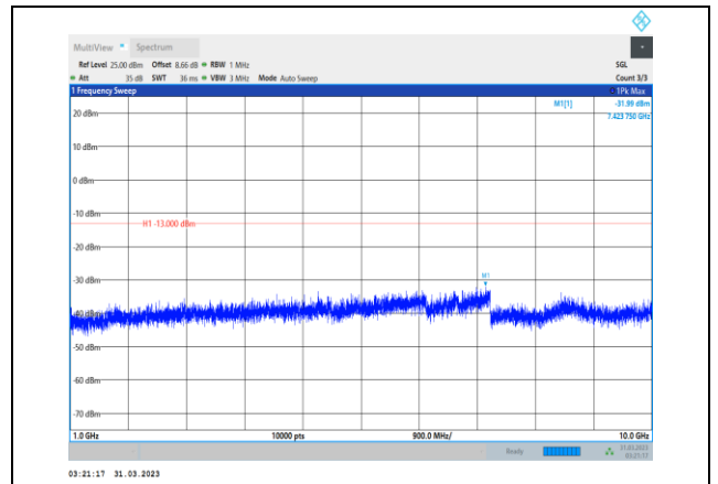
Band12-10MHz-QPSK-23095-1RB#0- Range2:1000~10000MHz
