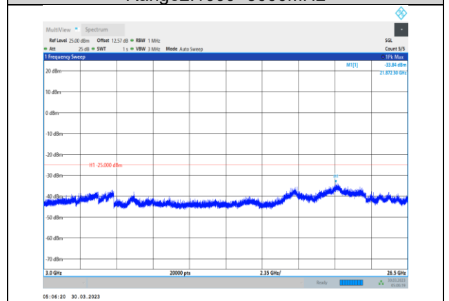
Band7-20MHz-64QAM-21350-1RB#0- Range3:3000~26500MHz
