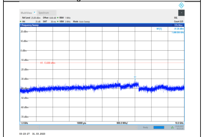
Band12-10MHz-64QAM-23130-1RB#0- Range2:1000~10000MHz
