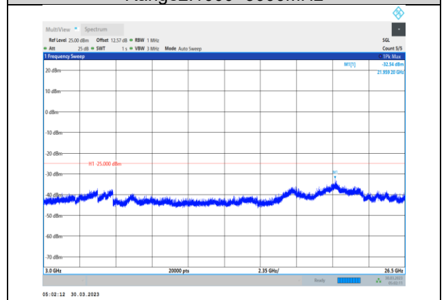
Band7-20MHz-64QAM-20850-1RB#0- Range3:3000~26500MHz
