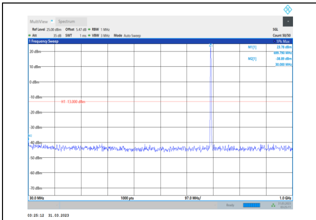
Band12-3MHz-64QAM-23025-1RB#0- Range1:30~1000MHz
