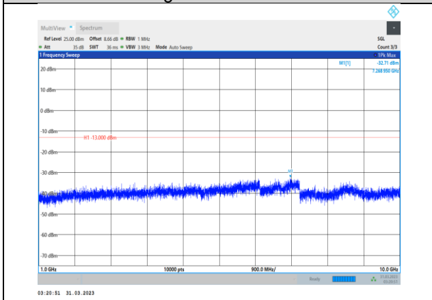
Band12-10MHz-64QAM-23060-1RB#0- Range2:1000~10000MHz
