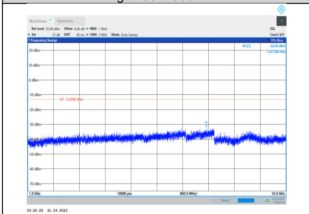
Band12-10MHz-16QAM-23060-1RB#0- Range2:1000~10000MHz
