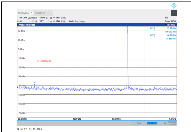
Band12-5MHz-64QAM-23035-1RB#0- Range1:30~1000MHz
