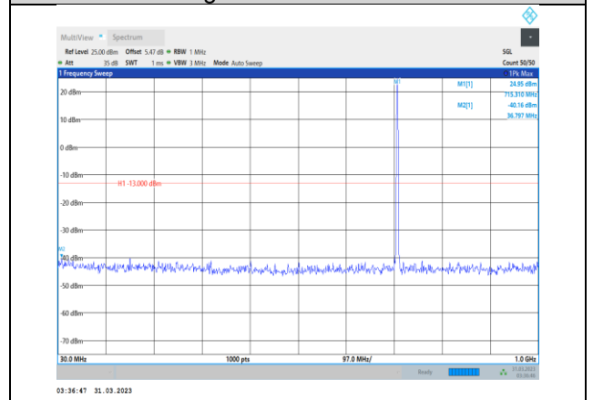
Band12-1.4MHz-QPSK-23173-1RB#0- Range1:30~1000MHz
