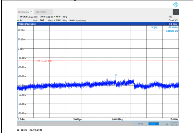
Band12-5MHz-64QAM-23035-1RB#0- Range2:1000~10000MHz
