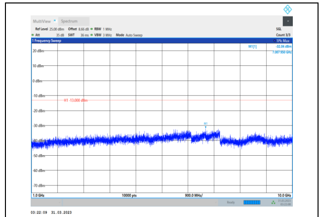
Band12-10MHz-64QAM-23095-1RB#0- Range2:1000~10000MHz
