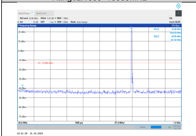
Band12-10MHz-QPSK-23095-1RB#0- Range1:30~1000MHz
