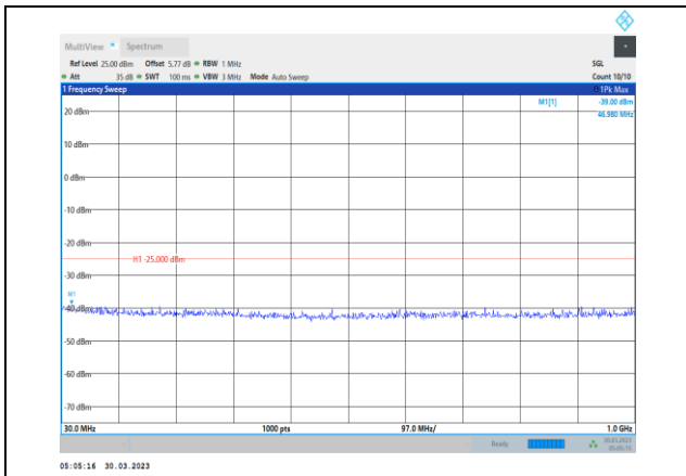
Band7-20MHz-16QAM-21350-1RB#0- Range1:30~1000MHz
