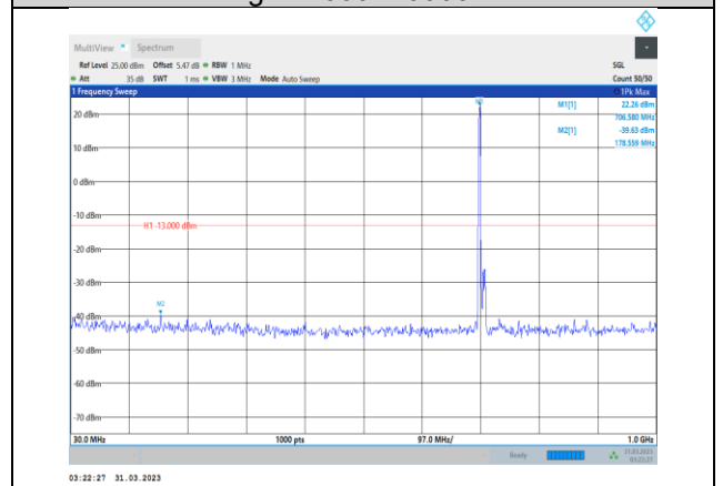
Band12-10MHz-QPSK-23130-1RB#0- Range1:30~1000MHz
