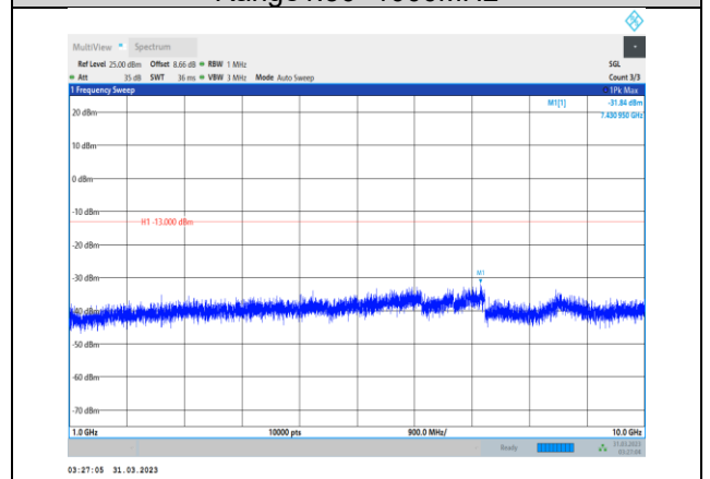
Band12-3MHz-QPSK-23165-1RB#0- Range2:1000~10000MHz
