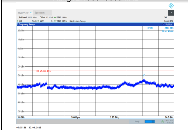
Band7-20MHz-16QAM-21350-1RB#0- Range3:3000~26500MHz
