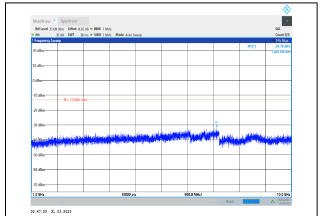
Band17-10MHz-16QAM-23790-1RB#0- Range2:1000~10000MHz
