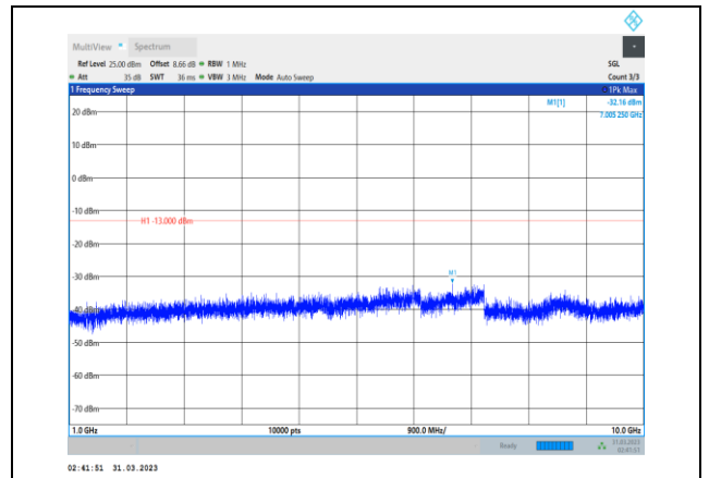
Band12-5MHz-QPSK-23095-1RB#0- Range2:1000~10000MHz
