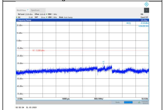
Band26-1.4MHz-QPSK-26783-1RB#0- Range2:1000~10000MHz
