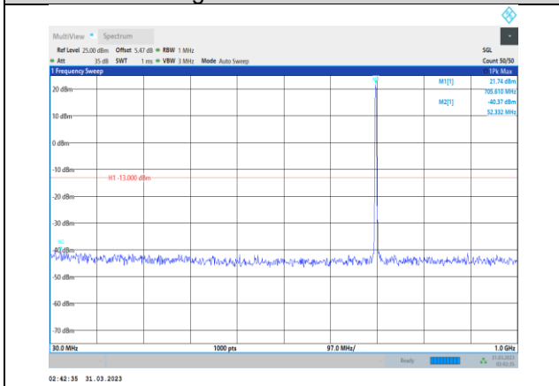
Band12-5MHz-64QAM-23095-1RB#0- Range1:30~1000MHz
