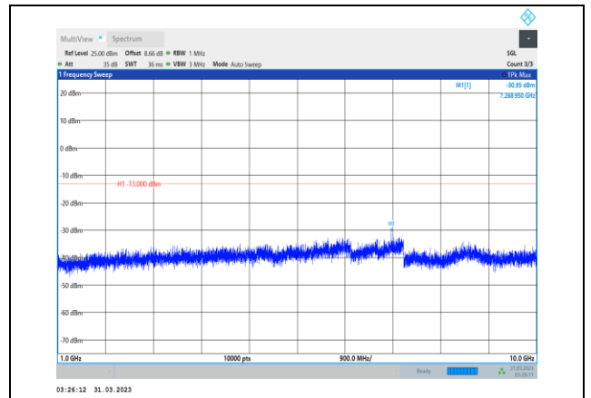
Band12-3MHz-16QAM-23095-1RB#0- Range2:1000~10000MHz
