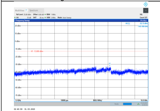
Band12-5MHz-16QAM-23035-1RB#0- Range2:1000~10000MHz
