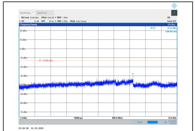
Band12-3MHz-64QAM-23095-1RB#0- Range2:1000~10000MHz
