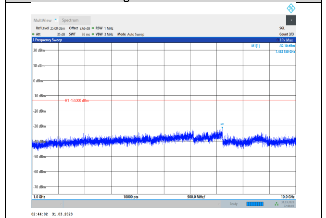
Band12-5MHz-64QAM-23155-1RB#0- Range2:1000~10000MHz
