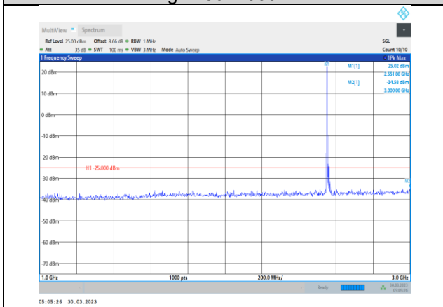
Band7-20MHz-16QAM-21350-1RB#0- Range2:1000~3000MHz
