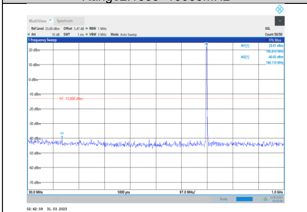
Band12-5MHz-16QAM-23095-1RB#0- Range1:30~1000MHz
