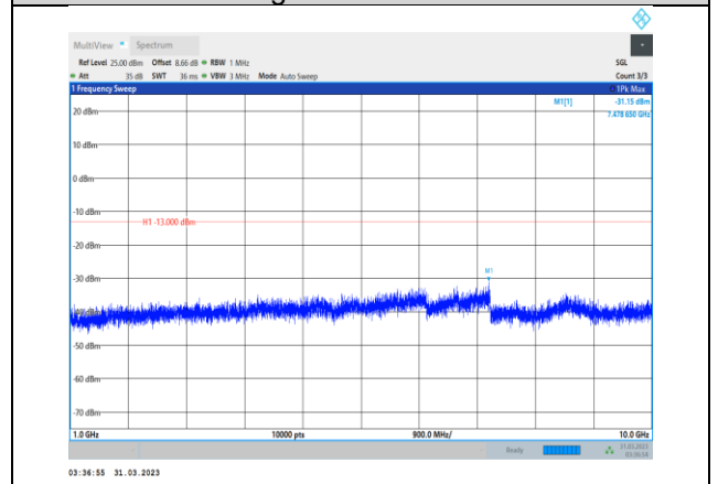
Band12-1.4MHz-QPSK-23173-1RB#0- Range2:1000~10000MHz
