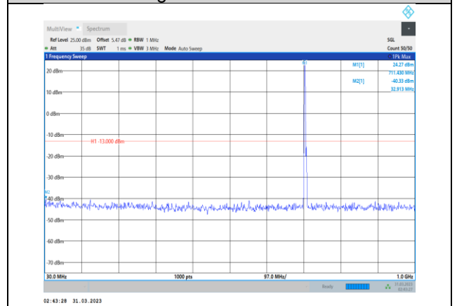
Band12-5MHz-16QAM-23155-1RB#0- Range1:30~1000MHz
