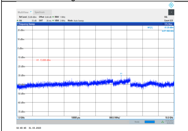
Band17-10MHz-16QAM-23780-1RB#0- Range2:1000~10000MHz
