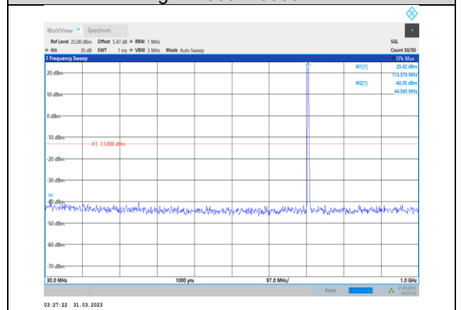
Band12-3MHz-16QAM-23165-1RB#0- Range1:30~1000MHz
