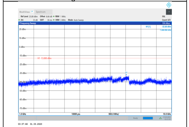
Band12-1.4MHz-64QAM-23173-1RB#0- Range2:1000~10000MHz
