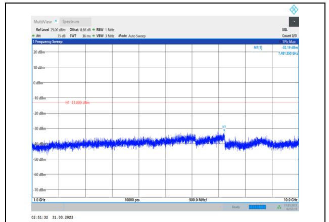
Band26-1.4MHz-16QAM-26740-1RB#0-Range2:1000~10000MHz
