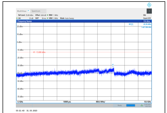
Band12-10MHz-16QAM-23095-1RB#0- Range2:1000~10000MHz
