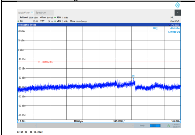
Band12-3MHz-64QAM-23025-1RB#0- Range2:1000~10000MHz
