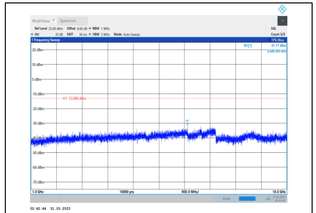
Band12-5MHz-64QAM-23095-1RB#0- Range2:1000~10000MHz
