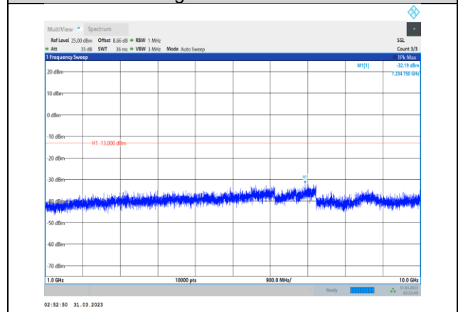
Band26-1.4MHz-16QAM-26783-1RB#0-Range2:1000~10000MHz
