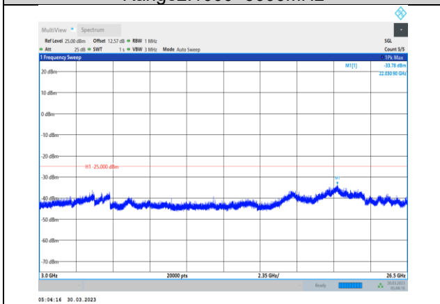
Band7-20MHz-64QAM-21100-1RB#0- Range3:3000~26500MHz
