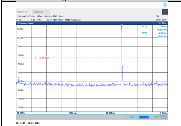
Band12-5MHz-QPSK-23095-1RB#0- Range1:30~1000MHz
