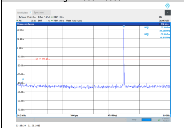
Band12-3MHz-QPSK-23095-1RB#0- Range1:30~1000MHz
