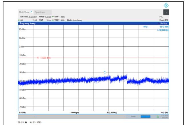
Band12-3MHz-QPSK-23095-1RB#0- Range2:1000~10000MHz
