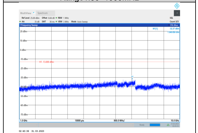
Band12-5MHz-16QAM-23155-1RB#0- Range2:1000~10000MHz
