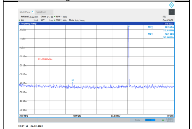
Band12-1.4MHz-16QAM-23173-1RB#0- Range1:30~1000MHz
