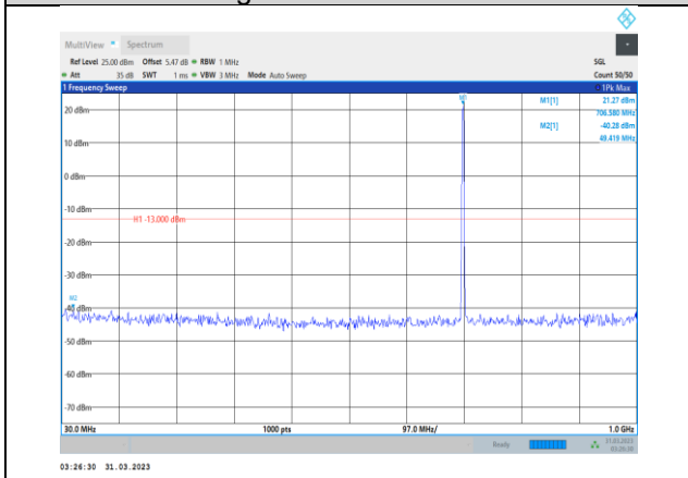
Band12-3MHz-64QAM-23095-1RB#0- Range1:30~1000MHz
