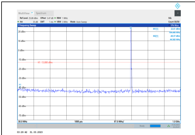
Band17-5MHz-QPSK-23755-1RB#0- Range1:30~1000MHz
