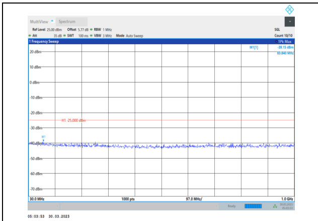
Band7-20MHz-64QAM-21100-1RB#0- Range1:30~1000MHz
