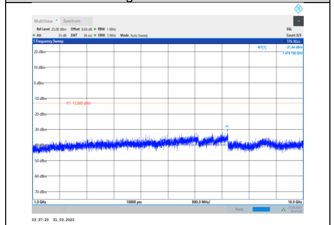
Band12-1.4MHz-16QAM-23173-1RB#0- Range2:1000~10000MHz
