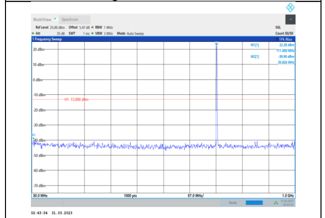
Band12-5MHz-64QAM-23155-1RB#0- Range1:30~1000MHz
