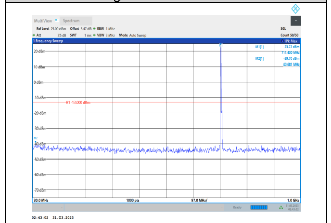
Band12-5MHz-QPSK-23155-1RB#0- Range1:30~1000MHz
