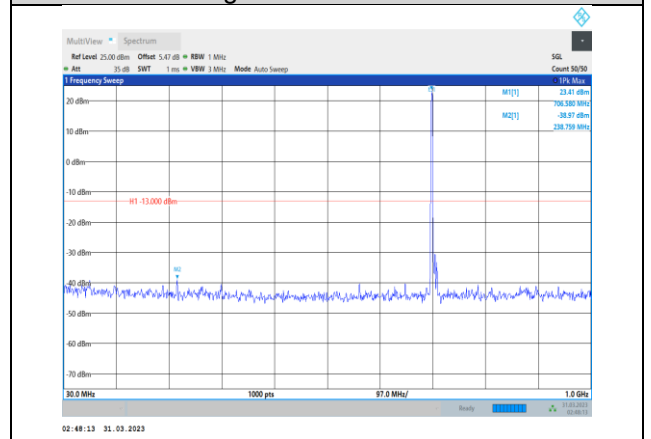
Band17-10MHz-16QAM-23800-1RB#0- Range1:30~1000MHz
