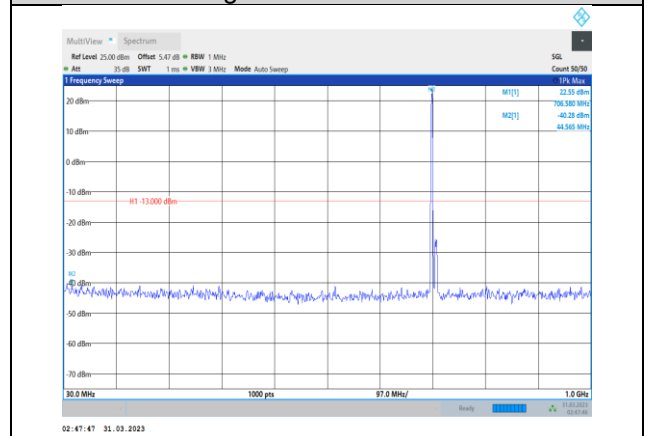
Band17-10MHz-QPSK-23800-1RB#0- Range1:30~1000MHz
