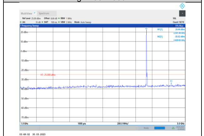
Band7-10MHz-16QAM-21100-1RB#0- Range2:1000~3000MHz
