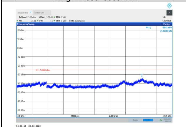
Band7-15MHz-64QAM-21375-1RB#0- Range3:3000~26500MHz
