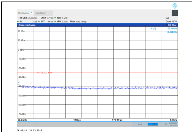
Band7-15MHz-64QAM-21375-1RB#0- Range1:30~1000MHz
