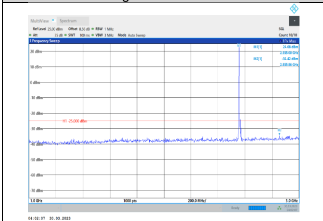
Band7-15MHz-QPSK-21375-1RB#0- Range2:1000~3000MHz
