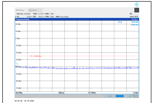
Band7-15MHz-16QAM-21375-1RB#0- Range1:30~1000MHz
