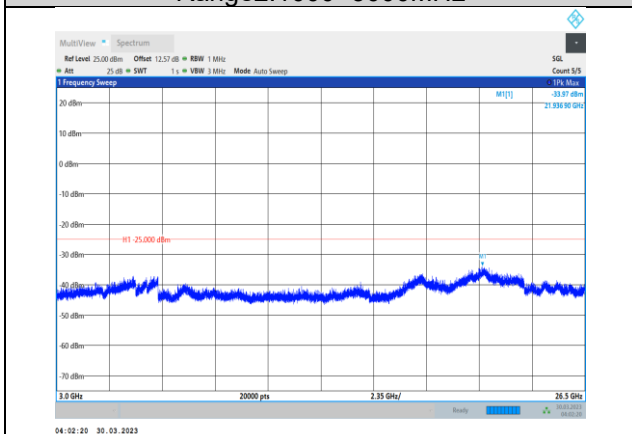
Band7-15MHz-QPSK-21375-1RB#0- Range3:3000~26500MHz
