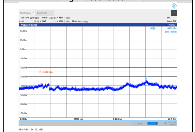
Band7-10MHz-64QAM-20800-1RB#0- Range3:3000~26500MHz
