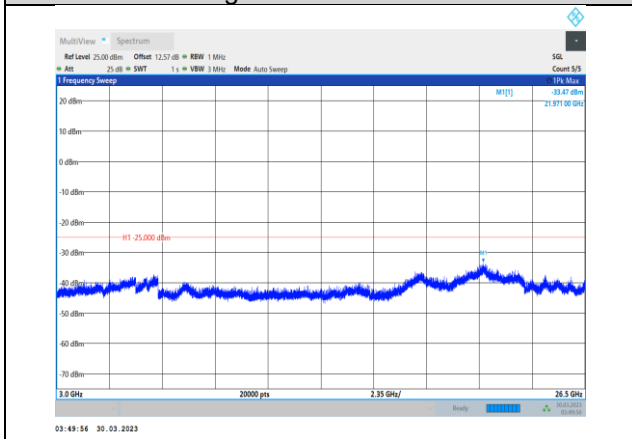
Band7-10MHz-64QAM-21100-1RB#0- Range3:3000~26500MHz
