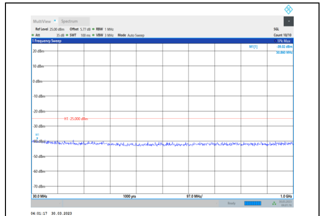
Band7-15MHz-64QAM-21100-1RB#0- Range1:30~1000MHz
