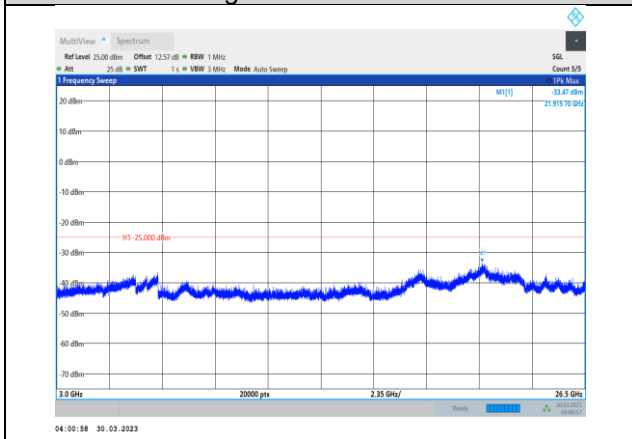
Band7-15MHz-16QAM-21100-1RB#0- Range3:3000~26500MHz
