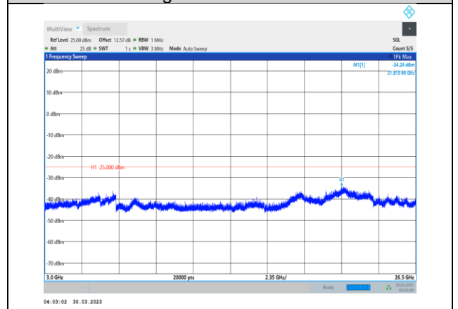
Band7-15MHz-16QAM-21375-1RB#0- Range3:3000~26500MHz
