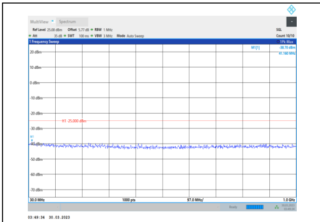
Band7-10MHz-64QAM-21100-1RB#0- Range1:30~1000MHz
