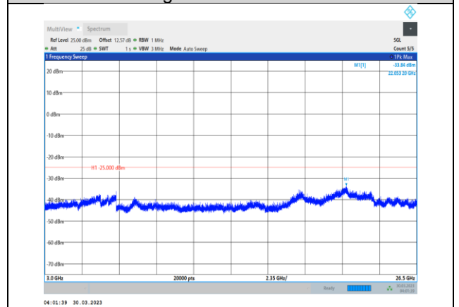
Band7-15MHz-64QAM-21100-1RB#0- Range3:3000~26500MHz
