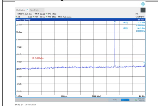
Band7-15MHz-64QAM-21100-1RB#0- Range2:1000~3000MHz
