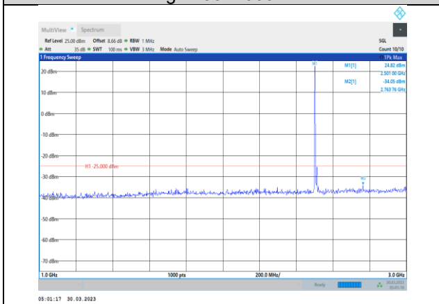
Band7-20MHz-16QAM-20850-1RB#0- Range2:1000~3000MHz
