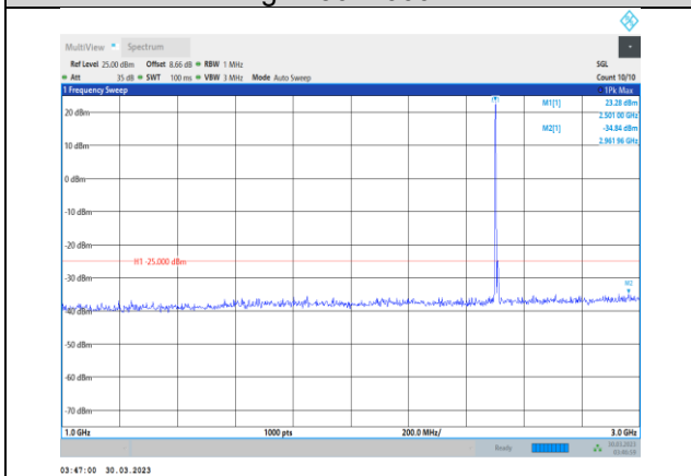
Band7-10MHz-16QAM-20800-1RB#0- Range2:1000~3000MHz
