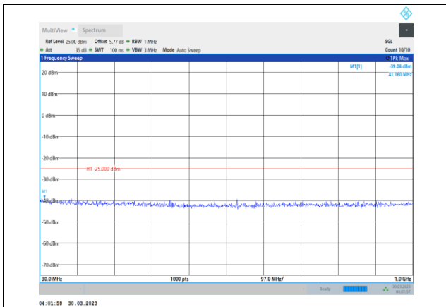
Band7-15MHz-QPSK-21375-1RB#0- Range1:30~1000MHz
