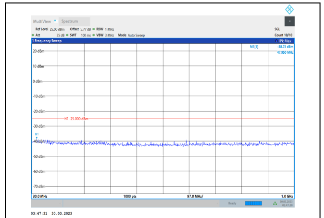
Band7-10MHz-64QAM-20800-1RB#0- Range1:30~1000MHz
