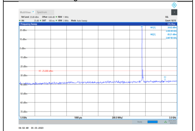
Band7-15MHz-16QAM-21375-1RB#0- Range2:1000~3000MHz
