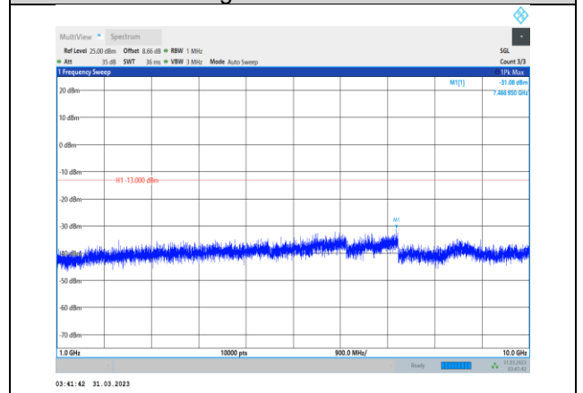
Band5-5MHz-QPSK-20625-1RB#0- Range2:1000~10000MHz
