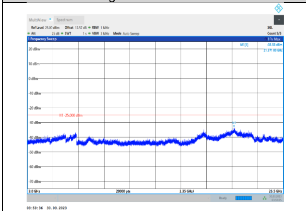
Band7-15MHz-64QAM-20825-1RB#0- Range3:3000~26500MHz
