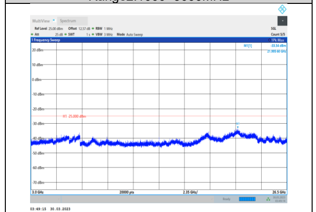
Band7-10MHz-16QAM-21100-1RB#0- Range3:3000~26500MHz
