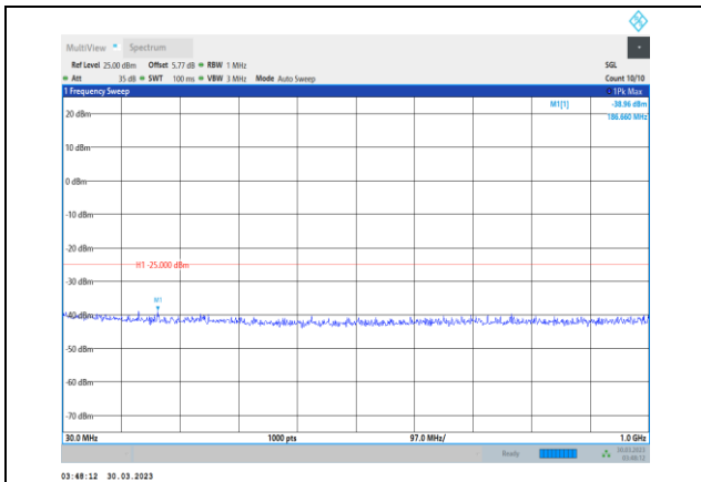
Band7-10MHz-QPSK-21100-1RB#0- Range1:30~1000MHz
