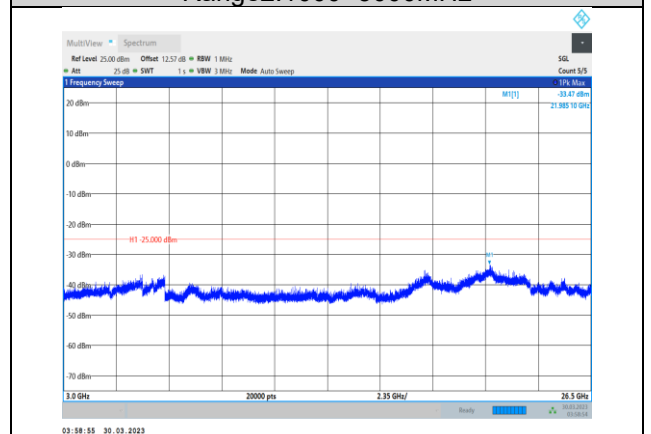
Band7-15MHz-16QAM-20825-1RB#0- Range3:3000~26500MHz
