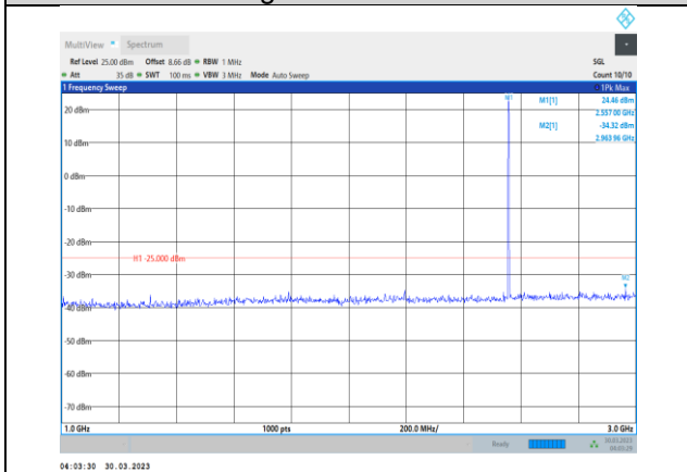
Band7-15MHz-64QAM-21375-1RB#0- Range2:1000~3000MHz
