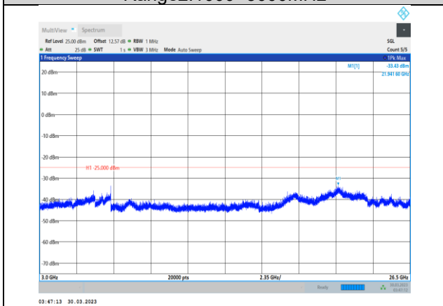
Band7-10MHz-16QAM-20800-1RB#0- Range3:3000~26500MHz
