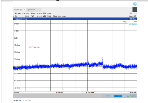
Band5-3MHz-64QAM-20415-1RB#0- Range2:1000~10000MHz
