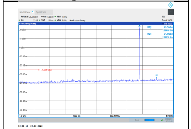
Band7-10MHz-64QAM-21400-1RB#0- Range2:1000~3000MHz
