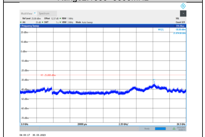
Band7-15MHz-QPSK-21100-1RB#0- Range3:3000~26500MHz
