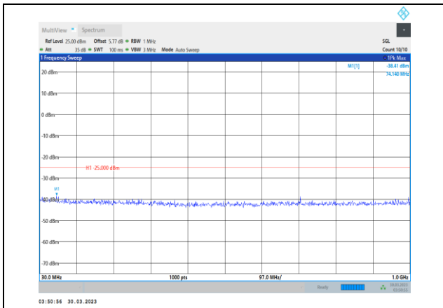
Band7-10MHz-16QAM-21400-1RB#0- Range1:30~1000MHz
