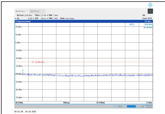
Band7-20MHz-16QAM-20850-1RB#0- Range1:30~1000MHz
