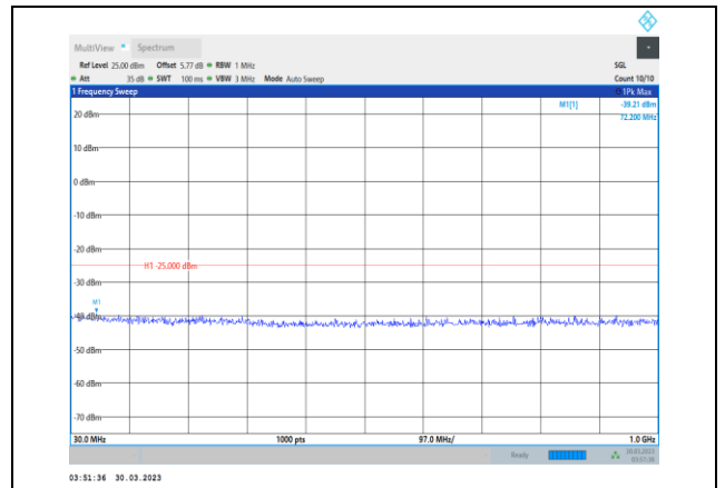
Band7-10MHz-64QAM-21400-1RB#0- Range1:30~1000MHz
