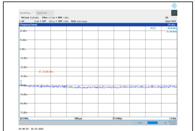
Band7-10MHz-16QAM-21100-1RB#0- Range1:30~1000MHz
