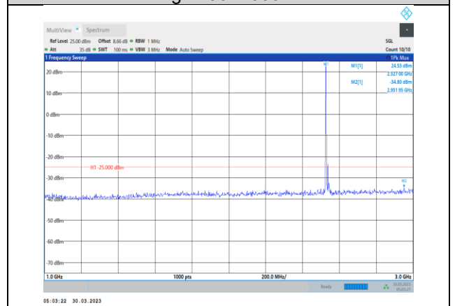
Band7-20MHz-16QAM-21100-1RB#0- Range2:1000~3000MHz
