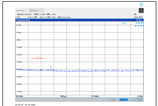
Band7-10MHz-QPSK-21400-1RB#0- Range1:30~1000MHz
