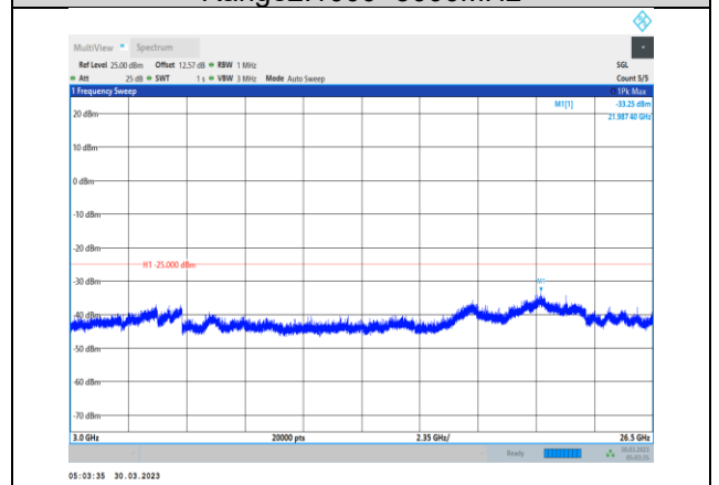
Band7-20MHz-16QAM-21100-1RB#0- Range3:3000~26500MHz
