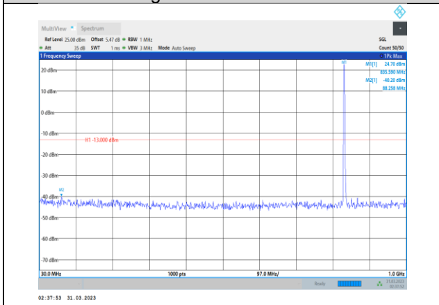
Band5-3MHz-64QAM-20525-1RB#0- Range1:30~1000MHz
