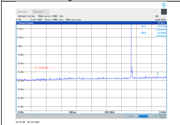
Band7-15MHz-16QAM-21100-1RB#0- Range2:1000~3000MHz
