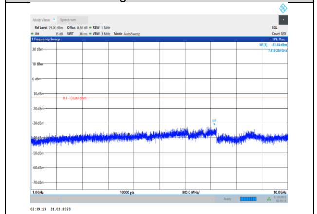
Band5-3MHz-64QAM-20635-1RB#0- Range2:1000~10000MHz
