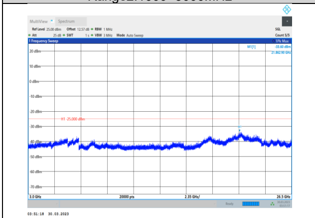
Band7-10MHz-16QAM-21400-1RB#0- Range3:3000~26500MHz
