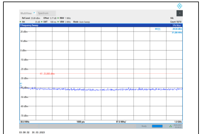
Band7-15MHz-16QAM-20825-1RB#0- Range1:30~1000MHz
