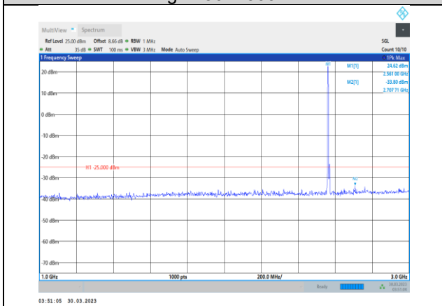
Band7-10MHz-16QAM-21400-1RB#0- Range2:1000~3000MHz
