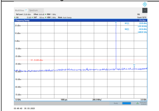
Band7-10MHz-64QAM-21100-1RB#0- Range2:1000~3000MHz
