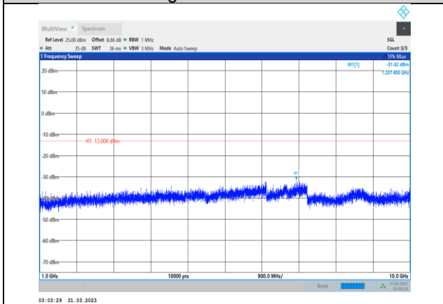
Band5-10MHz-QPSK-20450-1RB#0- Range2:1000~10000MHz
