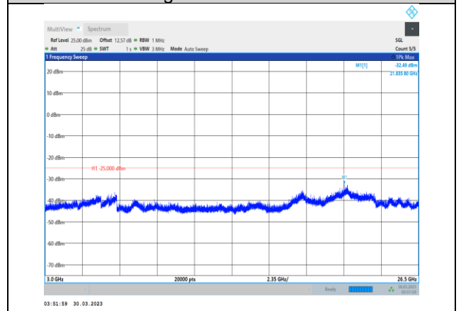
Band7-10MHz-64QAM-21400-1RB#0- Range3:3000~26500MHz
