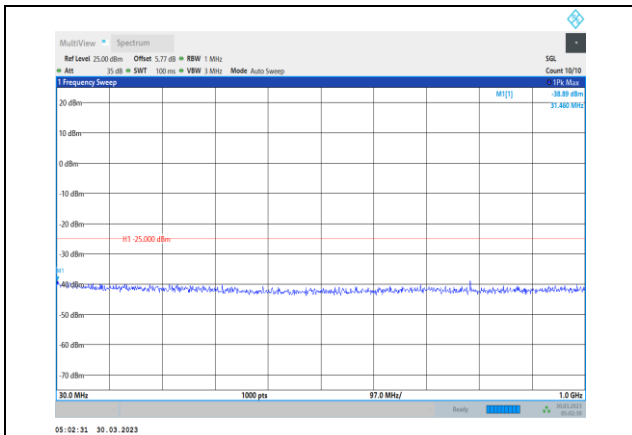
Band7-20MHz-QPSK-21100-1RB#0- Range1:30~1000MHz
