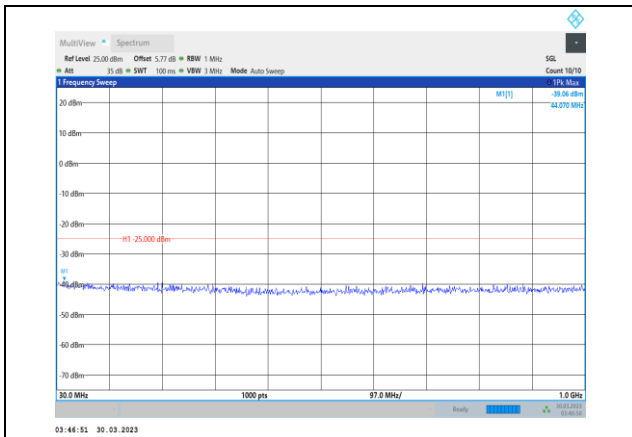
Band7-10MHz-16QAM-20800-1RB#0- Range1:30~1000MHz
