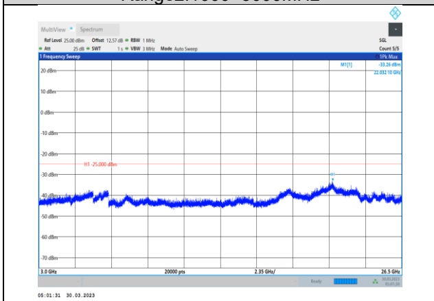
Band7-20MHz-16QAM-20850-1RB#0- Range3:3000~26500MHz
