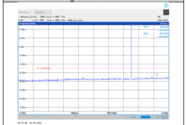
Band7-10MHz-64QAM-20800-1RB#0- Range2:1000~3000MHz
