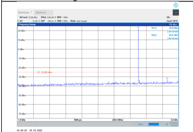
Band7-15MHz-64QAM-20825-1RB#0- Range2:1000~3000MHz
