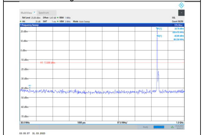
Band5-10MHz-QPSK-20600-1RB#0- Range1:30~1000MHz
