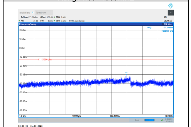
Band5-10MHz-QPSK-20600-1RB#0- Range2:1000~10000MHz
