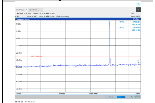
Band7-15MHz-16QAM-20825-1RB#0- Range2:1000~3000MHz
