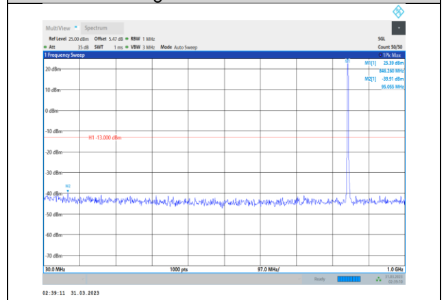
Band5-3MHz-64QAM-20635-1RB#0- Range1:30~1000MHz
