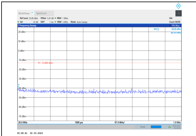
Band4-20MHz-16QAM-20050-1RB#0- Range1:30~1000MHz
