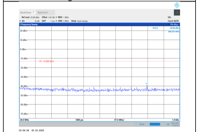
Band4-3MHz-64QAM-20385-1RB#0- Range1:30~1000MHz
