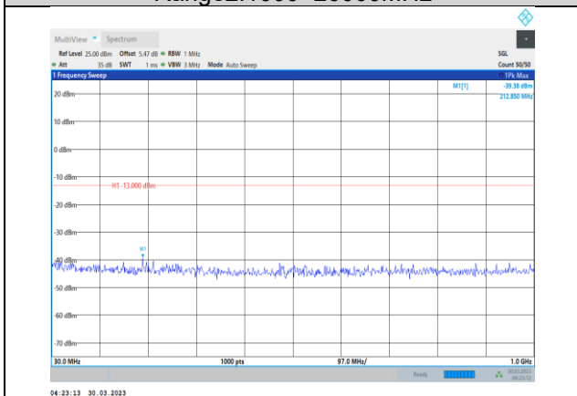
Band4-5MHz-64QAM-20175-1RB#0- Range1:30~1000MHz
