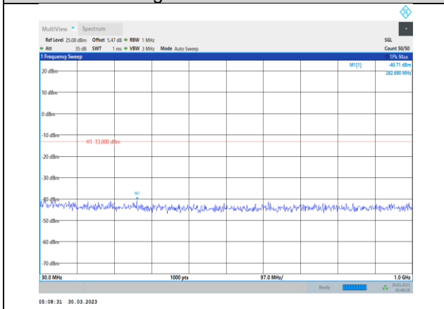
Band4-1.4MHz-QPSK-20175-1RB#0- Range1:30~1000MHz
