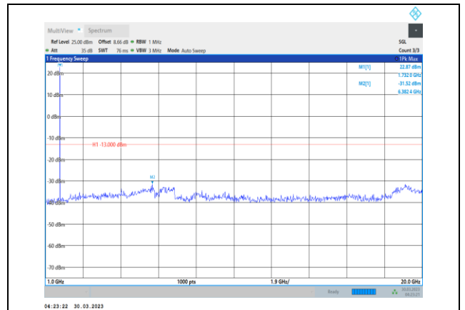
Band4-5MHz-64QAM-20175-1RB#0- Range2:1000~20000MHz
