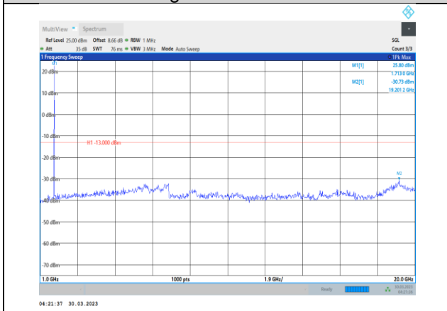
Band4-5MHz-16QAM-19975-1RB#0-Range2:1000~20000MHz
