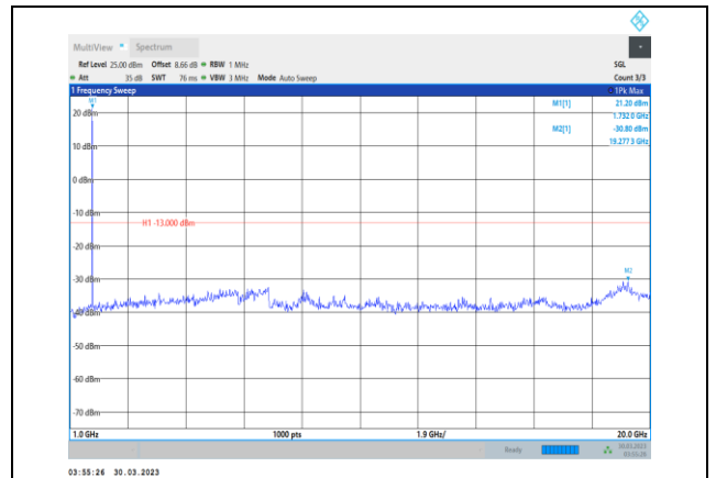
Band4-3MHz-64QAM-20175-1RB#0- Range2:1000~20000MHz
