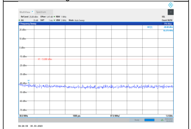
Band4-5MHz-16QAM-20375-1RB#0-Range1:30~1000MHz
