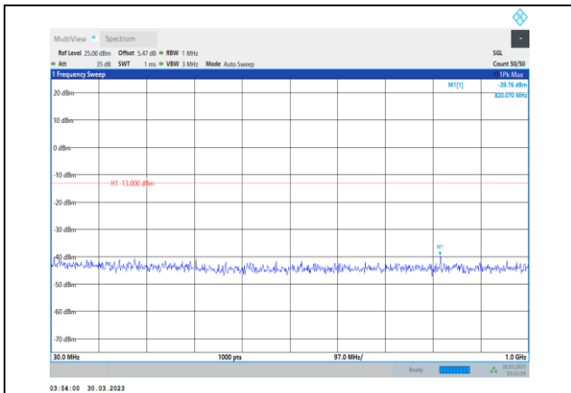
Band4-3MHz-64QAM-19965-1RB#0- Range1:30~1000MHz
