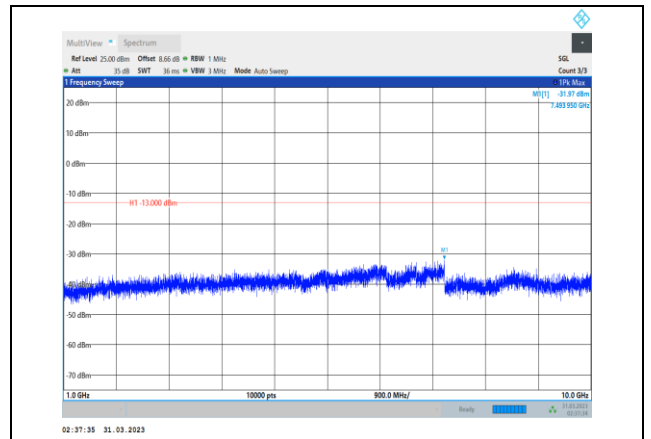
Band5-3MHz-16QAM-20525-1RB#0- Range2:1000~10000MHz
