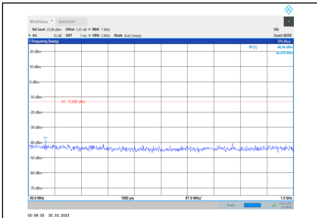
Band4-1.4MHz-64QAM-19957-1RB#0- Range1:30~1000MHz
