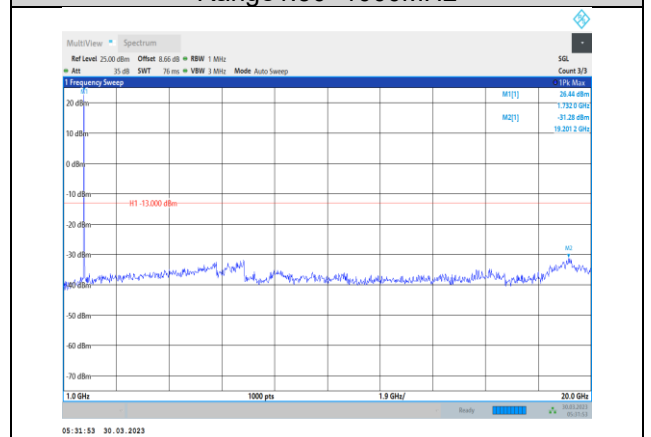
Band4-20MHz-64QAM-20300-1RB#0- Range2:1000~20000MHz
