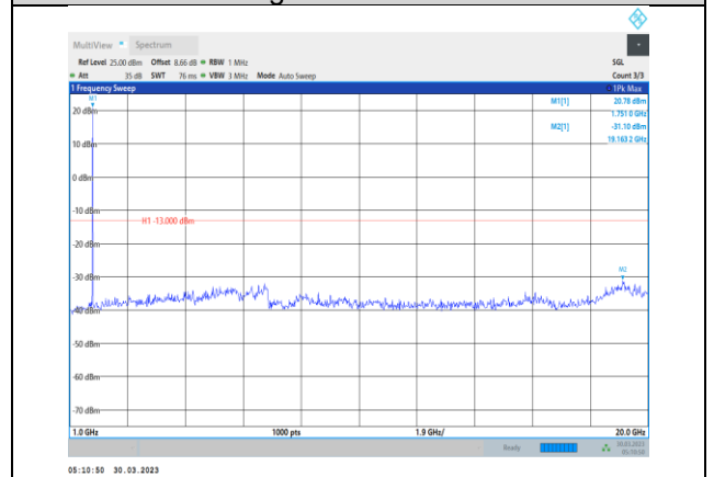
Band4-1.4MHz-64QAM-20393-1RB#0- Range2:1000~20000MHz
