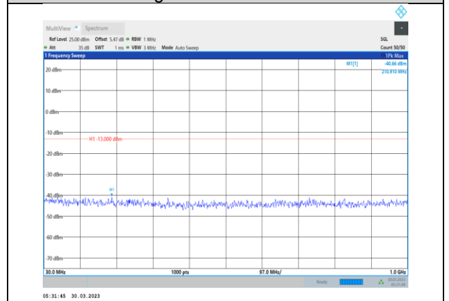
Band4-20MHz-64QAM-20300-1RB#0- Range1:30~1000MHz
