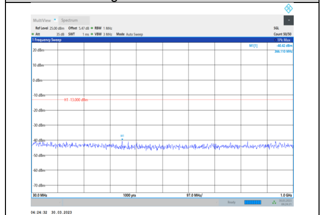
Band4-5MHz-64QAM-20375-1RB#0- Range1:30~1000MHz
