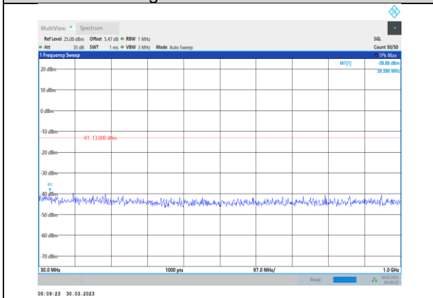
Band4-1.4MHz-64QAM-20175-1RB#0- Range1:30~1000MHz
