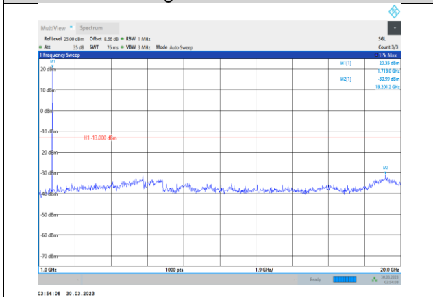
Band4-3MHz-64QAM-19965-1RB#0- Range2:1000~20000MHz
