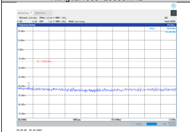
Band4-20MHz-64QAM-20175-1RB#0- Range1:30~1000MHz
