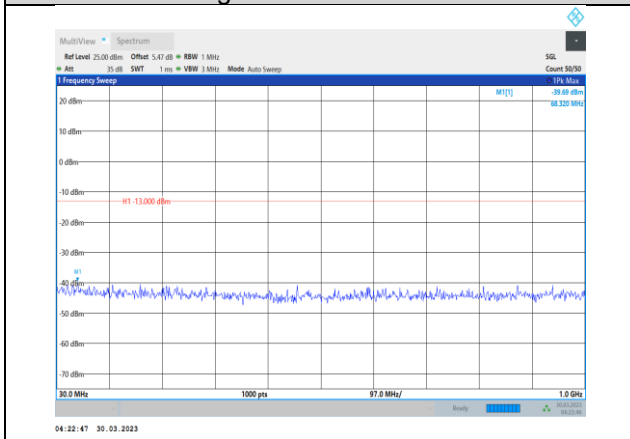
Band4-5MHz-16QAM-20175-1RB#0-Range1:30~1000MHz
