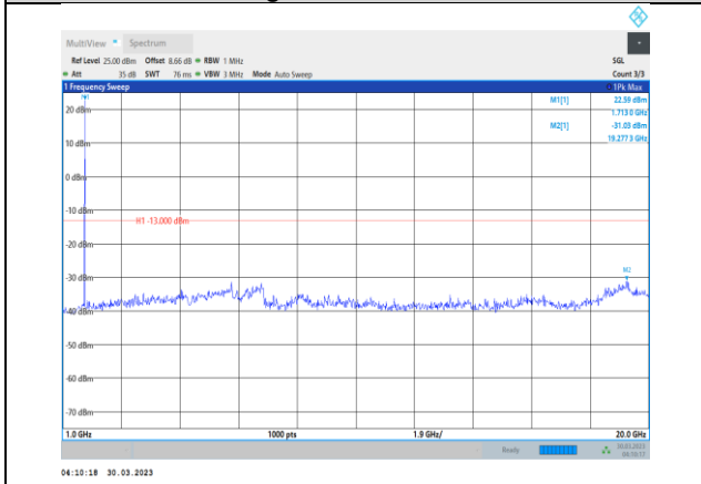
Band4-10MHz-64QAM-20000-1RB#0- Range2:1000~20000MHz
