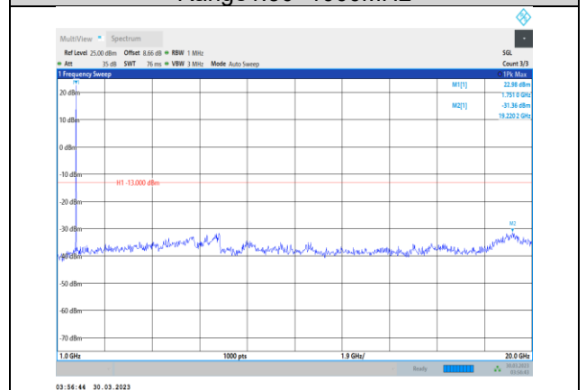
Band4-3MHz-64QAM-20385-1RB#0- Range2:1000~20000MHz
