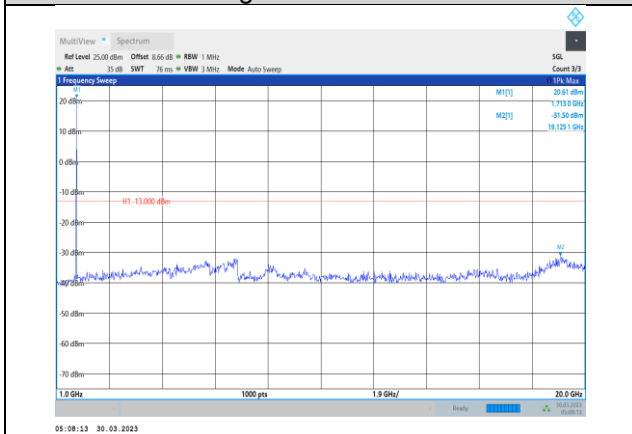
Band4-1.4MHz-64QAM-19957-1RB#0- Range2:1000~20000MHz
