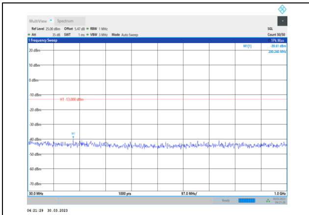
Band4-5MHz-16QAM-19975-1RB#0-Range1:30~1000MHz
