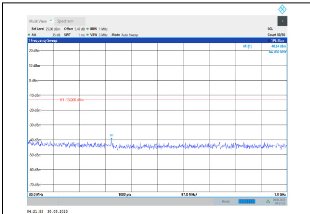
Band4-5MHz-64QAM-19975-1RB#0- Range1:30~1000MHz
