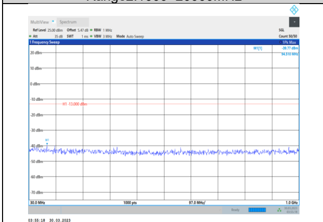
Band4-3MHz-64QAM-20175-1RB#0- Range1:30~1000MHz
