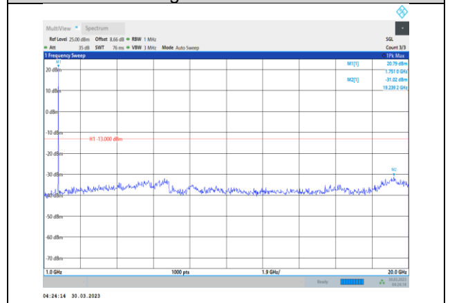
Band4-5MHz-16QAM-20375-1RB#0-Range2:1000~20000MHz
