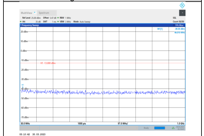
Band4-1.4MHz-64QAM-20393-1RB#0- Range1:30~1000MHz
