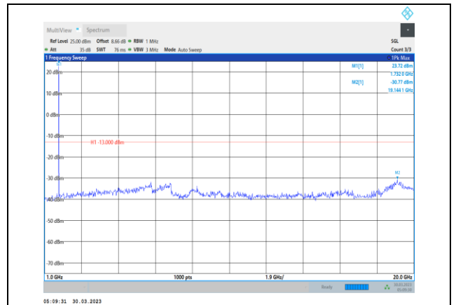
Band4-1.4MHz-64QAM-20175-1RB#0- Range2:1000~20000MHz
