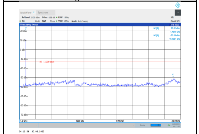
Band4-10MHz-64QAM-20350-1RB#0- Range2:1000~20000MHz
