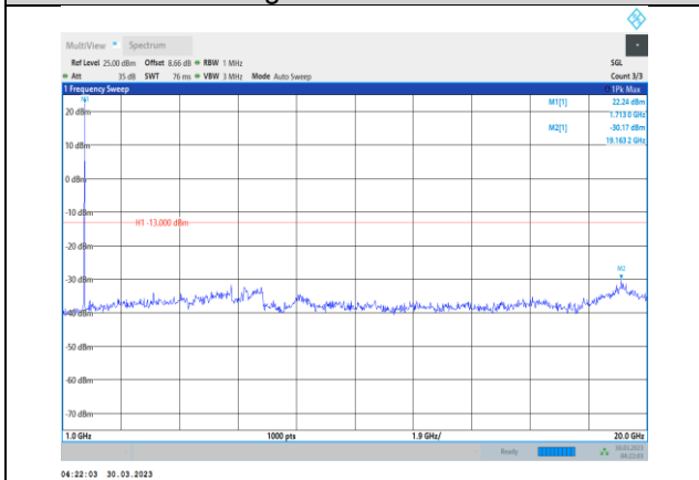
Band4-5MHz-64QAM-19975-1RB#0- Range2:1000~20000MHz
