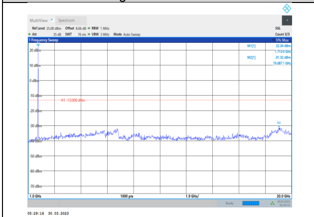
Band4-20MHz-64QAM-20050-1RB#0- Range2:1000~20000MHz
