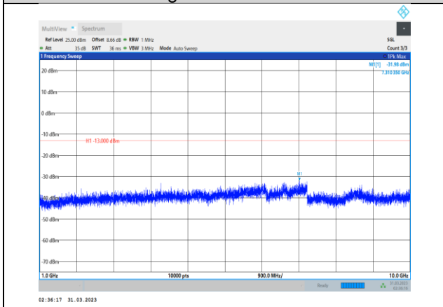
Band5-3MHz-16QAM-20415-1RB#0- Range2:1000~10000MHz
