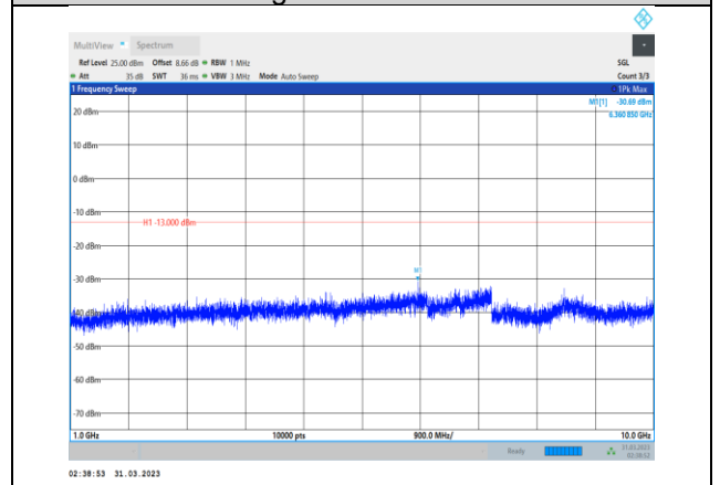
Band5-3MHz-16QAM-20635-1RB#0- Range2:1000~10000MHz
