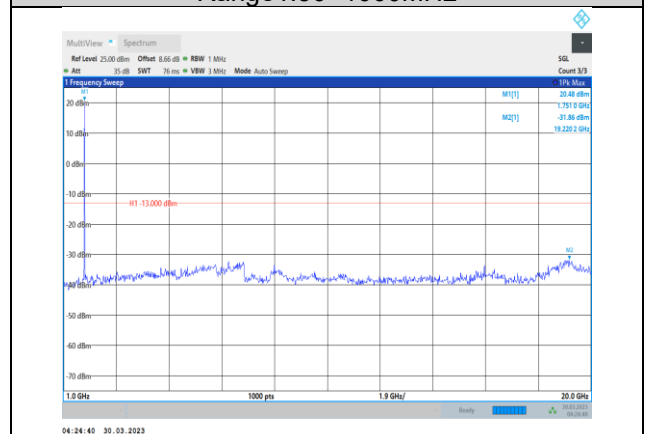
Band4-5MHz-64QAM-20375-1RB#0- Range2:1000~20000MHz
