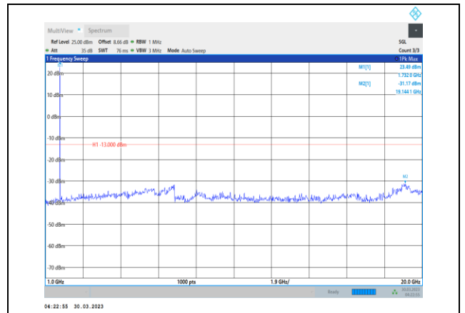
Band4-5MHz-16QAM-20175-1RB#0-Range2:1000~20000MHz
