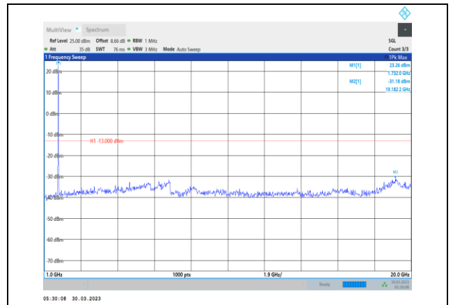
Band4-20MHz-16QAM-20175-1RB#0- Range2:1000~20000MHz
