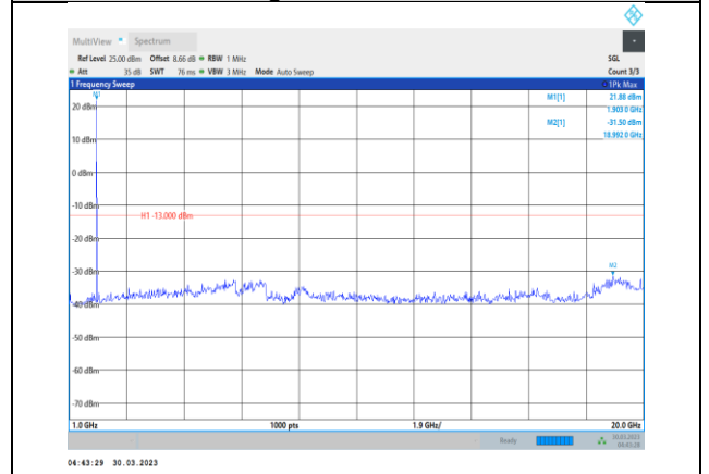
Band2-10MHz-64QAM-19150-1RB#0- Range2:1000~20000MHz
