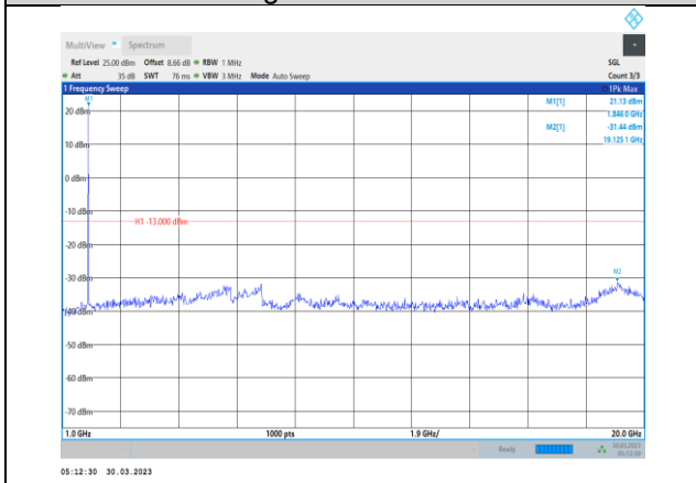
Band2-3MHz-16QAM-18615-1RB#0- Range2:1000~20000MHz
