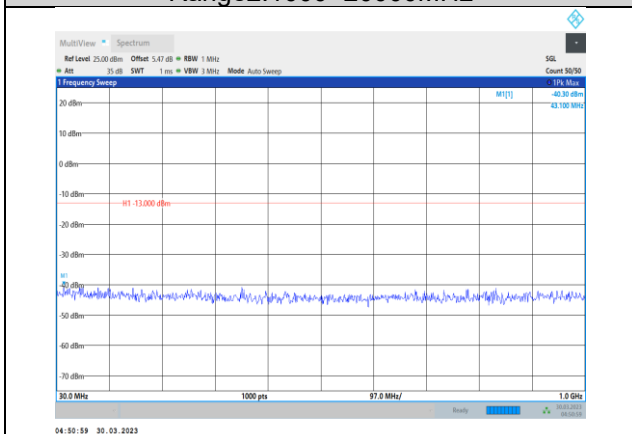
Band2-5MHz-64QAM-18900-1RB#0- Range1:30~1000MHz
