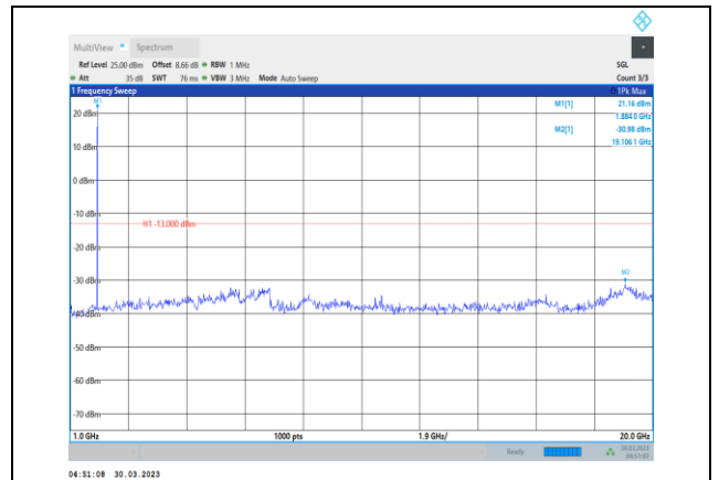
Band2-5MHz-64QAM-18900-1RB#0- Range2:1000~20000MHz
