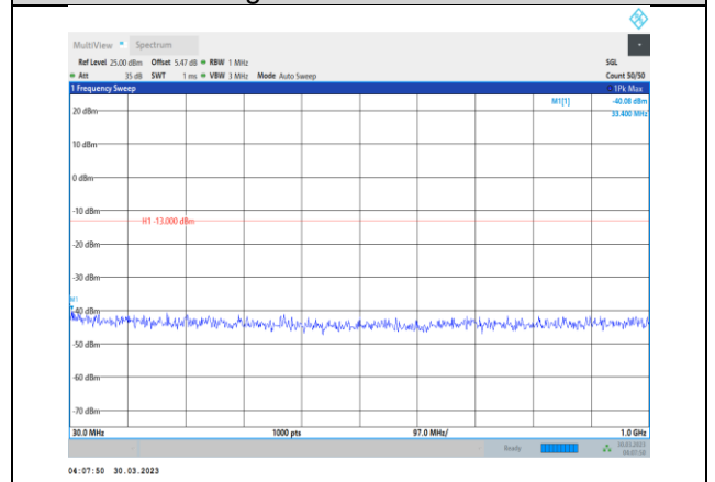
Band2-15MHz-16QAM-19125-1RB#0- Range1:30~1000MHz
