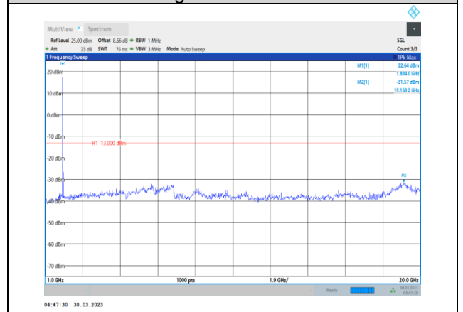
Band2-20MHz-16QAM-19100-1RB#0- Range2:1000~20000MHz
