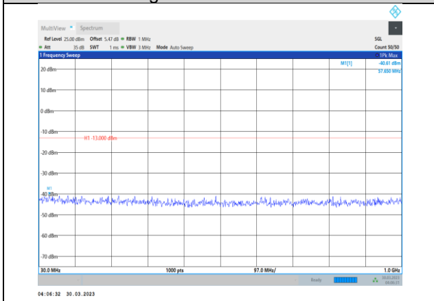
Band2-15MHz-16QAM-18900-1RB#0- Range1:30~1000MHz
