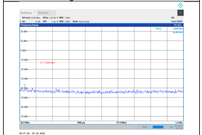
Band2-15MHz-QPSK-19125-1RB#0- Range1:30~1000MHz
