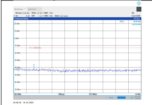
Band2-10MHz-64QAM-18900-1RB#0- Range1:30~1000MHz
