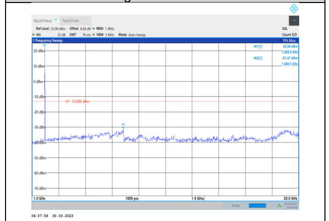
Band2-15MHz-16QAM-19125-1RB#0- Range2:1000~20000MHz
