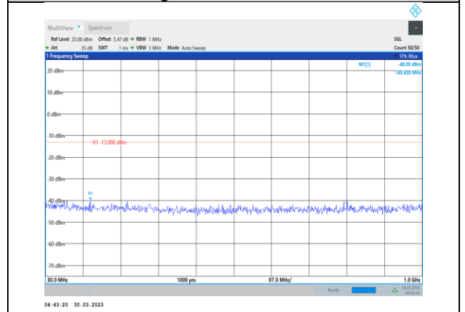
Band2-10MHz-64QAM-19150-1RB#0- Range1:30~1000MHz
