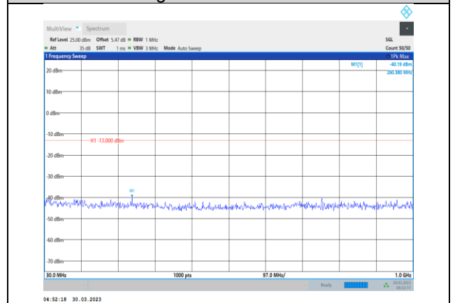
Band2-5MHz-64QAM-19175-1RB#0- Range1:30~1000MHz
