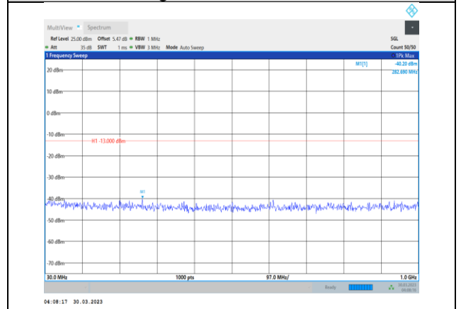
Band2-15MHz-64QAM-19125-1RB#0- Range1:30~1000MHz
