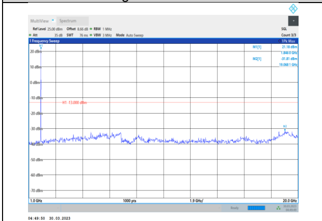
Band2-5MHz-64QAM-18625-1RB#0- Range2:1000~20000MHz
