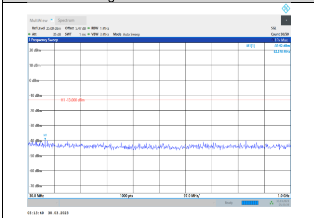
Band2-3MHz-16QAM-18900-1RB#0- Range1:30~1000MHz
