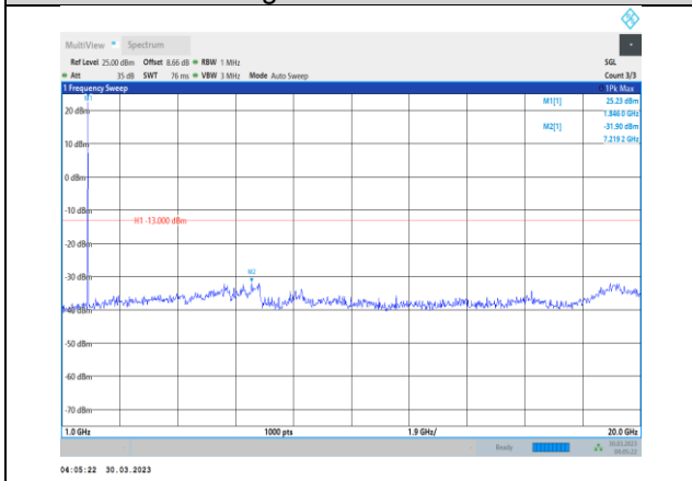
Band2-15MHz-16QAM-18675-1RB#0- Range2:1000~20000MHz
