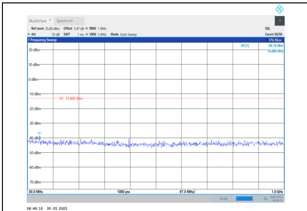
Band2-5MHz-16QAM-18625-1RB#0- Range1:30~1000MHz
