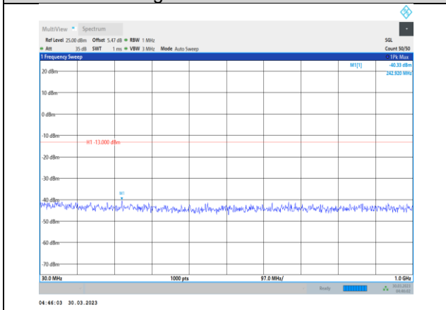
Band2-20MHz-16QAM-18900-1RB#0- Range1:30~1000MHz
