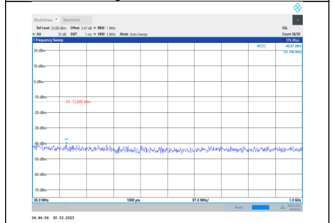
Band2-20MHz-QPSK-19100-1RB#0-Range1:30~1000MHz
