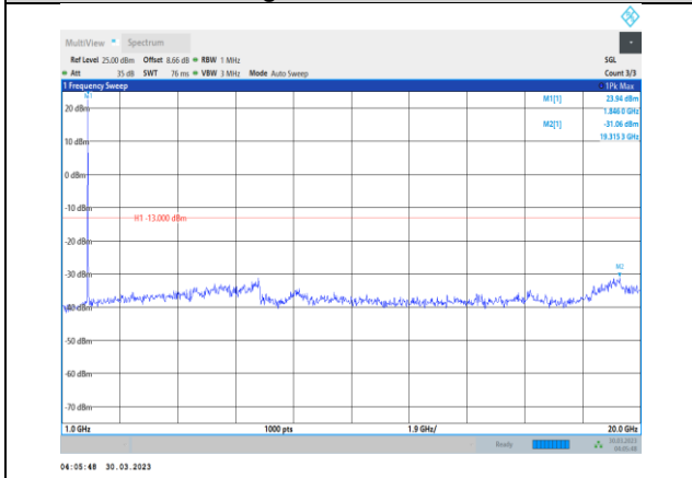
Band2-15MHz-64QAM-18675-1RB#0- Range2:1000~20000MHz
