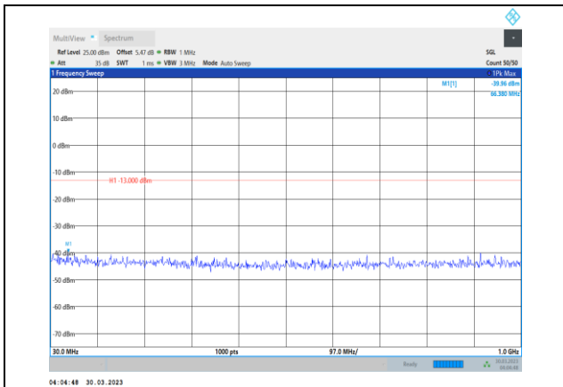
Band2-15MHz-QPSK-18675-1RB#0- Range1:30~1000MHz
