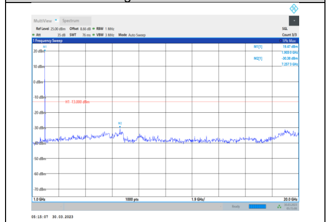
Band2-3MHz-16QAM-19185-1RB#0- Range2:1000~20000MHz
