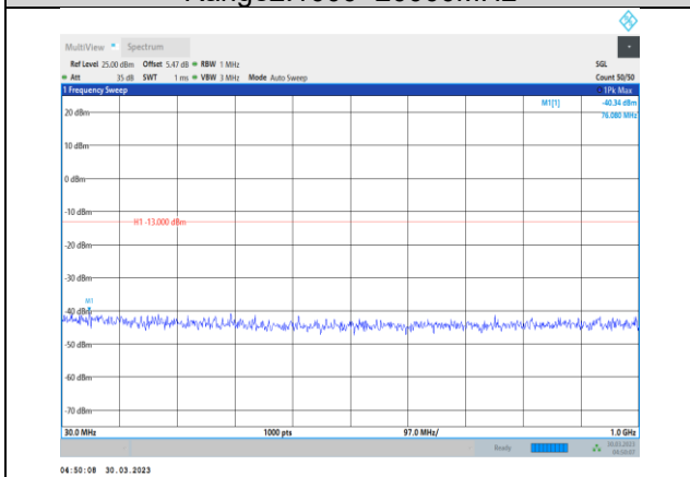
Band2-5MHz-QPSK-18900-1RB#0- Range1:30~1000MHz
