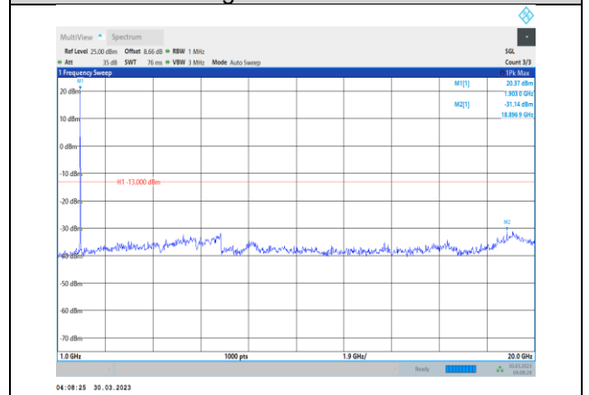
Band2-15MHz-64QAM-19125-1RB#0- Range2:1000~20000MHz
