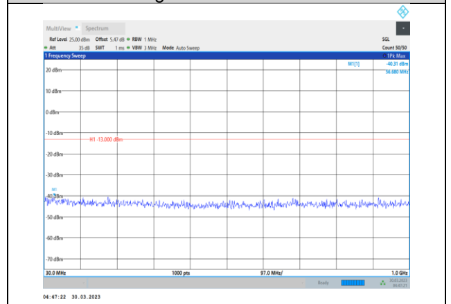
Band2-20MHz-16QAM-19100-1RB#0- Range1:30~1000MHz
