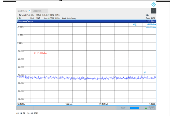
Band2-3MHz-16QAM-19185-1RB#0- Range1:30~1000MHz
