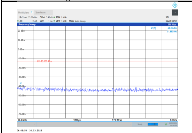
Band2-15MHz-64QAM-18900-1RB#0- Range1:30~1000MHz
