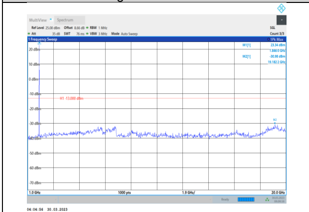
Band2-15MHz-QPSK-18675-1RB#0- Range2:1000~20000MHz
