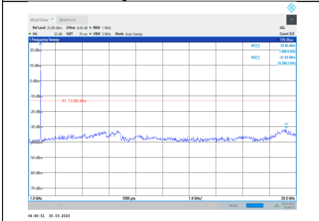
Band2-10MHz-64QAM-18650-1RB#0- Range2:1000~20000MHz
