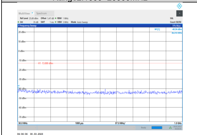
Band2-15MHz-QPSK-18900-1RB#0- Range1:30~1000MHz
