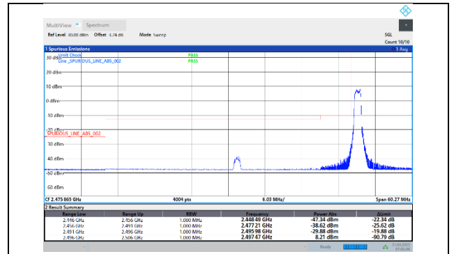
41-41-20MHz-20MHz-64QAM-64QAM-39750-39948-1RB#0-1RB#0
