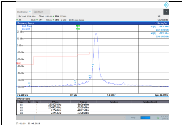
Band41-20MHz-64QAM-40340-1RB#0
