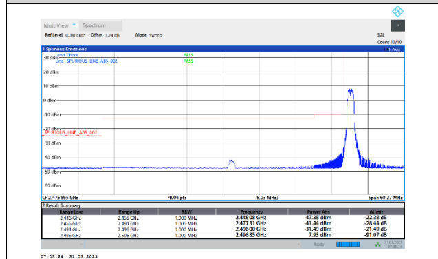
41-41-20MHz-20MHz-16QAM-16QAM-39750-39948-1RB#0-1RB#0
