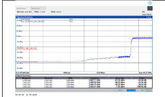
41-41-20MHz-20MHz-16QAM-16QAM-39750-39948-100RB#0-100RB#0
