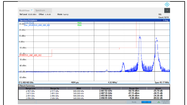
41-41-5MHz-20MHz-16QAM-16QAM-39683-39800-1RB#0-1RB#0
