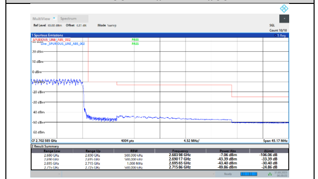
41-41-5MHz-20MHz-16QAM-16QAM-41373-41490-25RB#0-100RB#0
