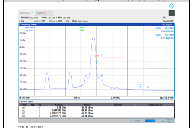
Band41-10MHz-64QAM-41540-1RB#49
