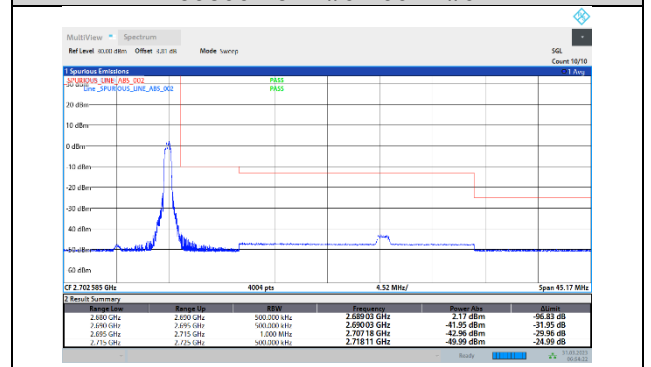
41-41-5MHz-20MHz-16QAM-16QAM-41373-41490-1RB#24-1RB#99
