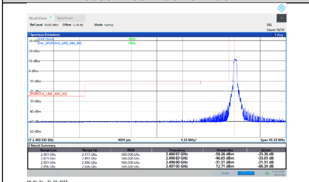
41-41-20MHz-5MHz-64QAM-64QAM-39750-39867-1RB#0-0RB#0
