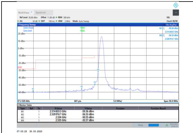
Band41-20MHz-16QAM-40140-1RB#0
