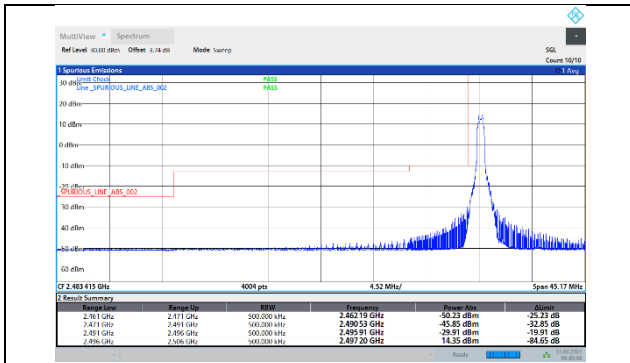
41-41-20MHz-5MHz-QPSK-QPSK-39750-39867-1RB#0-0RB#0
