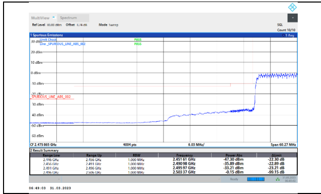
41-41-20MHz-20MHz-QPSK-QPSK-39750-39948-100RB#0-100RB#0
