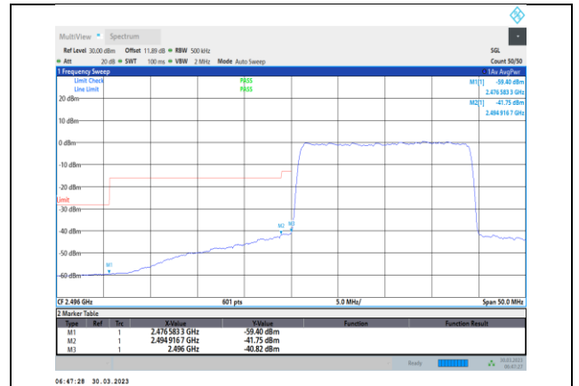
Band41-20MHz-64QAM-39750-100RB#0
