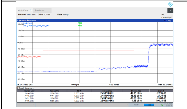
41-41-20MHz-20MHz-64QAM-64QAM-39750-39948-100RB#0-100RB#0
