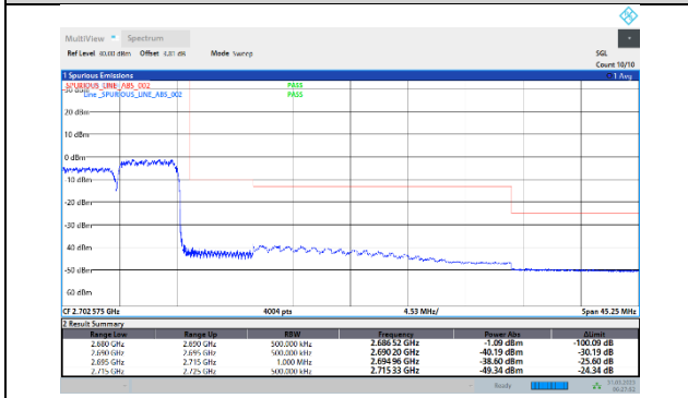
41-41-20MHz-5MHz-QPSK-QPSK-41440-41557-100RB#0-25RB#0
