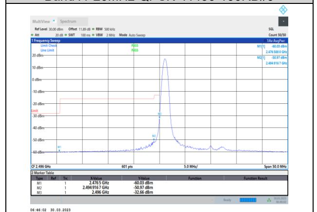
Band41-20MHz-16QAM-39750-1RB#0
