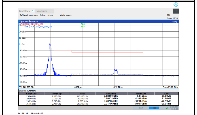
41-41-5MHz-20MHz-64QAM-64QAM-41373-41490-1RB#24-1RB#99
