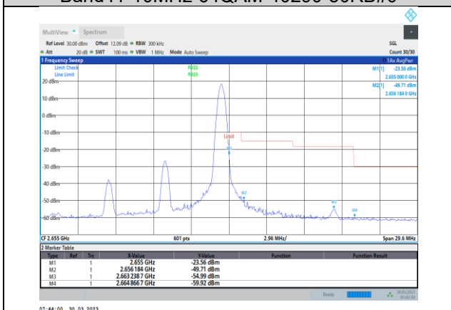
Band41-10MHz-64QAM-41190-1RB#49
