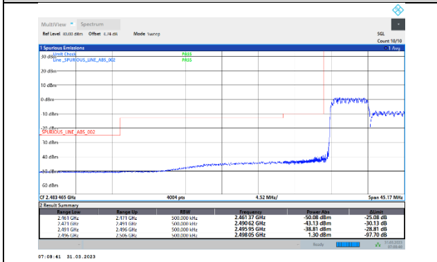
41-41-5MHz-20MHz-64QAM-64QAM-39683-39800-1RB#0-1RB#0
