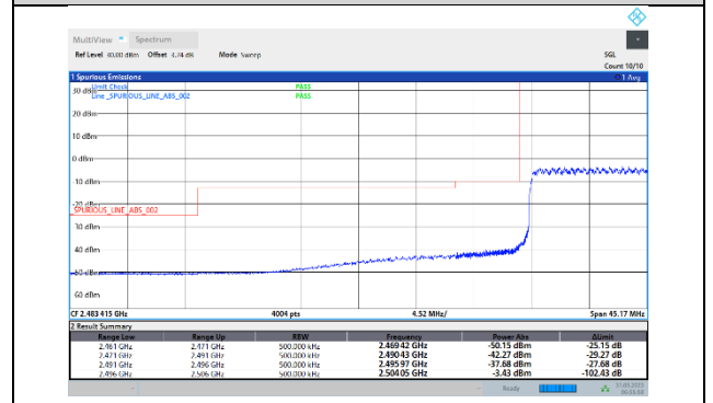
41-41-20MHz-5MHz-QPSK-QPSK-39750-39867-100RB#0-25RB#0
