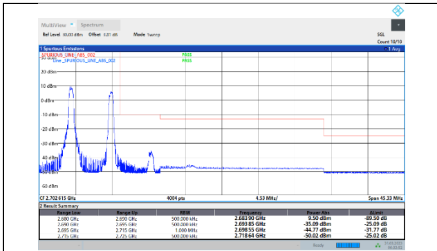
41-41-20MHz-5MHz-16QAM-16QAM-41440-41557-1RB#99-1RB#24
