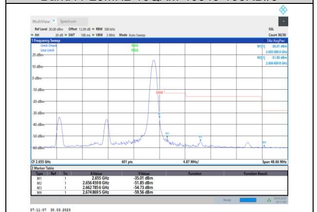
Band41-20MHz-16QAM-41140-1RB#99
