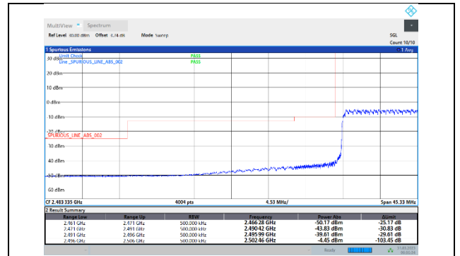
41-41-20MHz-5MHz-16QAM-16QAM-39750-39867-100RB#0-25RB#0
