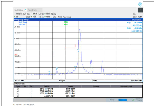
Band41-10MHz-64QAM-40290-1RB#0
