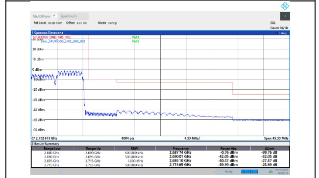
41-41-20MHz-5MHz-16QAM-16QAM-41440-41557-100RB#0-25RB#0
