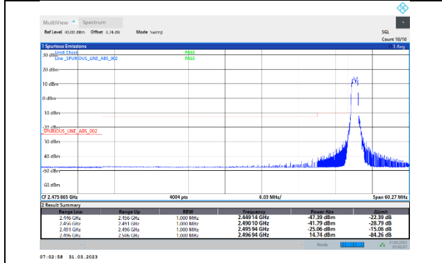
41-41-20MHz-20MHz-QPSK-QPSK-39750-39948-1RB#0-0RB#0
