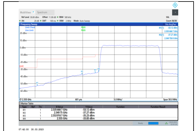
Band41-20MHz-16QAM-40340-100RB#0
