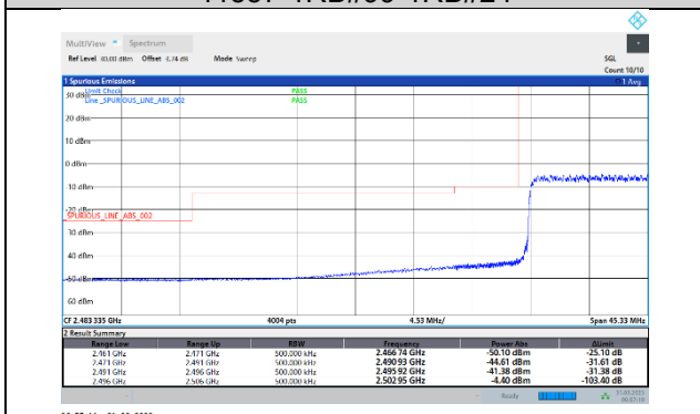
41-41-20MHz-5MHz-64QAM-64QAM-39750-39867-100RB#0-25RB#0
