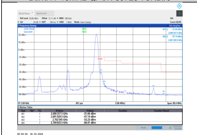
Band41-15MHz-QPSK-41515-1RB#74
