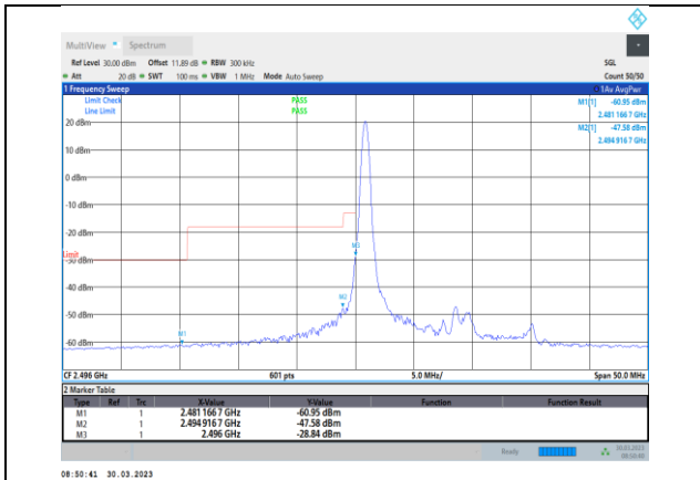
Band41-15MHz-QPSK-39725-1RB#0
