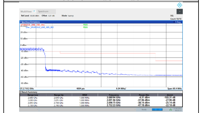
41-41-20MHz-20MHz-64QAM-64QAM-41292-41490-100RB#0-100RB#0
