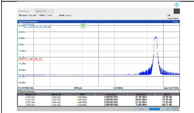
41-41-20MHz-20MHz-64QAM-64QAM-39750-39948-1RB#0-0RB#0
