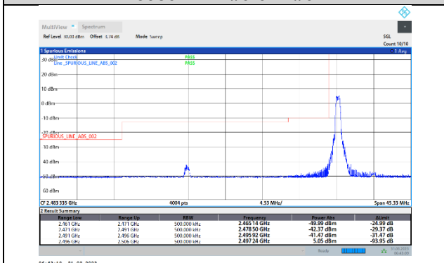
41-41-20MHz-5MHz-64QAM-64QAM-39750-39867-1RB#0-1RB#0
