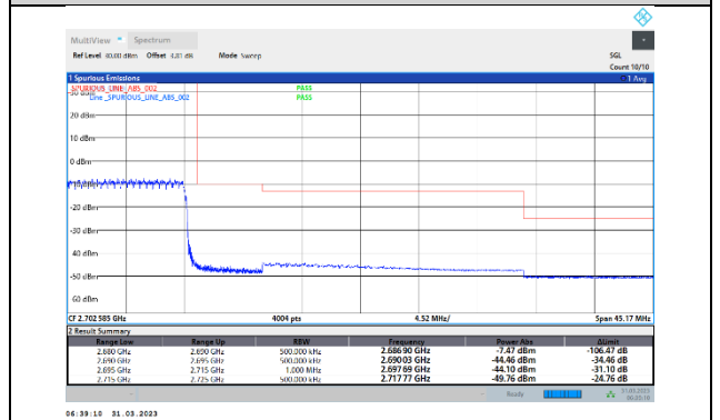
41-41-5MHz-20MHz-64QAM-64QAM-41373-41490-25RB#0-100RB#0
