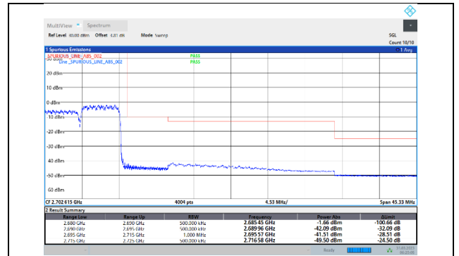
41-41-20MHz-5MHz-64QAM-64QAM-41440-41557-100RB#0-25RB#0
