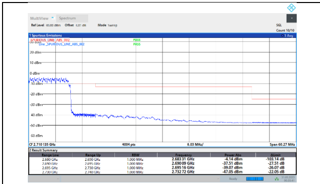
41-41-20MHz-20MHz-16QAM-16QAM-41292-41490-100RB#0-100RB#0
