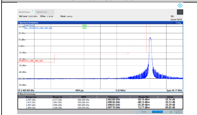
41-41-5MHz-20MHz-16QAM-16QAM-39683-39800-1RB#0-0RB#0
