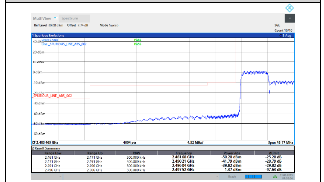
41-41-5MHz-20MHz-16QAM-16QAM-39683-39800-25RB#0-100RB#0
