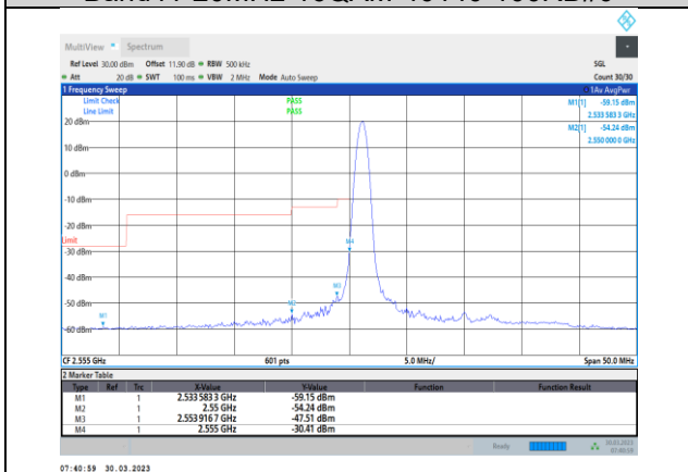
Band41-20MHz-16QAM-40340-1RB#0
