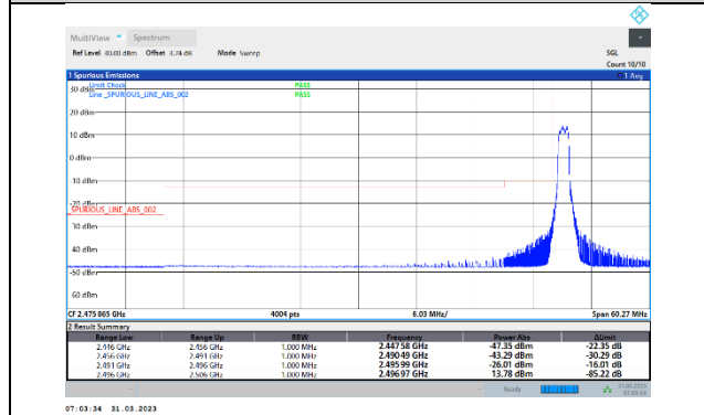
41-41-20MHz-20MHz-16QAM-16QAM-39750-39948-1RB#0-0RB#0
