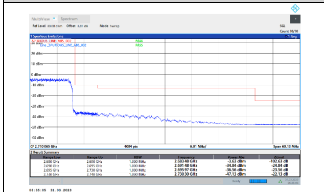
41-41-20MHz-20MHz-QPSK-QPSK-41292-41490-100RB#0-100RB#0
