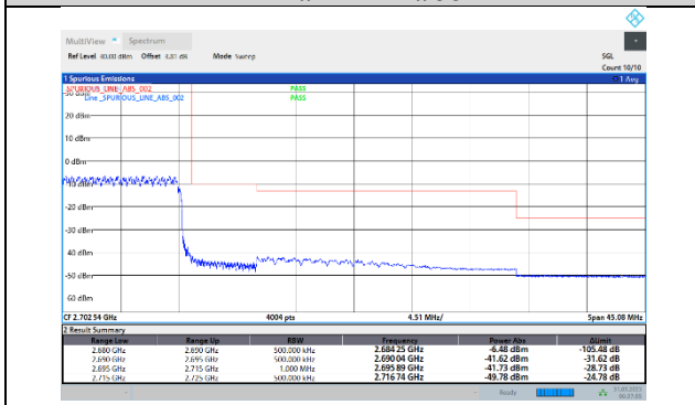
41-41-5MHz-20MHz-QPSK-QPSK-41373-41490-25RB#0-100RB#0
