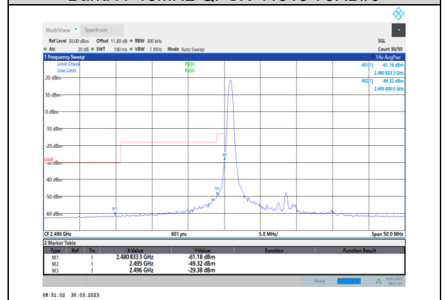
Band41-15MHz-16QAM-39725-1RB#0
