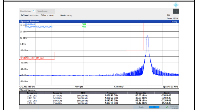
41-41-20MHz-5MHz-16QAM-16QAM-39750-39867-1RB#0-0RB#0
