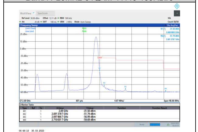
Band41-20MHz-64QAM-41490-100RB#0
