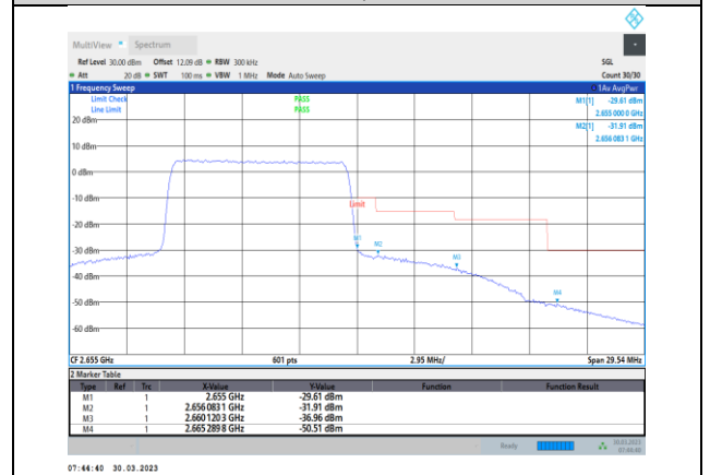
Band41-10MHz-16QAM-41190-50RB#0
