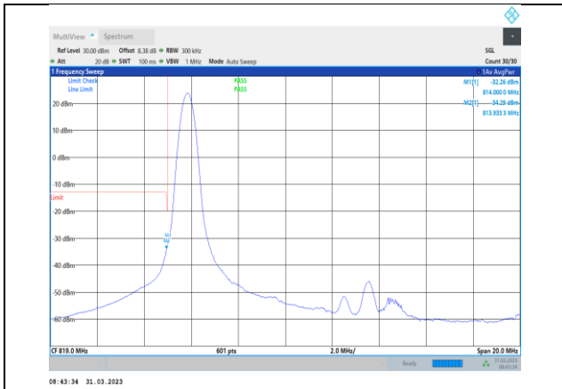
Band26-15MHz-16QAM-26765-1RB#0
