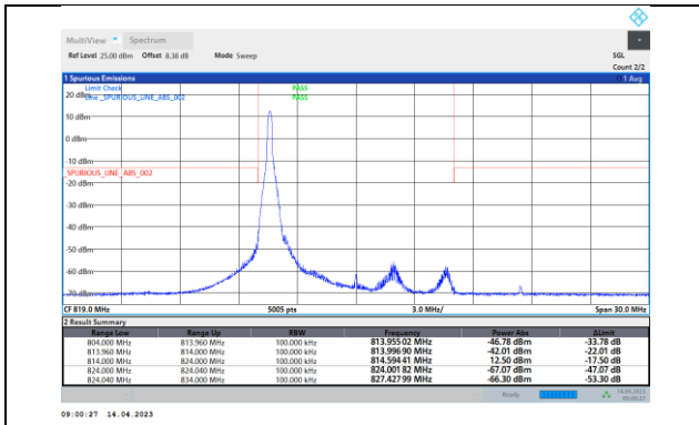
26(814-824)-10MHz-16QAM-26740-1RB#0
