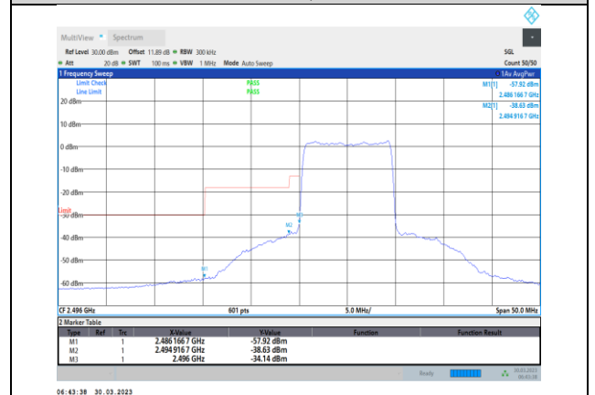
Band41-10MHz-16QAM-39700-50RB#0
