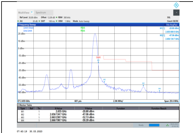
Band41-10MHz-QPSK-41190-1RB#49
