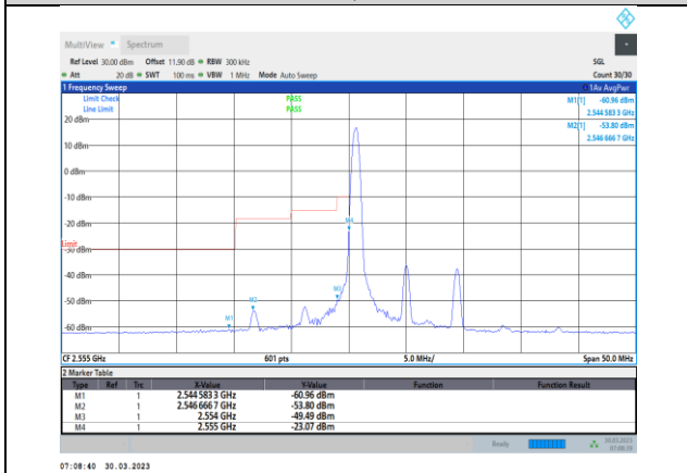
Band41-10MHz-16QAM-40290-1RB#0
