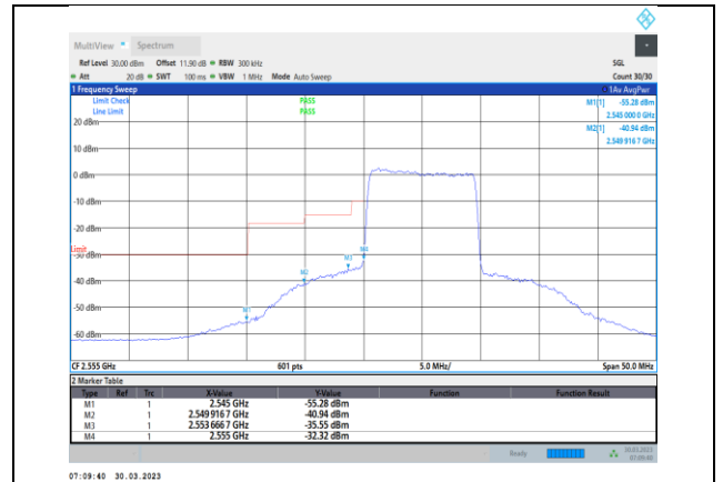
Band41-10MHz-16QAM-40290-50RB#0
