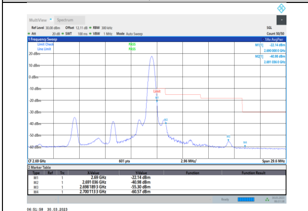
Band41-10MHz-QPSK-41540-1RB#49
