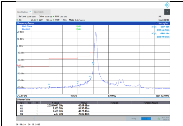
Band38-15MHz-QPSK-37825-1RB#0
