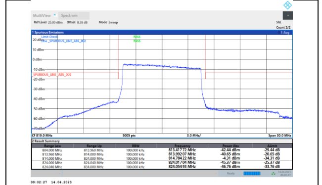
26(814-824)-10MHz-QPSK-26740-50RB#0
