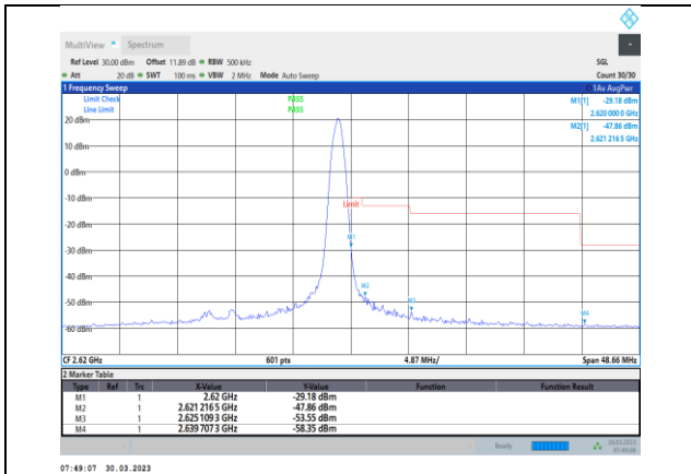
Band38-20MHz-16QAM-38150-1RB#99
