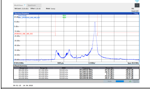
26(814-824)-10MHz-QPSK-26740-1RB#49
