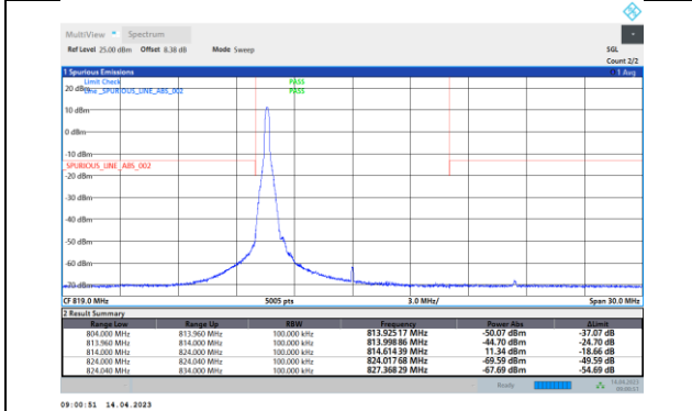
26(814-824)-10MHz-64QAM-26740-1RB#0
