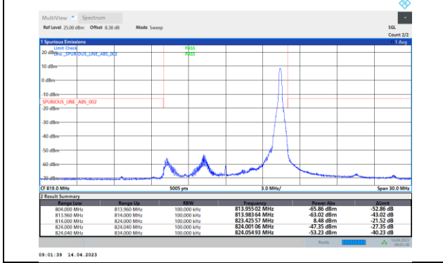
26(814-824)-10MHz-16QAM-26740-1RB#49
