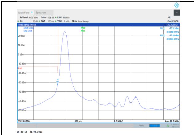
Band26-15MHz-QPSK-26765-1RB#0
