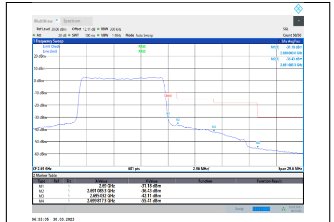
Band41-10MHz-QPSK-41540-50RB#0
