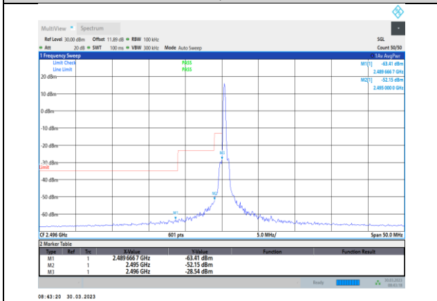
Band41-5MHz-64QAM-39675-1RB#0
