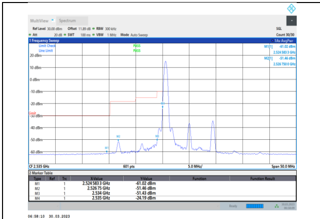
Band41-10MHz-16QAM-40090-1RB#0
