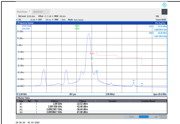
Band41-10MHz-16QAM-41540-1RB#49
