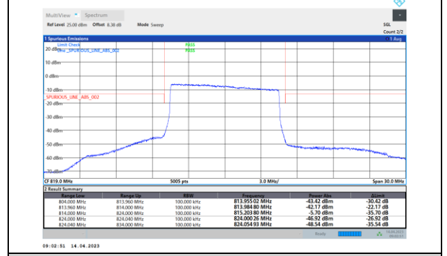
26(814-824)-10MHz-16QAM-26740-50RB#0
