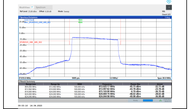
26(814-824)-10MHz-64QAM-26740-50RB#0
