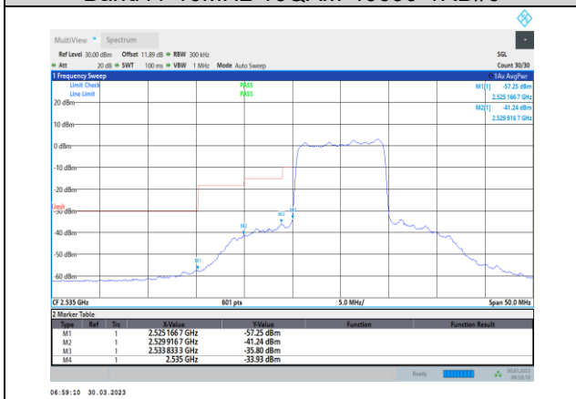
Band41-10MHz-16QAM-40090-50RB#0
