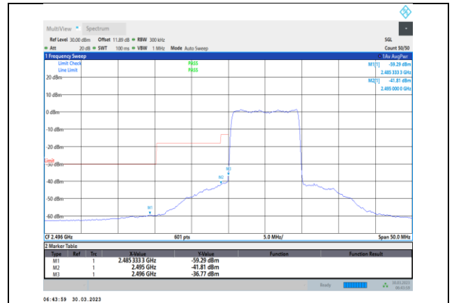
Band41-10MHz-64QAM-39700-50RB#0
