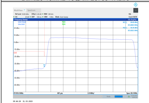
Band26-15MHz-16QAM-26765-75RB#0
