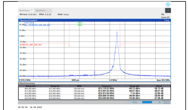
26(814-824)-10MHz-64QAM-26740-1RB#49
