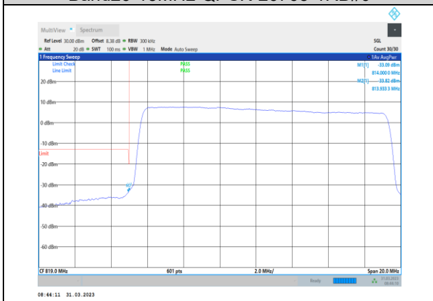
Band26-15MHz-QPSK-26765-75RB#0
