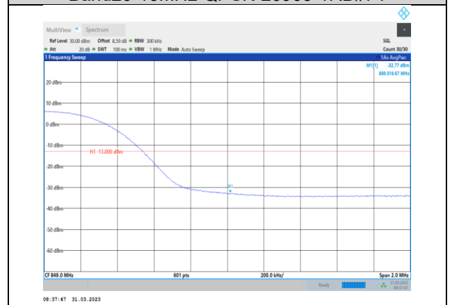
Band26-15MHz-QPSK-26965-75RB#0
