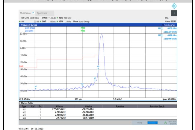
Band38-20MHz-16QAM-37850-1RB#0
