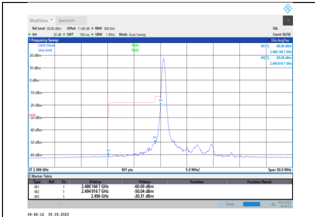
Band41-10MHz-QPSK-39700-1RB#0
