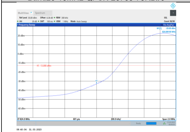
Band26-15MHz-QPSK-26865-1RB#0
