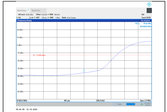
Band26-15MHz-QPSK-26865-75RB#0
