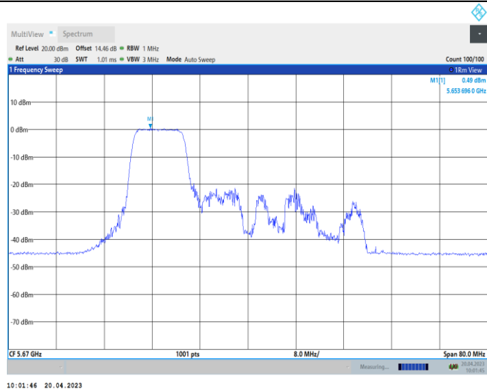
11AX40_Ant10_5670_242Tone_RU61
