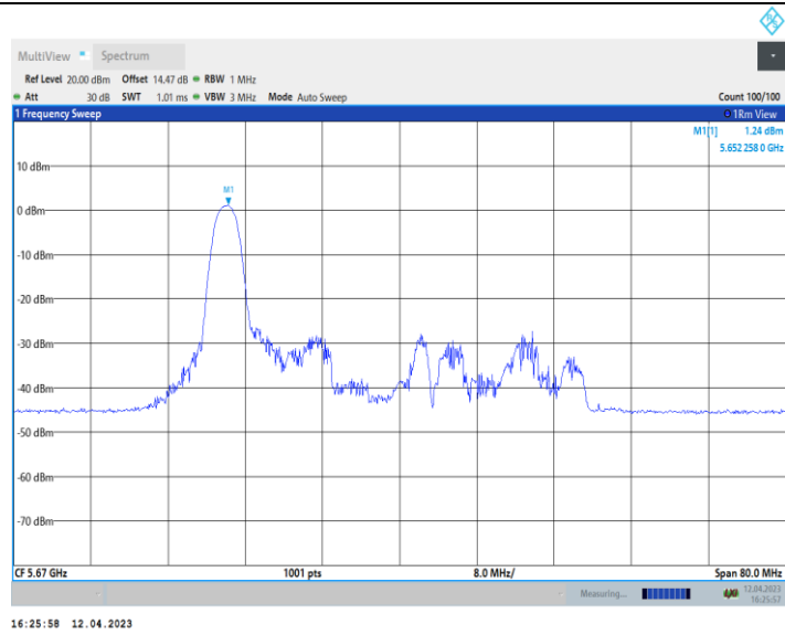
11AX40_Ant10_5670_52Tone_RU37
