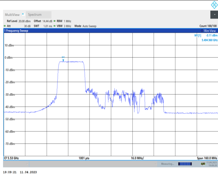
11AX80_Ant9_5530_484Tone_RU61
