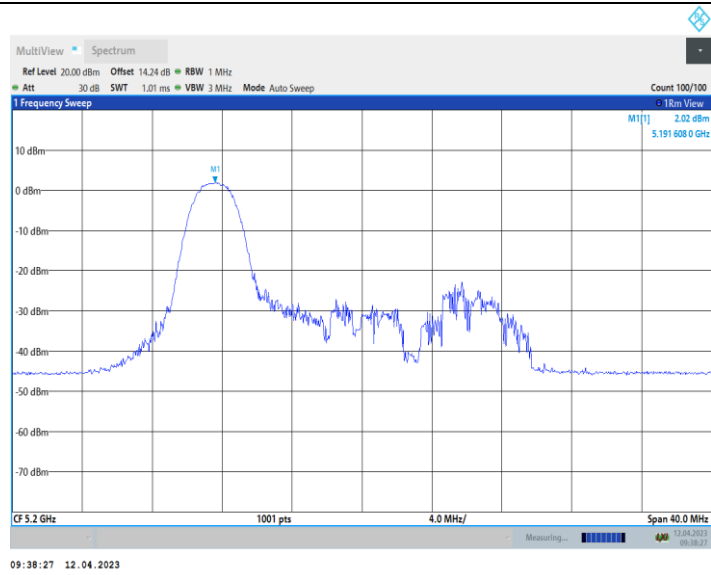
11AX20_Ant10_5200_52Tone_RU37
