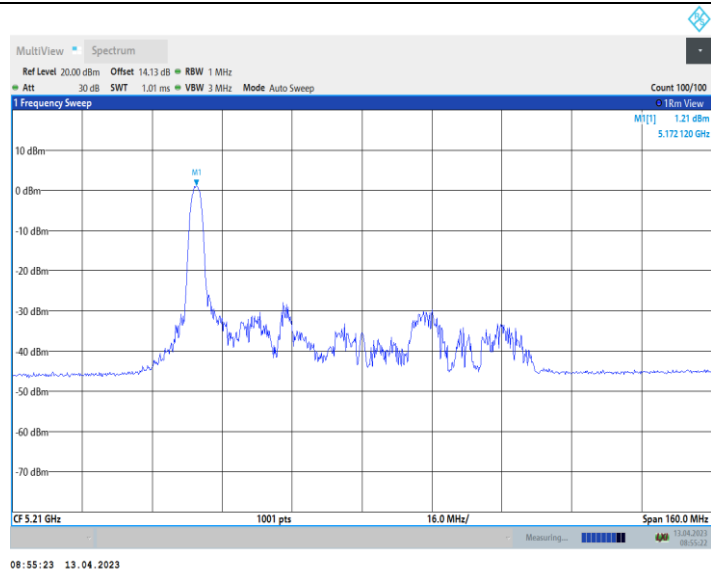
11AX80_Ant10_5210_52Tone_RU37
