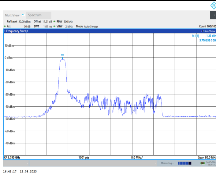
11AX40_Ant10_5795_52Tone_RU37
