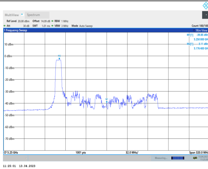
11AX160_Ant9_5250_UNII-1_242Tone_RU61
