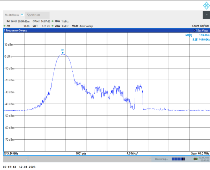
11AX20_Ant10_5240_52Tone_RU37
