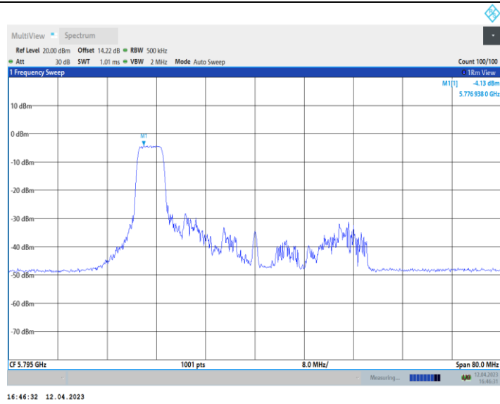
11AX40_Ant10_5795_106Tone_RU53
