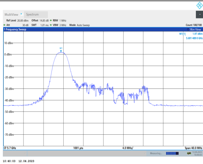
11AX20_Ant10_5700_52Tone_RU37
