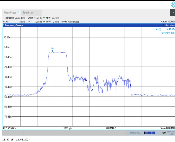
11AX40_Ant10_5755_242Tone_RU61
