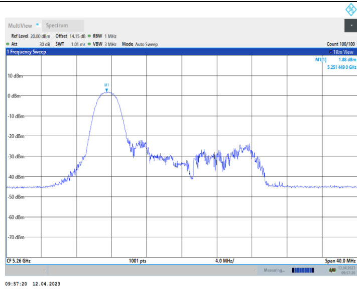
11AX20_Ant10_5260_52Tone_RU37
