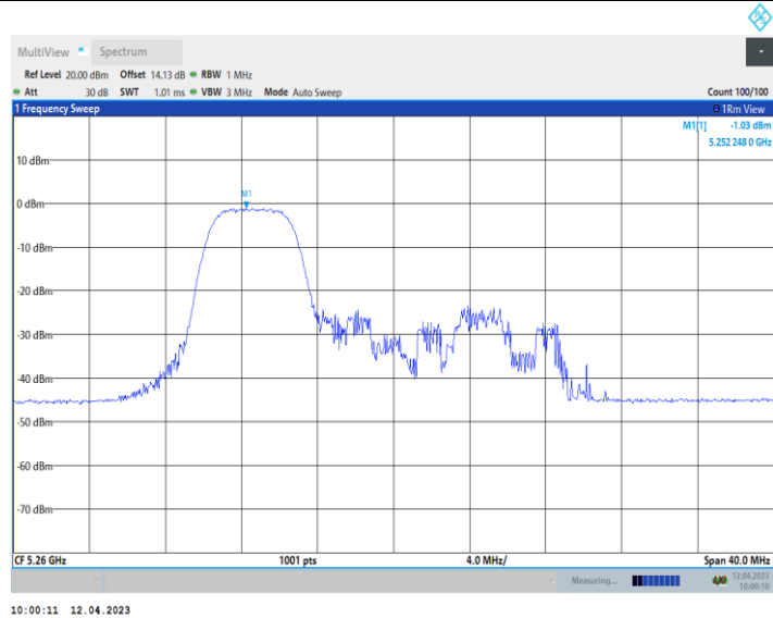
11AX20_Ant10_5260_106Tone_RU53
