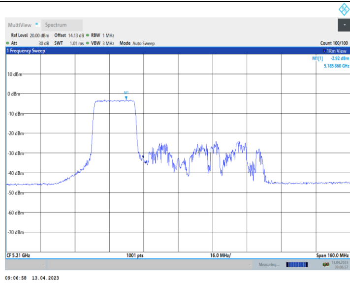
11AX80_Ant10_5210_484Tone_RU65
