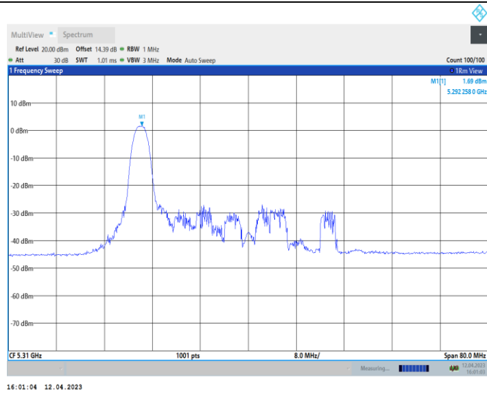
11AX40_Ant10_5310_52Tone_RU37
