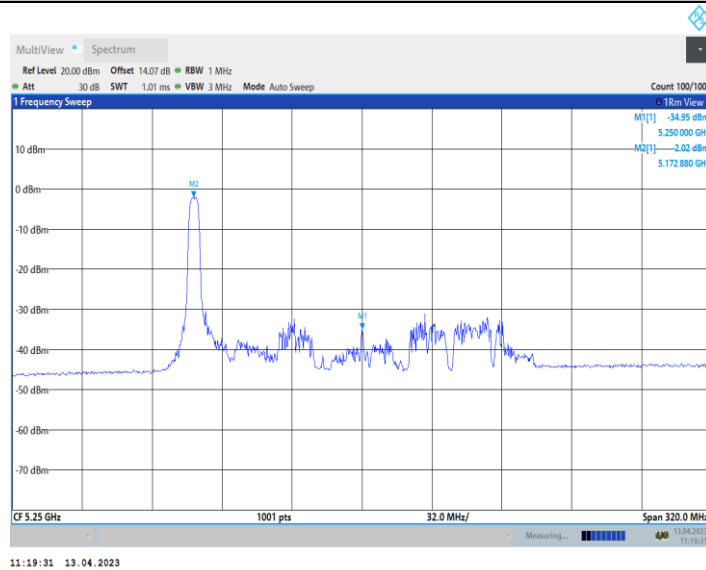
11AX160_Ant9_5250_UNII-1_106Tone_RU53
