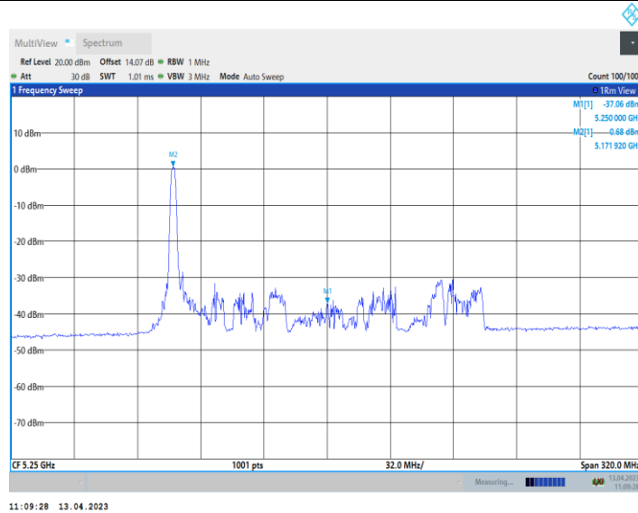
11AX160_Ant9_5250_UNII-1_52Tone_RU37
