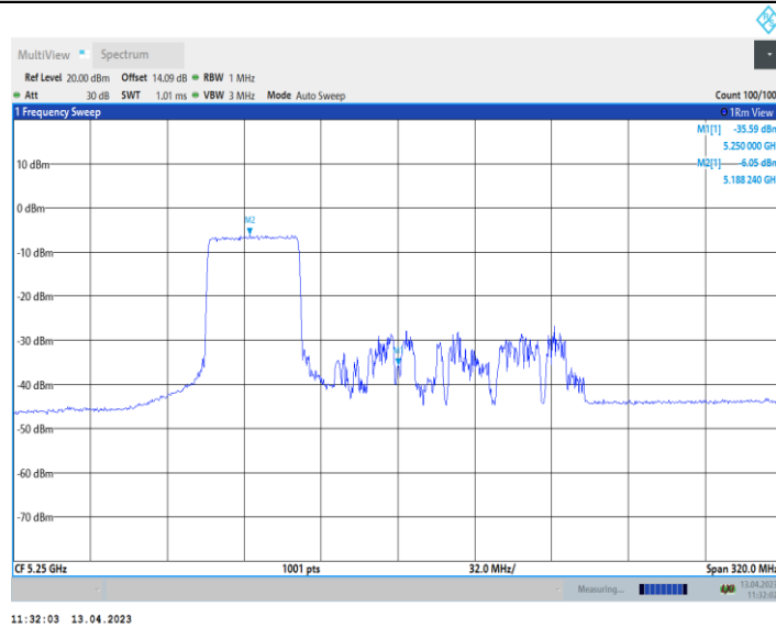
11AX160_Ant9_5250_UNII-1_996Tone_RU67
