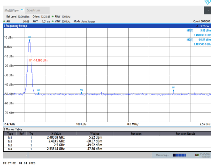
BLE_BT4.0_Ant9_High_2480
