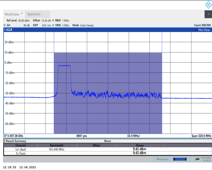
11AX160_Ant9_5570_484Tone_RU65
