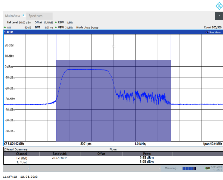
11AX40_Ant10_5190_26Tone_RU0
