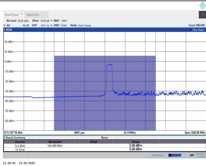
11AX160_Ant9_5250_UNII-1_242Tone_RU61
