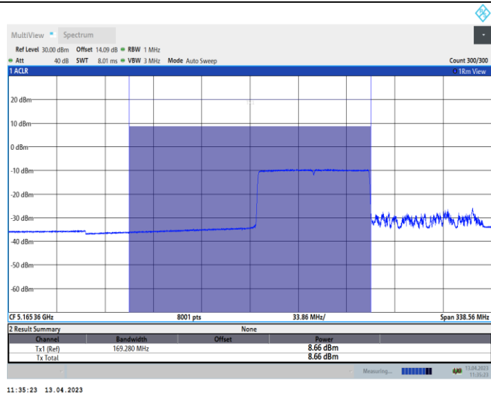
11AX160_Ant9_5250_UNII-2A_26Tone_RU0
