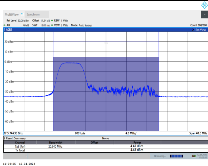
11AX20_Ant10_5745_106Tone_RU53
