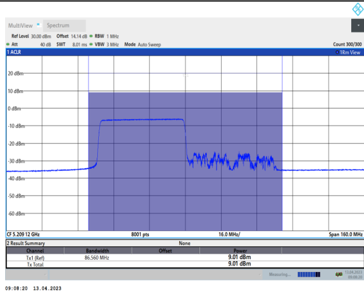
11AX80_Ant10_5290_26Tone_RU0
