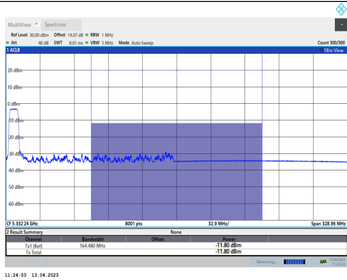
11AX160_Ant9_5250_UNII-2A_242Tone_RU61
