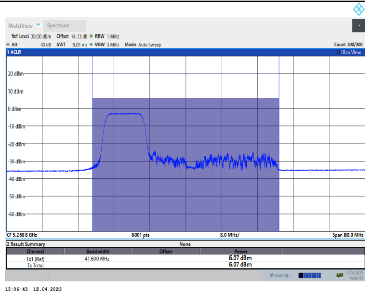
11AX40_Ant10_5270_242Tone_RU61
