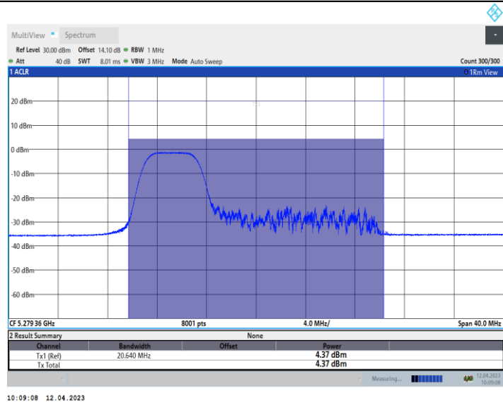
11AX20_Ant10_5280_106Tone_RU53
