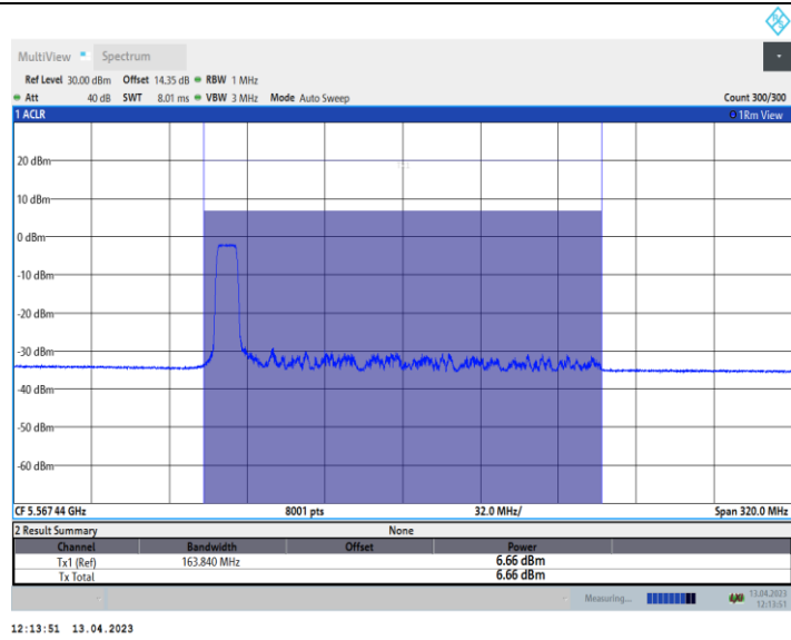
11AX160_Ant9_5570_242Tone_RU61
