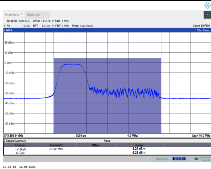
11AX20_Ant10_5600_106Tone_RU53
