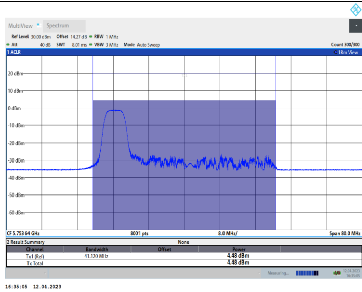
11AX40_Ant10_5755_106Tone_RU53
