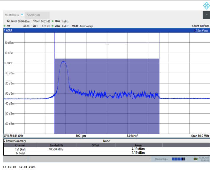
11AX40_Ant10_5795_52Tone_RU37
