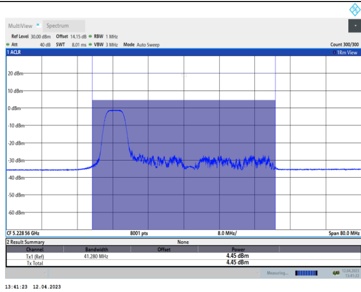
11AX40_Ant10_5230_106Tone_RU53
