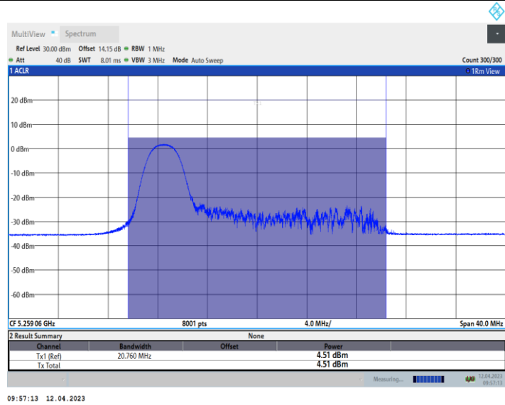
11AX20_Ant10_5260_52Tone_RU37
