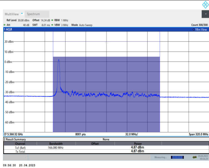
11AX160_Ant9_5570_52Tone_RU37
