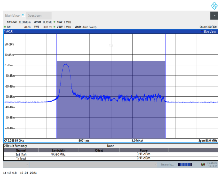
11AX40_Ant10_5590_52Tone_RU37
