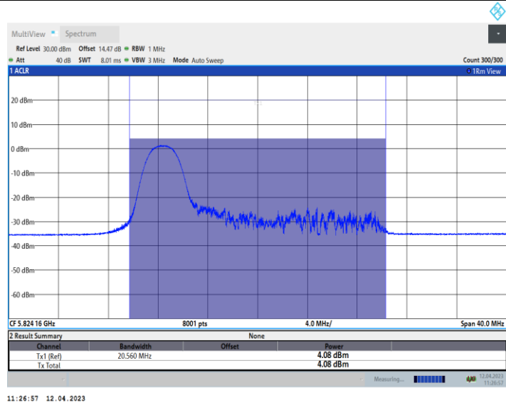
11AX20_Ant10_5825_52Tone_RU37
