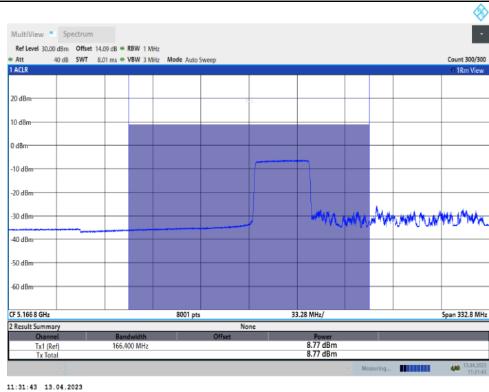
11AX160_Ant9_5250_UNII-1_996Tone_RU67
