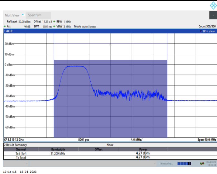
11AX20_Ant10_5320_106Tone_RU53
