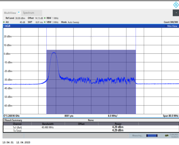
11AX40_Ant10_5270_52Tone_RU37
