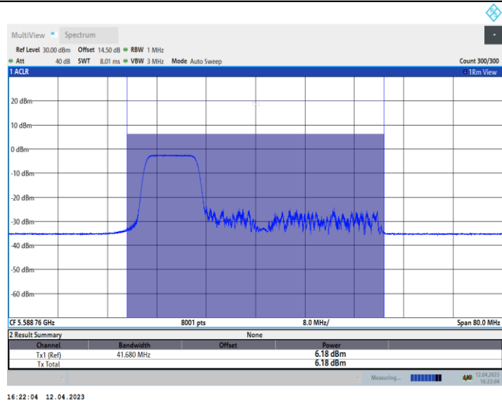
11AX40_Ant10_5590_242Tone_RU61
