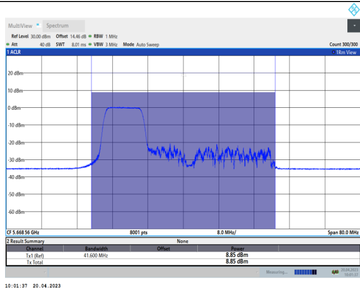
11AX40_Ant10_5670_242Tone_RU61
