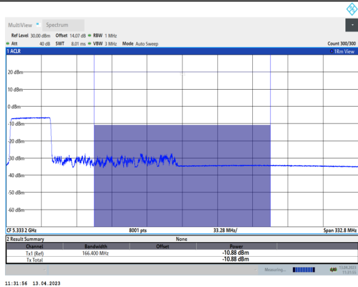
11AX160_Ant9_5250_UNII-2A_996Tone_RU67
