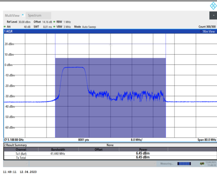
11AX40_Ant10_5190_242Tone_RU61
