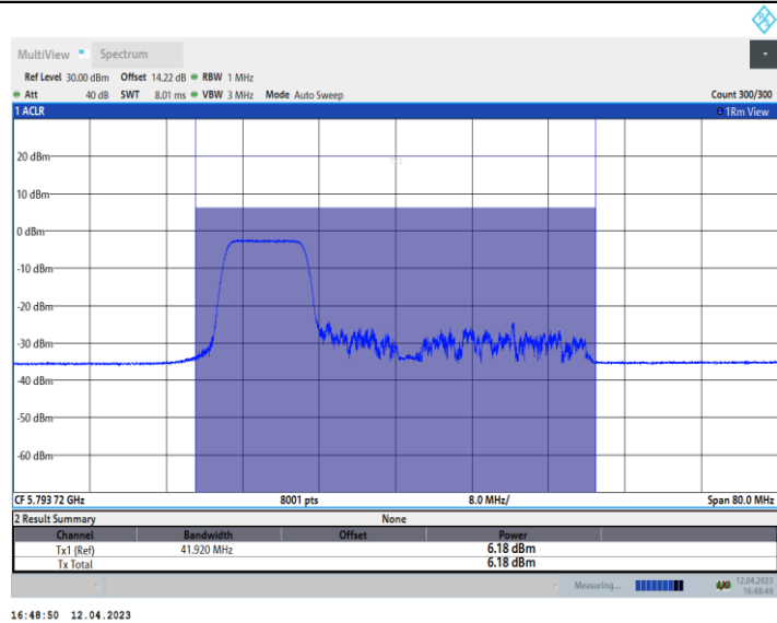
11AX40_Ant10_5795_242Tone_RU61
