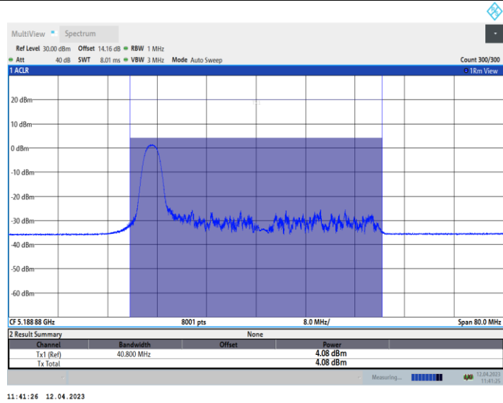
11AX40_Ant10_5190_52Tone_RU37
