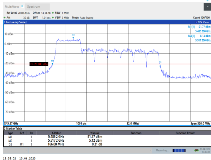
11AX160_Ant9_5570_996Tone_RU67
