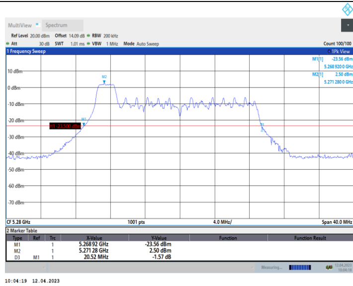
11AX20_Ant10_5280_52Tone_RU37
