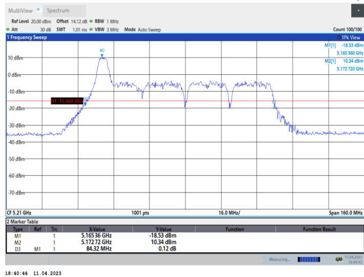
11AX80_Ant9_5210_242Tone_RU61
