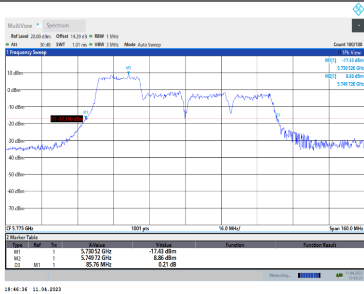
11AX80_Ant9_5775_484Tone_RU65
