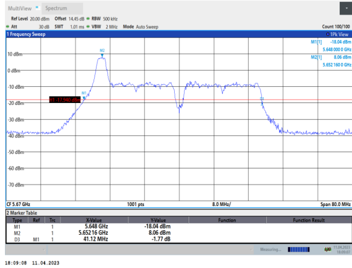
11AX40_Ant9_5670_52Tone_RU37
