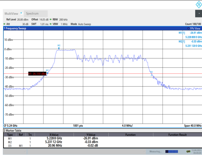
11AX20_Ant10_5240_52Tone_RU37
