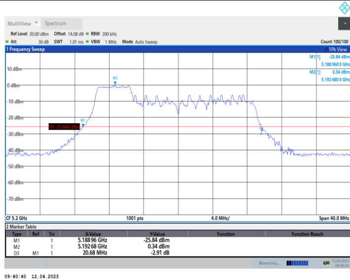
11AX20_Ant10_5200_106Tone_RU53
