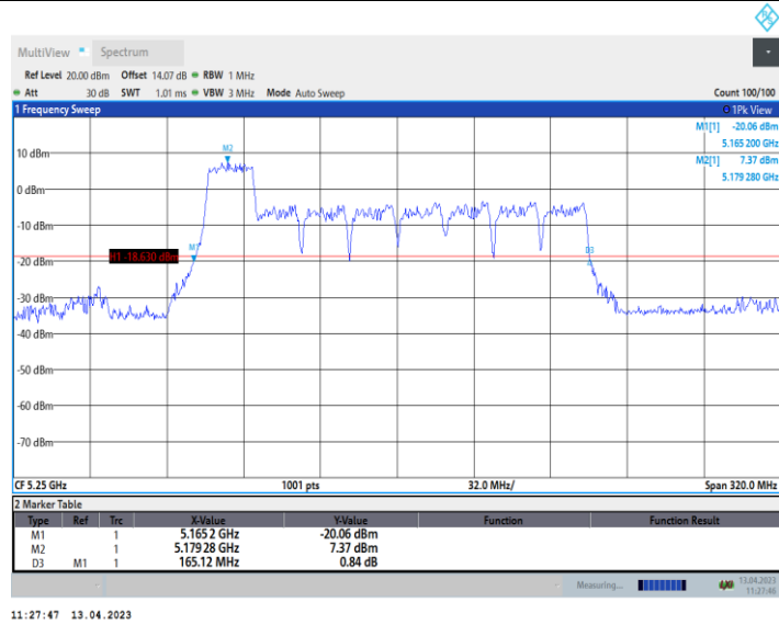
11AX160_Ant9_5250_484Tone_RU65
