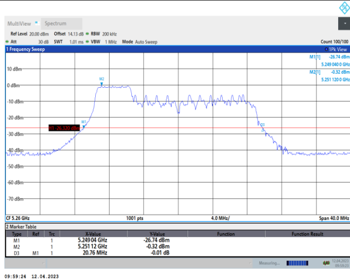
11AX20_Ant10_5260_106Tone_RU53
