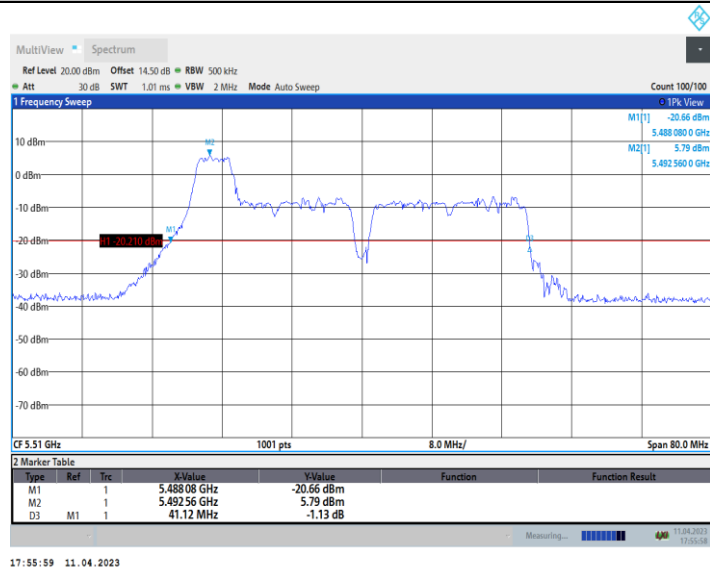
11AX40_Ant9_5510_106Tone_RU53
