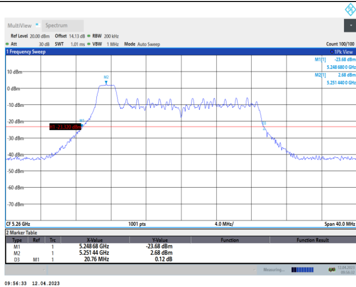
11AX20_Ant10_5260_52Tone_RU37
