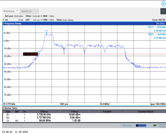
11AX80_Ant9_5775_242Tone_RU61
