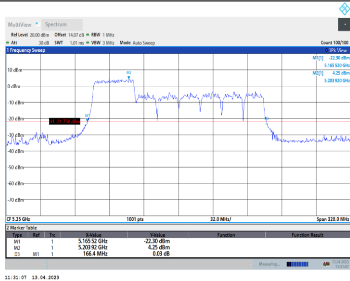
11AX160_Ant9_5250_996Tone_RU67
