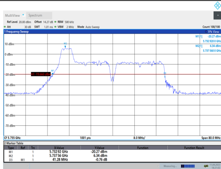
11AX40_Ant9_5755_106Tone_RU53
