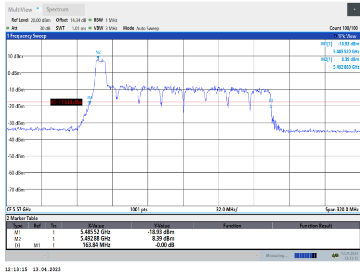
11AX160_Ant9_5570_242Tone_RU61
