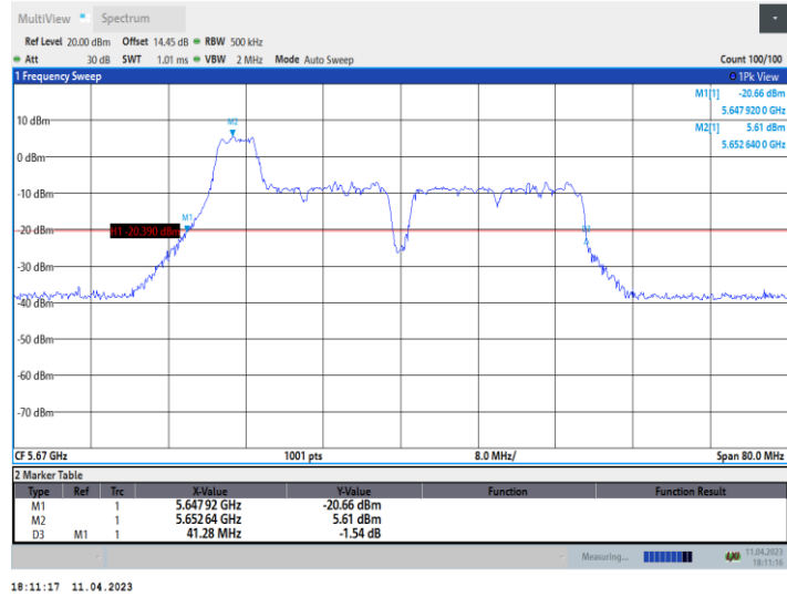
11AX40_Ant9_5670_106Tone_RU53
