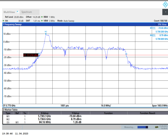
11AX80_Ant9_5775_106Tone_RU53
