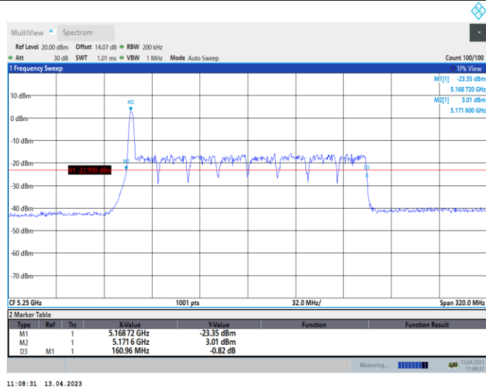
11AX160_Ant9_5250_52Tone_RU37
