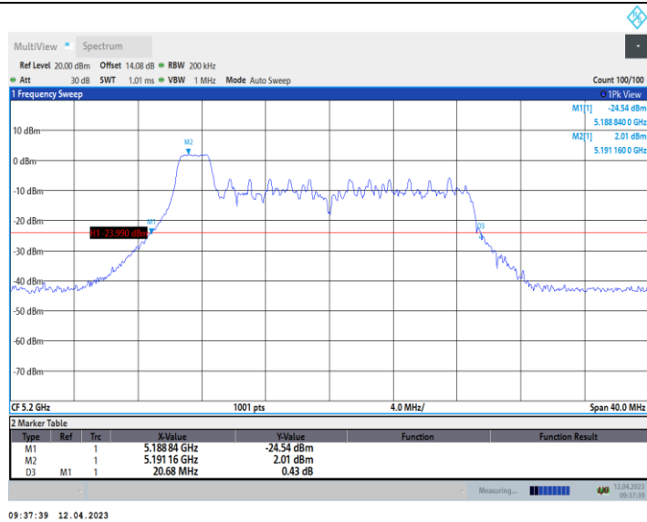
11AX20_Ant10_5200_52Tone_RU37
