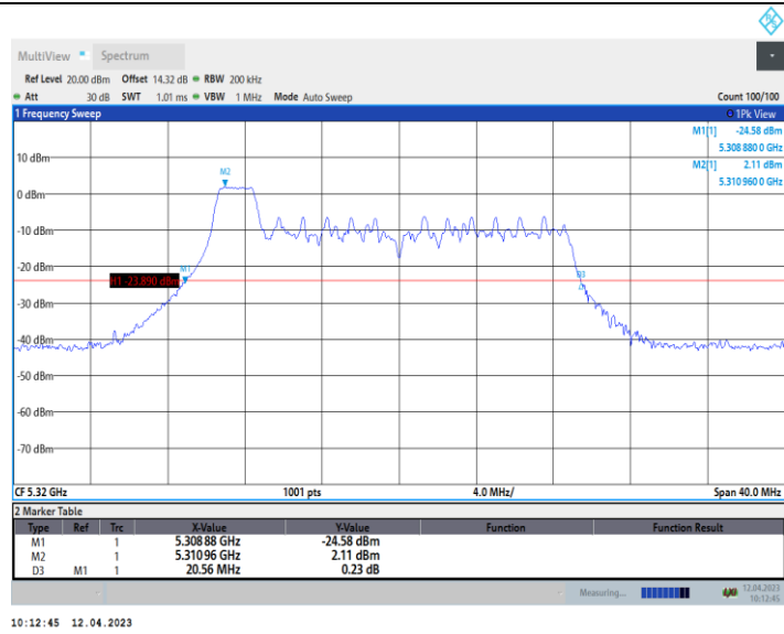
11AX20_Ant10_5320_52Tone_RU37
