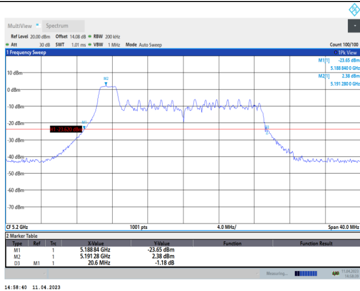
11AX20_Ant9_5200_52Tone_RU37
