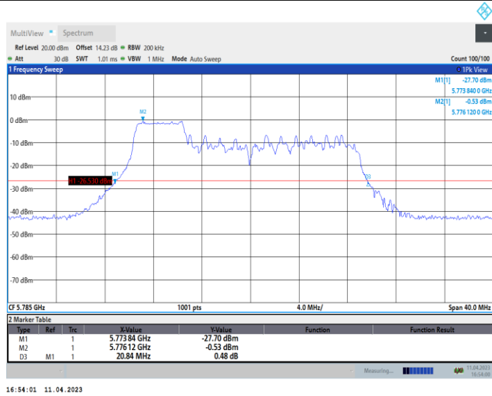
11AX20_Ant9_5785_106Tone_RU53
