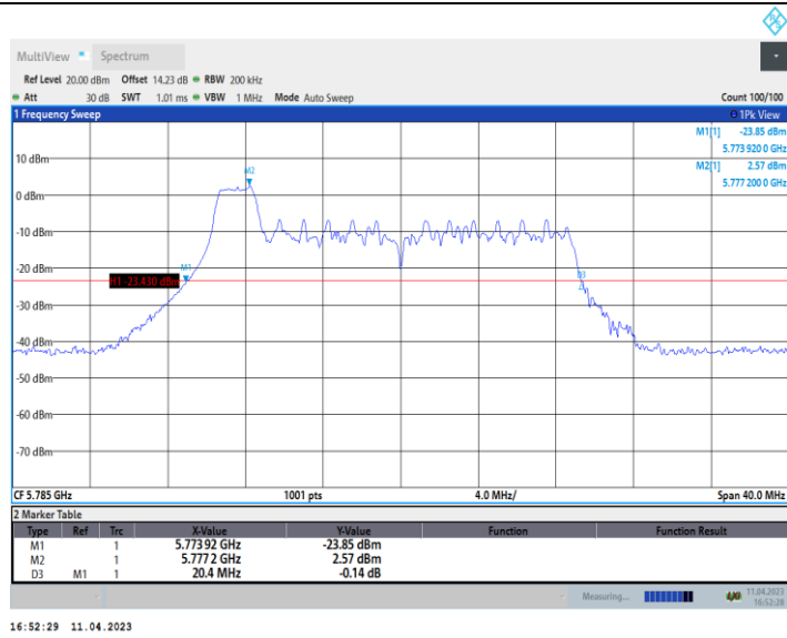
11AX20_Ant9_5785_52Tone_RU37
