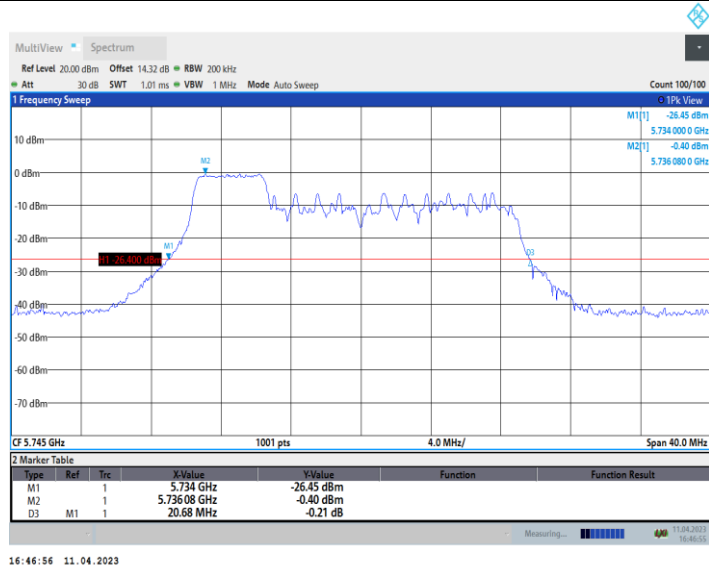
11AX20_Ant9_5745_106Tone_RU53
