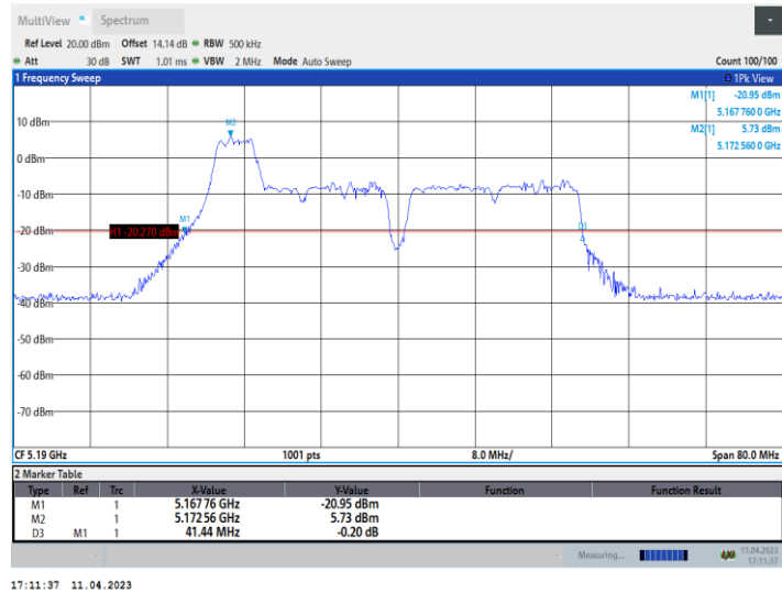
11AX40_Ant9_5190_106Tone_RU53
