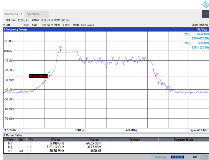
11AX20_Ant9_5200_52Tone_RU37
