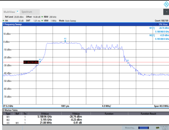
11AX20_Ant9_5200_106Tone_RU53
