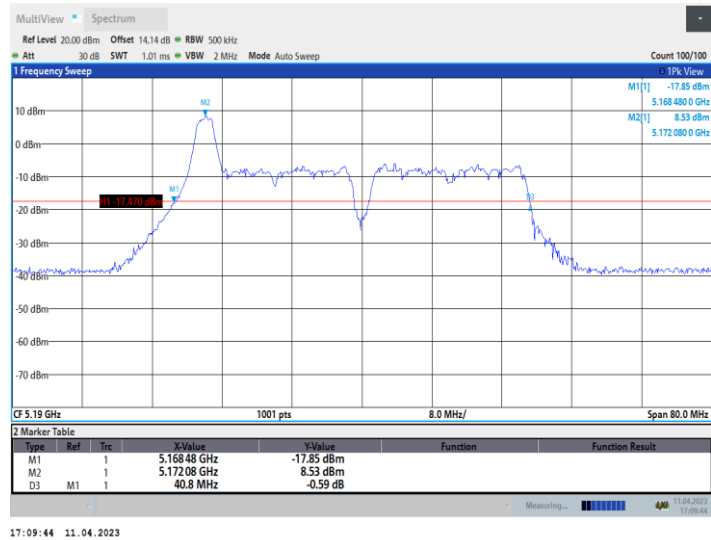
11AX40_Ant9_5190_52Tone_RU37
