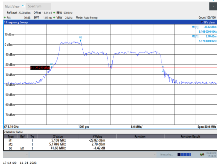
11AX40_Ant9_5190_242Tone_RU61
