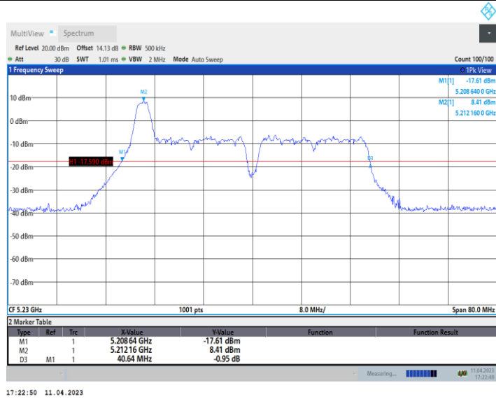
11AX40_Ant9_5230_52Tone_RU37
