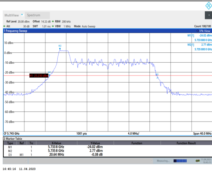
11AX20_Ant9_5745_52Tone_RU37
