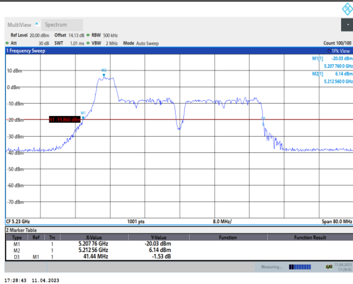
11AX40_Ant9_5230_106Tone_RU53
