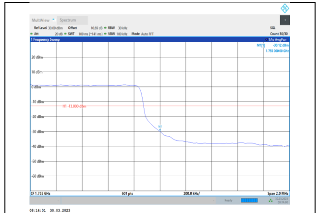
Band4-3MHz-QPSK-20385-15RB#0
