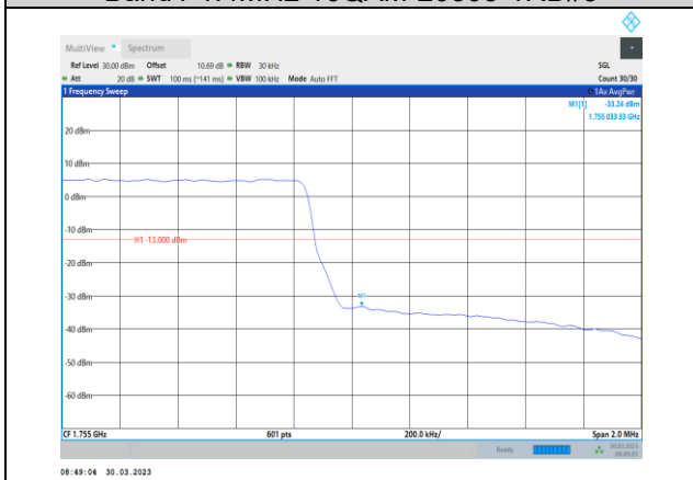
Band4-1.4MHz-16QAM-20393-6RB#0
