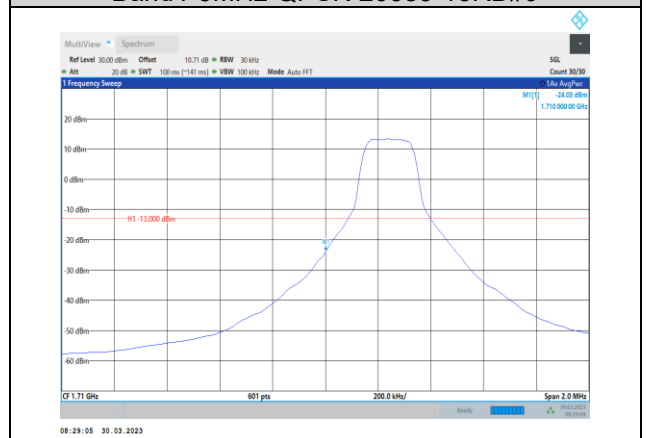
Band4-3MHz-16QAM-19965-1RB#0
