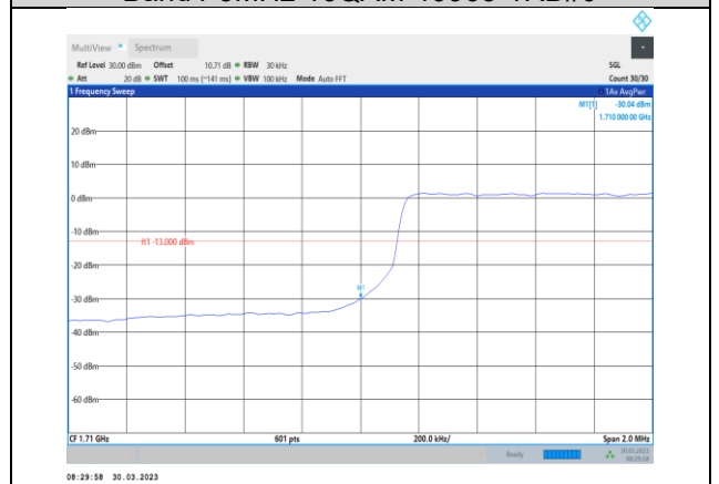
Band4-3MHz-16QAM-19965-15RB#0
