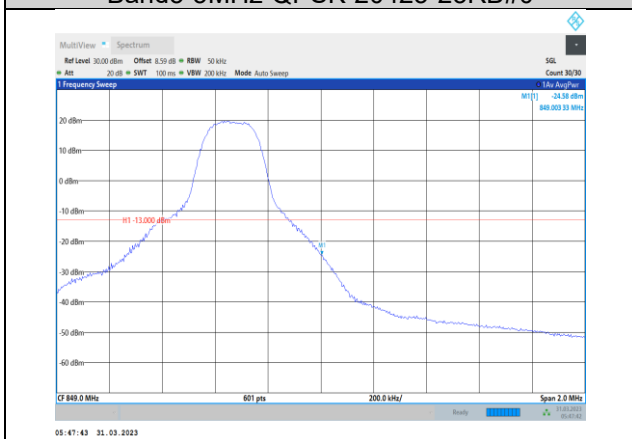
Band5-5MHz-QPSK-20625-1RB#24
