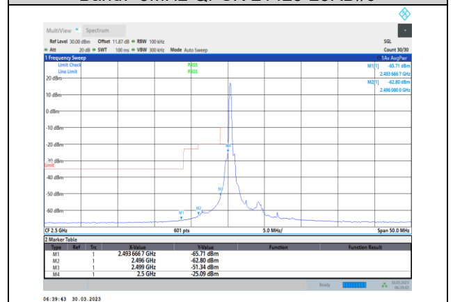
Band7-5MHz-16QAM-20775-1RB#0
