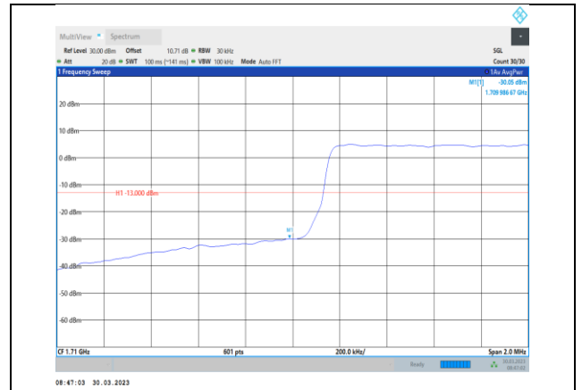
Band4-1.4MHz-64QAM-19957-6RB#0
