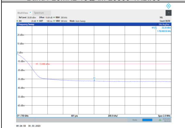
Band4-20MHz-16QAM-20300-100RB#0
