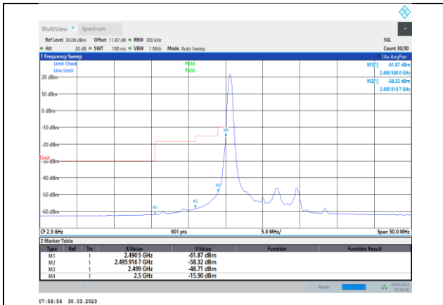
Band7-10MHz-QPSK-20800-1RB#0
