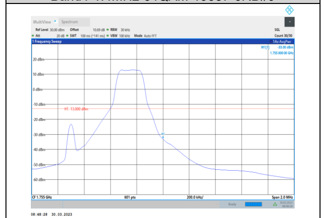
Band4-1.4MHz-64QAM-20393-1RB#5
