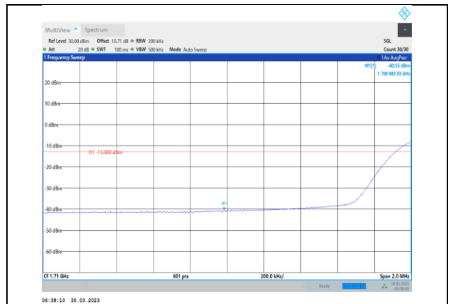
Band4-20MHz-64QAM-20050-100RB#0
