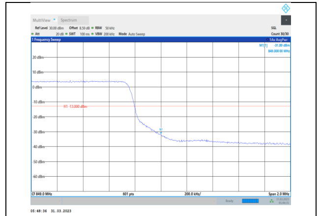
Band5-5MHz-QPSK-20625-25RB#0
