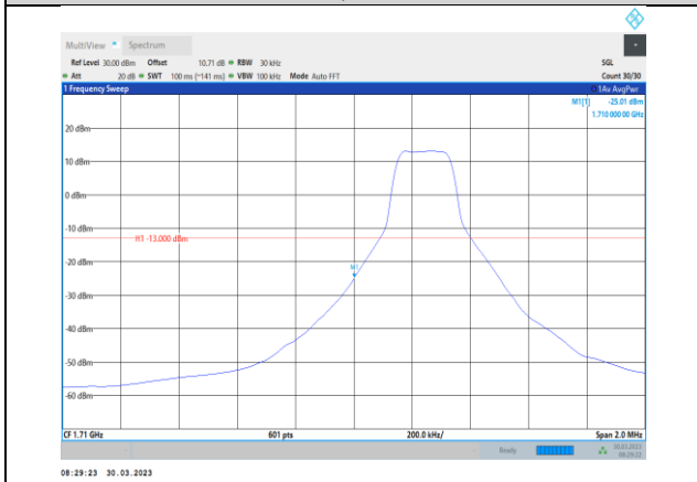
Band4-3MHz-64QAM-19965-1RB#0
