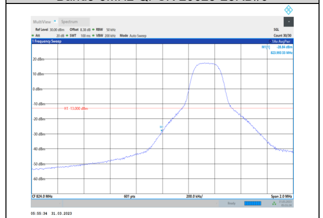
Band5-5MHz-16QAM-20425-1RB#0
