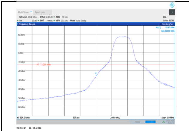
Band5-5MHz-QPSK-20425-1RB#0
