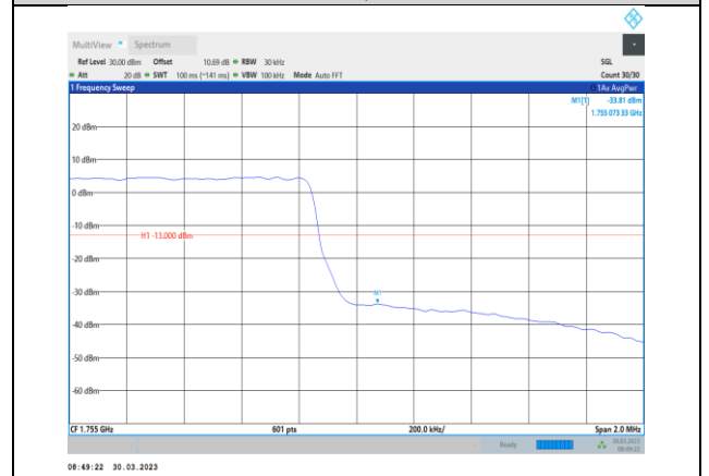
Band4-1.4MHz-64QAM-20393-6RB#0
