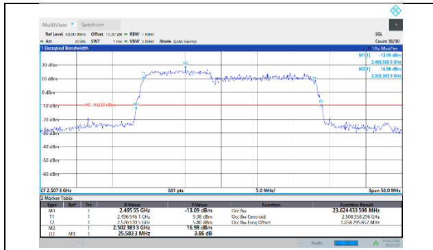
41-41-10MHz-15MHz-QPSK-QPSK-39703-39823-50RB#0-75RB#0
