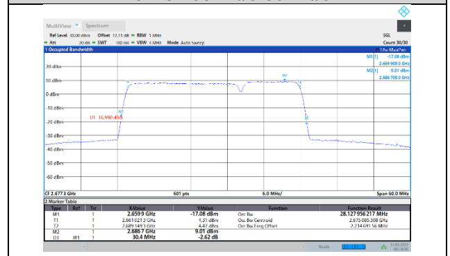
41-41-20MHz-10MHz-64QAM-64QAM-41391-41535-100RB#0-50RB#0
