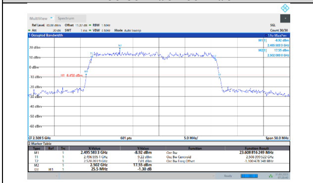
41-41-15MHz-10MHz-QPSK-QPSK-39725-39845-75RB#0-50RB#0
