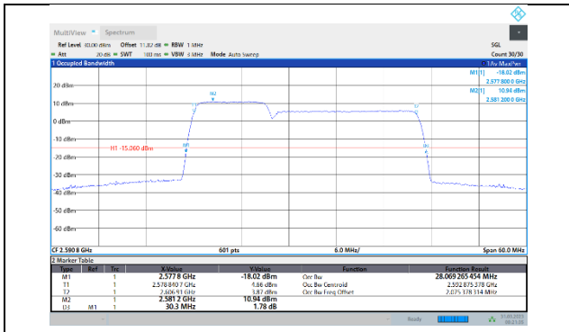
41-41-10MHz-20MHz-64QAM-64QAM-40526-40670-50RB#0-100RB#0
