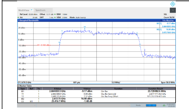
41-41-10MHz-15MHz-QPSK-QPSK-41395-41515-50RB#0-75RB#0
