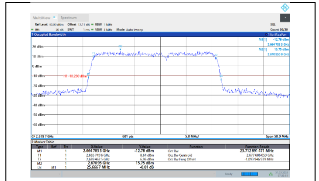
41-41-15MHz-10MHz-QPSK-QPSK-41417-41537-75RB#0-50RB#0
