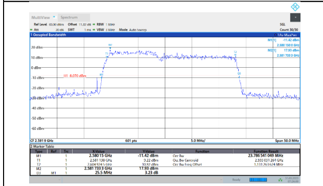
41-41-10MHz-15MHz-QPSK-QPSK-40549-40669-50RB#0-75RB#0
