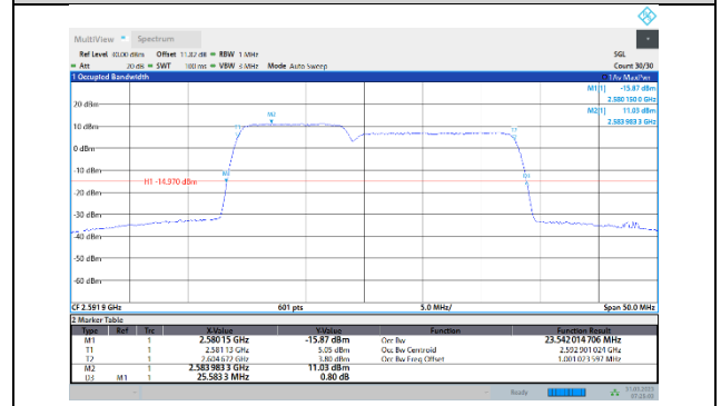
41-41-10MHz-15MHz-64QAM-64QAM-40549-40669-50RB#0-75RB#0
