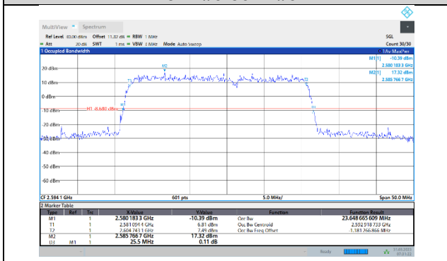
41-41-15MHz-10MHz-QPSK-QPSK-40571-40691-75RB#0-50RB#0
