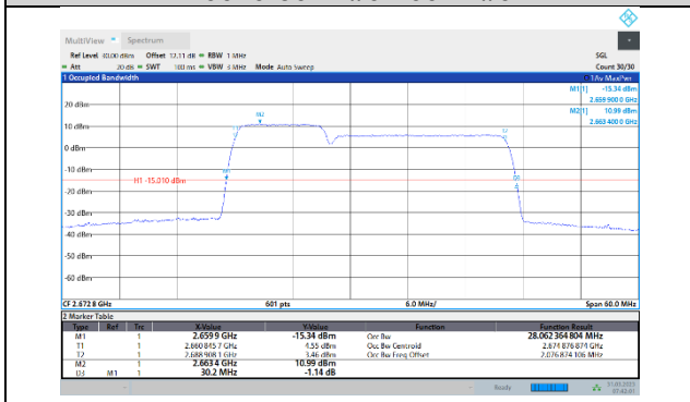
41-41-10MHz-20MHz-64QAM-64QAM-41346-41490-50RB#0-100RB#0
