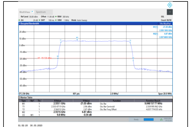
Band41-10MHz-64QAM-40290-50RB#0
