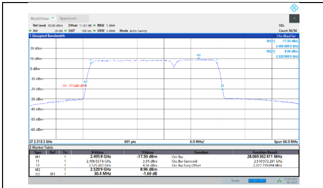
41-41-20MHz-10MHz-16QAM-16QAM-39750-39894-100RB#0-50RB#0
