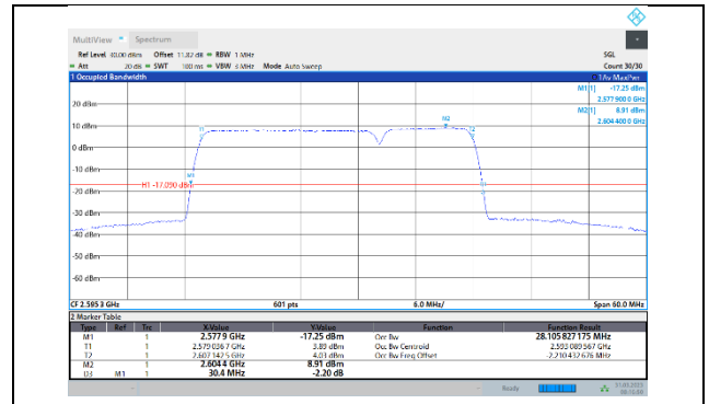
41-41-20MHz-10MHz-64QAM-64QAM-40571-40715-100RB#0-50RB#0
