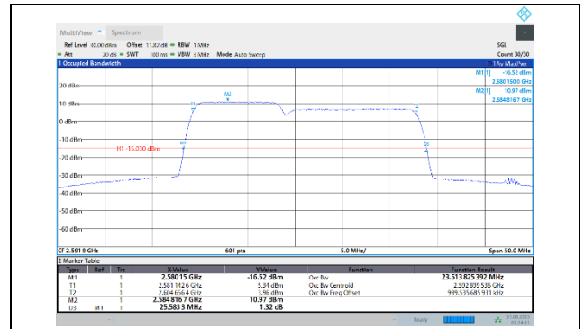
41-41-10MHz-15MHz-16QAM-16QAM-40549-40669-50RB#0-75RB#0
