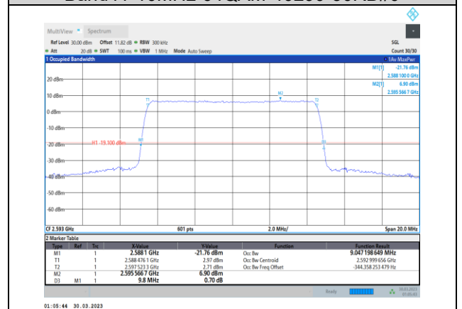
Band41-10MHz-64QAM-40620-50RB#0
