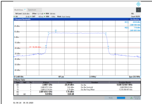
Band41-10MHz-16QAM-41540-50RB#0
