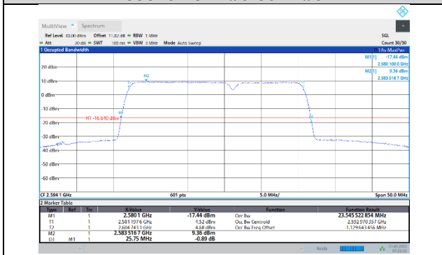
41-41-15MHz-10MHz-64QAM-64QAM-40571-40691-75RB#0-50RB#0
