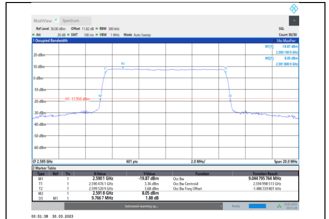
Band41-10MHz-16QAM-40640-50RB#0
