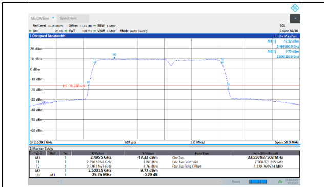
41-41-15MHz-10MHz-64QAM-64QAM-39725-39845-75RB#0-50RB#0
