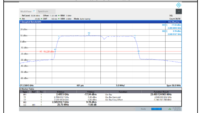
41-41-15MHz-10MHz-16QAM-16QAM-39725-39845-75RB#0-50RB#0
