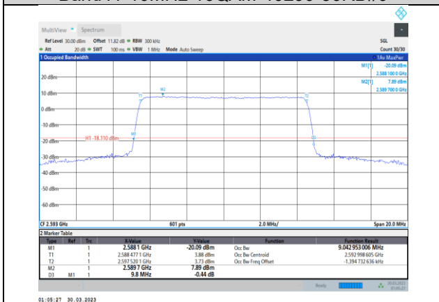
Band41-10MHz-16QAM-40620-50RB#0
