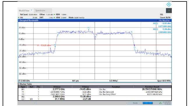
41-41-15MHz-15MHz-QPSK-QPSK-40545-40695-75RB#0-75RB#0
