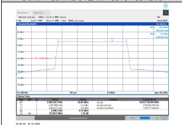
Band41-20MHz-64QAM-40620-100RB#0
