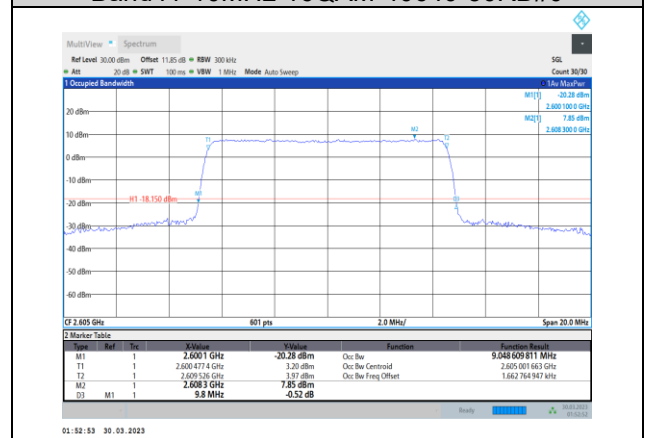
Band41-10MHz-16QAM-40740-50RB#0
