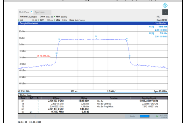
Band41-10MHz-16QAM-39700-50RB#0
