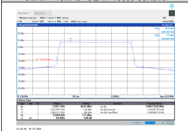
Band41-10MHz-16QAM-40290-50RB#0
