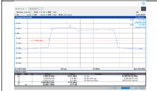
41-41-10MHz-15MHz-16QAM-16QAM-39703-39823-50RB#0-75RB#0
