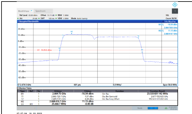
41-41-10MHz-15MHz-64QAM-64QAM-41395-41515-50RB#0-75RB#0
