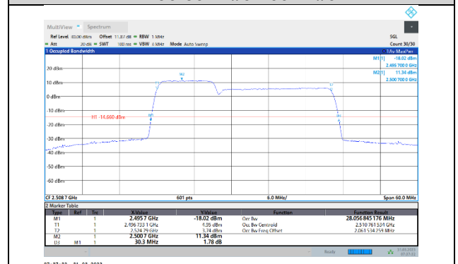
41-41-10MHz-20MHz-64QAM-64QAM-39705-39849-50RB#0-100RB#0
