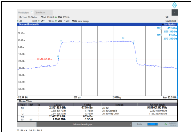
Band41-10MHz-16QAM-40090-50RB#0
