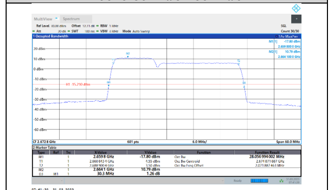
41-41-10MHz-20MHz-16QAM-16QAM-41346-41490-50RB#0-100RB#0
