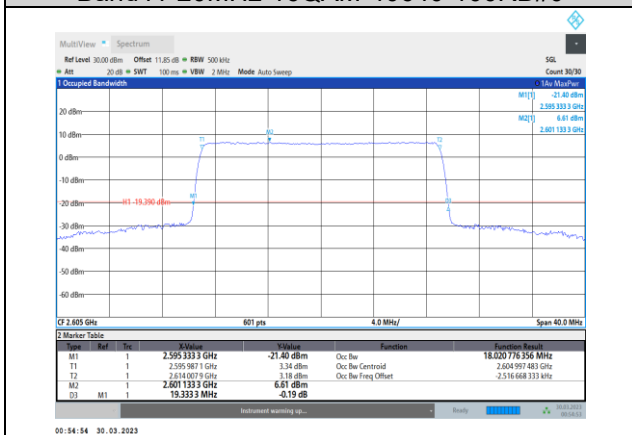
Band41-20MHz-16QAM-40740-100RB#0
