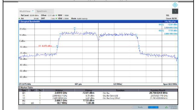
41-41-15MHz-15MHz-QPSK-QPSK-41365-41515-75RB#0-75RB#0
