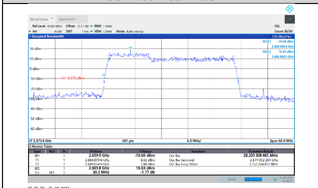
41-41-10MHz-20MHz-QPSK-QPSK-41346-41490-50RB#0-100RB#0
