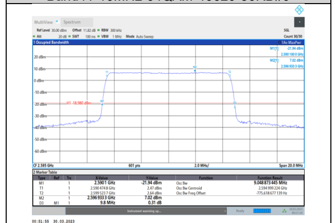
Band41-10MHz-64QAM-40640-50RB#0
