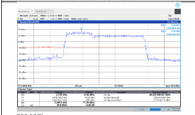
41-41-10MHz-20MHz-QPSK-QPSK-40526-40670-50RB#0-100RB#0
