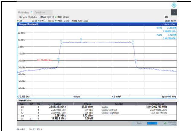
Band41-20MHz-16QAM-40640-100RB#0
