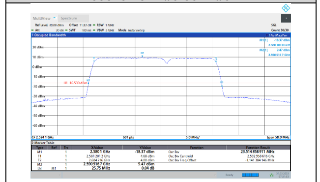
41-41-15MHz-10MHz-16QAM-16QAM-40571-40691-75RB#0-50RB#0
