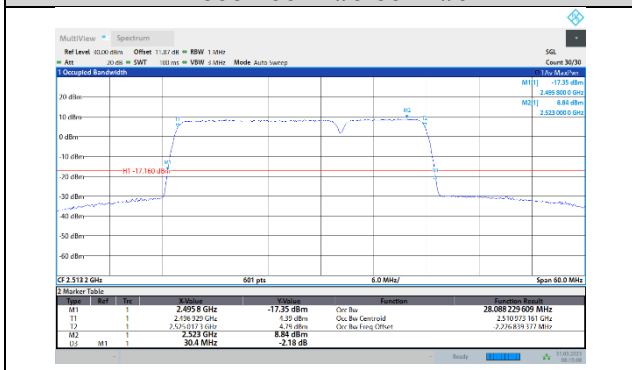
41-41-20MHz-10MHz-64QAM-64QAM-39750-39894-100RB#0-50RB#0
