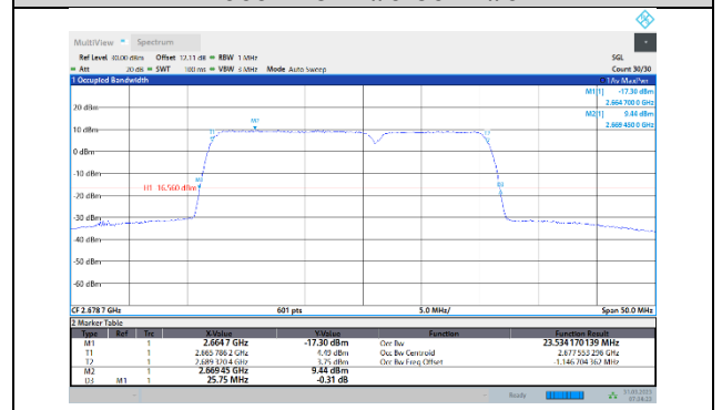
41-41-15MHz-10MHz-16QAM-16QAM-41417-41537-75RB#0-50RB#0
