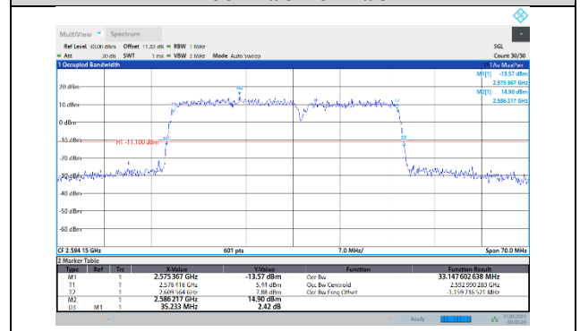
41-41-20MHz-15MHz-QPSK-QPSK-40546-40717-100RB#0-75RB#0
