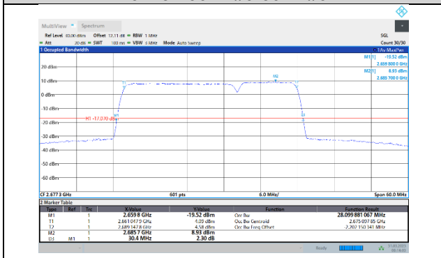
41-41-20MHz-10MHz-16QAM-16QAM-41391-41535-100RB#0-50RB#0
