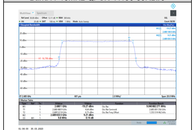
Band41-10MHz-QPSK-41540-50RB#0
