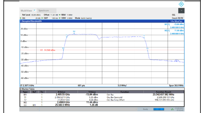
41-41-10MHz-15MHz-64QAM-64QAM-39703-39823-50RB#0-75RB#0
