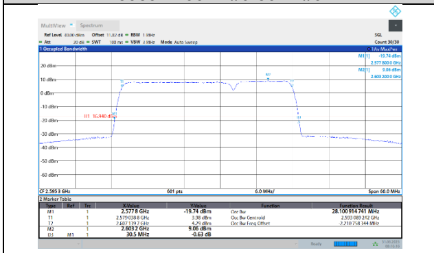
41-41-20MHz-10MHz-16QAM-16QAM-40571-40715-100RB#0-50RB#0
