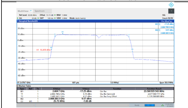
41-41-15MHz-10MHz-64QAM-64QAM-41417-41537-75RB#0-50RB#0
