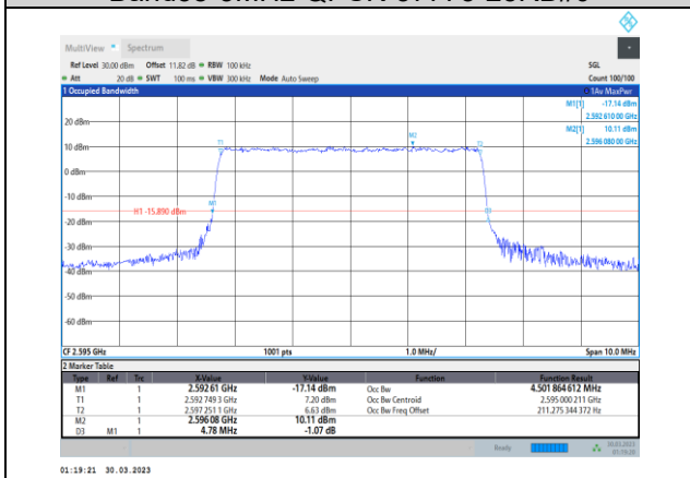
Band38-5MHz-QPSK-38000-25RB#0
