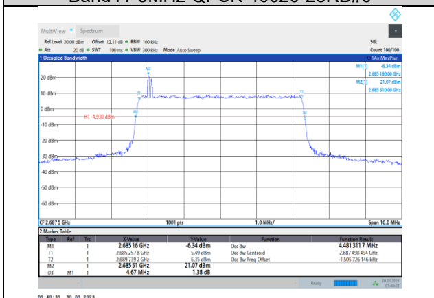
Band41-5MHz-QPSK-41565-25RB#0
