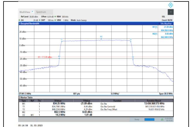
Band26-15MHz-QPSK-26965-75RB#0
