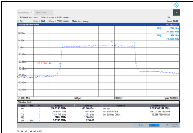
Band17-10MHz-16QAM-23780-50RB#0
