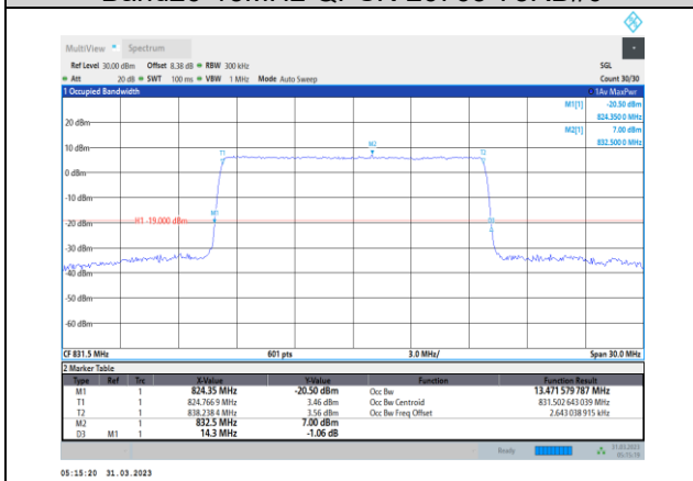
Band26-15MHz-QPSK-26865-75RB#0
