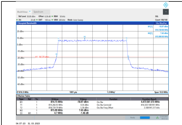
Band26-5MHz-64QAM-26715-25RB#0
