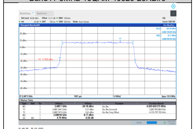
Band41-5MHz-16QAM-41565-25RB#0
