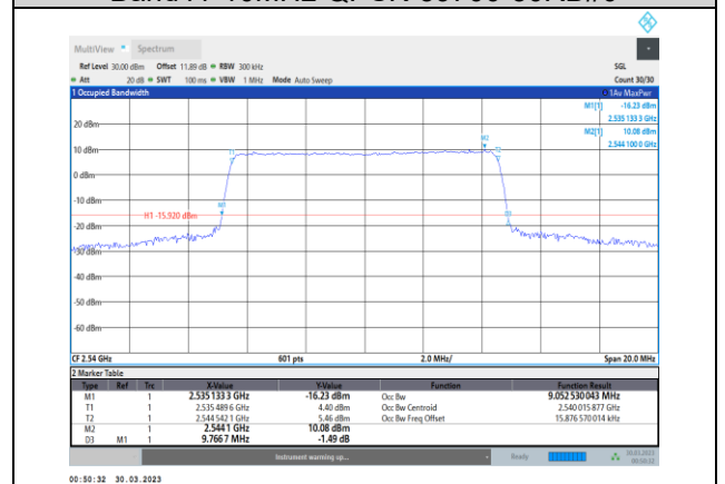
Band41-10MHz-QPSK-40090-50RB#0
