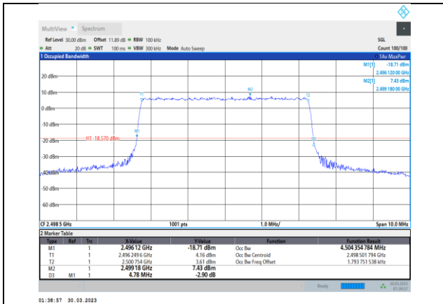
Band41-5MHz-64QAM-39675-25RB#0
