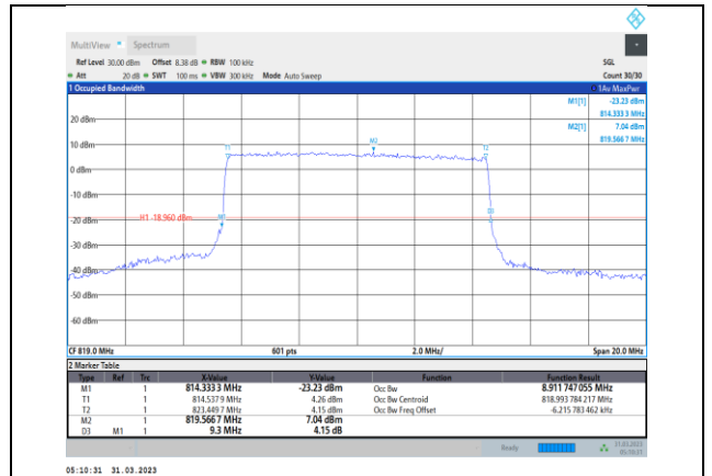
Band26-10MHz-QPSK-26740-50RB#0
