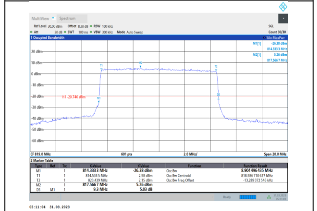
Band26-10MHz-64QAM-26740-50RB#0
