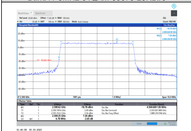
Band41-5MHz-64QAM-40620-25RB#0
