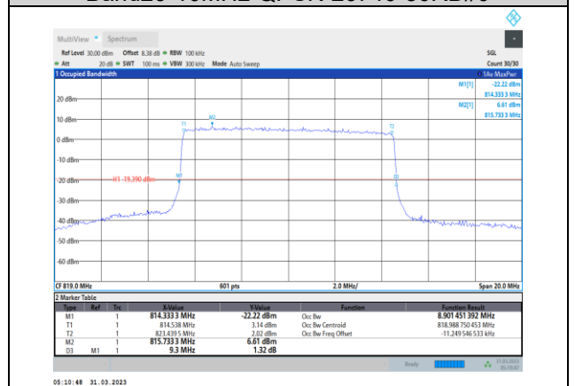
Band26-10MHz-16QAM-26740-50RB#0
