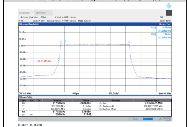
Band26-3MHz-64QAM-26740-15RB#0
