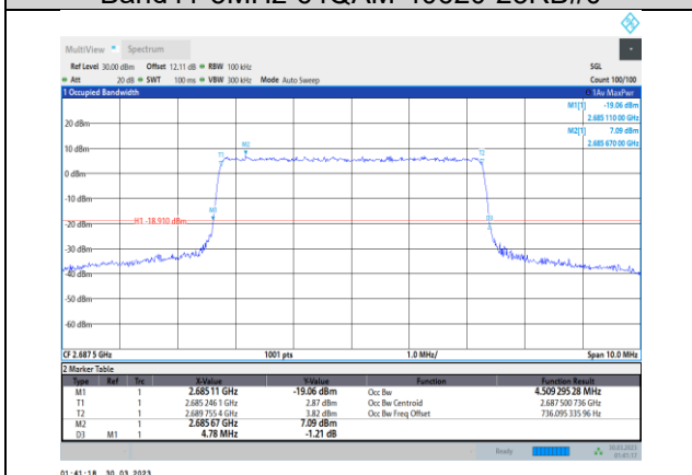
Band41-5MHz-64QAM-41565-25RB#0
