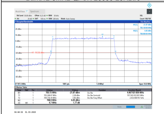
Band12-5MHz-QPSK-23095-25RB#0
