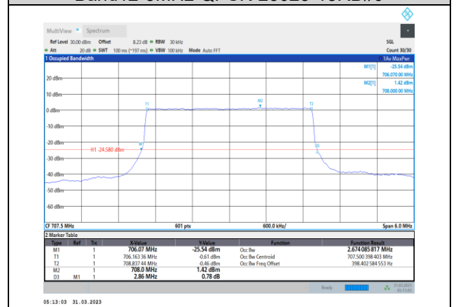
Band12-3MHz-QPSK-23095-15RB#0
