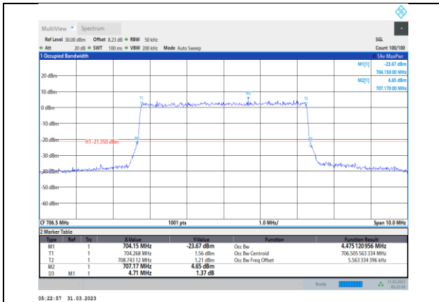
Band17-5MHz-64QAM-23755-25RB#0
