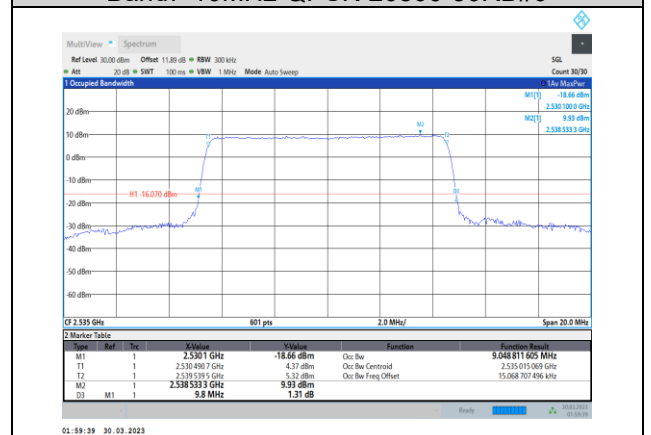
Band7-10MHz-QPSK-2100-50RB#0
