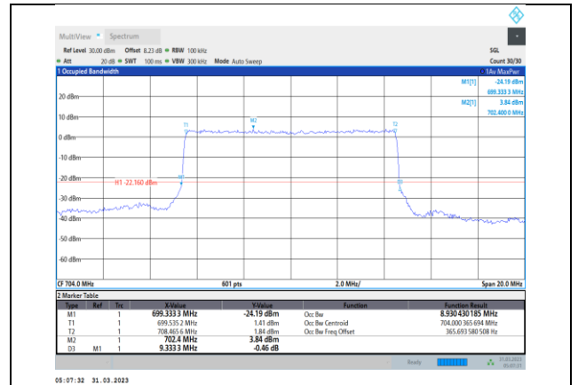
Band12-10MHz-QPSK-23060-50RB#0
