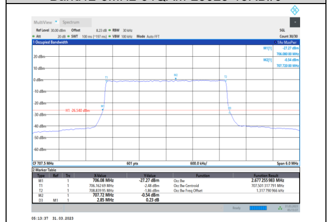
Band12-3MHz-64QAM-23095-15RB#0
