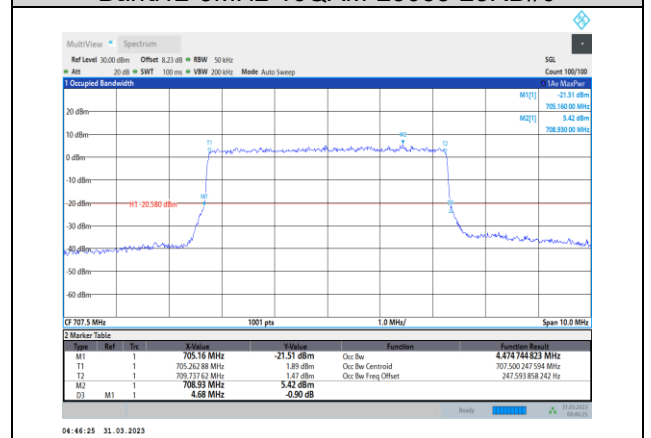
Band12-5MHz-16QAM-23095-25RB#0
