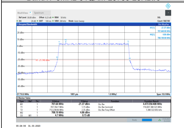
Band17-5MHz-64QAM-23790-25RB#0
