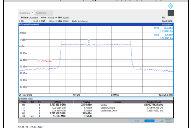
Band4-10MHz-64QAM-20175-50RB#0
