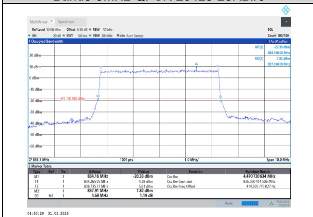
Band5-5MHz-QPSK-20525-25RB#0
