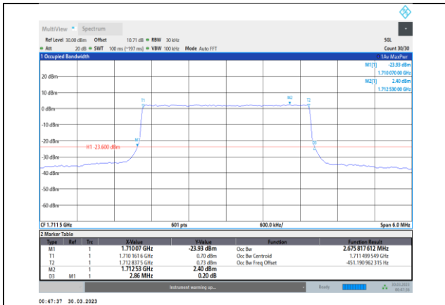
Band4-3MHz-16QAM-19965-15RB#0
