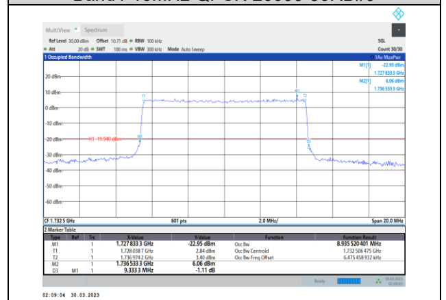
Band4-10MHz-QPSK-20175-50RB#0
