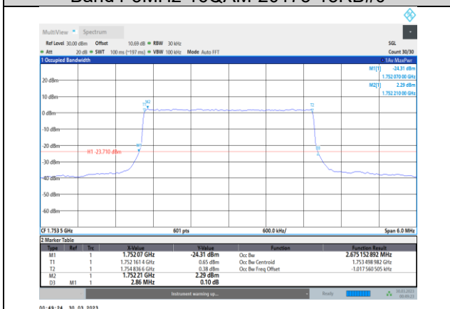
Band4-3MHz-16QAM-20385-15RB#0
