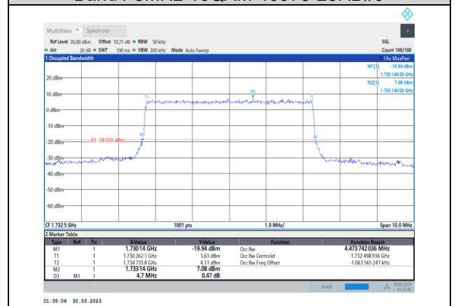
Band4-5MHz-16QAM-20175-25RB#0
