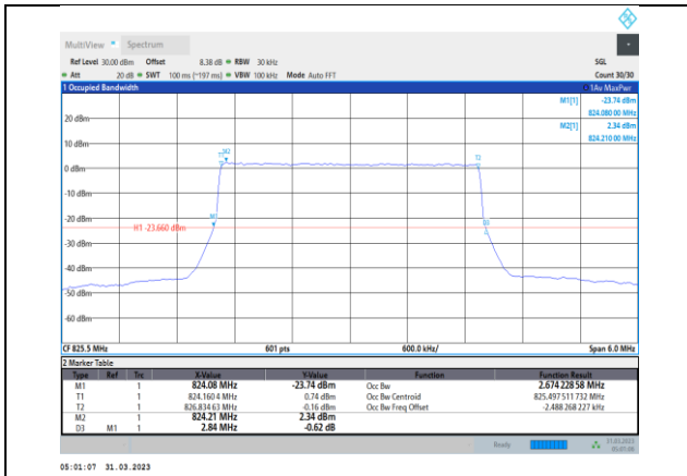
Band5-3MHz-16QAM-20415-15RB#0
