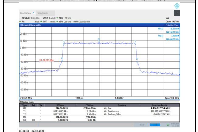
Band5-5MHz-16QAM-20625-25RB#0
