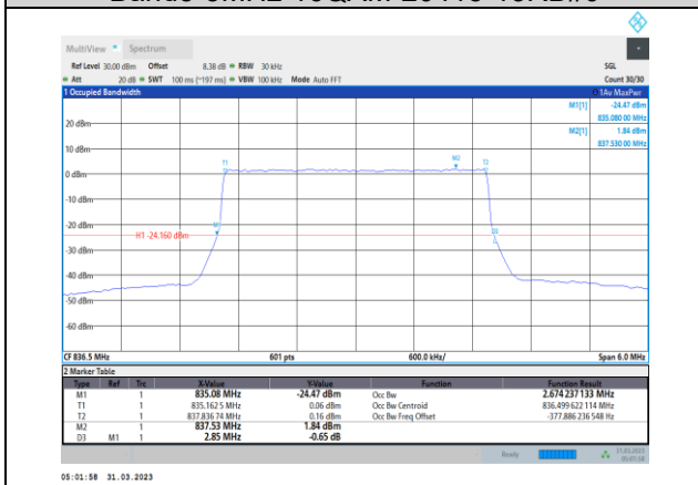
Band5-3MHz-16QAM-20525-15RB#0
