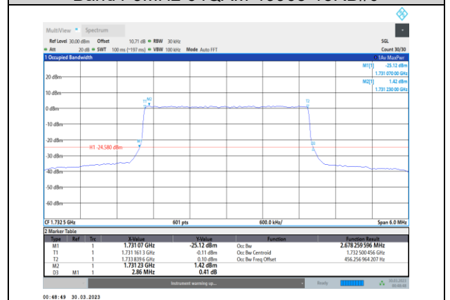
Band4-3MHz-64QAM-20175-15RB#0
