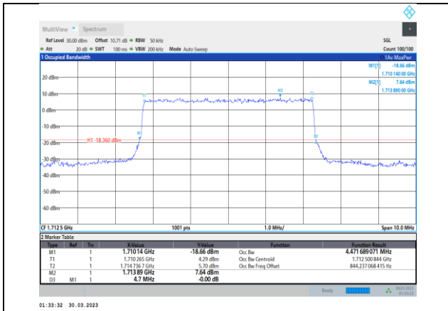
Band4-5MHz-QPSK-19975-25RB#0
