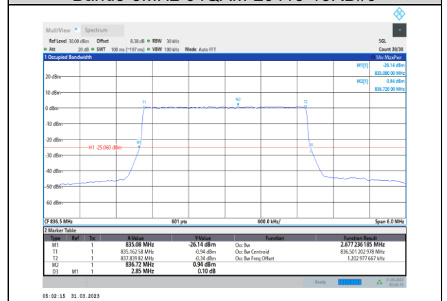
Band5-3MHz-64QAM-20525-15RB#0
