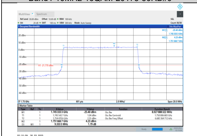
Band4-10MHz-16QAM-20350-50RB#0
