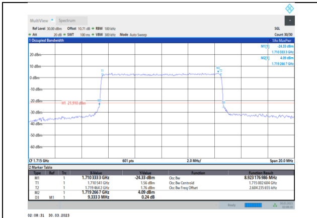
Band4-10MHz-16QAM-20000-50RB#0
