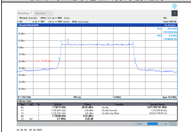
Band4-5MHz-64QAM-20175-25RB#0
