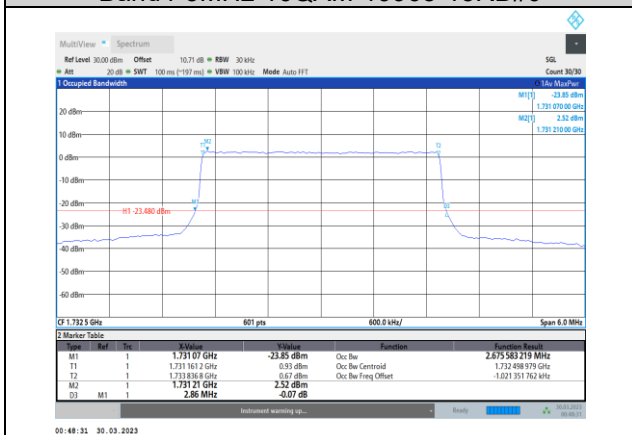
Band4-3MHz-16QAM-20175-15RB#0
