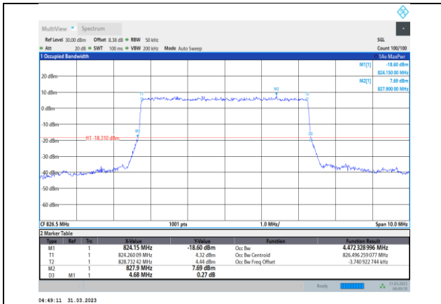
Band5-5MHz-QPSK-20425-25RB#0
