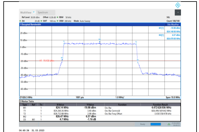
Band5-5MHz-16QAM-20425-25RB#0
