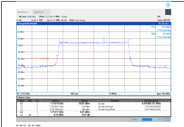
Band4-5MHz-64QAM-19975-25RB#0
