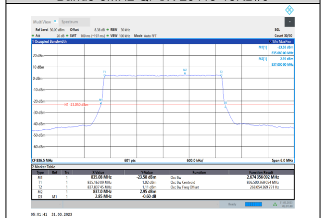
Band5-3MHz-QPSK-20525-15RB#0
