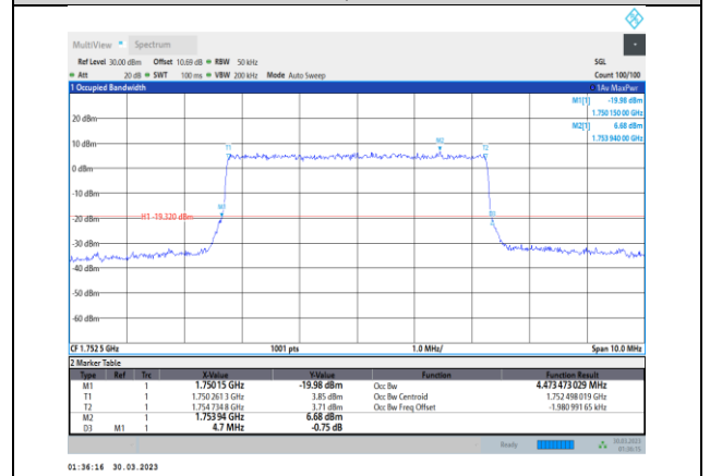
Band4-5MHz-16QAM-20375-25RB#0
