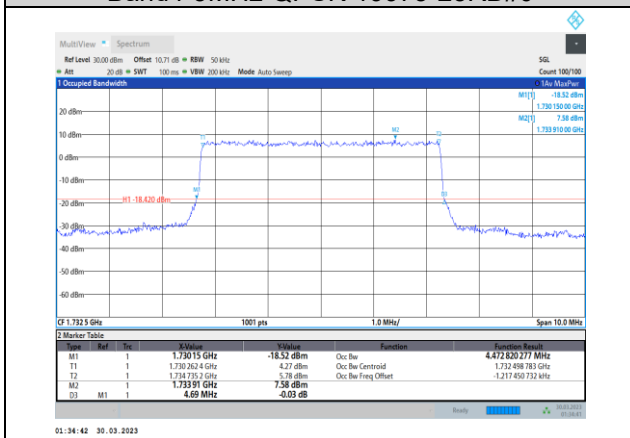
Band4-5MHz-QPSK-20175-25RB#0
