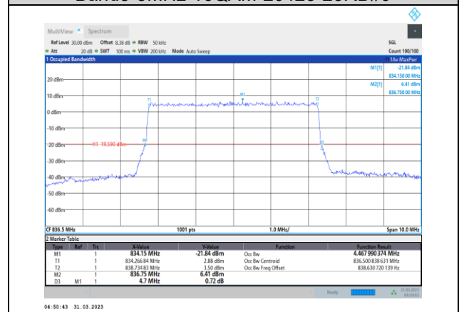
Band5-5MHz-16QAM-20525-25RB#0
