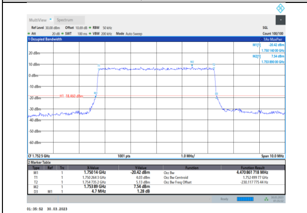
Band4-5MHz-QPSK-20375-25RB#0
