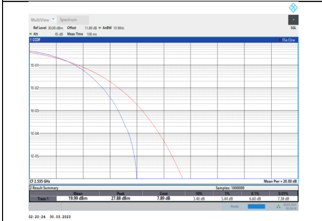
Band7-20MHz-16QAM-21100-100RB#0
