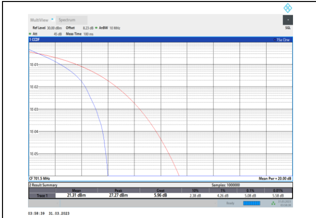
Band12-5MHz-QPSK-23035-25RB#0
