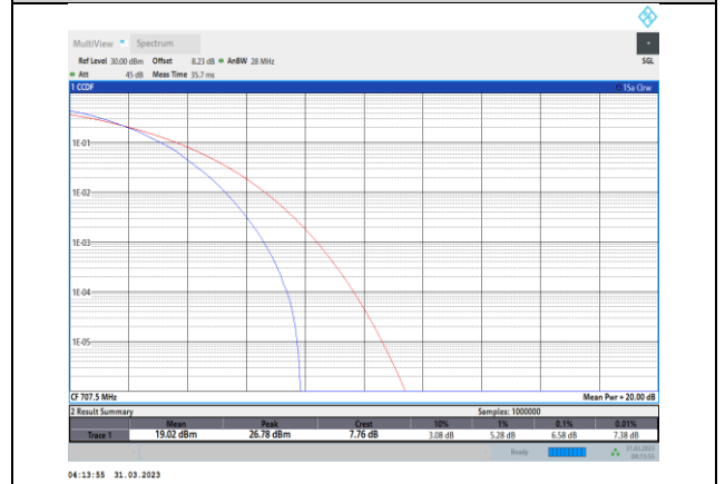
Band12-3MHz-64QAM-23095-15RB#0
