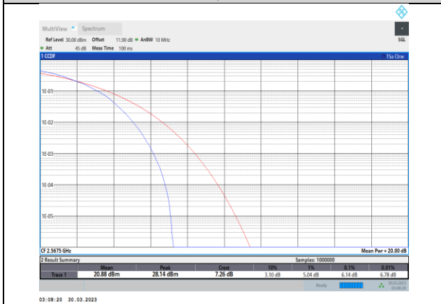
Band7-5MHz-64QAM-21425-25RB#0
