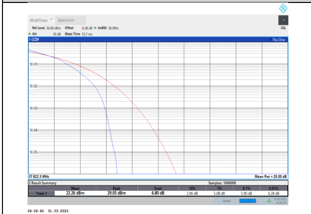
Band26-3MHz-16QAM-26775-15RB#0
