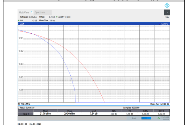
Band12-5MHz-16QAM-23155-25RB#0
