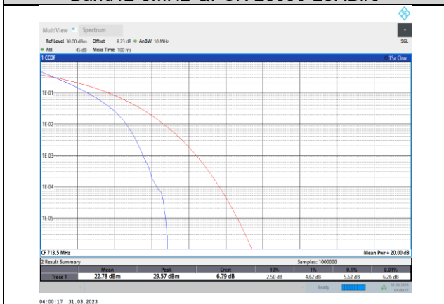
Band12-5MHz-QPSK-23155-25RB#0
