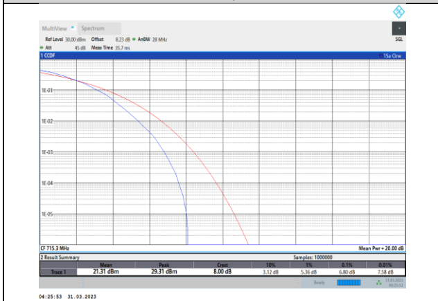
Band12-1.4MHz-64QAM-23173-6RB#0
