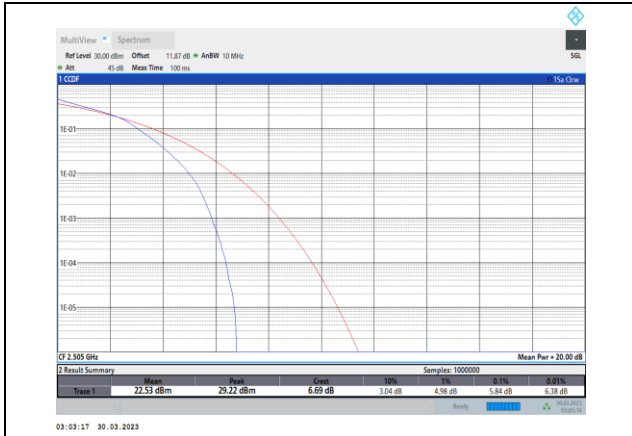
Band7-10MHz-16QAM-20800-50RB#0
