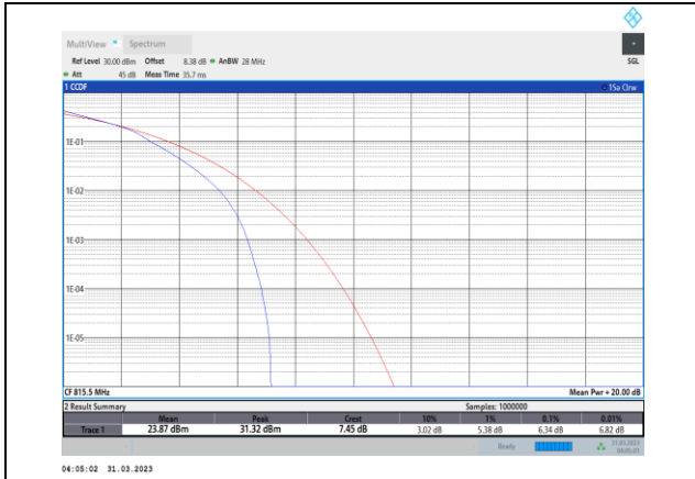
Band26-3MHz-16QAM-26705-15RB#0
