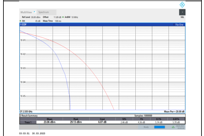
Band7-10MHz-QPSK-21100-50RB#0
