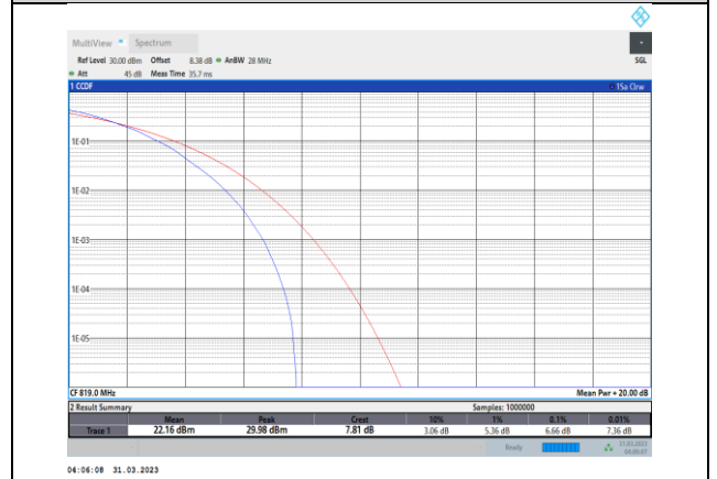
Band26-3MHz-64QAM-26740-15RB#0
