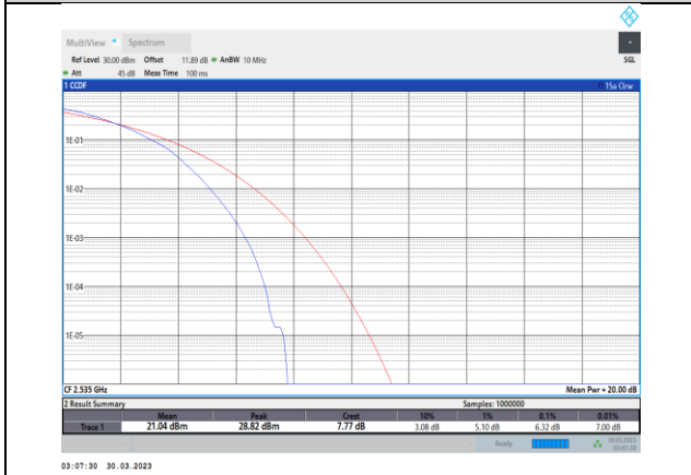
Band7-5MHz-64QAM-21100-25RB#0
