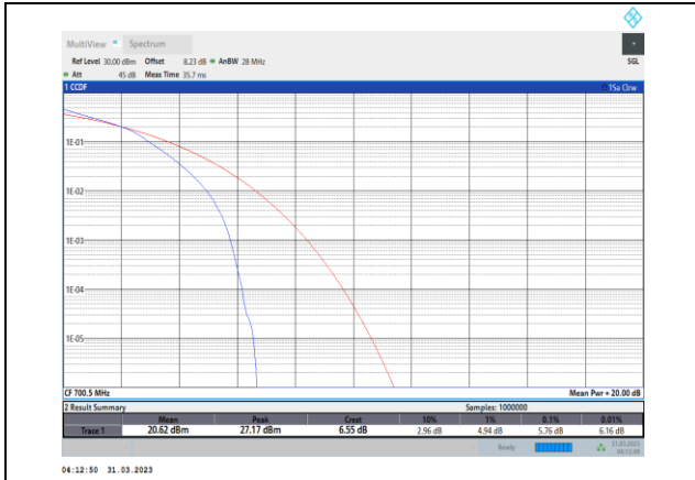
Band12-3MHz-16QAM-23025-15RB#0
