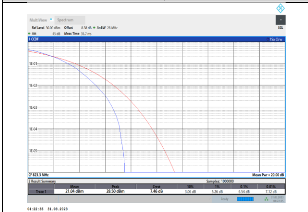
Band26-1.4MHz-64QAM-26783-6RB#0
