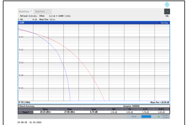
Band12-5MHz-16QAM-23035-25RB#0
