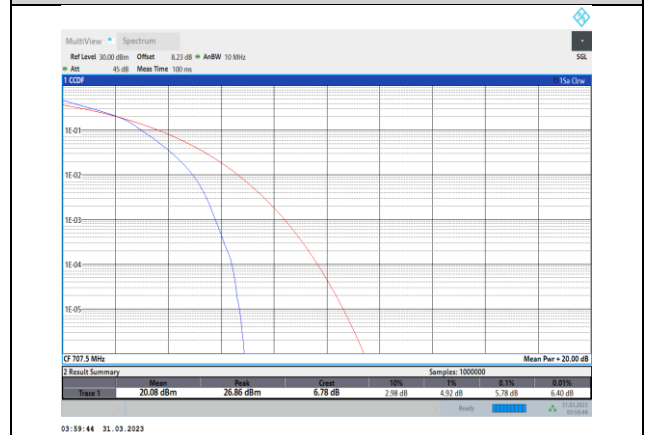
Band12-5MHz-16QAM-23095-25RB#0
