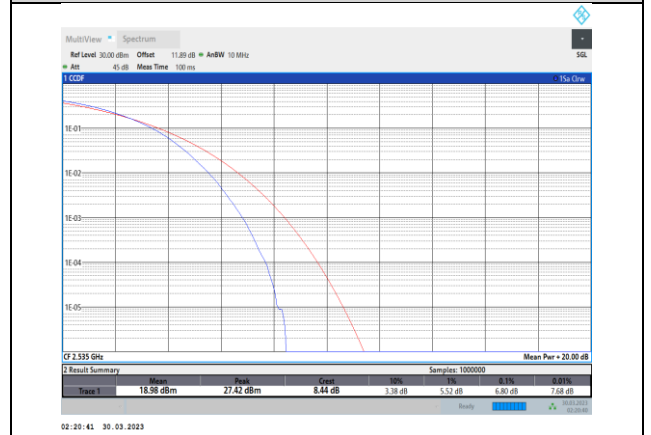
Band7-20MHz-64QAM-21100-100RB#0
