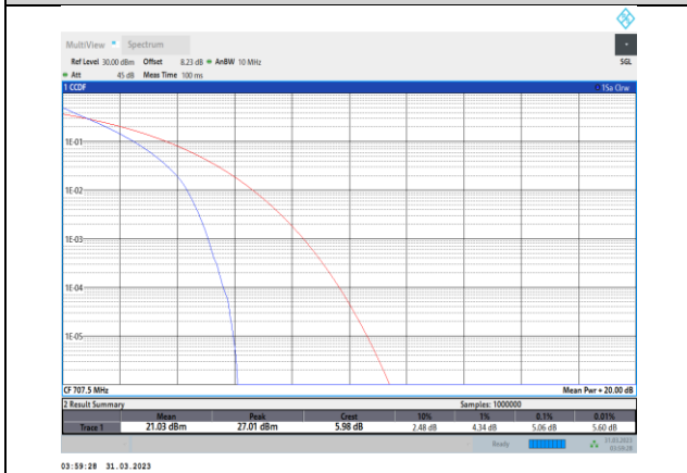
Band12-5MHz-QPSK-23095-25RB#0
