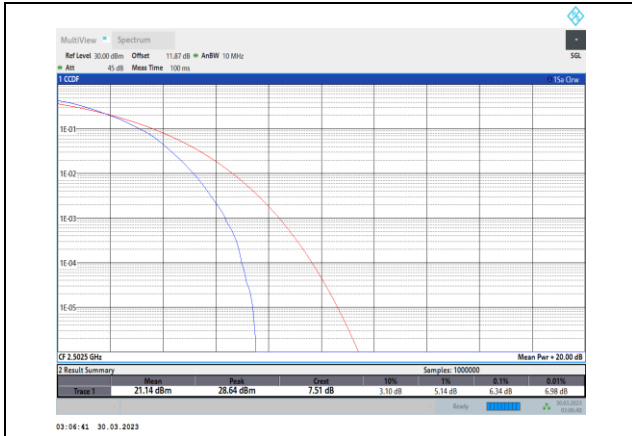
Band7-5MHz-64QAM-20775-25RB#0
