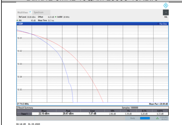
Band12-3MHz-16QAM-23165-15RB#0
