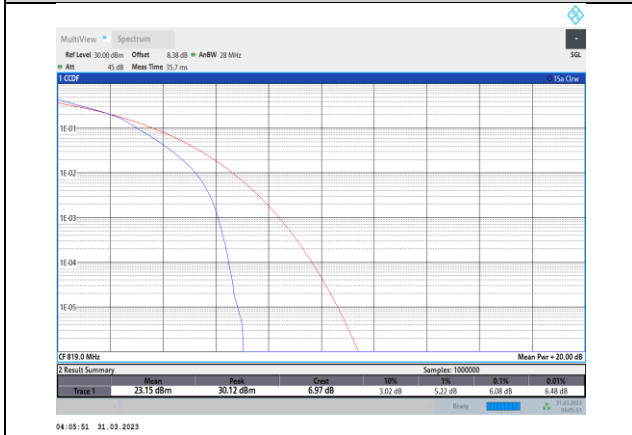
Band26-3MHz-16QAM-26740-15RB#0
