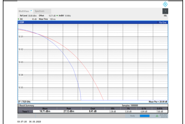
Band4-20MHz-64QAM-20175-100RB#0
