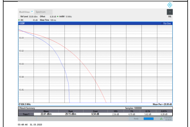
Band5-10MHz-QPSK-20525-50RB#0
