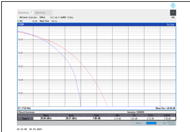
Band4-5MHz-64QAM-19975-25RB#0
