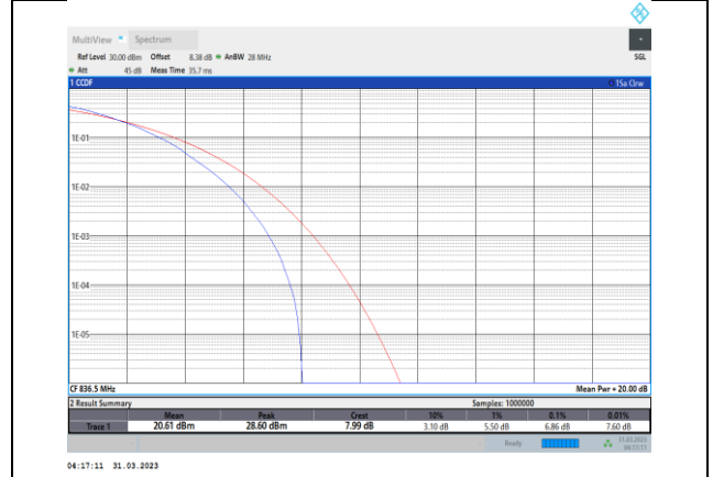
Band5-3MHz-64QAM-20525-15RB#0
