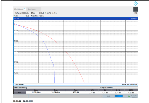
Band5-5MHz-QPSK-20525-25RB#0
