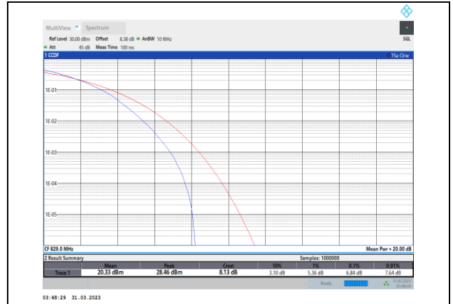
Band5-10MHz-64QAM-20450-50RB#0
