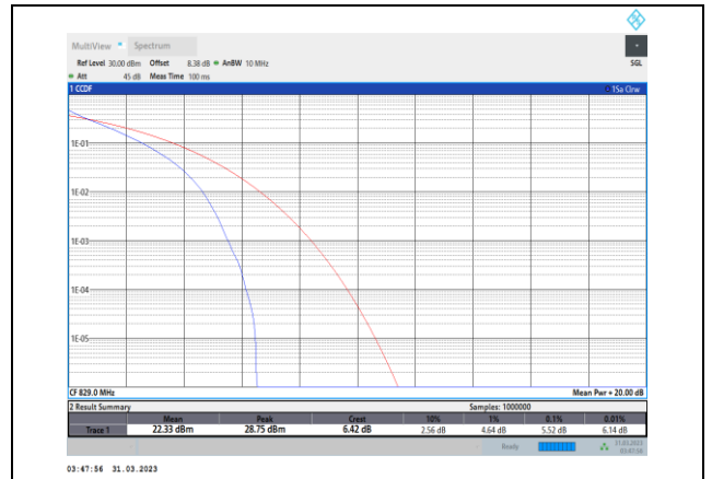
Band5-10MHz-QPSK-20450-50RB#0
