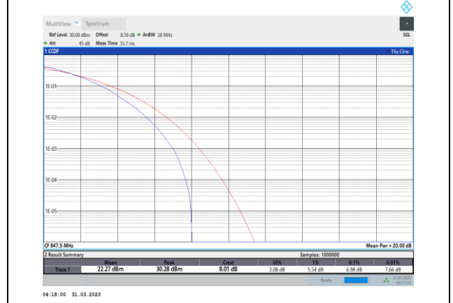
Band5-3MHz-64QAM-20635-15RB#0
