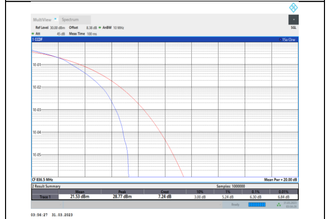
Band5-5MHz-16QAM-20525-25RB#0
