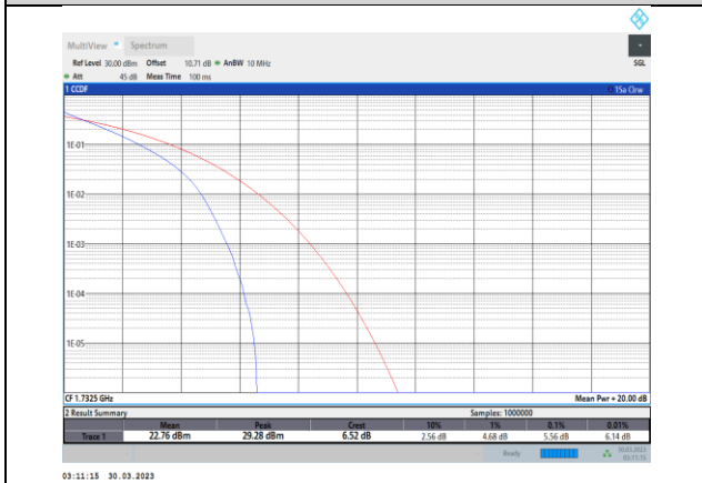
Band4-5MHz-QPSK-20175-25RB#0
