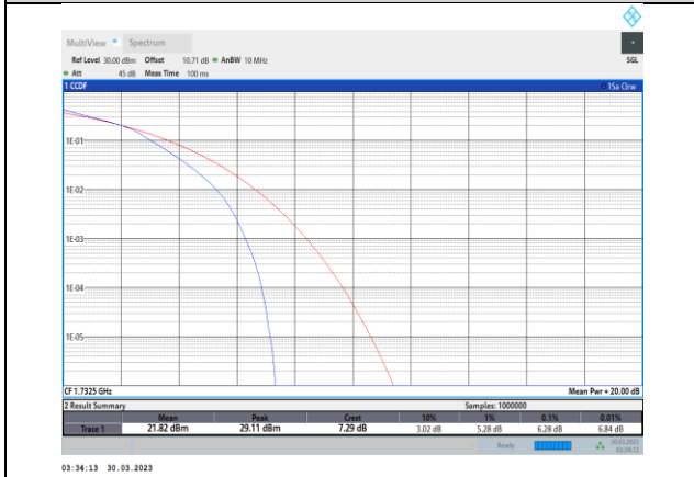
Band4-10MHz-16QAM-20175-50RB#0
