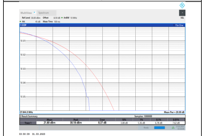
Band5-10MHz-64QAM-20600-50RB#0
