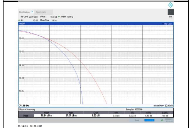
Band2-20MHz-64QAM-18900-100RB#0
