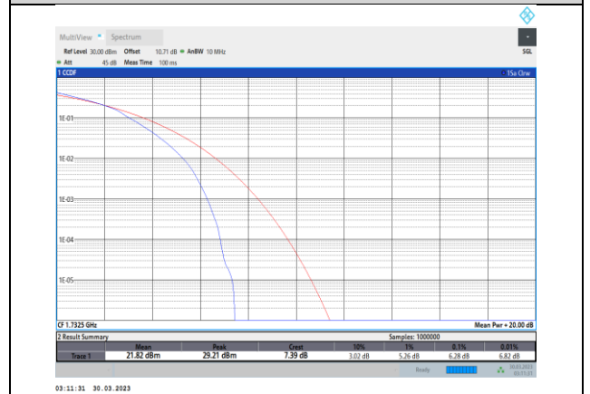
Band4-5MHz-16QAM-20175-25RB#0
