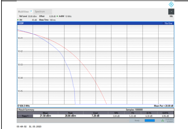
Band5-10MHz-16QAM-20525-50RB#0
