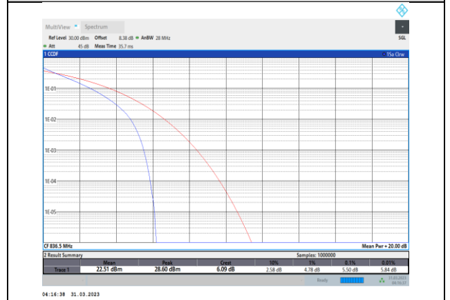
Band5-3MHz-QPSK-20525-15RB#0
