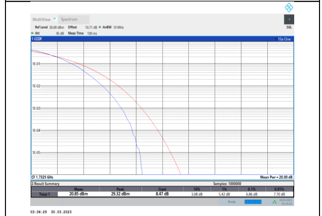
Band4-10MHz-64QAM-20175-50RB#0
