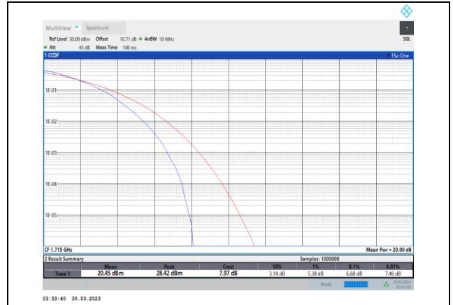
Band4-10MHz-64QAM-20000-50RB#0
