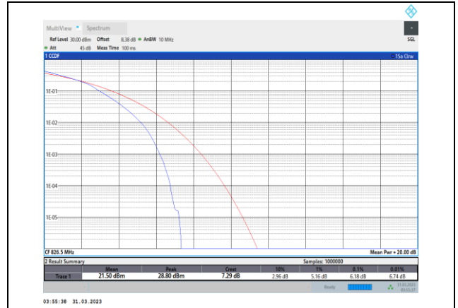
Band5-5MHz-16QAM-20425-25RB#0
