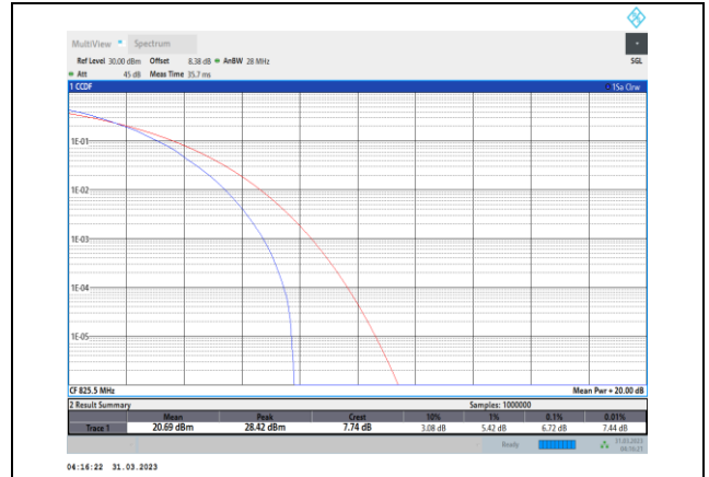
Band5-3MHz-64QAM-20415-15RB#0
