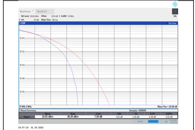
Band5-5MHz-16QAM-20625-25RB#0
