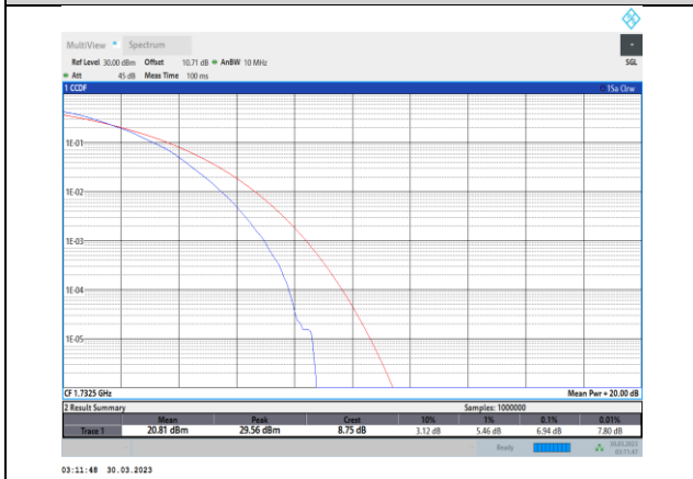
Band4-5MHz-64QAM-20175-25RB#0
