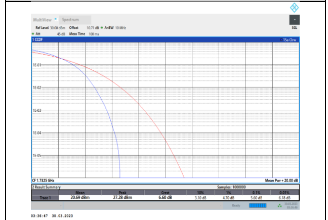
Band4-20MHz-QPSK-20175-100RB#0
