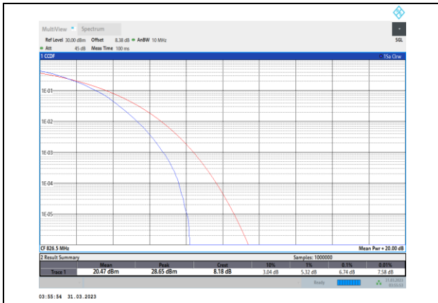
Band5-5MHz-64QAM-20425-25RB#0
