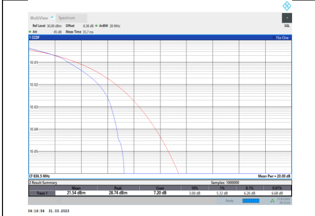
Band5-3MHz-16QAM-20525-15RB#0
