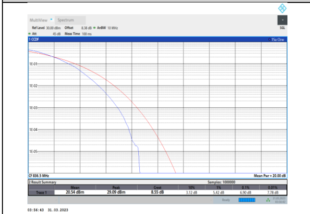
Band5-5MHz-64QAM-20525-25RB#0
