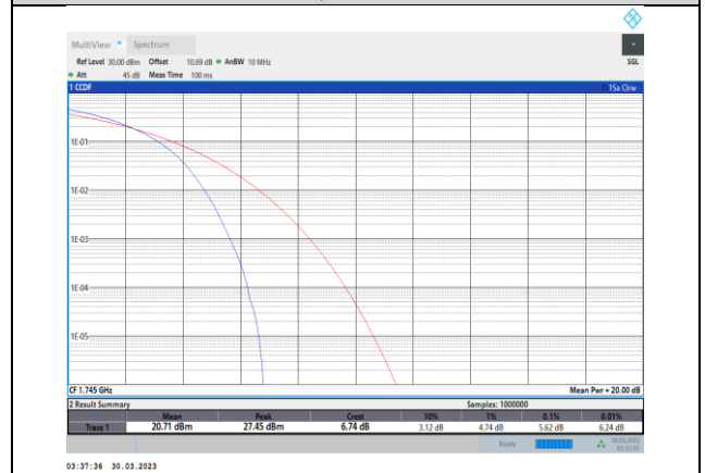
Band4-20MHz-QPSK-20300-100RB#0
