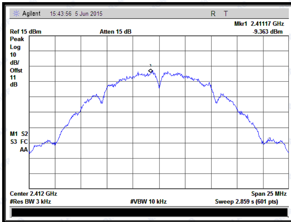
(Channel = 1 @ 802.11b)
