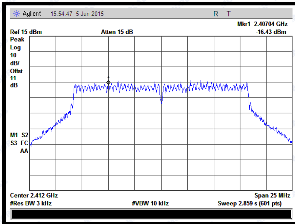
(Channel = 1 @ 802.11g)
