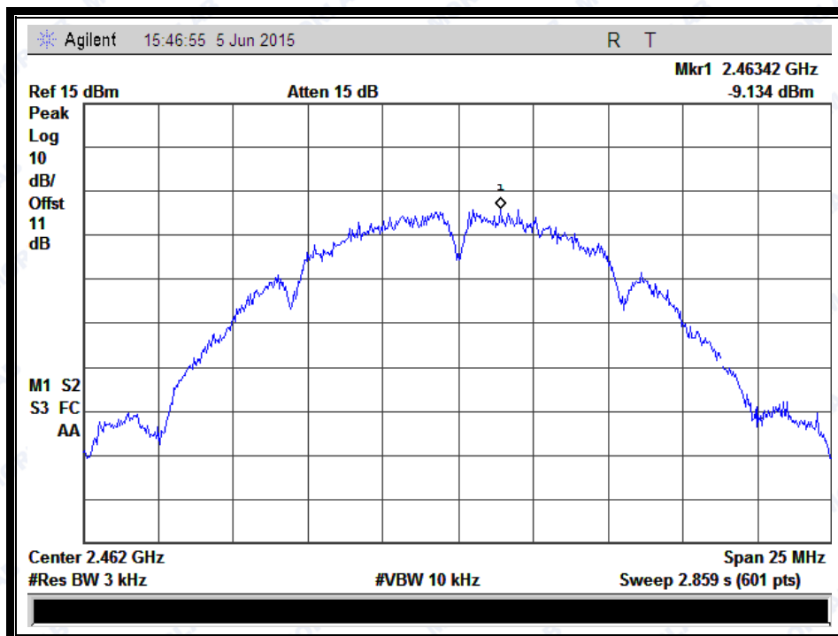
(Channel = 11 @ 802.11b)
