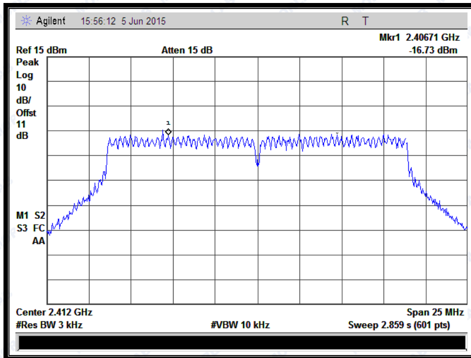
(Channel = 1 @ 802.11n-20MHz)
