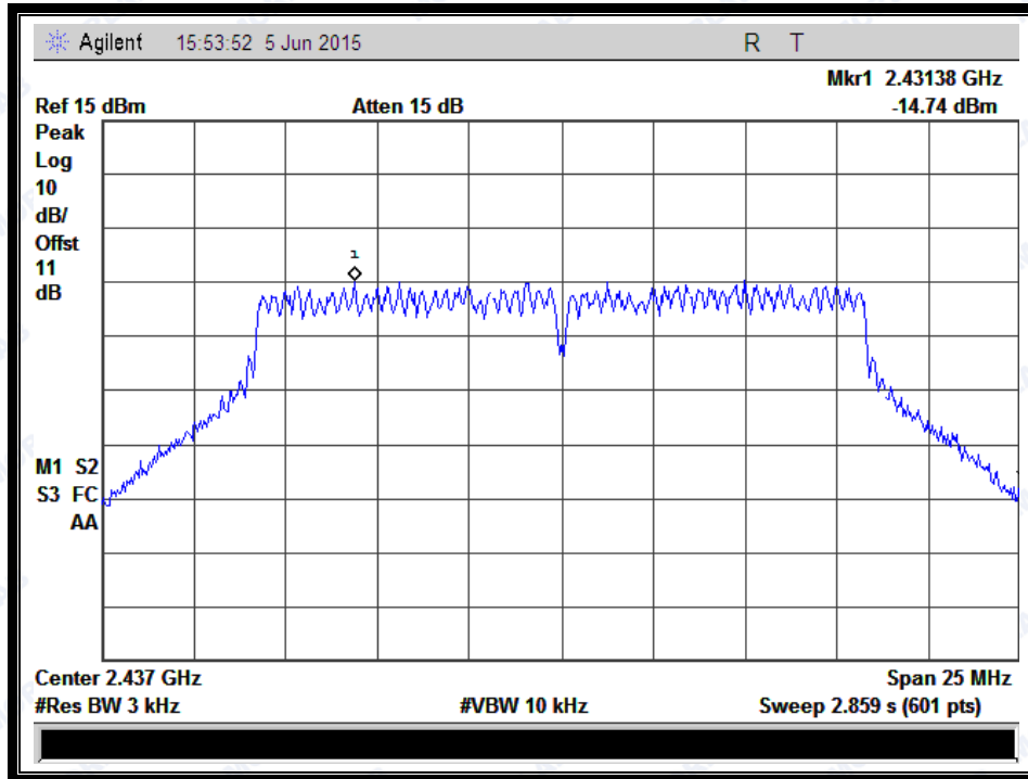
(Channel = 6 @ 802.11g)
