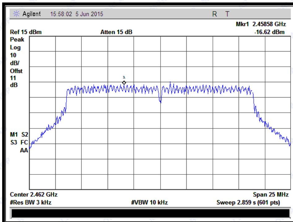
(Channel = 11 @ 802.11n-20MHz)
