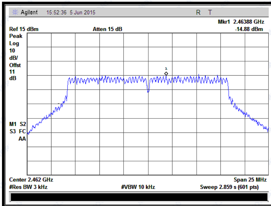
(Channel = 11 @ 802.11g)
