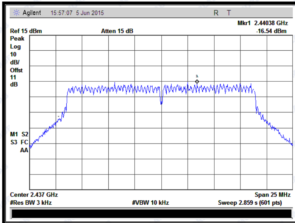
(Channel = 6 @ 802.11n-20MHz)
