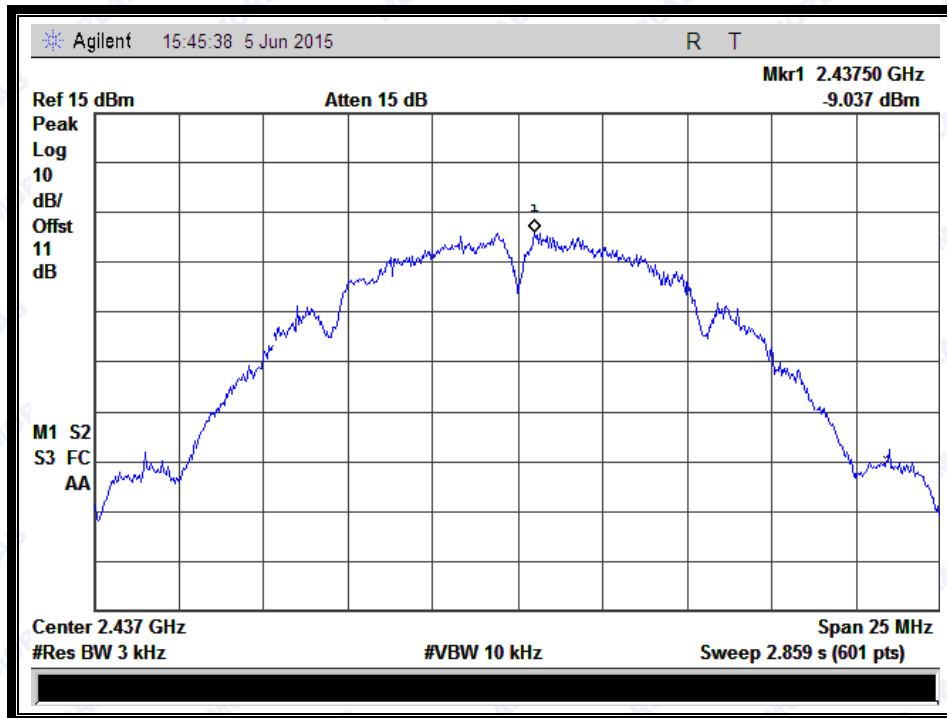
(Channel = 6 @ 802.11b)
