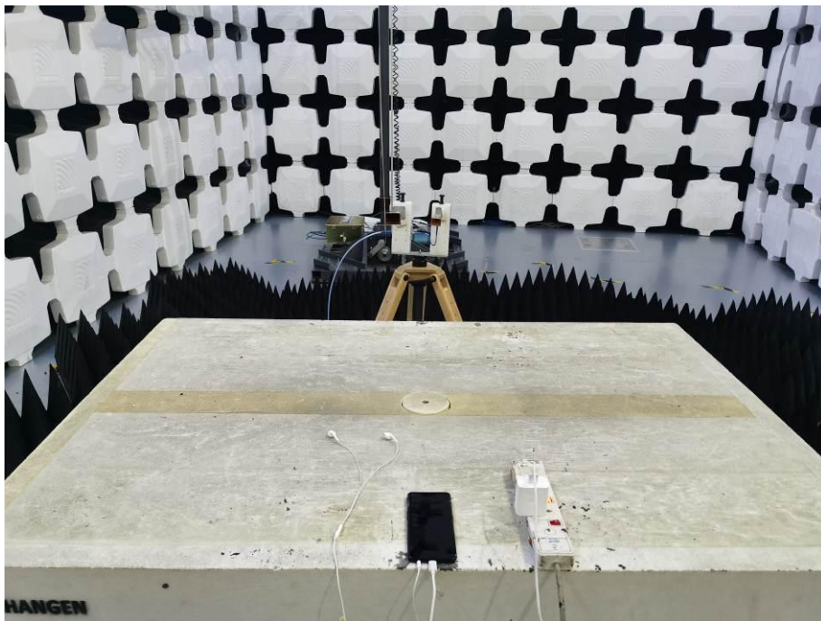
8. Radiated Emissions (Part 15B Camera/Video Player/FM receiver/GSM receiver/WCDMA receiver/LTE receiver,26.5GHz-40GHz)
