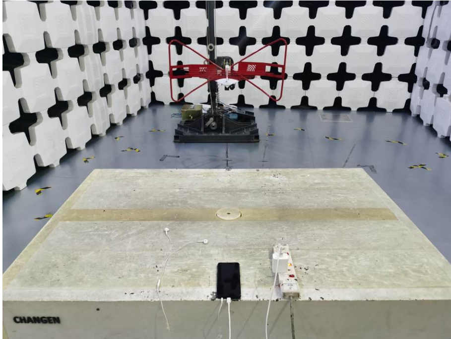
5. Radiated Emissions (Part 15B Camera/Video Player/FM receiver/GSM receiver/WCDMA receiver/LTE receiver,30MHz-1GHz)
