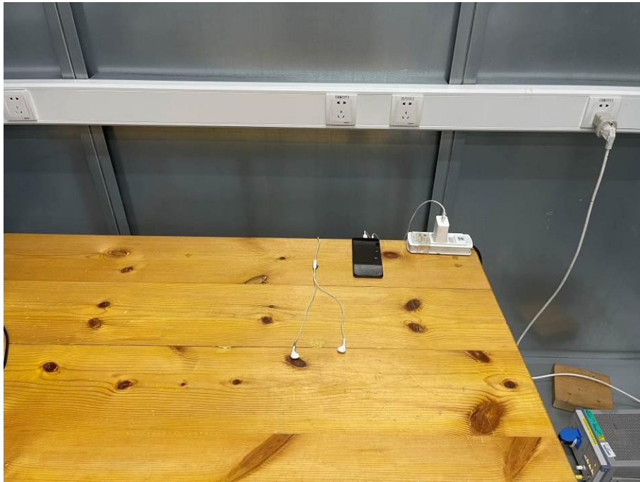
17. Conducted Emission (Part 15B& Part 15C&E, Camera/Video Player/FM receiver Wi-Fi/Bluetooth)
