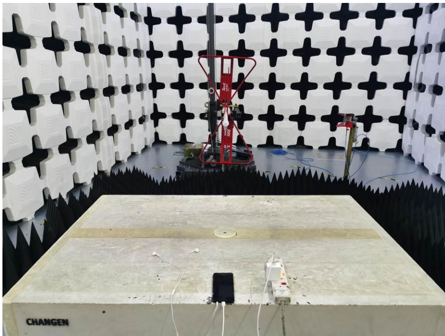
6. Radiated Emissions (Part 15B Camera/Video Player/FM receiver/GSM receiver/WCDMA receiver/LTE receiver,1GHz-18GHz)
