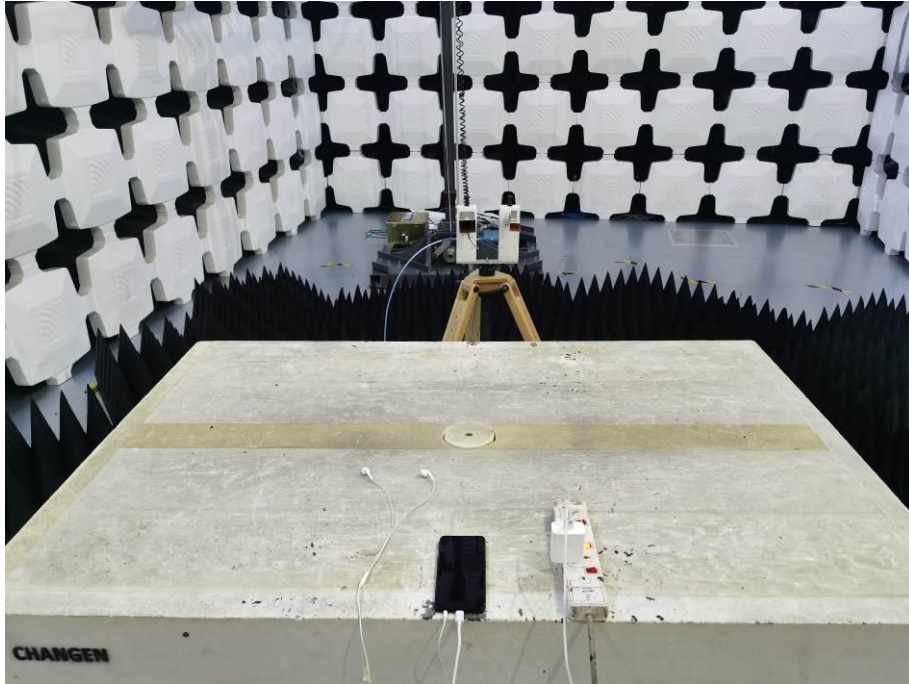
7. Radiated Emissions (Part 15B Camera/Video Player/FM receiver/GSM receiver/WCDMA receiver/LTE receiver,18GHz-26.5GHz)
