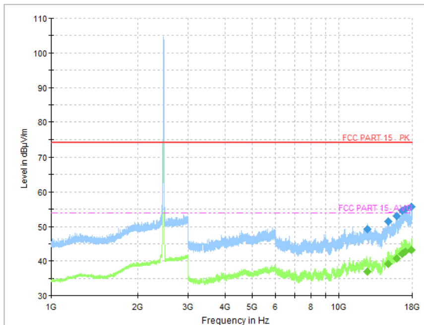
Fig.59 Radiated Spurious Emission (802.11g, CH11, 1 GHz-18 GHz)
