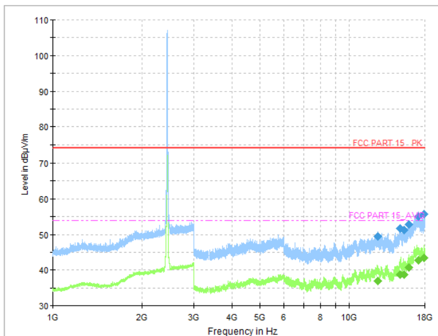
Fig.63 Radiated Spurious Emission (802.11n-HT20, CH6, 1 GHz-18 GHz)
