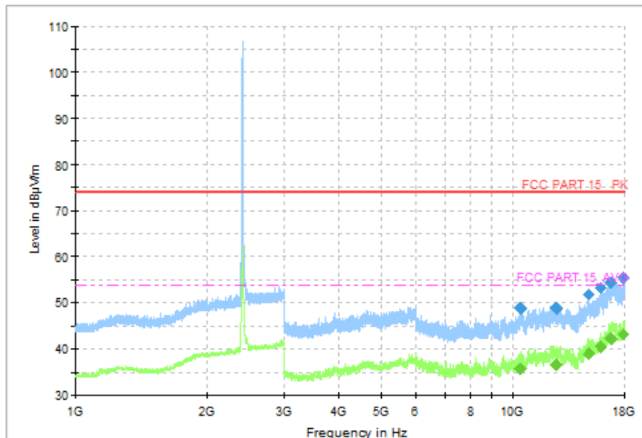
Fig.57 Radiated Spurious Emission (802.11g, CH1, 1 GHz-18 GHz)
