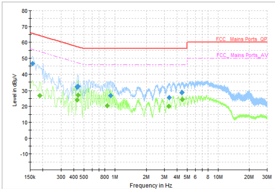
Fig. 79 AC Power line Conducted Emission (Traffic)
