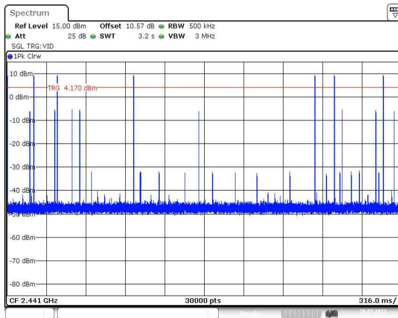
Fig. 72 Number of Burst in Observation Period (Dwell Time) (8DPSK, CH39)
