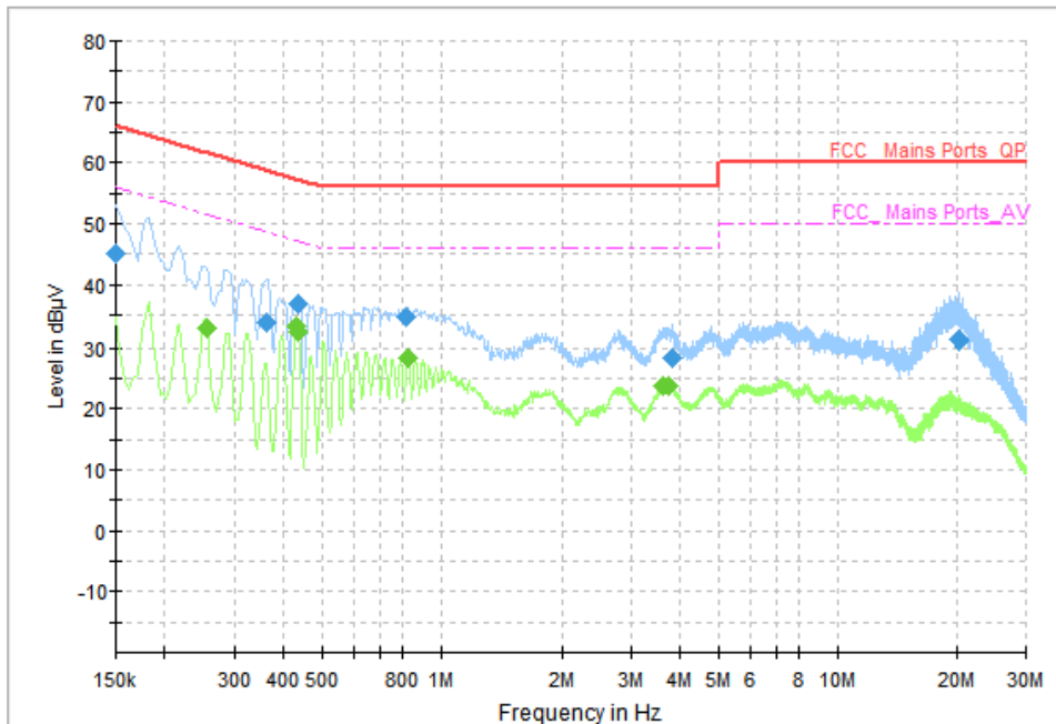
Fig. 80 AC Power line Conducted Emission (Idle)
