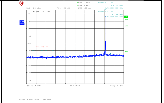
Band38-5MHz-16QAM-38225-1RB#0-Range2:1000~3000MHz
