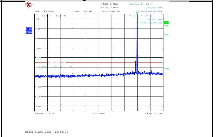
Band38-5MHz-QPSK-38000-1RB#0- Range2:1000~3000MHz
