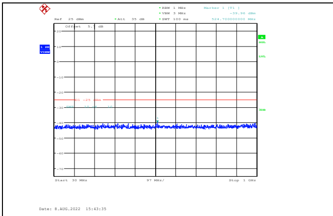
Band38-5MHz-16QAM-38000-1RB#0-Range1:30~1000MHz
