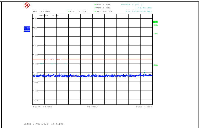
Band38-20MHz-64QAM-38150-1RB#0-Range1:30~1000MHz
