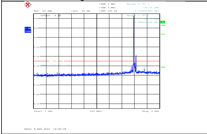
Band38-20MHz-64QAM-38000-1RB#0-Range2:1000~3000MHz
