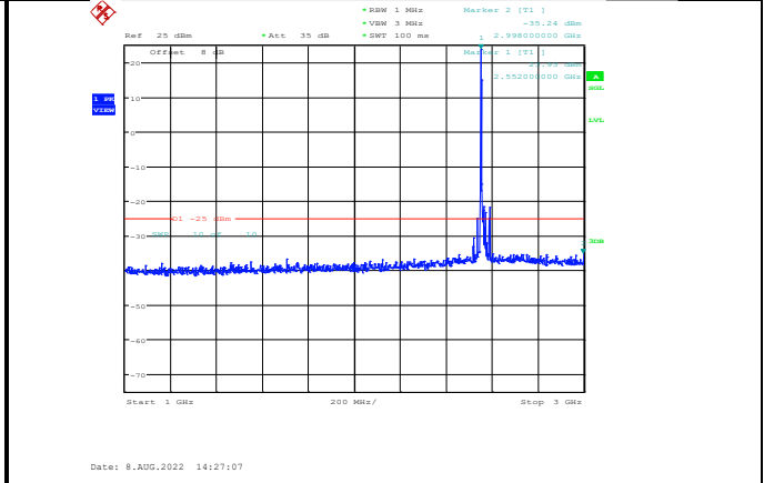
Band7-20MHz-64QAM-21350-1RB#0-Range2:1000~3000MHz
