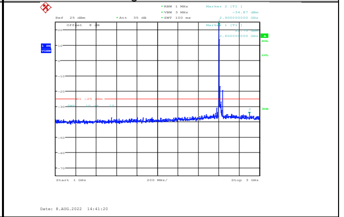
Band38-20MHz-64QAM-38150-1RB#0-Range2:1000~3000MHz
