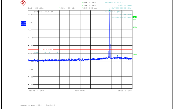
Band38-5MHz-16QAM-37775-1RB#0-Range2:1000~3000MHz
