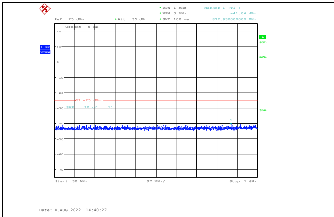
Band38-20MHz-64QAM-38000-1RB#0-Range1:30~1000MHz
