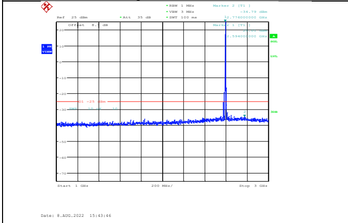
Band38-5MHz-16QAM-38000-1RB#0-Range2:1000~3000MHz
