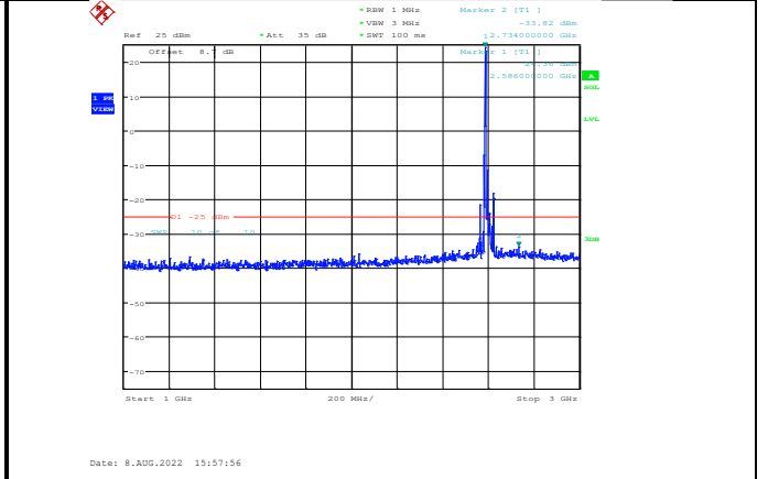
Band38-20MHz-16QAM-38000-1RB#0-Range2:1000~3000MHz
