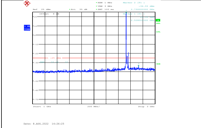
Band7-20MHz-64QAM-21100-1RB#0-Range2:1000~3000MHz
