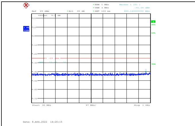
Band7-20MHz-64QAM-21100-1RB#0-Range1:30~1000MHz
