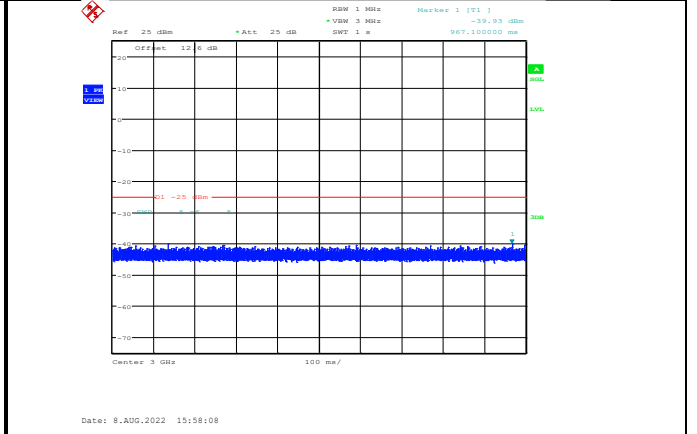
Band38-20MHz-16QAM-38000-1RB#0-Range3:3000~27000MHz
