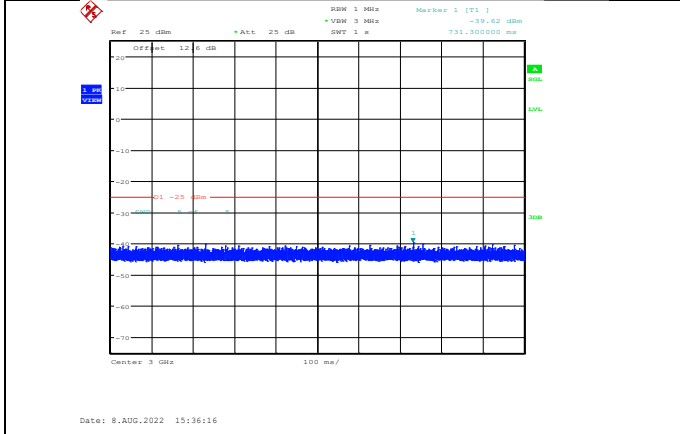
Band7-20MHz-16QAM-21350-1RB#0-Range3:3000~27000MHz
