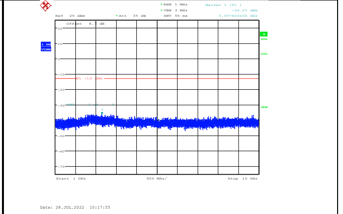
Band5-5MHz-16QAM-20625-1RB#0-Range2:1000~10000MHz
