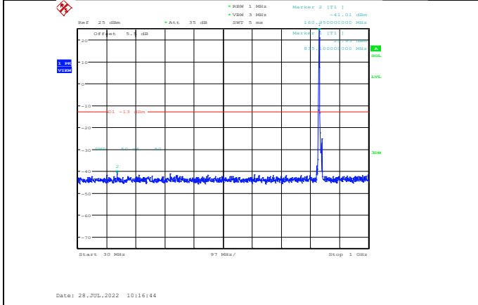
Band5-5MHz-16QAM-20525-1RB#0-Range1:30~1000MHz
