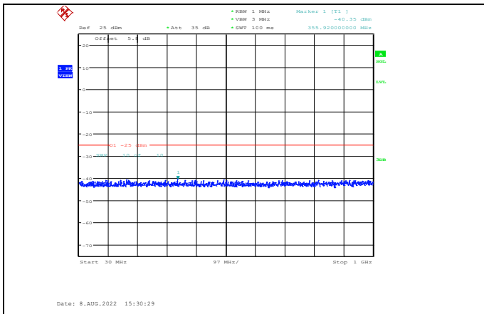
Band7-15MHz-QPSK-21375-1RB#0-Range1:30~1000MHz
