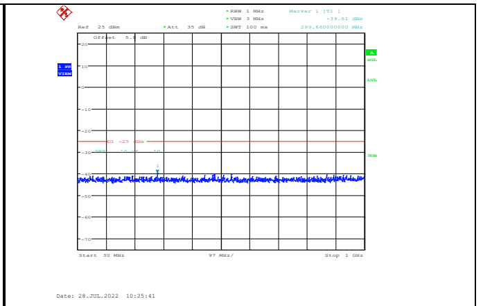
Band7-5MHz-QPSK-21100-1RB#0- Range1:30~1000MHz
