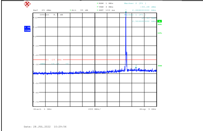
Band7-10MHz-16QAM-20800-1RB#0-Range2:1000~3000MHz
