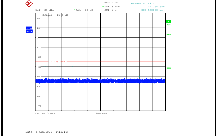
Band7-10MHz-64QAM-21400-1RB#0-Range3:3000~27000MHz
