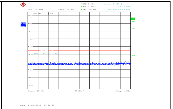
Band7-20MHz-16QAM-21100-1RB#0-Range1:30~1000MHz
