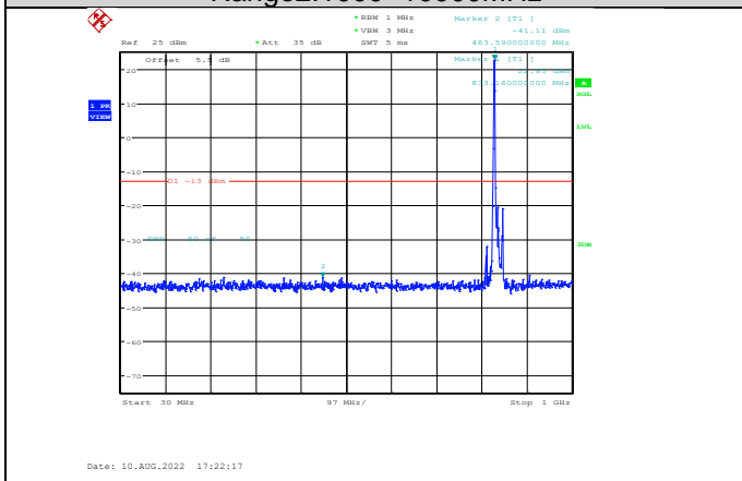
Band5-10MHz-64QAM-20525-1RB#0- Range1:30~1000MHz
