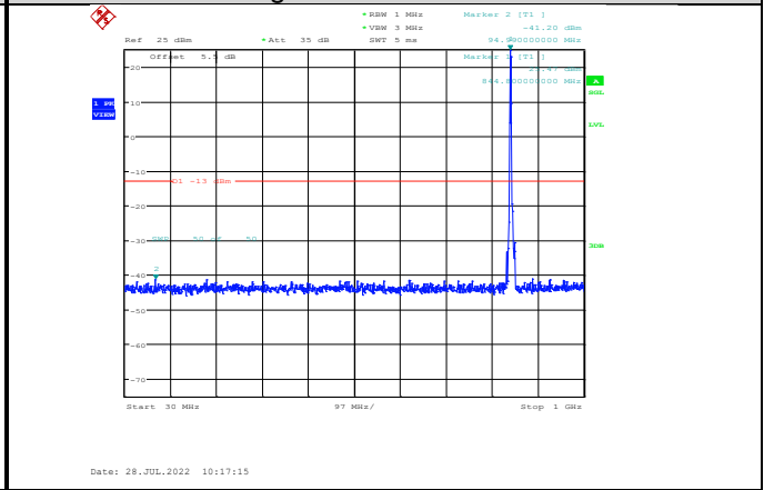
Band5-5MHz-QPSK-20625-1RB#0- Range1:30~1000MHz
