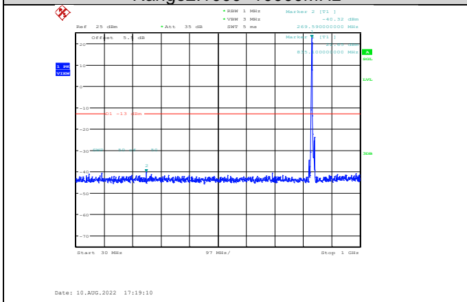
Band5-5MHz-64QAM-20525-1RB#0- Range1:30~1000MHz
