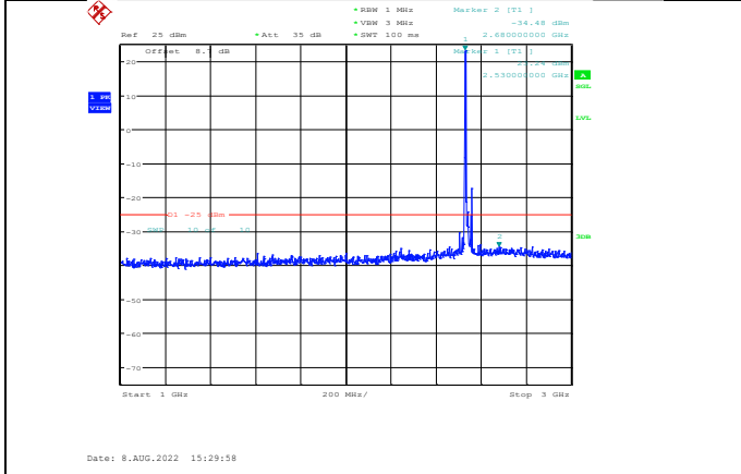
Band7-15MHz-16QAM-21100-1RB#0-Range2:1000~3000MHz
