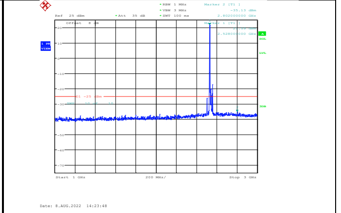
Band7-15MHz-64QAM-21100-1RB#0-Range2:1000~3000MHz
