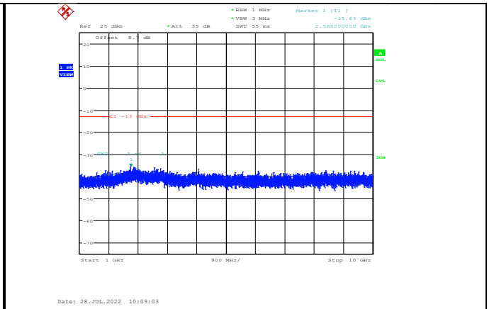
Band5-1.4MHz-QPSK-20525-1RB#0-Range2:1000~10000MHz
