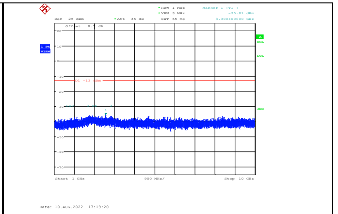
Band5-5MHz-64QAM-20525-1RB#0- Range2:1000~10000MHz
