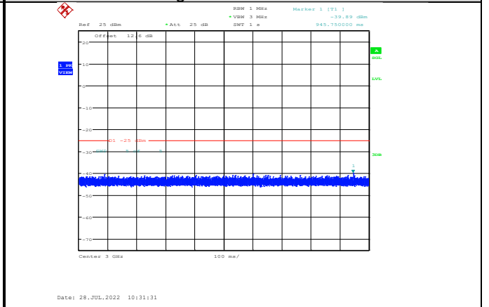
Band7-10MHz-16QAM-21100-1RB#0-Range3:3000~27000MHz
