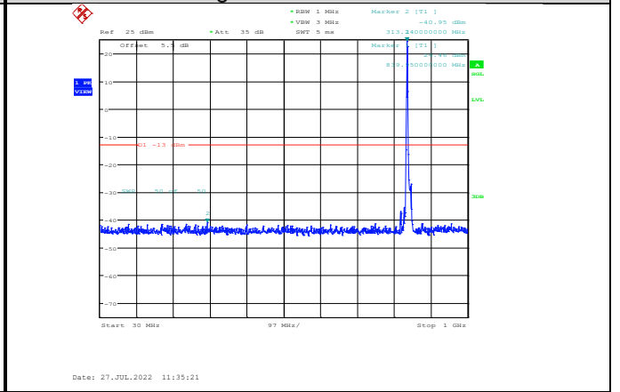
Band5-10MHz-16QAM-20600-1RB#0- Range1:30~1000MHz
