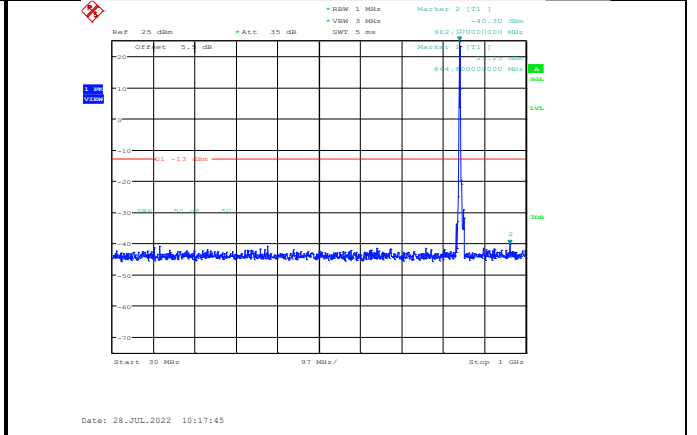
Band5-5MHz-16QAM-20625-1RB#0-Range1:30~1000MHz
