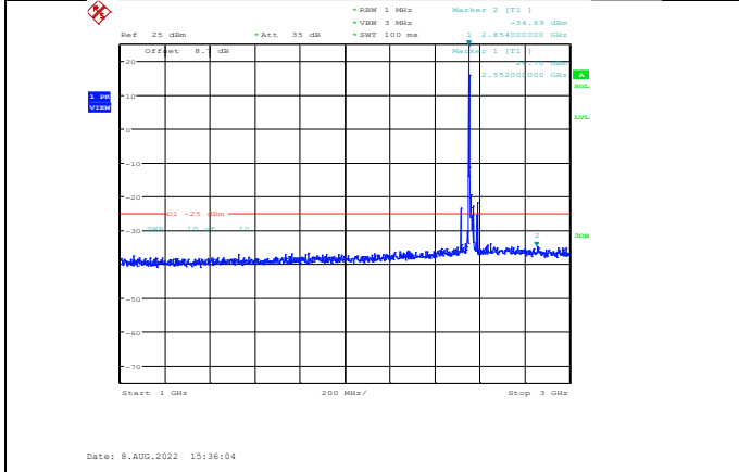
Band7-20MHz-16QAM-21350-1RB#0-Range2:1000~3000MHz
