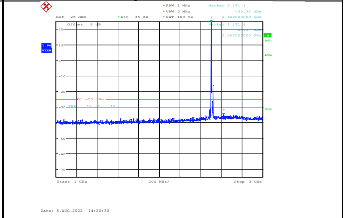
Band7-10MHz-64QAM-20800-1RB#0-Range2:1000~3000MHz
