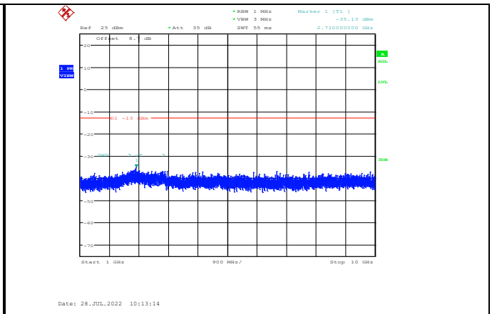
Band5-3MHz-16QAM-20525-1RB#0-Range2:1000~10000MHz
