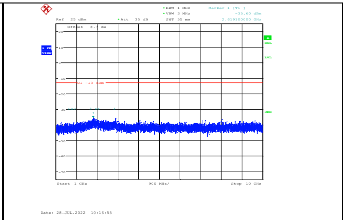
Band5-5MHz-16QAM-20525-1RB#0-Range2:1000~10000MHz
