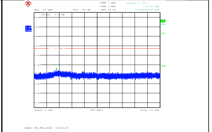
Band5-3MHz-16QAM-20635-1RB#0-Range2:1000~10000MHz
