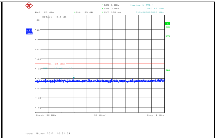
Band7-10MHz-16QAM-21100-1RB#0-Range1:30~1000MHz
