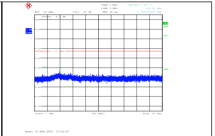
Band5-10MHz-64QAM-20525-1RB#0- Range2:1000~10000MHz
