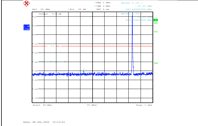
Band5-3MHz-16QAM-20525-1RB#0-Range1:30~1000MHz
