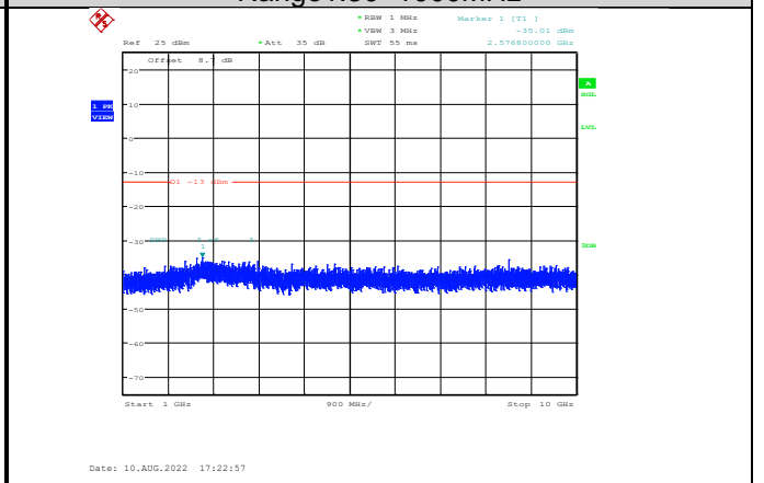
Band5-10MHz-64QAM-20600-1RB#0- Range2:1000~10000MHz
