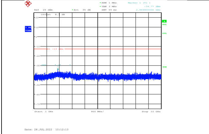
Band5-3MHz-16QAM-20415-1RB#0-Range2:1000~10000MHz
