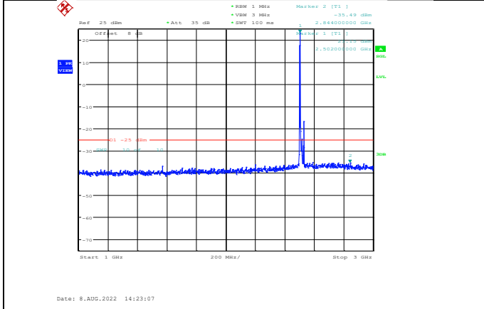
Band7-15MHz-64QAM-20825-1RB#0-Range2:1000~3000MHz
