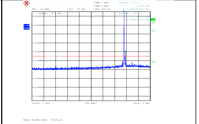
Band7-15MHz-16QAM-21375-1RB#0-Range2:1000~3000MHz
