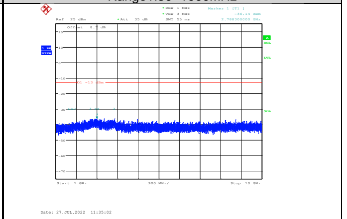
Band5-10MHz-QPSK-20600-1RB#0- Range2:1000~10000MHz
