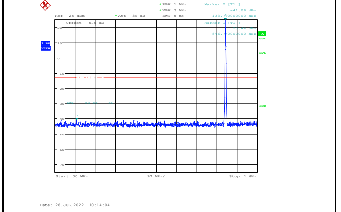
Band5-3MHz-16QAM-20635-1RB#0-Range1:30~1000MHz
