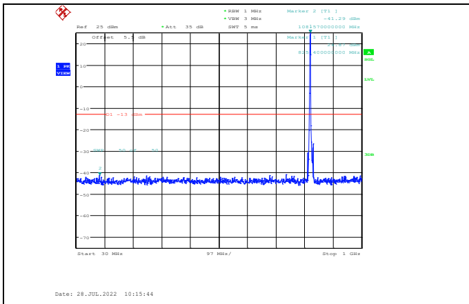
Band5-5MHz-16QAM-20425-1RB#0-Range1:30~1000MHz
