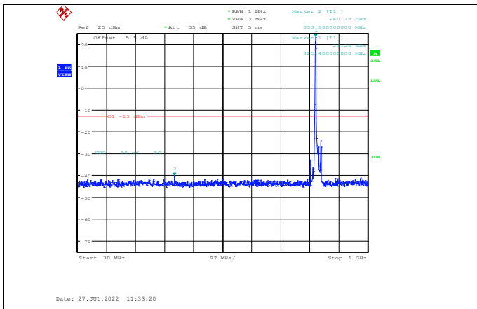
Band5-10MHz-16QAM-20450-1RB#0- Range1:30~1000MHz
