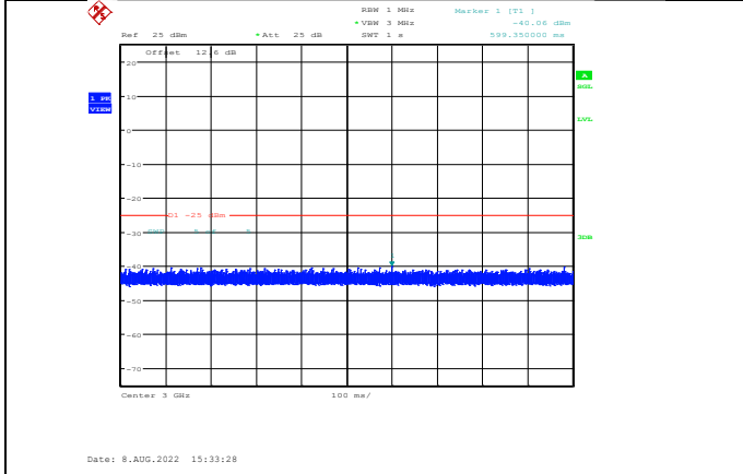
Band7-20MHz-16QAM-20850-1RB#0-Range3:3000~27000MHz
