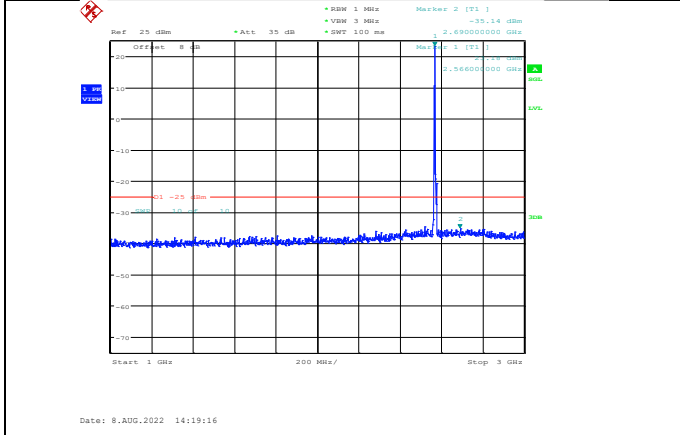
Band7-5MHz-64QAM-21425-1RB#0-Range2:1000~3000MHz
