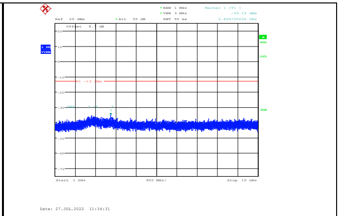
Band5-10MHz-16QAM-20525-1RB#0- Range2:1000~10000MHz
