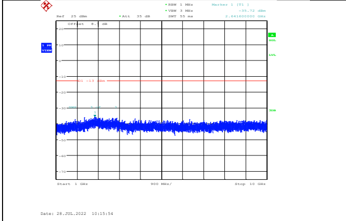
Band5-5MHz-16QAM-20425-1RB#0-Range2:1000~10000MHz
