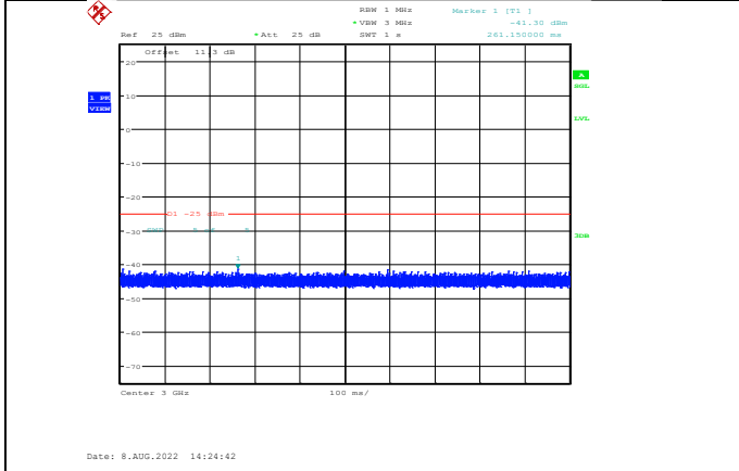
Band7-15MHz-64QAM-21375-1RB#0-Range3:3000~27000MHz
