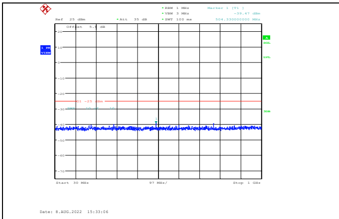
Band7-20MHz-16QAM-20850-1RB#0-Range1:30~1000MHz
