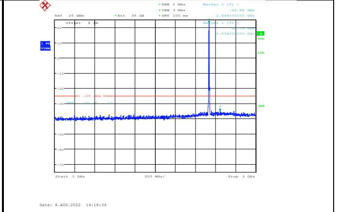
Band7-5MHz-64QAM-21100-1RB#0- Range2:1000~3000MHz
