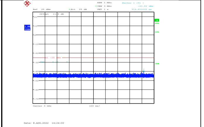
Band7-15MHz-64QAM-21100-1RB#0-Range3:3000~27000MHz
