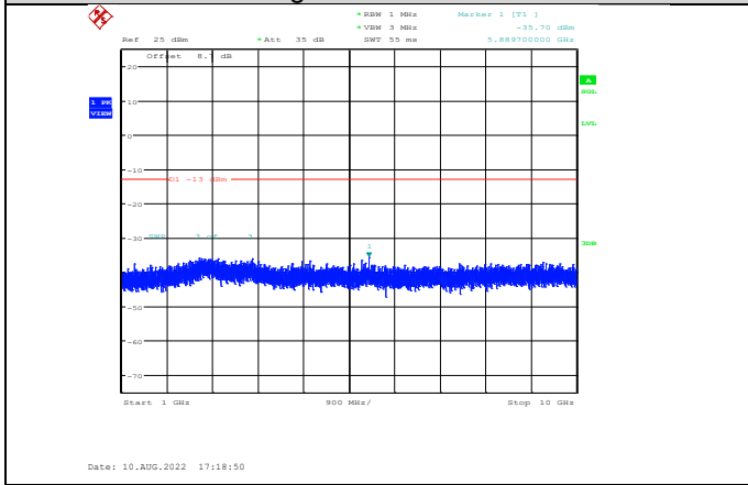
Band5-5MHz-64QAM-20425-1RB#0- Range2:1000~10000MHz
