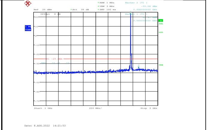
Band7-10MHz-64QAM-21400-1RB#0-Range2:1000~3000MHz
