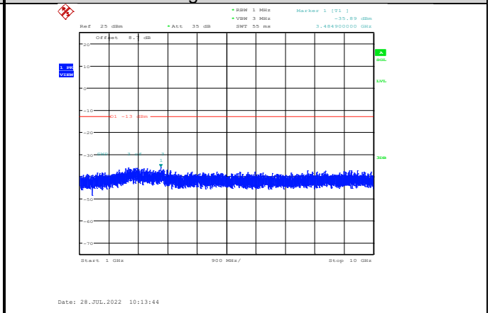
Band5-3MHz-QPSK-20635-1RB#0- Range2:1000~10000MHz
