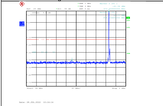
Band5-5MHz-QPSK-20525-1RB#0- Range1:30~1000MHz
