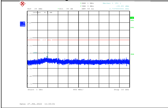
Band5-10MHz-QPSK-20450-1RB#0- Range2:1000~10000MHz
