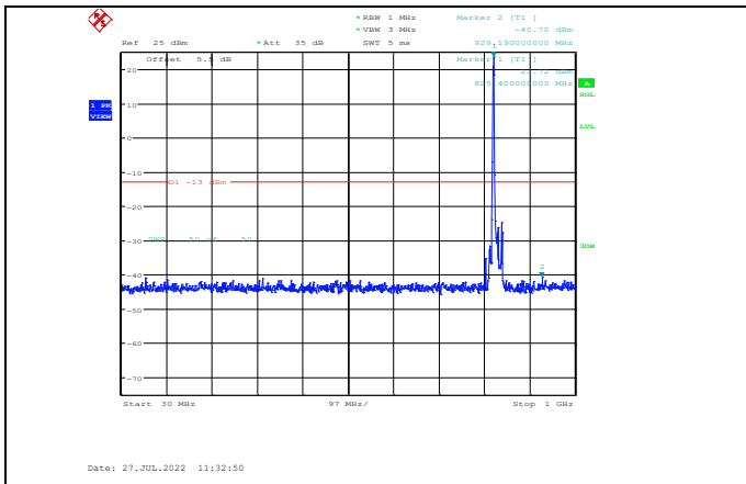
Band5-10MHz-QPSK-20450-1RB#0- Range1:30~1000MHz
