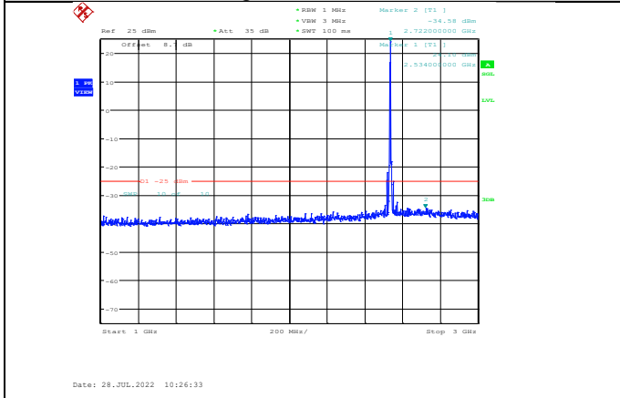
Band7-5MHz-16QAM-21100-1RB#0- Range2:1000~3000MHz
