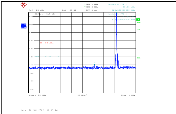
Band5-5MHz-QPSK-20425-1RB#0- Range1:30~1000MHz
