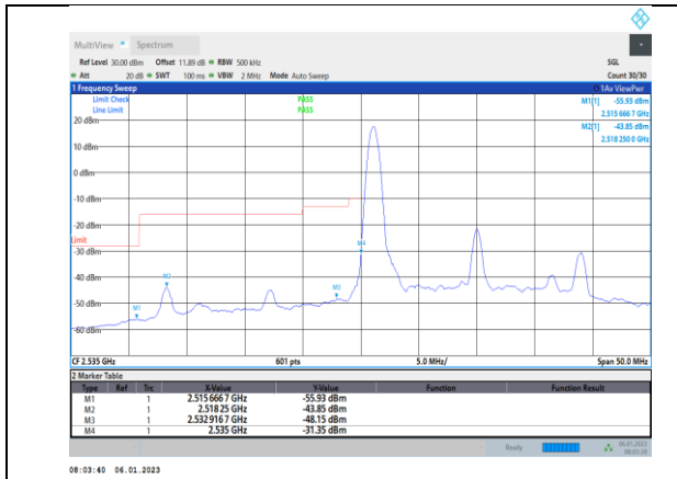
Band41-20MHz-64QAM-40140-100RB#0
