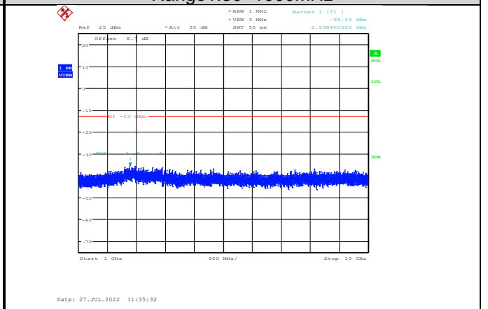
Band5-10MHz-16QAM-20600-1RB#0- Range2:1000~10000MHz
