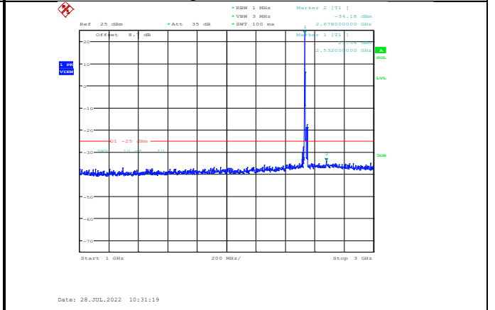
Band7-10MHz-16QAM-21100-1RB#0-Range2:1000~3000MHz
