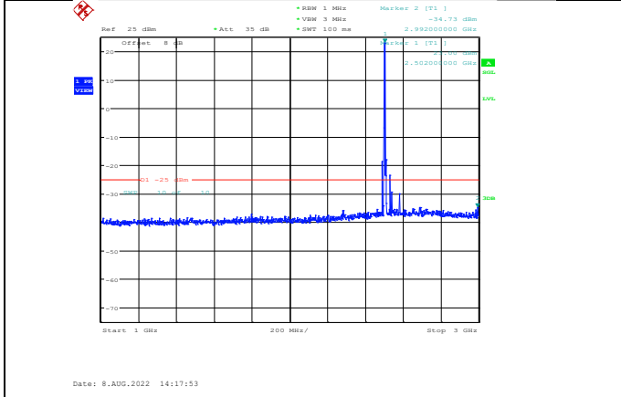
Band7-5MHz-64QAM-20775-1RB#0- Range2:1000~3000MHz
