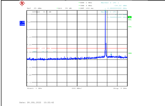
Band7-10MHz-16QAM-21400-1RB#0-Range2:1000~3000MHz
