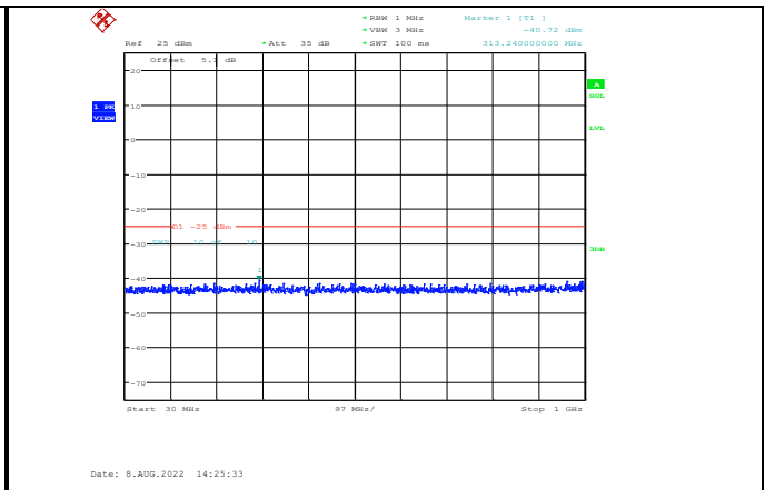
Band7-20MHz-64QAM-20850-1RB#0-Range1:30~1000MHz
