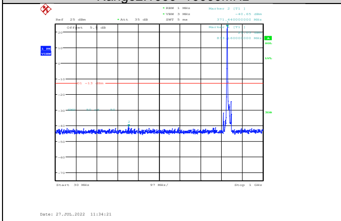
Band5-10MHz-16QAM-20525-1RB#0- Range1:30~1000MHz
