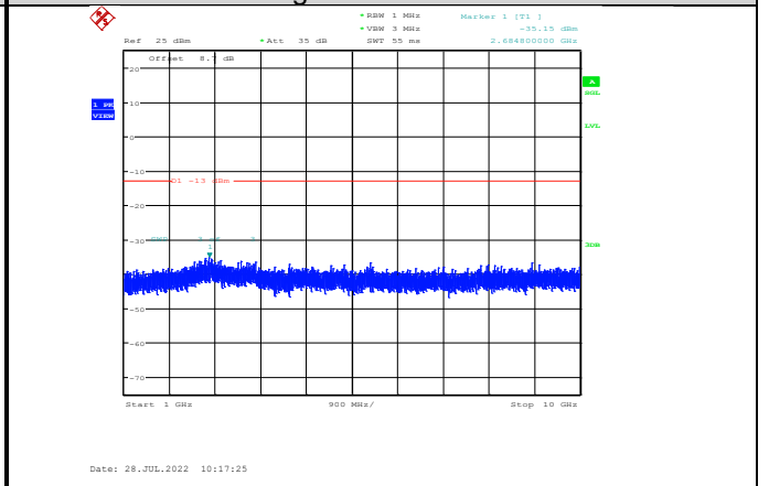
Band5-5MHz-QPSK-20625-1RB#0- Range2:1000~10000MHz
