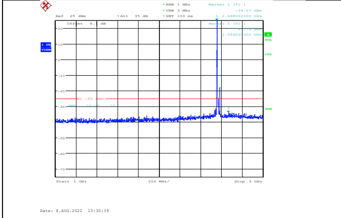
Band7-15MHz-QPSK-21375-1RB#0-Range2:1000~3000MHz
