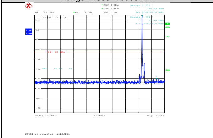
Band5-10MHz-QPSK-20525-1RB#0- Range1:30~1000MHz
