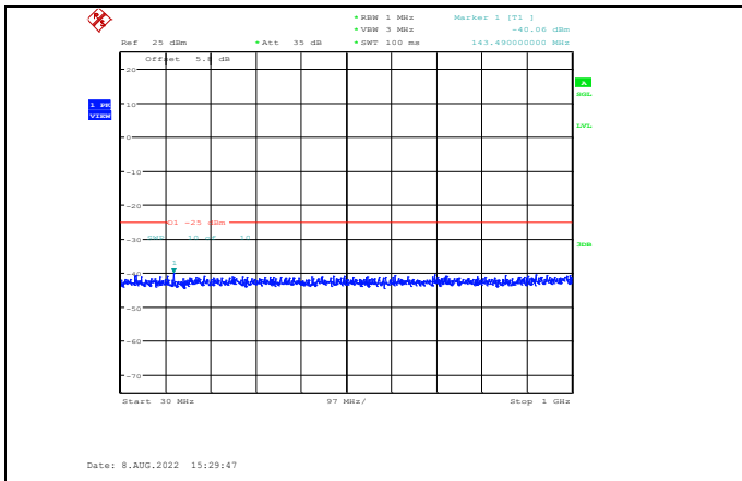
Band7-15MHz-16QAM-21100-1RB#0-Range1:30~1000MHz
