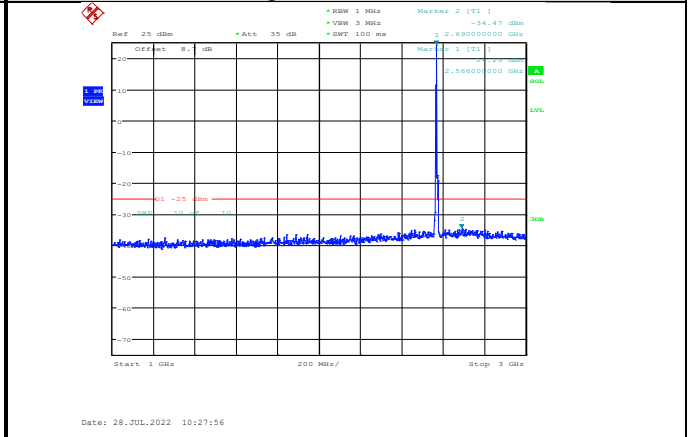
Band7-5MHz-16QAM-21425-1RB#0- Range2:1000~3000MHz
