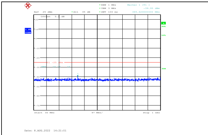
Band7-10MHz-64QAM-21100-1RB#0-Range1:30~1000MHz
