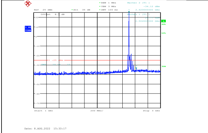
Band7-20MHz-16QAM-20850-1RB#0-Range2:1000~3000MHz
