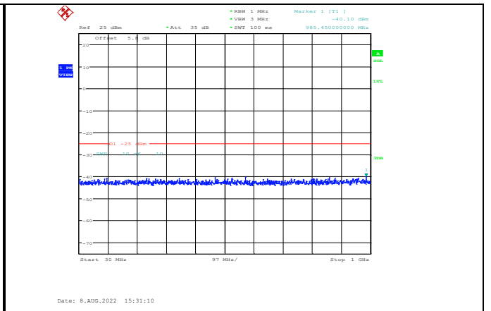
Band7-15MHz-16QAM-21375-1RB#0-Range1:30~1000MHz
