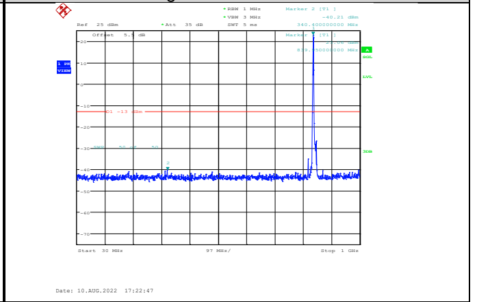
Band5-10MHz-64QAM-20600-1RB#0- Range1:30~1000MHz
