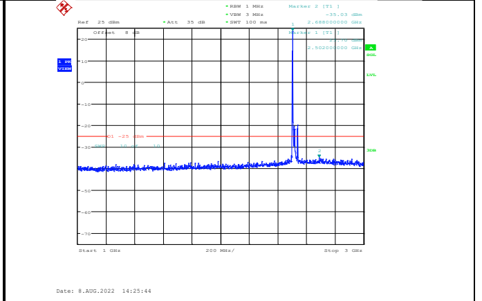
Band7-20MHz-64QAM-20850-1RB#0-Range2:1000~3000MHz
