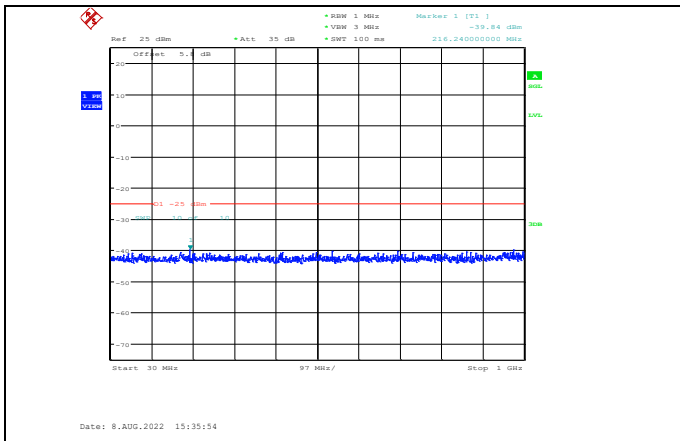
Band7-20MHz-16QAM-21350-1RB#0-Range1:30~1000MHz
