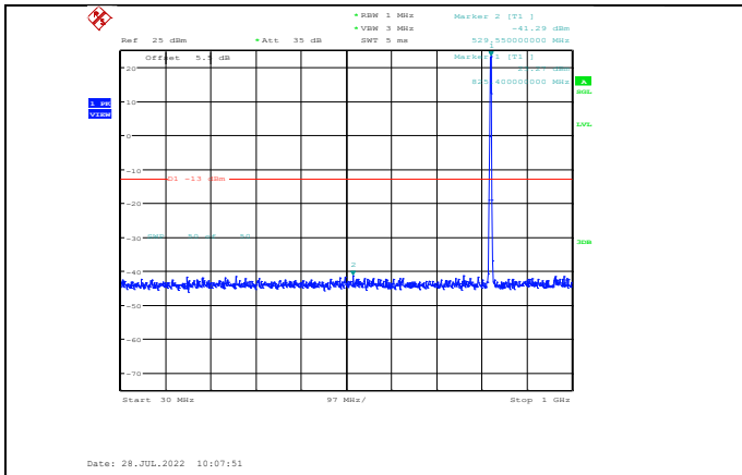
Band5-1.4MHz-QPSK-20407-1RB#0-Range1:30~1000MHz
