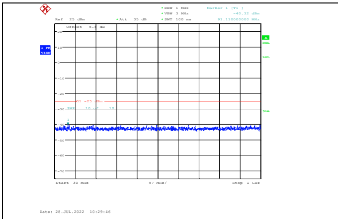
Band7-10MHz-16QAM-20800-1RB#0-Range1:30~1000MHz
