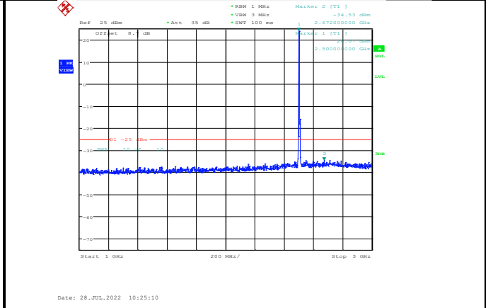
Band7-5MHz-16QAM-20775-1RB#0-Range2:1000~3000MHz
