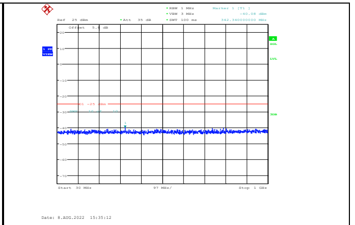
Band7-20MHz-QPSK-21350-1RB#0-Range1:30~1000MHz
