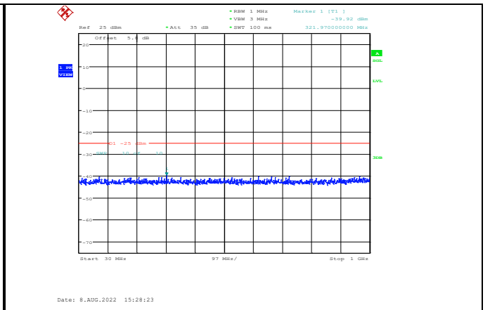
Band7-15MHz-16QAM-20825-1RB#0-Range1:30~1000MHz
