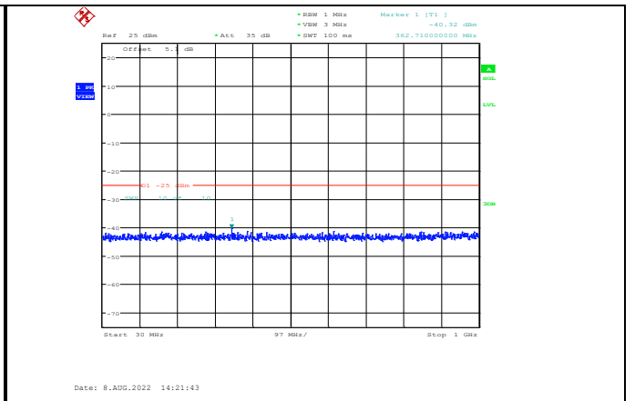
Band7-10MHz-64QAM-21400-1RB#0-Range1:30~1000MHz
