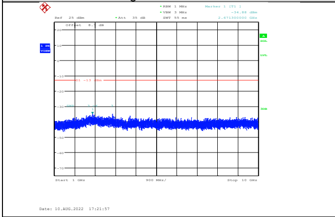
Band5-10MHz-64QAM-20450-1RB#0- Range2:1000~10000MHz
