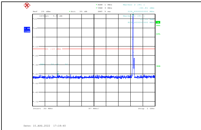
Band5-5MHz-64QAM-20425-1RB#0- Range1:30~1000MHz
