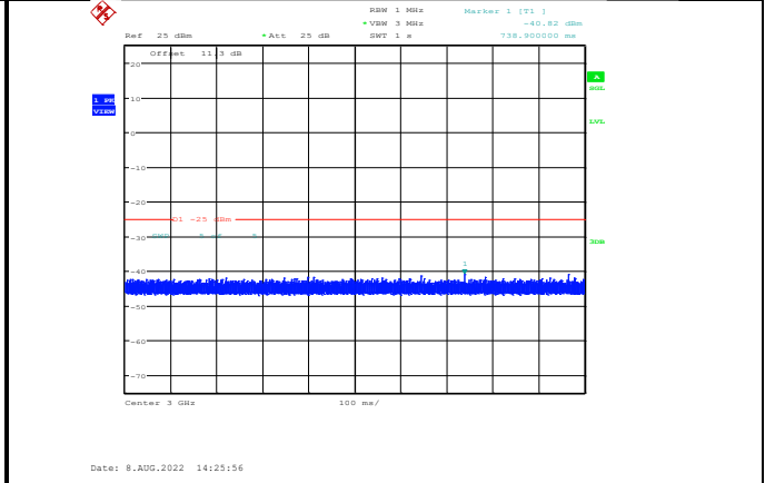
Band7-20MHz-64QAM-20850-1RB#0-Range3:3000~27000MHz
