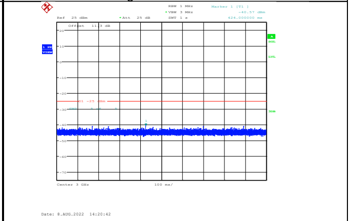
Band7-10MHz-64QAM-20800-1RB#0-Range3:3000~27000MHz
