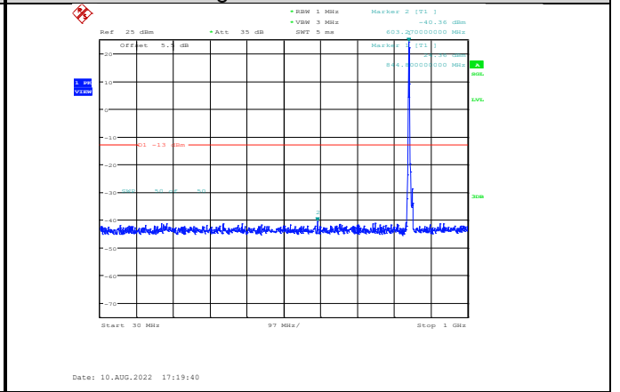
Band5-5MHz-64QAM-20625-1RB#0- Range1:30~1000MHz
