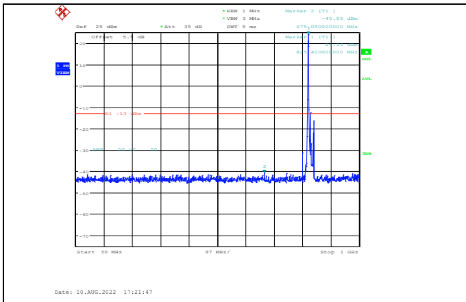
Band5-10MHz-64QAM-20450-1RB#0- Range1:30~1000MHz
