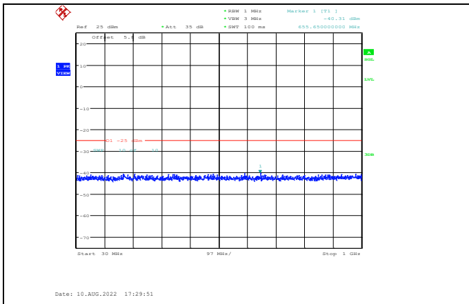
Band7-5MHz-QPSK-20775-1RB#0- Range1:30~1000MHz
