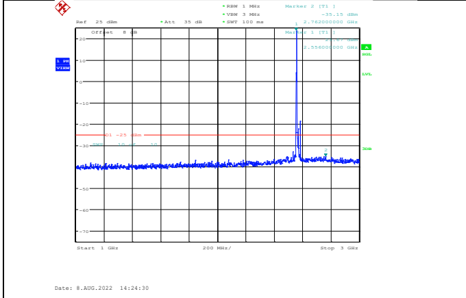
Band7-15MHz-64QAM-21375-1RB#0-Range2:1000~3000MHz
