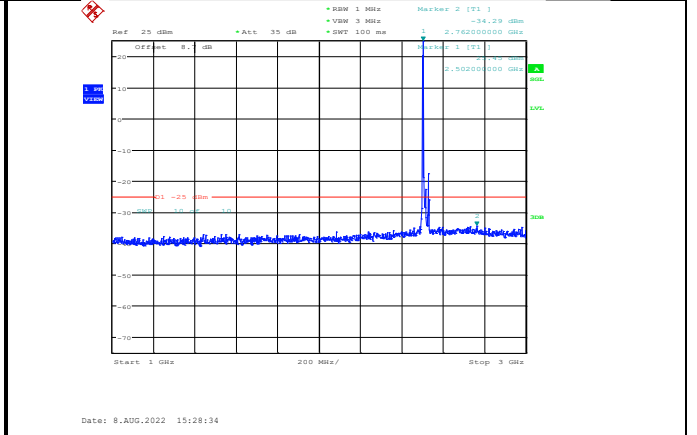
Band7-15MHz-16QAM-20825-1RB#0-Range2:1000~3000MHz
