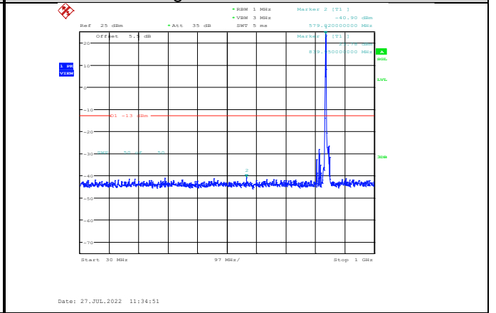
Band5-10MHz-QPSK-20600-1RB#0- Range1:30~1000MHz
