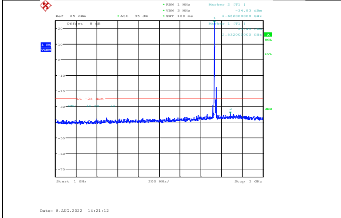
Band7-10MHz-64QAM-21100-1RB#0-Range2:1000~3000MHz
