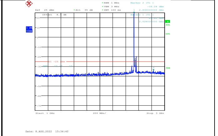
Band7-20MHz-16QAM-21100-1RB#0-Range2:1000~3000MHz
