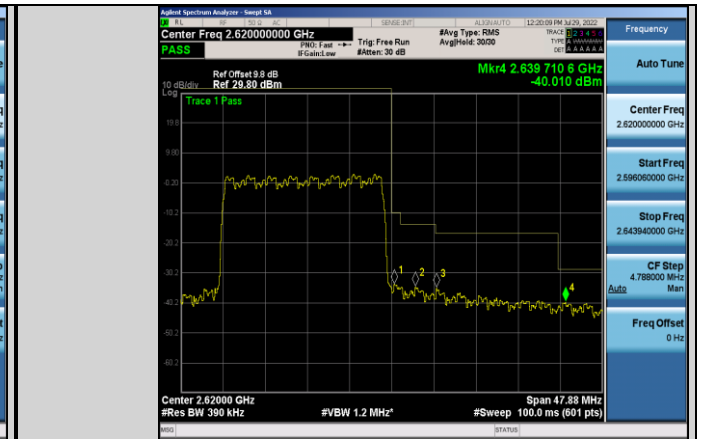
Band38-20MHz-16QAM-38150-100RB#0
