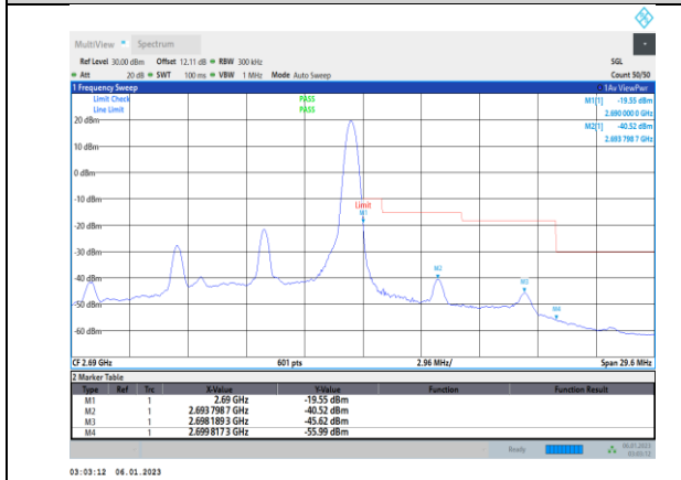
Band41-10MHz-16QAM-41540-50RB#0
