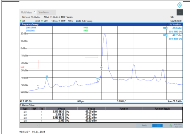
Band41-20MHz-16QAM-40140-100RB#0
