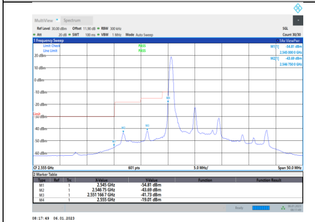
Band41-10MHz-64QAM-40290-50RB#0
