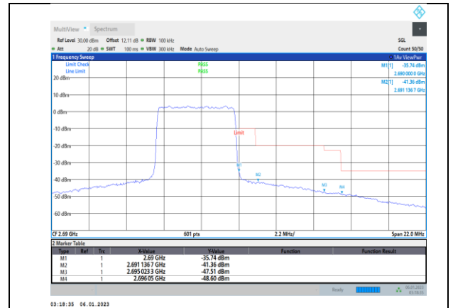
Band41-5MHz-64QAM-39675-1RB#0
