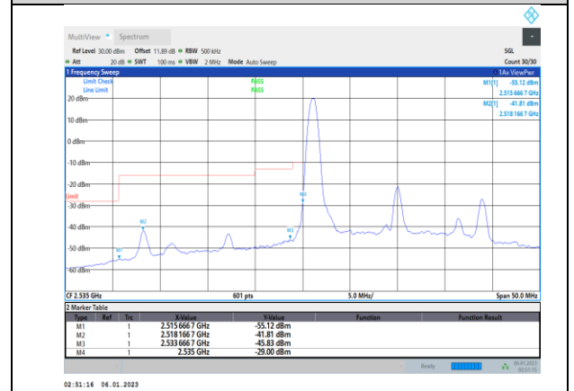
Band41-20MHz-QPSK-40140-100RB#0
