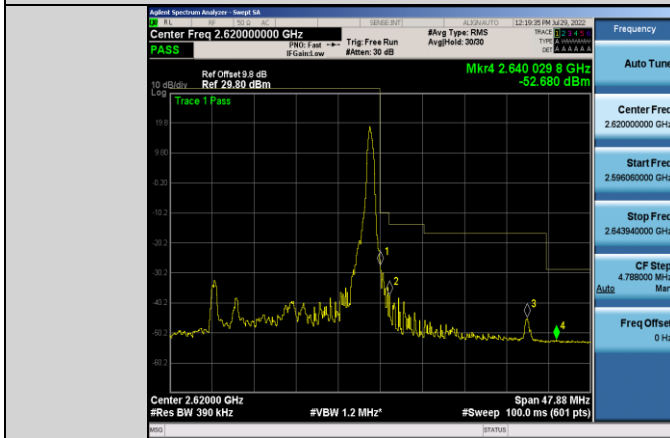
Band38-20MHz-16QAM-38150-1RB#99
