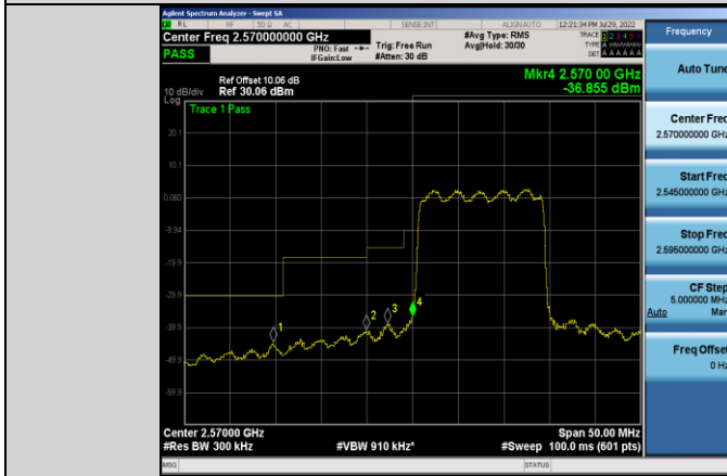
Band38-15MHz-16QAM-37825-75RB#0
