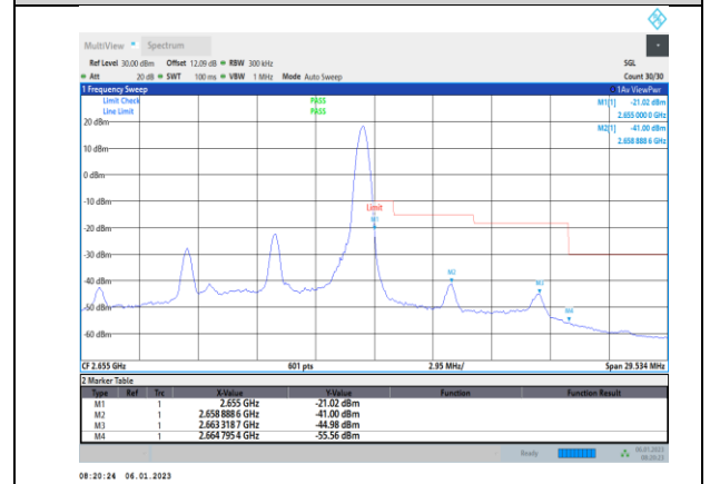
Band41-10MHz-64QAM-41190-50RB#0
