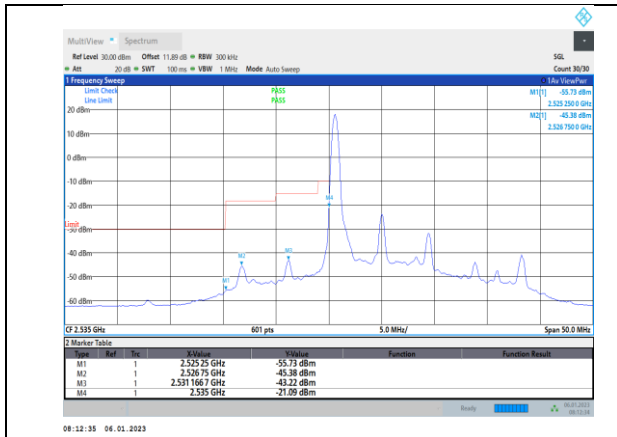
Band41-10MHz-64QAM-40090-50RB#0
