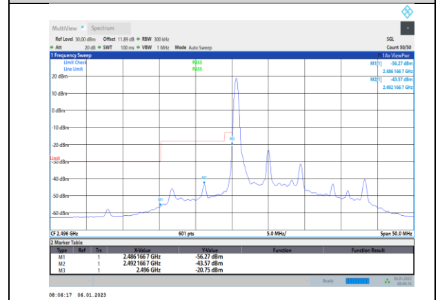
Band41-10MHz-64QAM-39700-50RB#0
