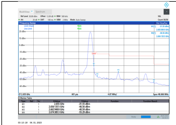
Band41-20MHz-16QAM-41140-100RB#0
