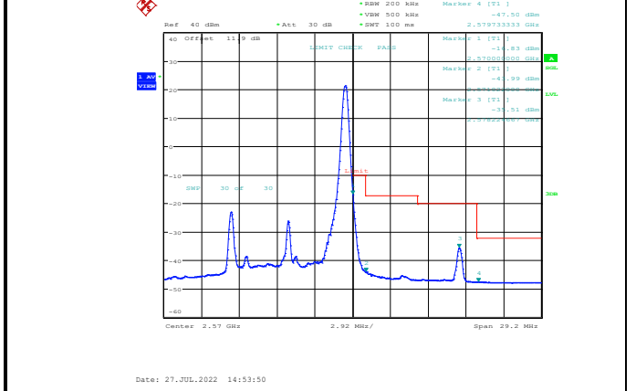
Band7-10MHz-QPSK-21400-1RB#49
