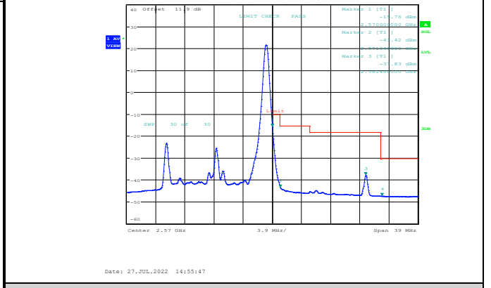
Band7-15MHz-QPSK-21375-1RB#74
