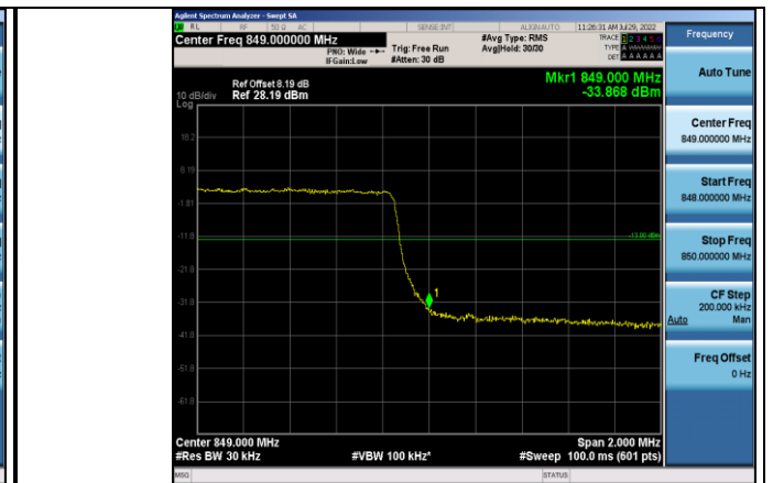
Band5-3MHz-16QAM-20635-15RB#0
