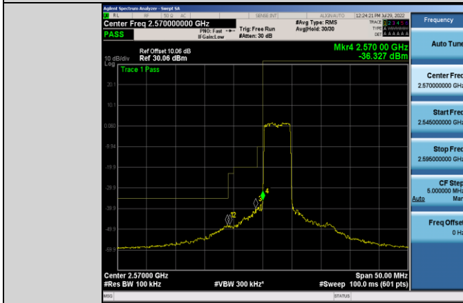
Band38-5MHz-16QAM-37775-25RB#0
