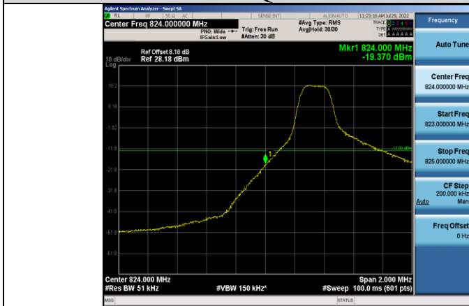
Band5-5MHz-QPSK-20425-1RB#0
