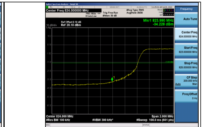
Band5-10MHz-QPSK-20450-50RB#0
