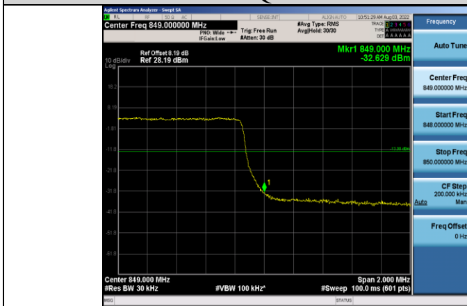
Band5-3MHz-64QAM-20635-15RB#0
