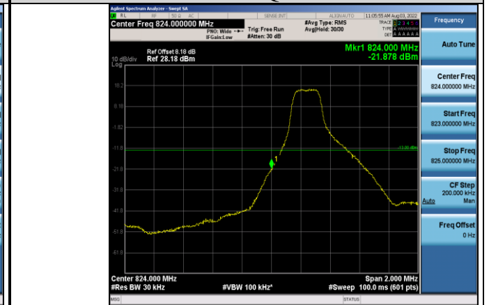
Band5-3MHz-64QAM-20415-1RB#0
