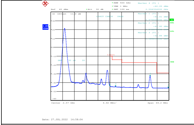
Band7-20MHz-16QAM-21350-1RB#0
