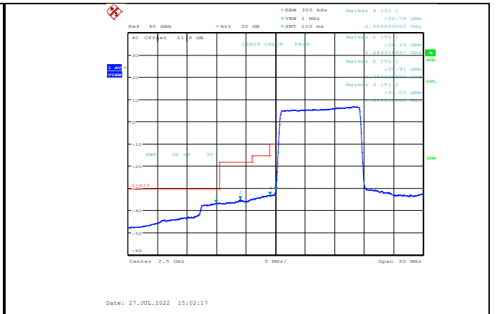
Band7-15MHz-QPSK-20825-75RB#0
