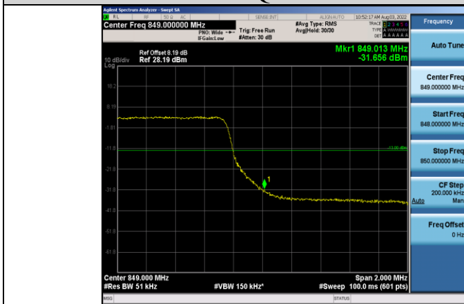
Band5-5MHz-64QAM-20625-25RB#0
