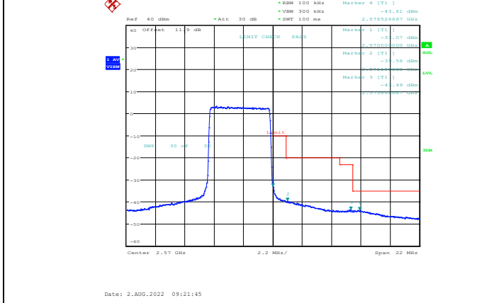
Band7-5MHz-64QAM-21425-25RB#0
