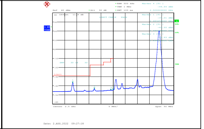
Band7-20MHz-64QAM-20850-1RB#99
