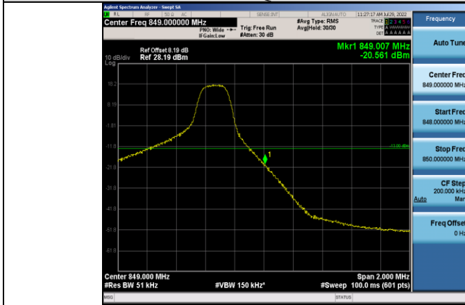
Band5-5MHz-16QAM-20625-1RB#24
