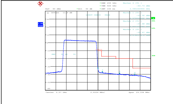
Band7-10MHz-64QAM-21400-50RB#0
