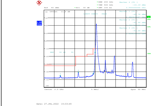
Band7-10MHz-QPSK-20800-1RB#0
