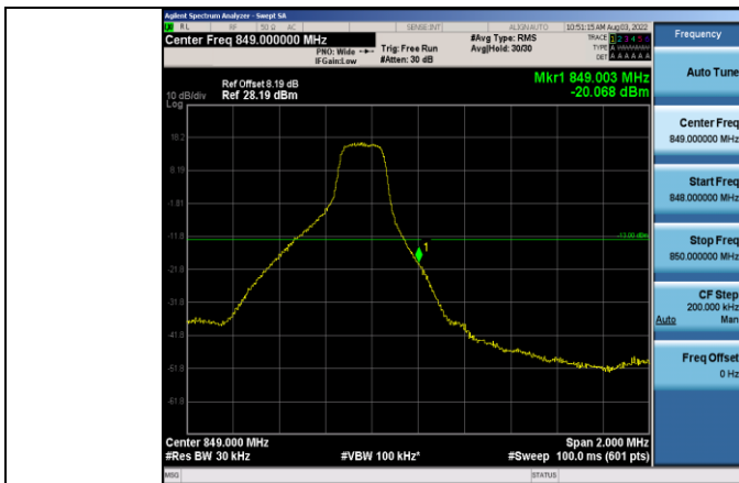
Band5-3MHz-64QAM-20635-1RB#14
