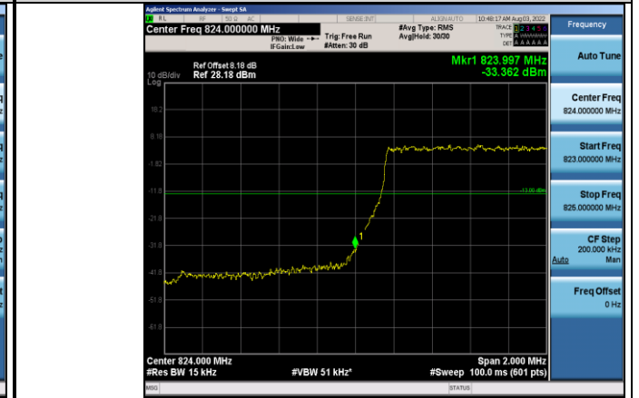
Band5-1.4MHz-64QAM-20407-6RB#0
