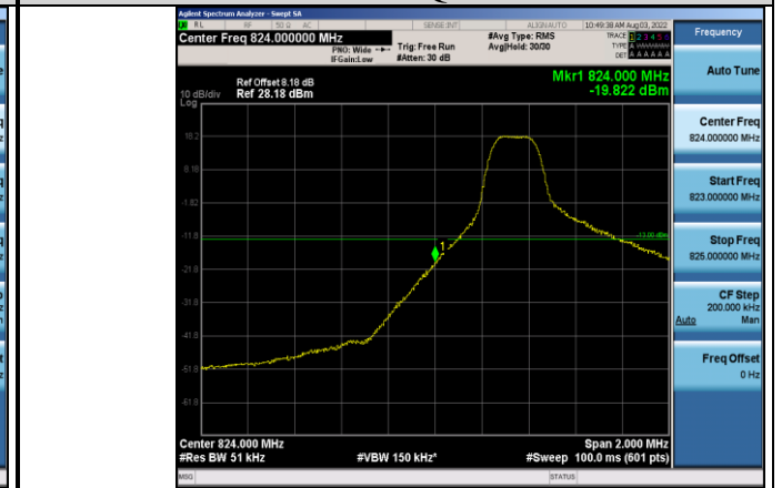
Band5-5MHz-64QAM-20425-1RB#0
