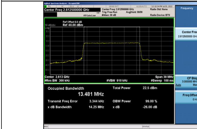
Band38-15MHz-QPSK-38175-75RB#0
