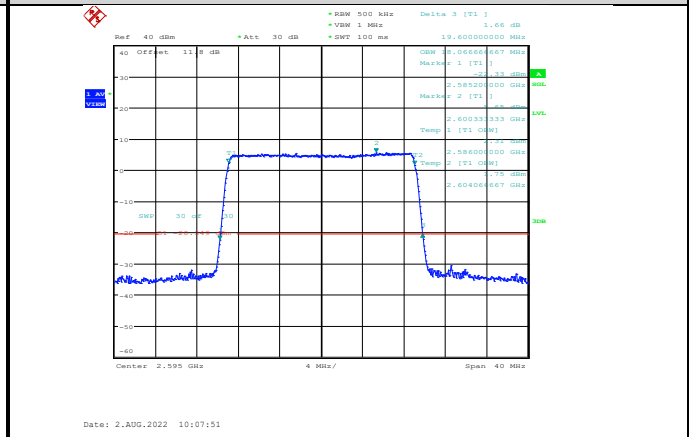
Band38-20MHz-64QAM-38000-100RB#0
