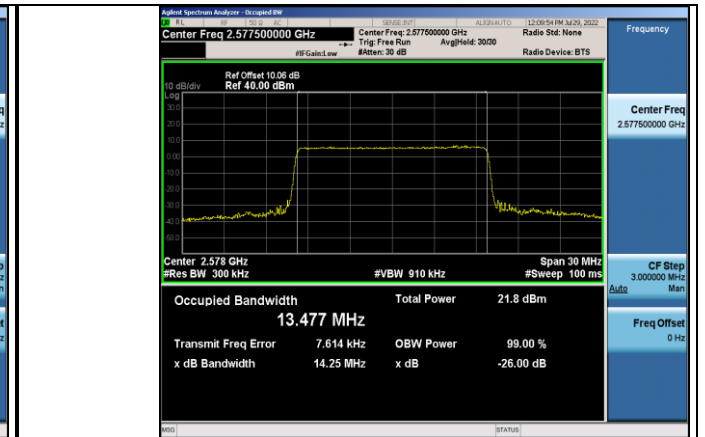
Band38-15MHz-16QAM-37825-75RB#0
