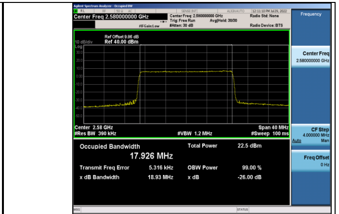
Band38-20MHz-QPSK-37850-100RB#0
