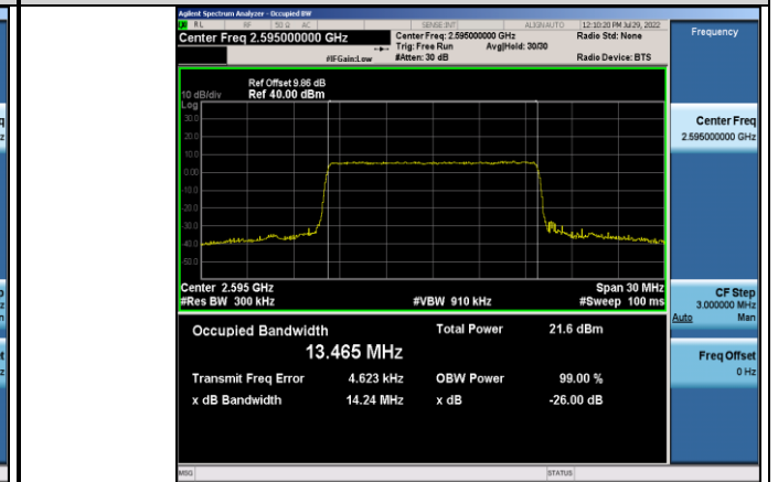
Band38-15MHz-16QAM-38000-75RB#0
