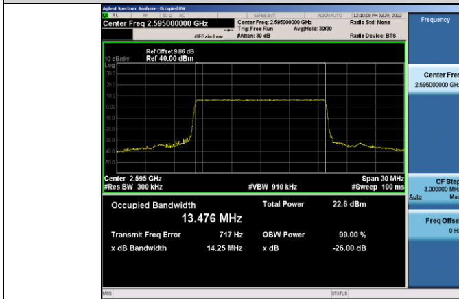
Band38-15MHz-QPSK-38000-75RB#0
