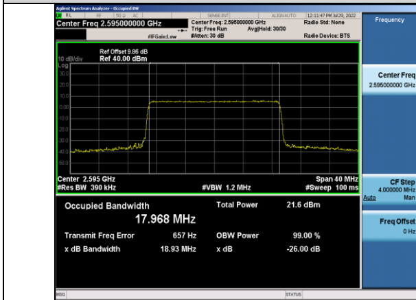
Band38-20MHz-16QAM-38000-100RB#0
