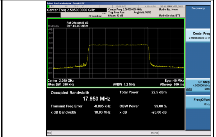
Band38-20MHz-QPSK-38000-100RB#0
