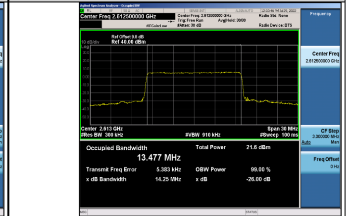
Band38-15MHz-16QAM-38175-75RB#0
