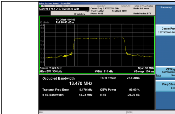
Band38-15MHz-QPSK-37825-75RB#0
