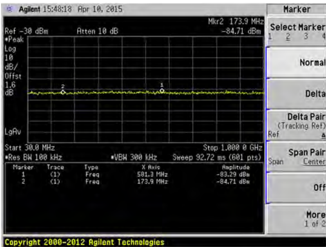
HIGH CHANNEL, SPURIOUS 30 MHz ~ 1 GHz
