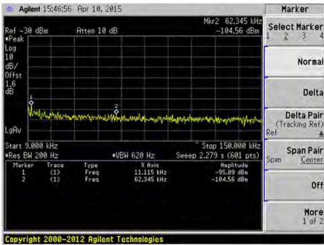
HIGH CHANNEL, SPURIOUS 9 kHz ~ 150 kHz
