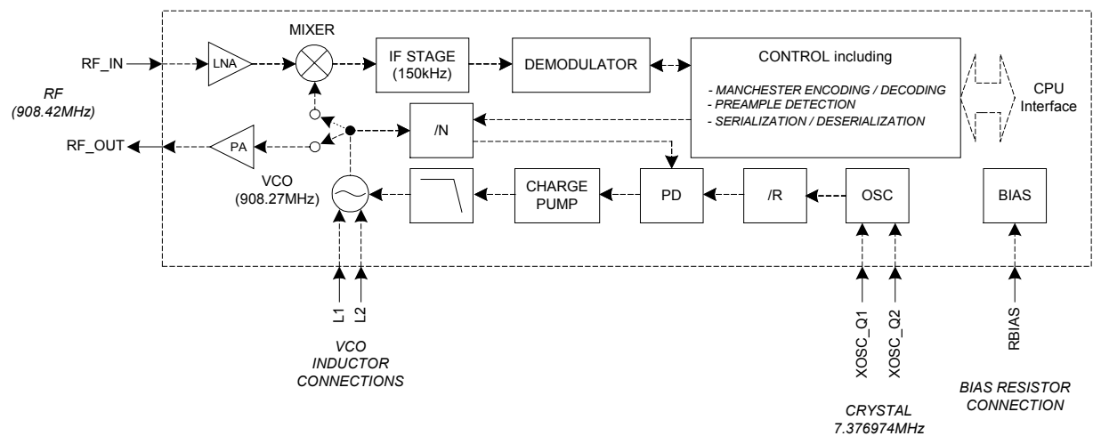
RF Transceiver Block Diagram
