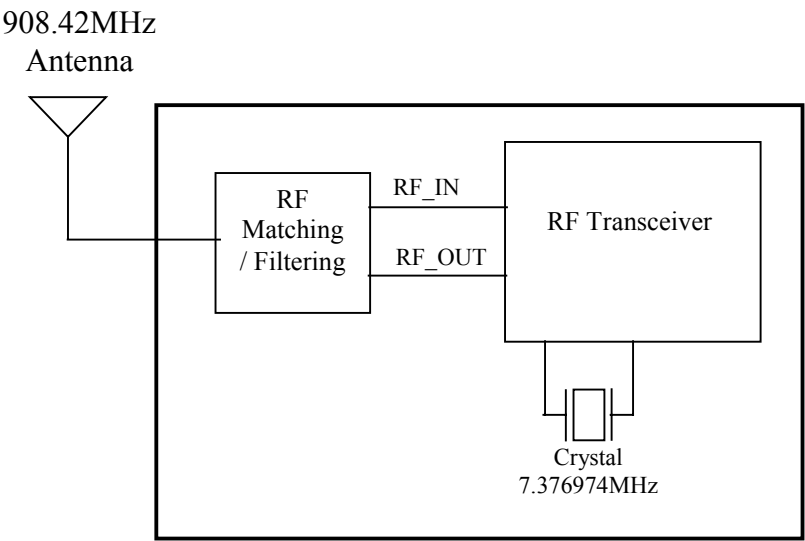
RF Transceiver Block Diagram
