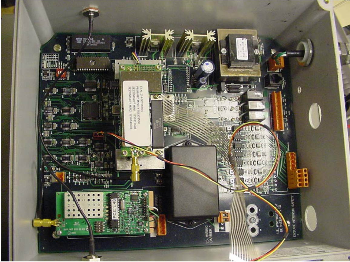
Conducted showing module installed in sample power supply
