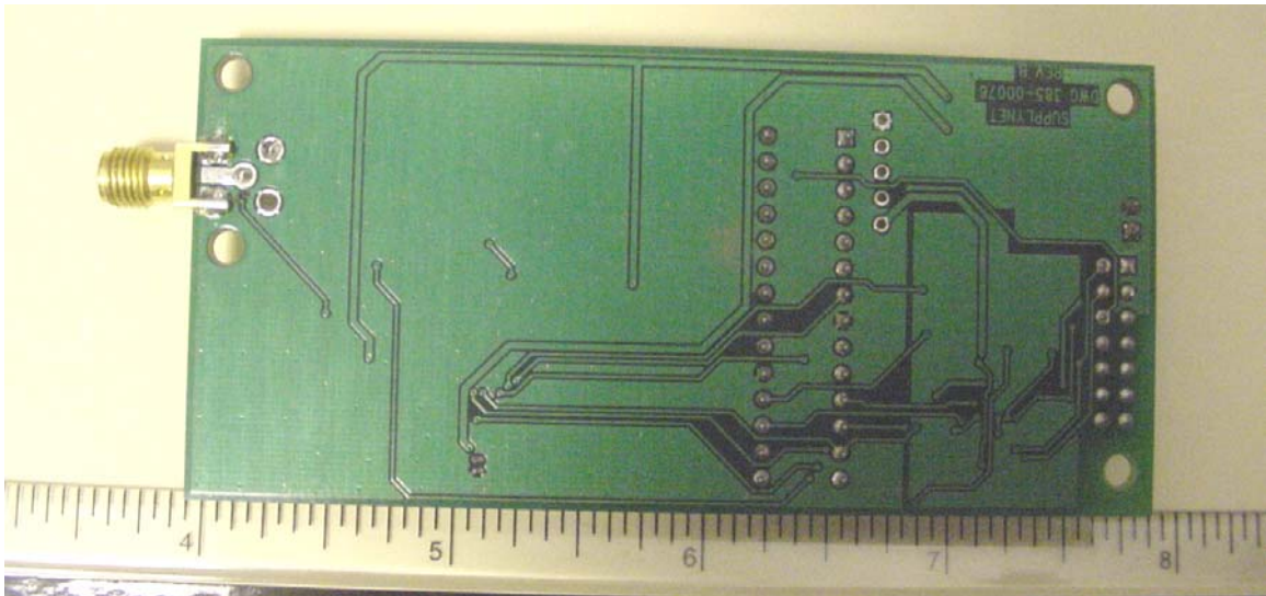
Solder Side
