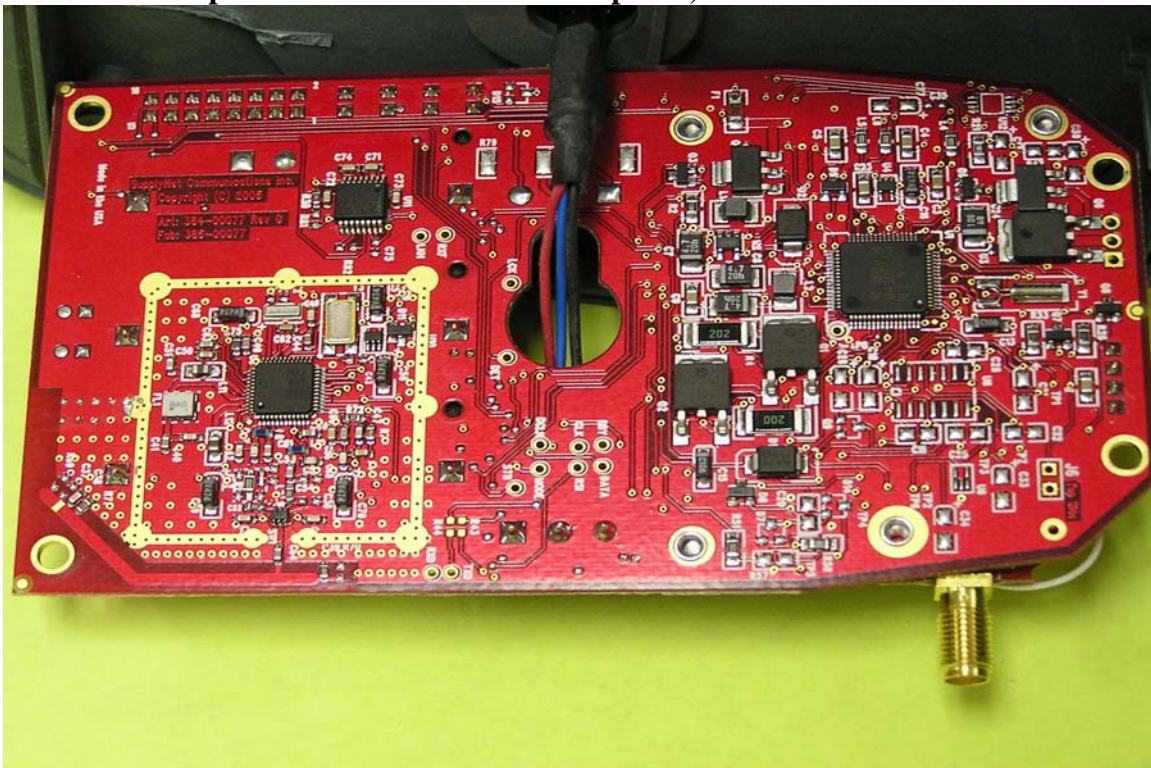
Prophet 4000 Picture 2: Internal photo, Back side PCB Board
