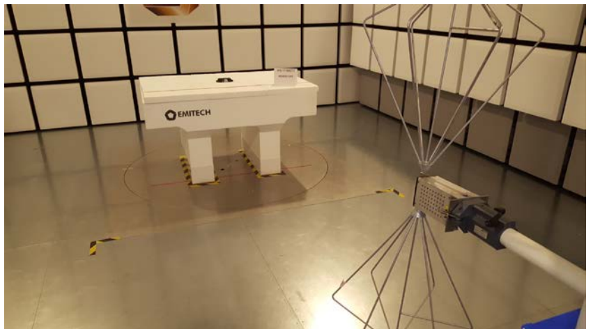
Radiated measurement ( f < 1\text{GHz} )
