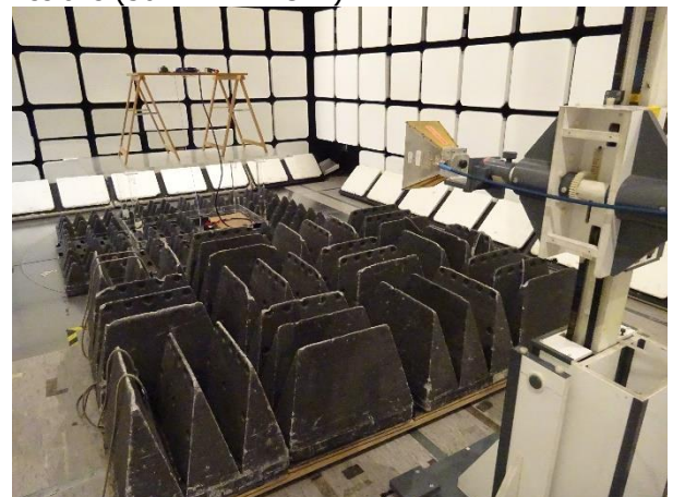
Radio-frequency radiated emissions (1 GHz - 10 GHz)
