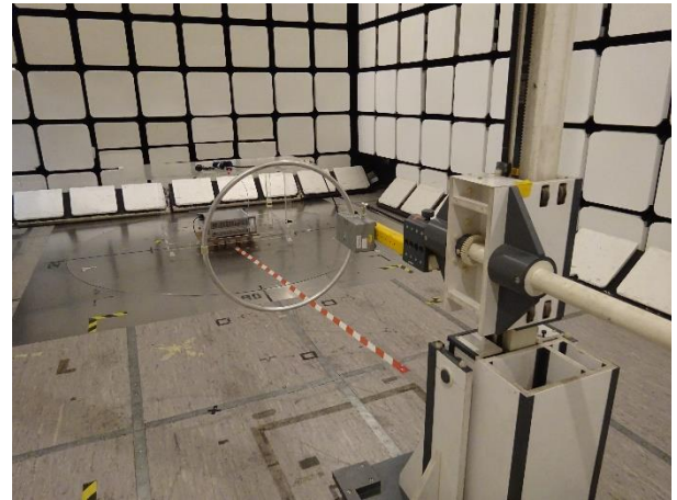
Radio-frequency radiated emissions (9 kHz - 30 MHz).
