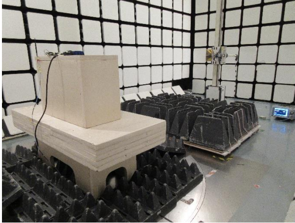
Radio-frequency radiated emissions (10 GHz – 18 GHz)
