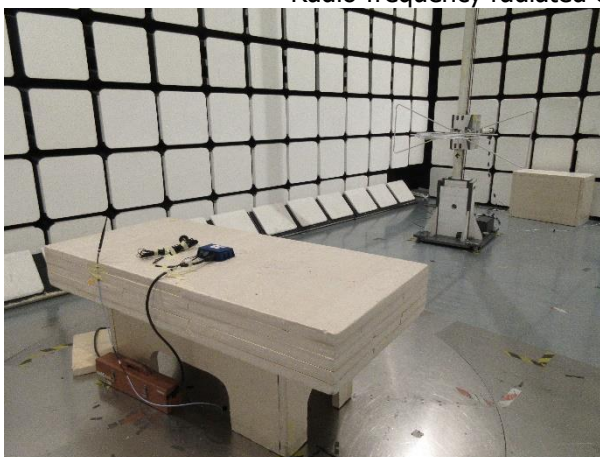
Radio-frequency radiated emissions (30 MHz - 1 GHz)
