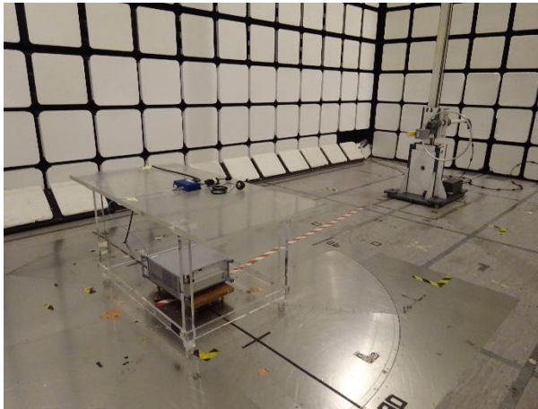
Radio-frequency radiated emissions (9 kHz - 30 MHz).
