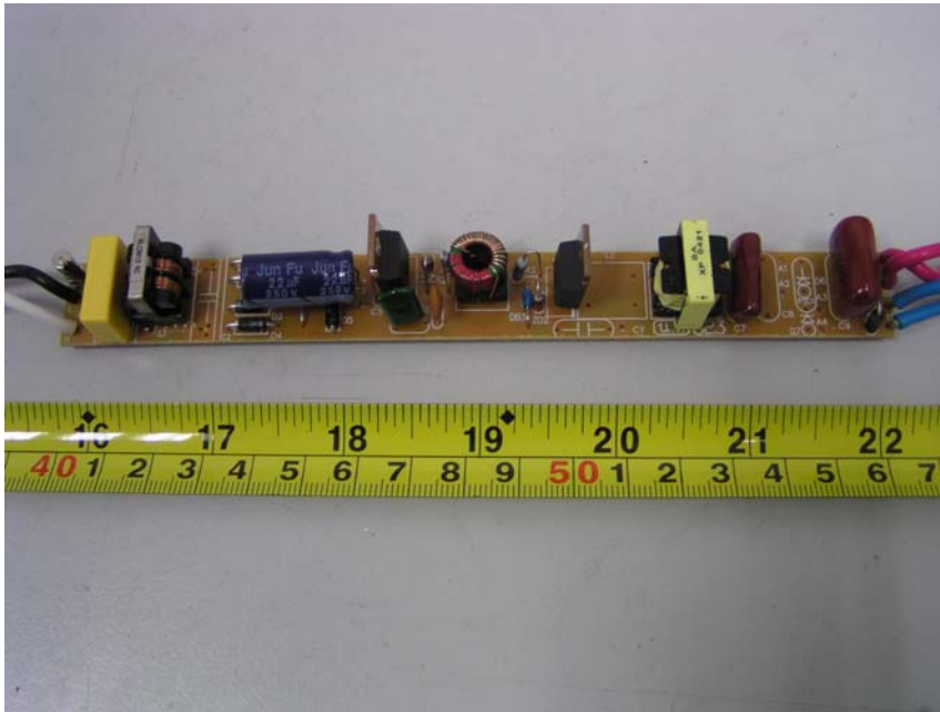
EBA-008L1A-T5: Component View
