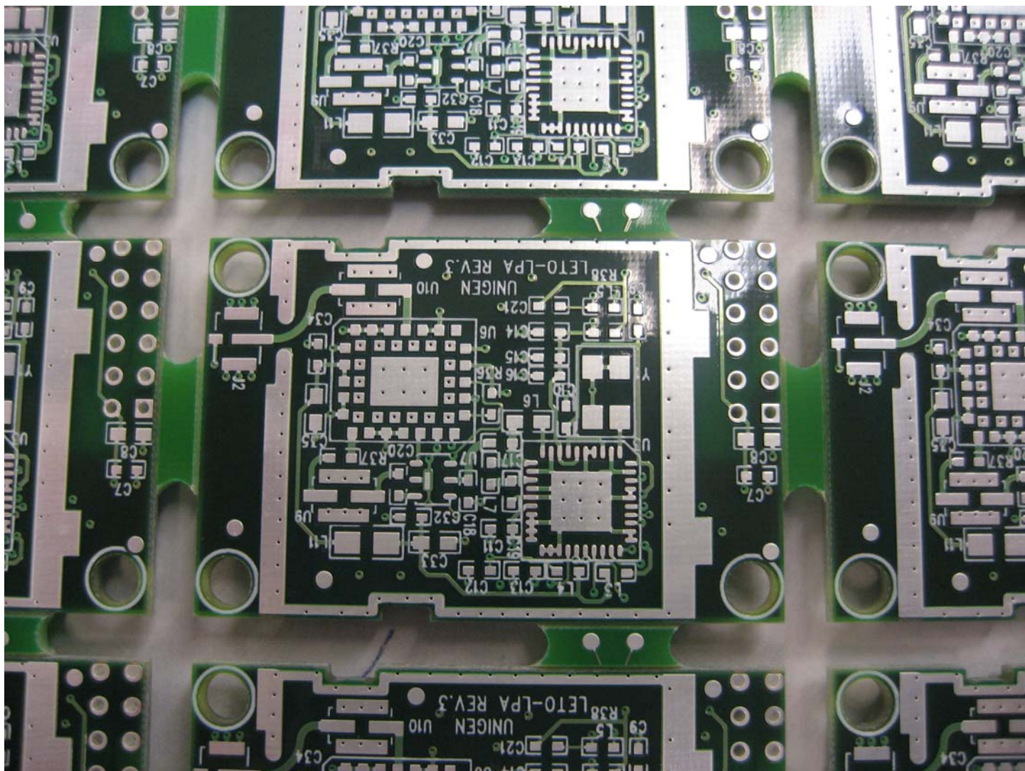
LETO-LPA Photo (internal view)
